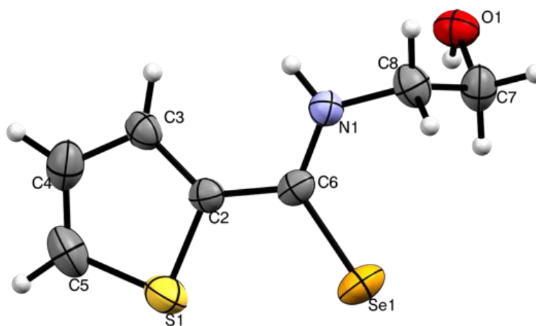
Figure 2. ORTEP representation of selenoamide 3f . Ellipsoids are shown at 30% probability level. Selected bond lengths [ \text{\AA} ] and angles [deg]: \text{Se}(1)\text{-C}(6) 1.836(3), \text{N}(1)\text{-C}(6) 1.321(3), \text{C}(6)\text{-C}(2) 1.453 (3); \text{C}(2)\text{-C}(6)\text{-Se}(1) 120.28 (16), \text{N}(1)\text{-C}(6)\text{-Se}(1) 122.97(17), \text{N}(1)\text{-C}(6)\text{-C}(2) 116.73(19).
