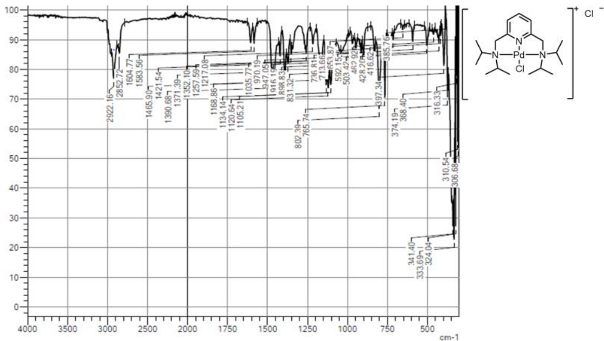
Figure A26: FT-IR of 8b
