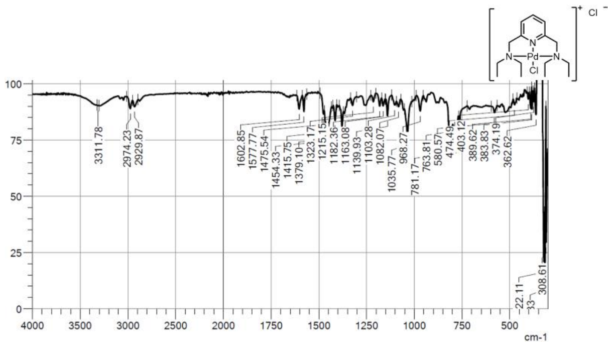
Figure A25: FT-IR of 8a
