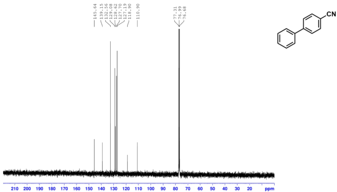
Figure A58: 13 C NMR of 13o recorded in CDCl 3
