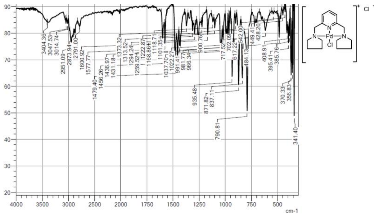
Figure A28: FT-IR of 8d
