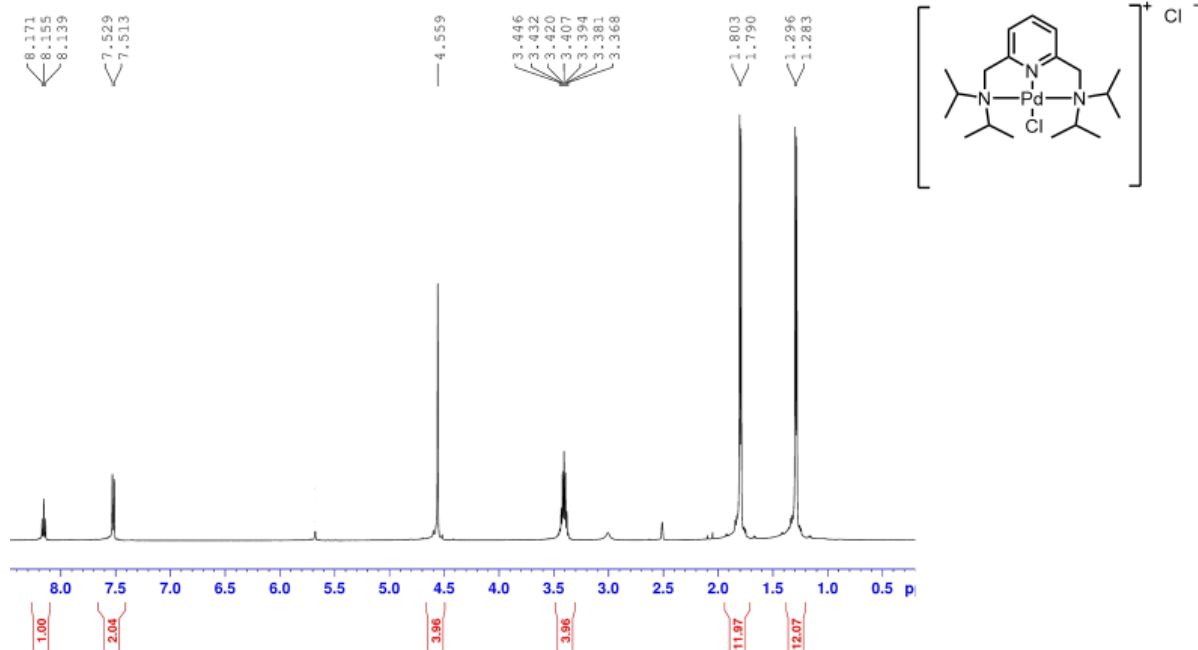
Figure A11: ^1\text{H} NMR of 8b recorded in \text{DMSO-}d_6
