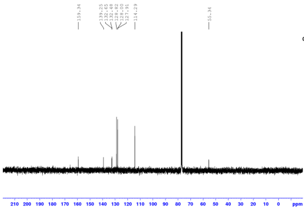
Figure A36: ^{13}\text{C NMR} of 13d recorded in \text{CDCl}_3
