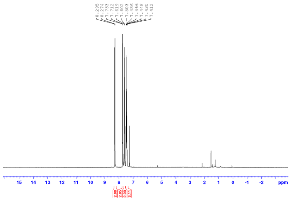
Figure A53: 1 H NMR of 13m recorded in CDCl 3
