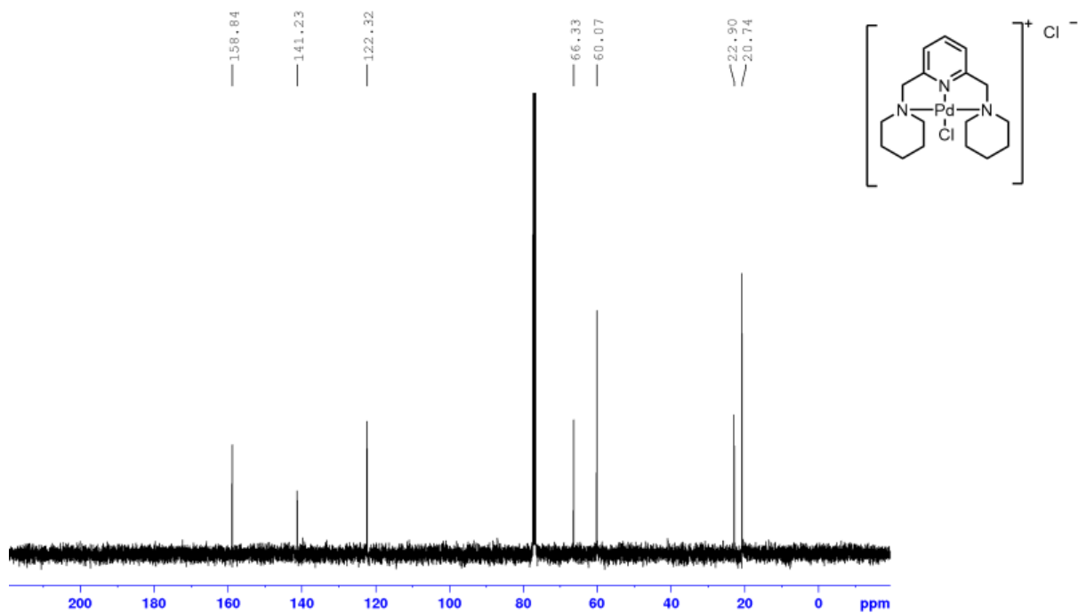
Figure A14: 13 C NMR of 8c recorded in CDCl 3
