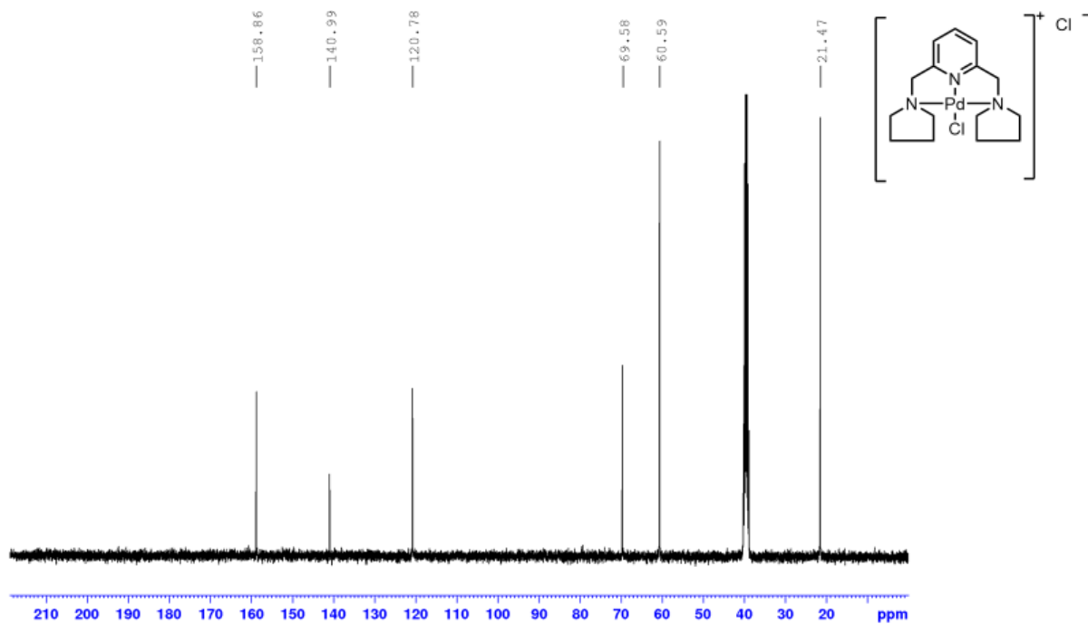
Figure A16: ^{13}\text{C} NMR of 8d recorded in \text{DMSO-}d_6
