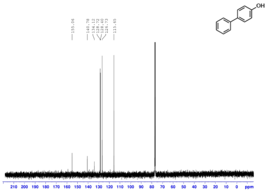
Figure A38: 13 C NMR of 13e recorded in CDCl 3
