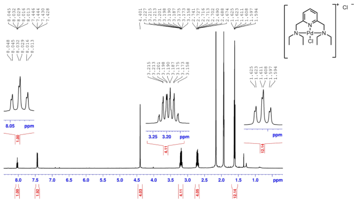
Figure A9: ^1\text{H} NMR of 8a recorded in \text{CD}_3\text{CN}
