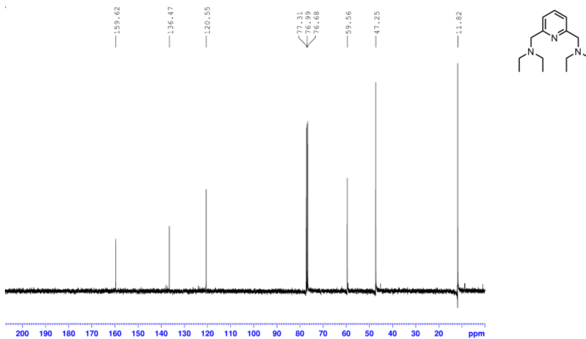
Figure A2: ^{13}\text{C} NMR of 10a recorded in \text{CDCl}_3
