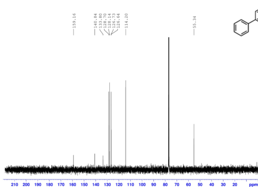
Figure A30: ^{13}\text{C} NMR of 13a recorded in \text{CDCl}_3
