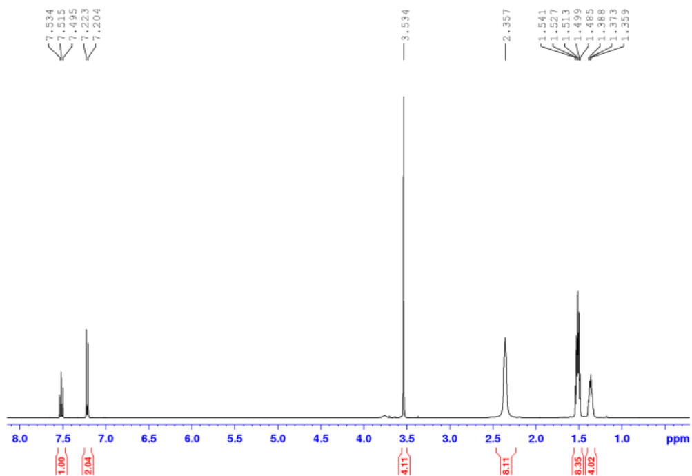
Figure A5: ^1\text{H} NMR of 10c recorded in \text{CDCl}_3
