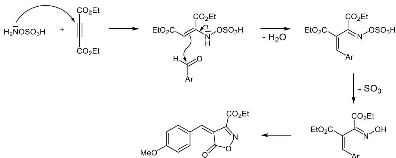
Scheme 2. Plausible mechanism of formation of esters of 4-(arylmethylene)-5-oxo-4,5-dihydroisoxazole-3-carboxylic acids.
