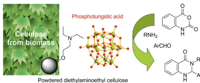
Scheme 5. Biopolymer-supported solid acidic catalyst for the synthesis of 2,3-dihydroquinazolin-4(1H)-ones from isatoic anhydride, amines, and aldehydes. (From ref. 58 Monatsh. Chem. 2015 , 146 , 1859-1864)
