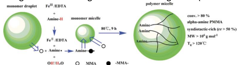
Scheme 1. Radical polymerization of methyl methacrylate (MMA). (From ref. 11 Macromol. React. Eng. 2016 , 10 , 269-279)
