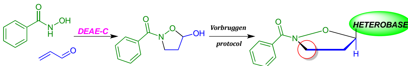
Scheme 9. Vorbrüggen protocol to nucleoside analogues
