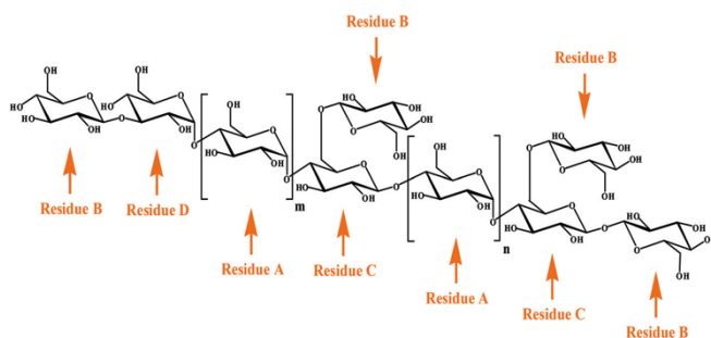
Figure 5. Structure of Polysaccharides of type PL70-1-1. (From ref. 12 Food Funct. 2018 , 9 , 2644-2652)
