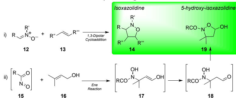
Scheme 7. General approaches to Isoxazolidines and 5-hydroxy-isoxazolidines.
