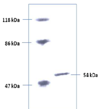
Figure 8. SDS-PAGE of purified GI (20 \mu g) produced by S. albaduncus . Lane 1: Molecular mass standards ( \beta -galactosidase, 118 kDa; Bovine serum albumin, 86 kDa; ovalbumine, 47 kDa). Lane 2: purified GI enzyme produced by S. albaduncus . (From ref.36 Afr. J. Microbiol. Res. 2013 , 7, 2682-2688)
