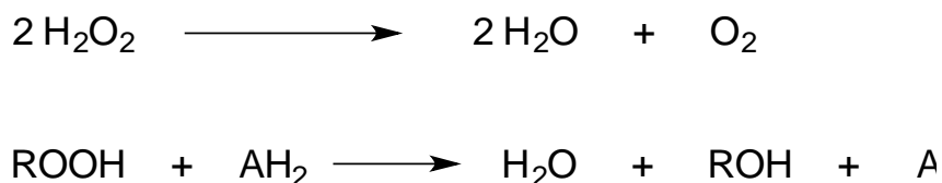
Scheme 3. Catalyzed reduction of hydroperoxides.
