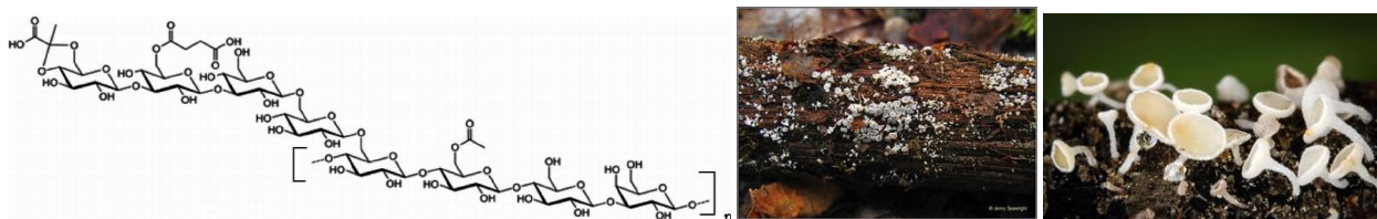
Figure 4. Structure of exopolysaccharide (pictures of Lachnum ).
