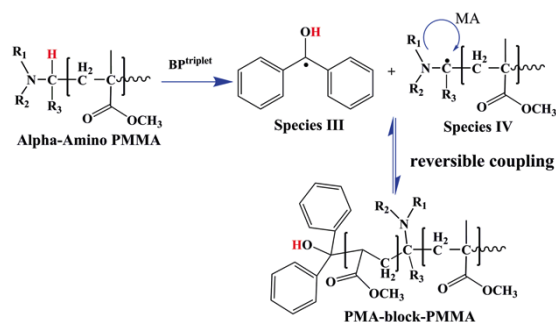
Scheme 2. UV-induced BP-initiated radical polymerization of MA using the alpha-amino poly methylmethacrylate (PMMA). (From ref. 11 Macromol. React. Eng. 2016 , 10 , 269-279)
