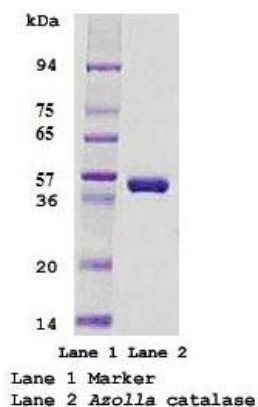
Figure 7. Molecular mass of purified catalase. (From ref. 32 Int. J. Curr. Microbiol. Appl. Sci. 2016 , 5, 836-844)
