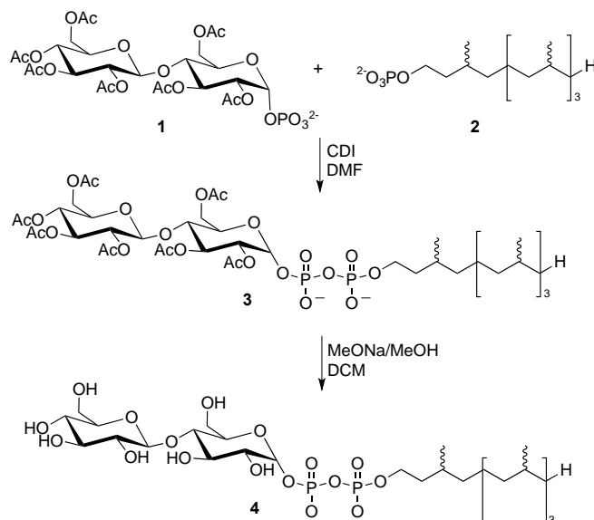
Scheme 4. Synthesis of \alpha -D-cellobiosyldiphosphate 4 .
