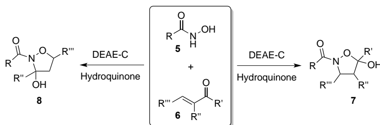
Scheme 6. Synthesis of 3- and 5-hydroxyisoxazolidines 7 and 8 by reaction of hydroxylamines 5 and \alpha,\beta -unsaturated carbonyl compounds 6 .
