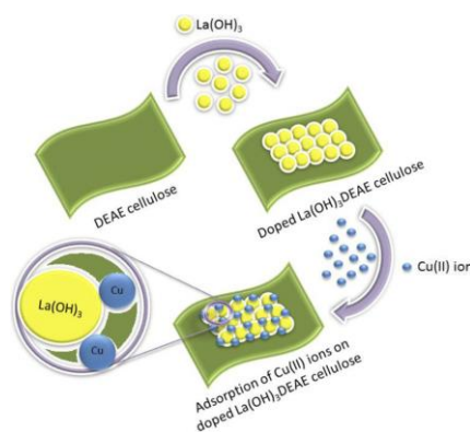
Figure 10. Schematic view of adsorption on modified DEAE-C. (From ref. 59 Nanoscale Res. Lett. 2014 , 9 , 466)
