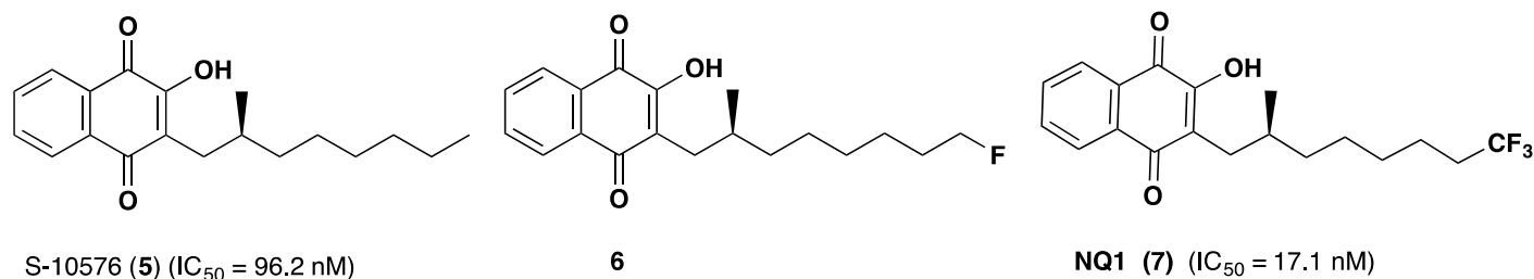
Figure 2. Structures of antimalarial naphthoquinones 5-7 .
