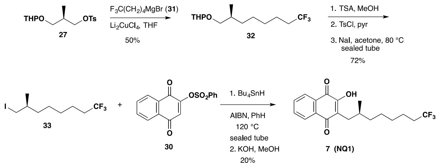
Scheme 4. Synthesis of ( S )-2-hydroxy-3-(8,8,8-trifluoro-2-methyloctyl)naphthalene-1,4-dione ( 7 ) (NQ1).
