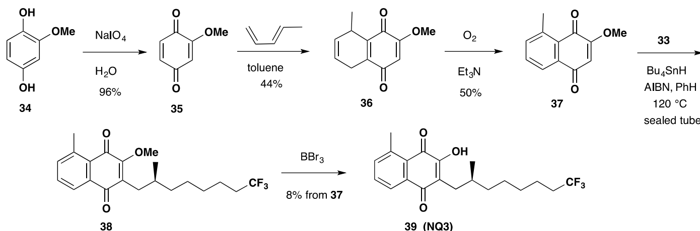
Scheme 5. Synthesis of ( S )-3-hydroxy-5-methyl-2-(8,8,8-trifluoro-2-methyloctyl)naphthalene-1,4-dione ( 39 ) (NQ3).
