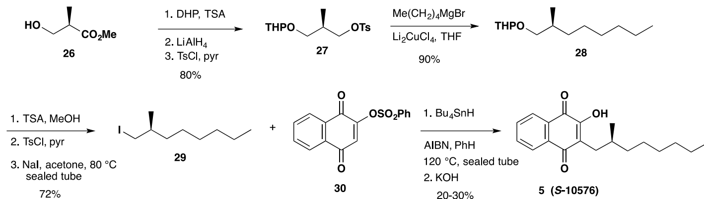
Scheme 3. Synthesis of ( S )-2-hydroxy-3-(2-methyloctyl)naphthalene-1,4-dione ( 5 ) (S-10576).
