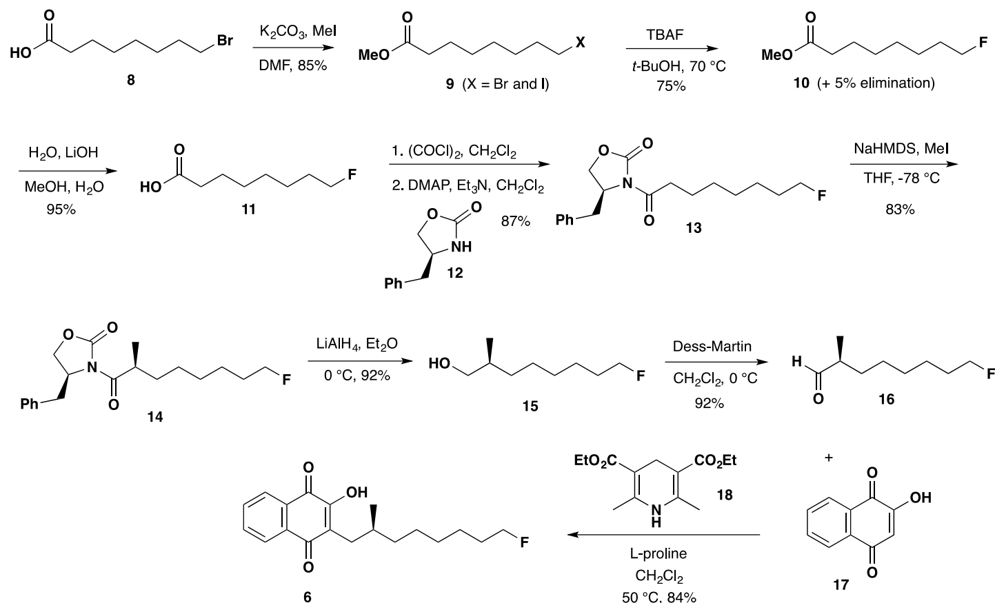
Scheme 1. Synthesis of ( S )-2-(8-fluoro-2-methyloctyl)-3-hydroxynaphthalene-1,4-dione ( 6 ). 17
