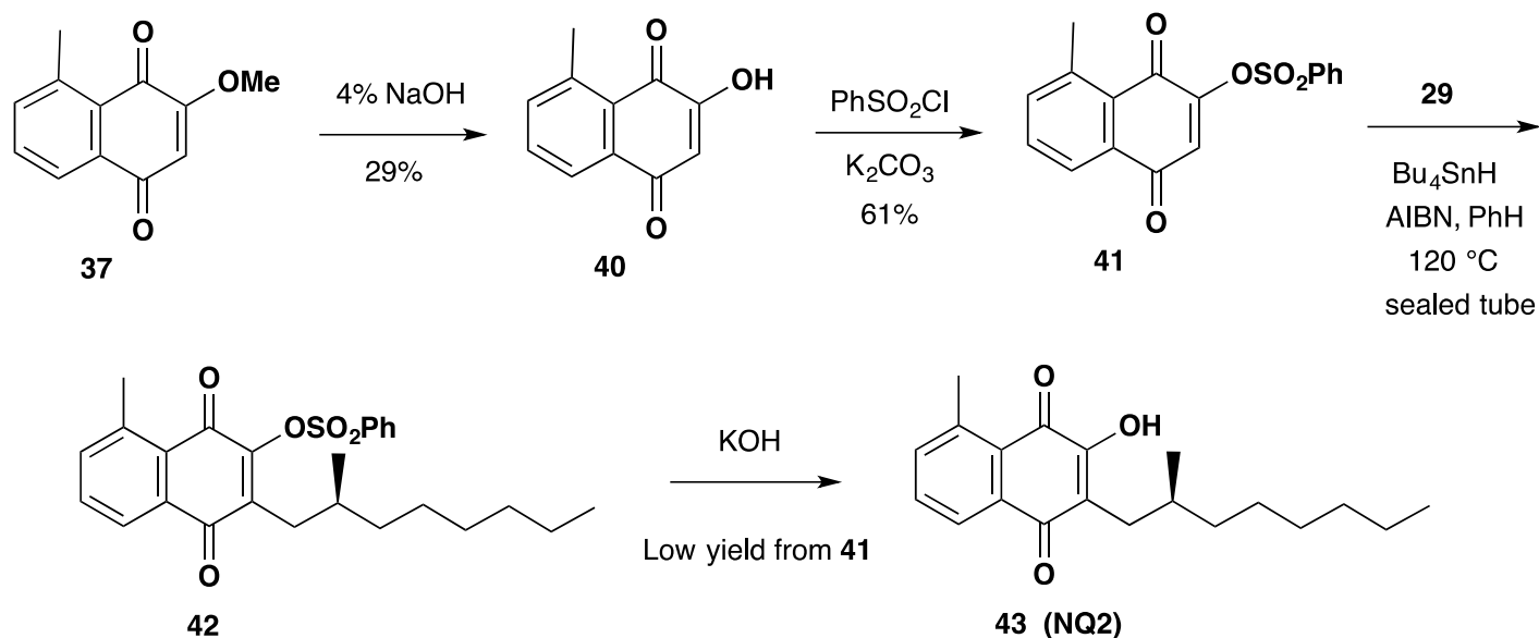
Scheme 6. Synthesis of ( S )-3-hydroxy-5-methyl-2-(2-methyloctyl)naphthalene-1,4-dione ( 43 ) (NQ2).
