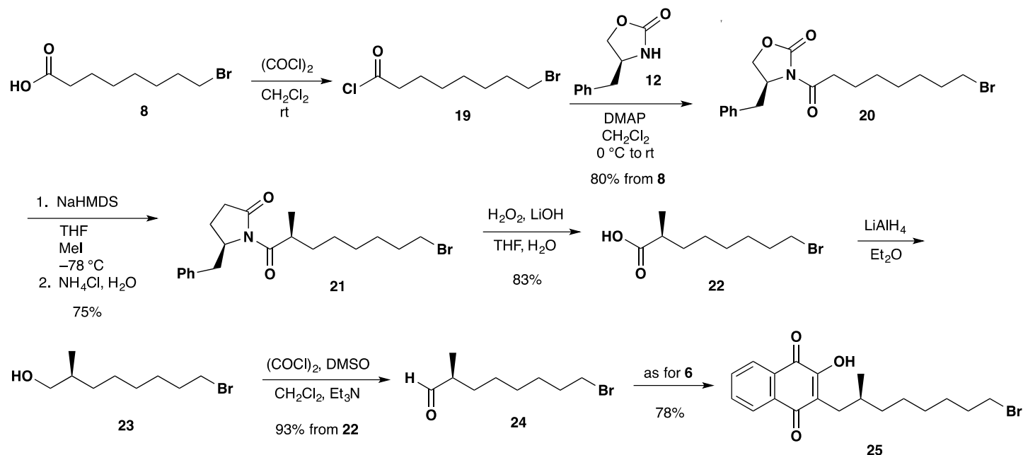
Scheme 2. Synthesis of ( S )-2-(8-bromo-2-methyloctyl)-3-hydroxynaphthalene-1,4-dione ( 25 ).
