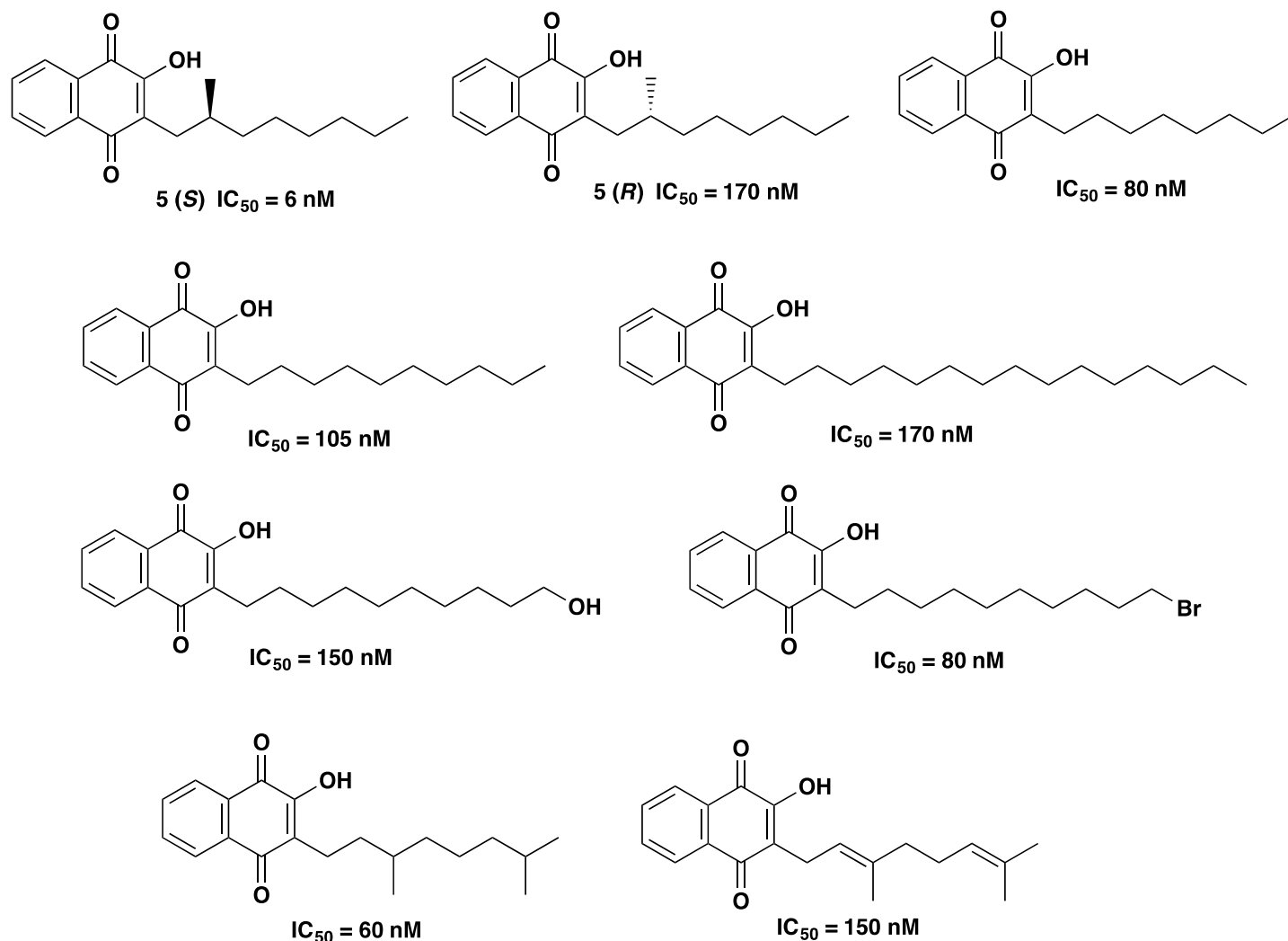
Figure 3. Structures of 2-hydroxynaphthalene-1,4-diones and IC_{50} (nM) against the yeast bc1 complex.
