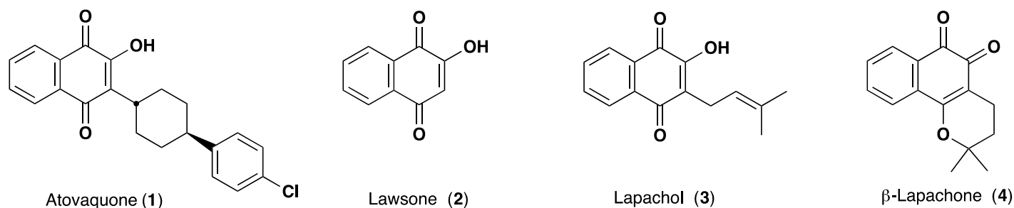
Figure 1. Structures of antimalarial naphthoquinones 1-4 .
