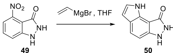
Scheme 7. Synthesis of pyrrolo[2,3- e ]indazole-3-one 50 . 26
