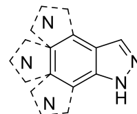
Pyrroloindazole regioisomers
