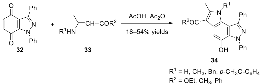
Scheme 5. Nenitzescu indole synthesis applied to the preparation of compounds 34 . 23
