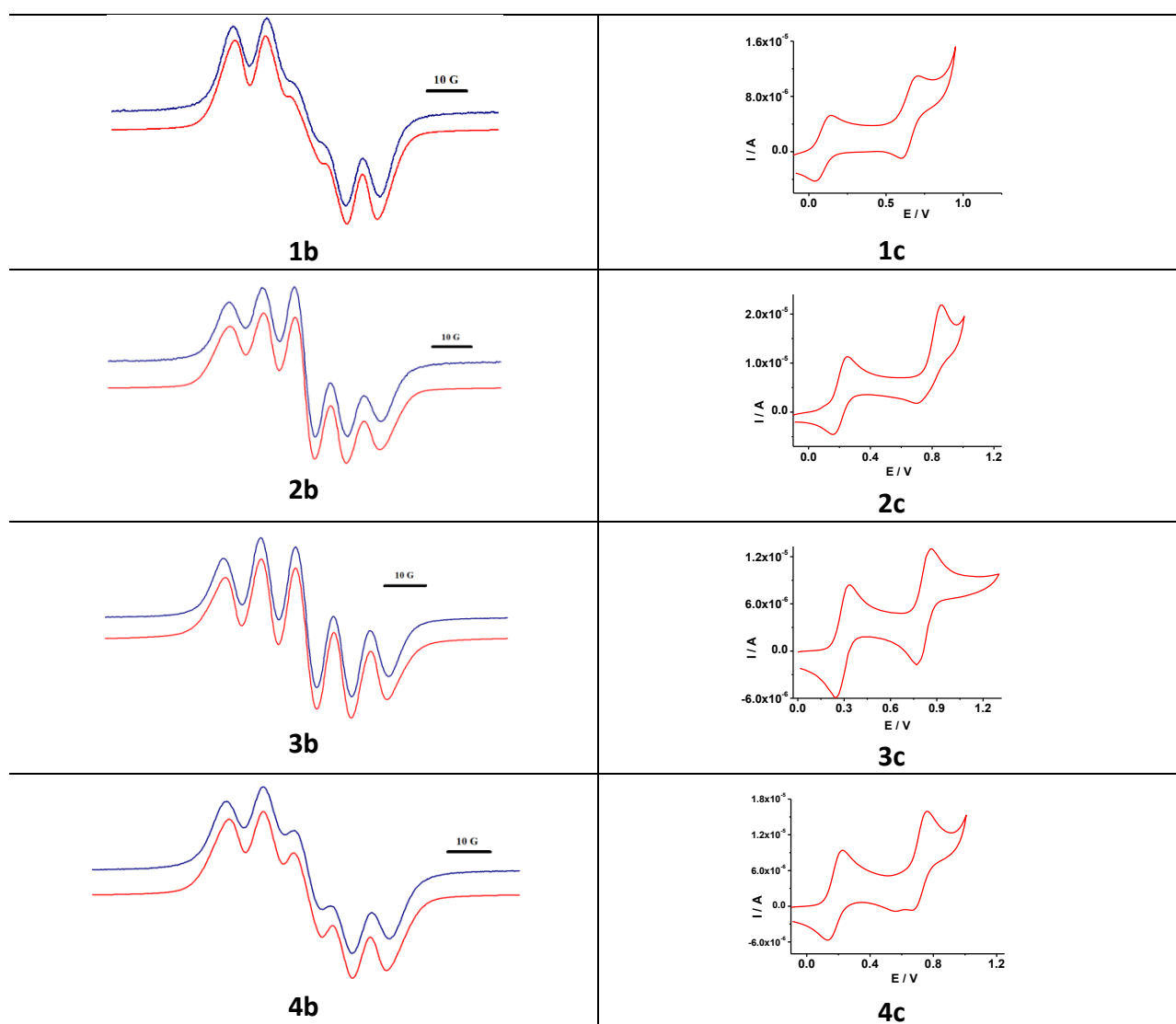
Figure 4. ESR spectra (left), of free radicals 1b-5b (experimental-blue, simulated-red), and CVs (right), of anions 1c-5c .
