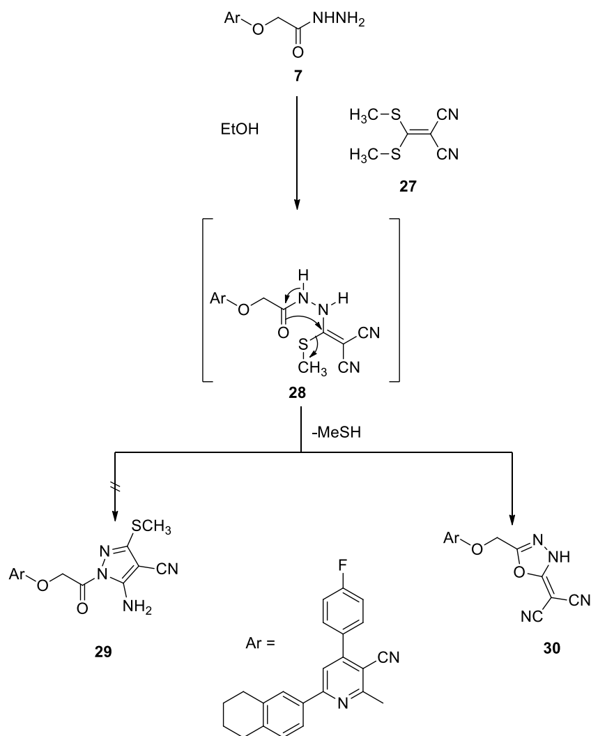
Scheme 6. Synthesis of compound 30 from acetohydrazide 7 .
