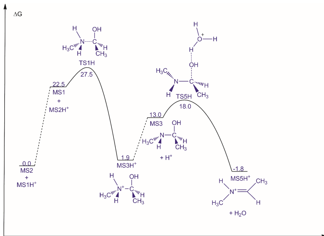
Figure 6. Free energy profile for carbinolamine formation and decomposition in acid medium (formation of E-isomer). Units in kcal mol -1 , standard state of 1 mol L -1 for all species but water, whose standard state is pure liquid.
