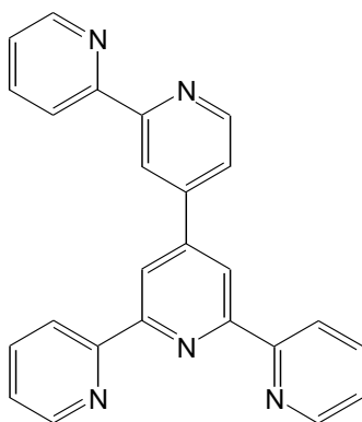
Figure 1. 4'-(2,2'-bipyridin-4-yl)-2,2':6'-2''-terpyridine ligand. 3
