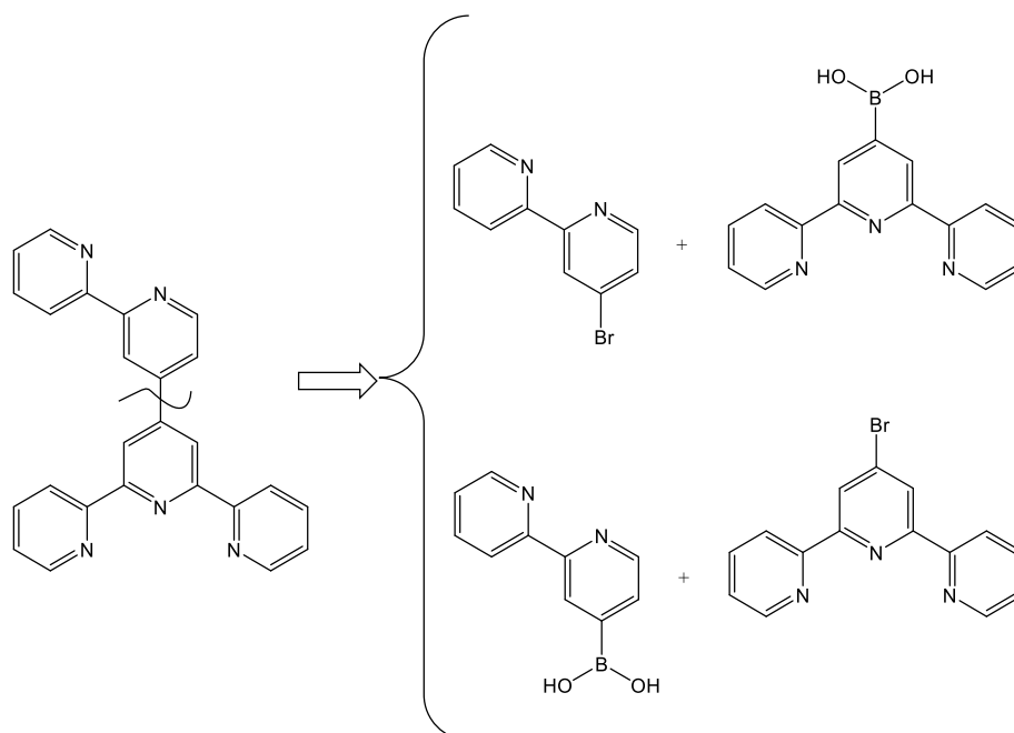
Figure 2. Proposed disconnection approach for the synthesis of 4'-(2,2'-bipyridin-4-yl)-2,2':6'-2''-terpyridine ligand.
