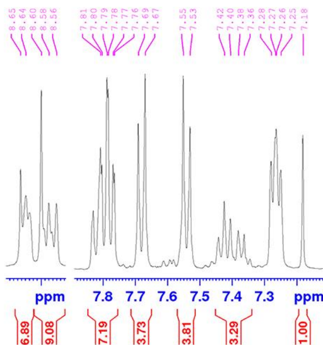
Figure 3. 1 H NMR spectrum of ligand ( I ) in CDCl 3 .
