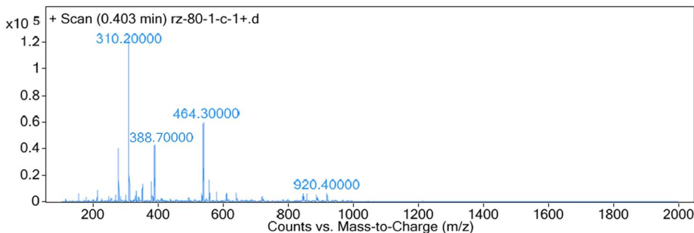
Figure 5. LC-MS of the ligand (I) in CDCl 3 showed a pick at m/z 464.3 ([M+H] + ) and a peak at m/z 388.7 ([M – C 5 H 4 N + H] + ).
