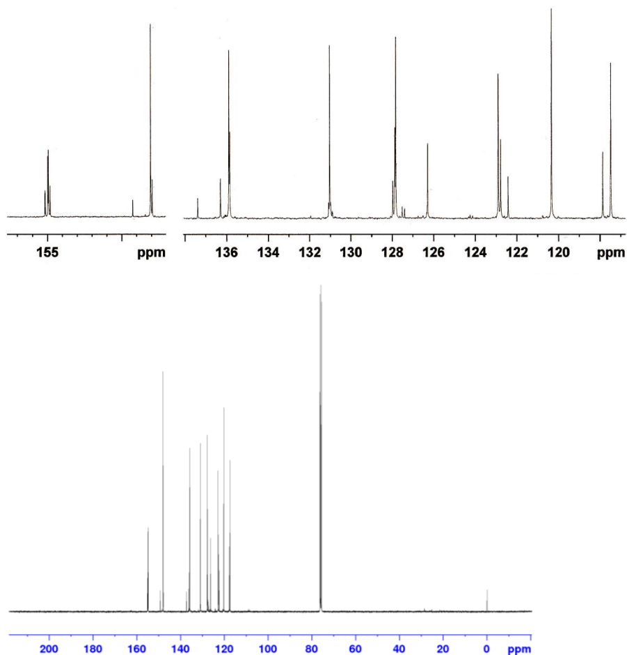
Figure 4. ^{13}\text{C} NMR of ligand (I) in \text{CDCl}_3 .
