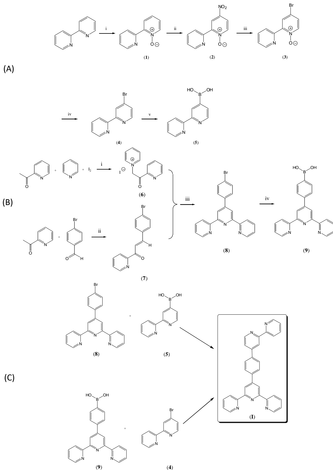
Scheme 1. (A) (i) m -chloroperbenzoic acid, \text{CH}_3\text{Cl} , 0 °C then r.t., 18 h; (ii) \text{H}_2\text{SO}_4 , \text{HNO}_3 , 105 °C, 5 h; (iii) acetyl bromide, HOAc, 60 °C, 2 h; (iv) \text{PBr}_3 , \text{CHCl}_3 , 0 °C then reflux, under Ar; (v) triisopropyl borate, n -butyl lithium, THF, -78 °C, under Ar; (B) (i) 105-110 °C; (ii) aq. NaOH, MeOH, 30 min, rt; (iii) \text{NH}_4\text{OAc} , glacial acetic acid, reflux, 7 h, NaOH; (iv) triisopropyl borate, n -butyl lithium, THF, -78 °C, under Ar; (C) \text{Pd}(\text{PPh}_3)_4 , aq. \text{Na}_2\text{CO}_3 , under Ar, reflux, overnight.
