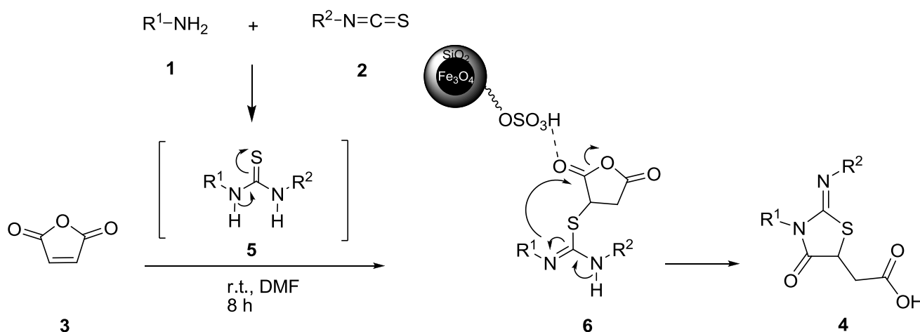
Scheme 1. Mechanistic rationalization for the formation of product 4 .
