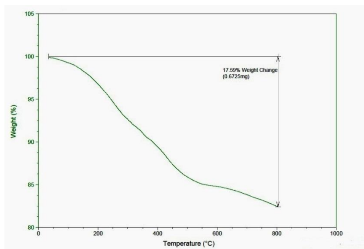
Figure 3. TGA analysis of the \text{Fe}_3\text{O}_4@\text{SiO}_2\text{-SO}_3\text{H} .
