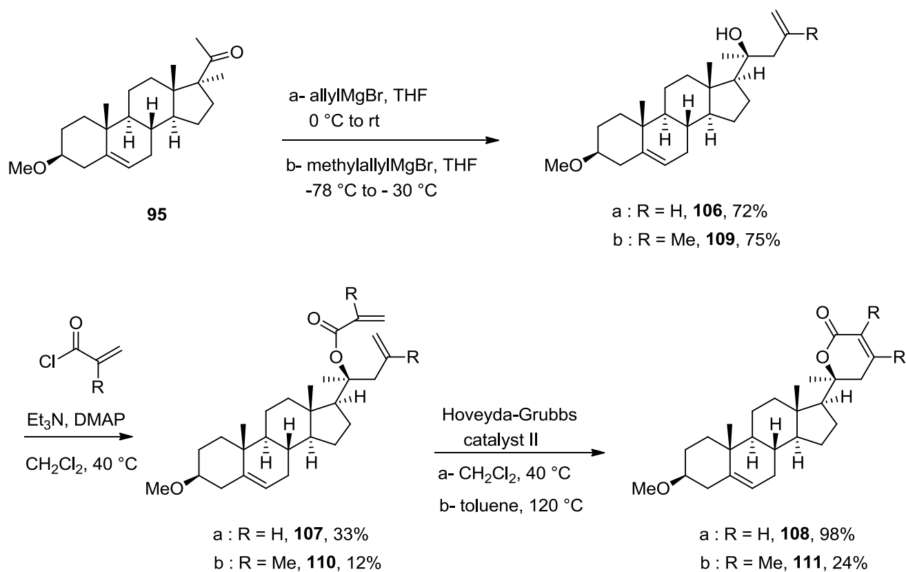
Scheme 23. Synthesis of the dihydropyrones 108 , 111 by RCM reactions
