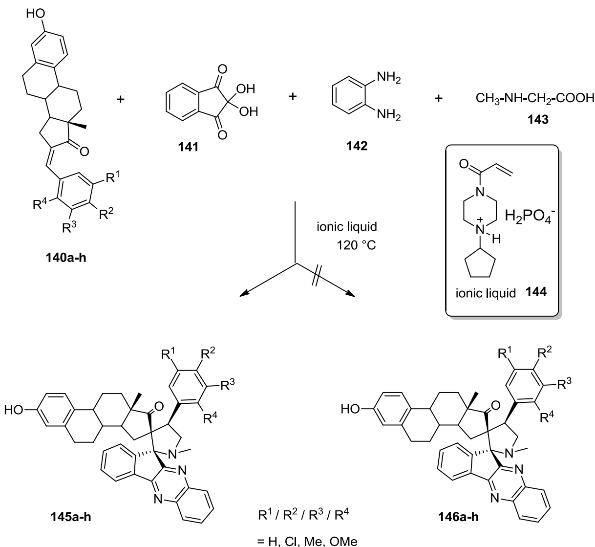
Scheme 31. Synthesis of steroidal spiro-indenoquinoxaline-pyrrolidines 145a-h .
