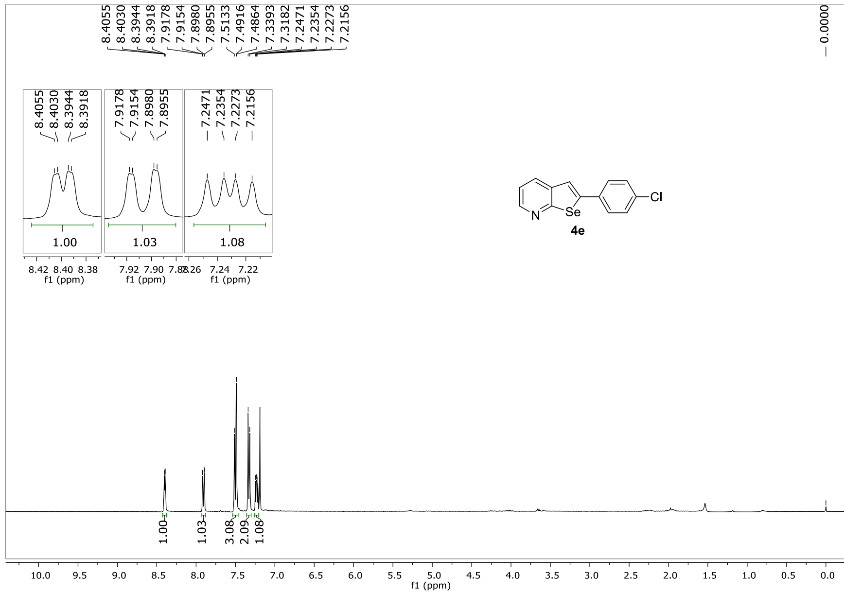
Figure 9: 1 H NMR (400 MHz, CDCl 3 ) spectrum of compound 4e .
