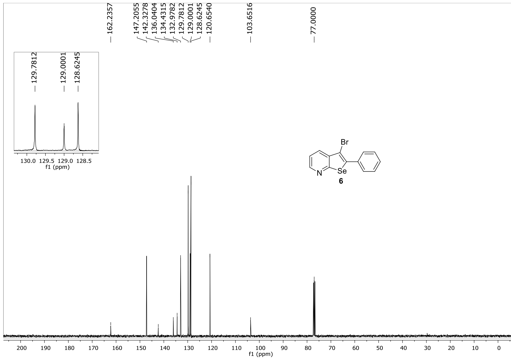
Figure 20: 13 C NMR (100 MHz, CDCl 3 ) spectrum of compound 6.
