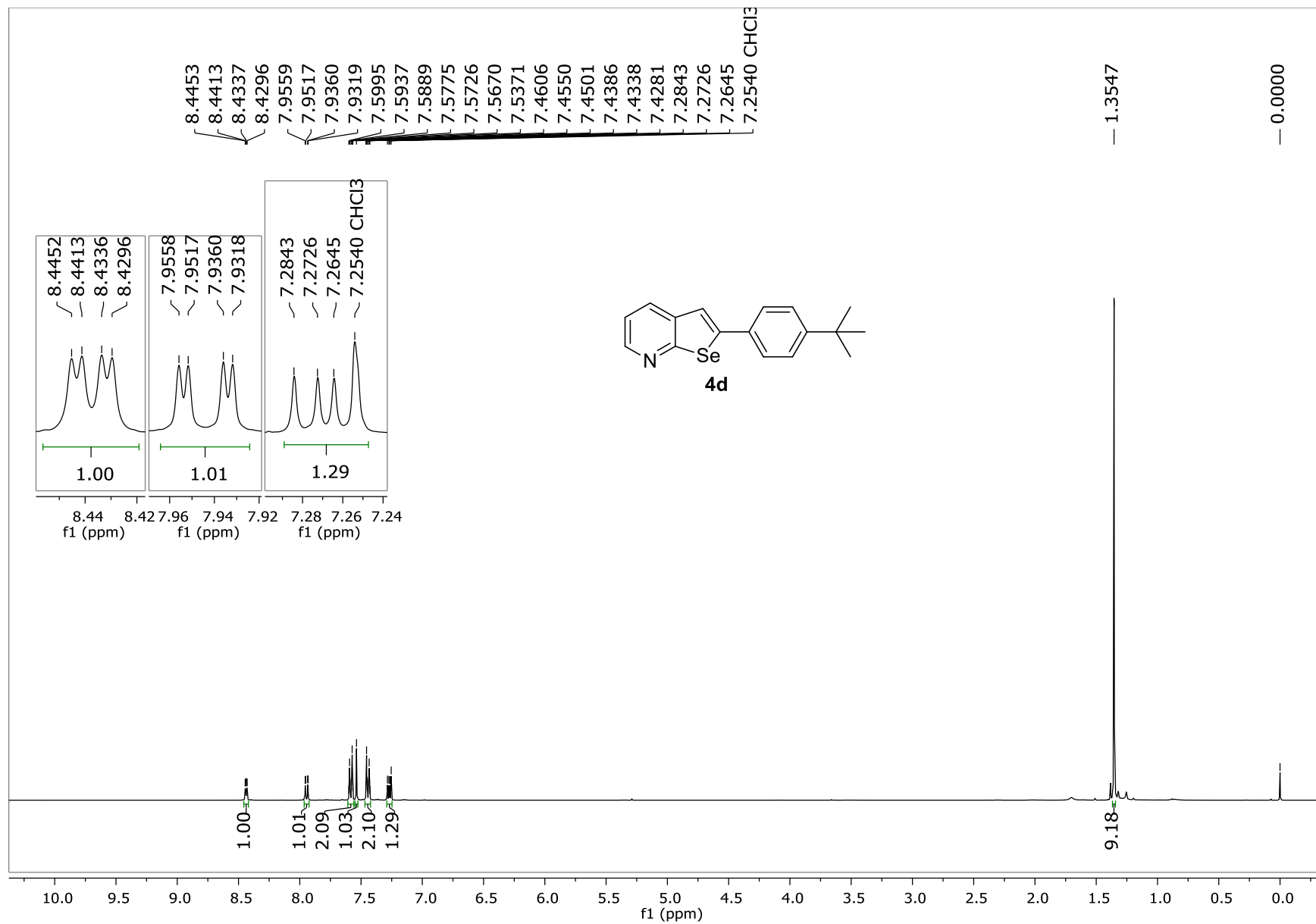
Figure 7: ^1\text{H} NMR (400 MHz, \text{CDCl}_3 ) spectrum of compound 4d .
