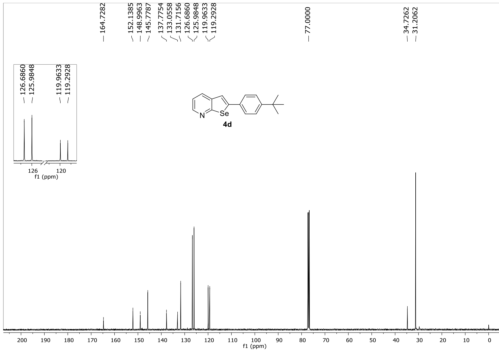
Figure 8: 13 C NMR (100 MHz, CDCl 3 ) spectrum of compound 4d .
