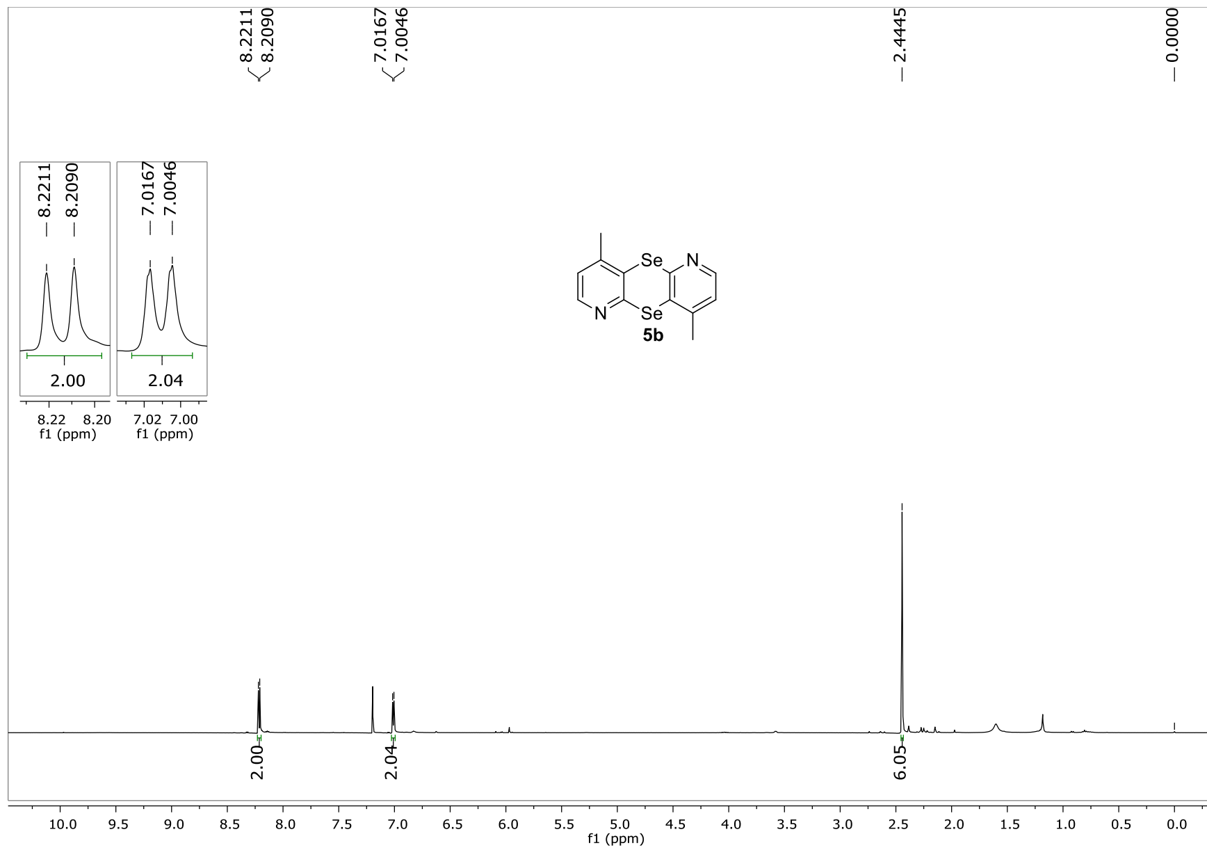
Figure 15: ^1\text{H} NMR (400 MHz, \text{CDCl}_3 ) spectrum of compound 5b .
