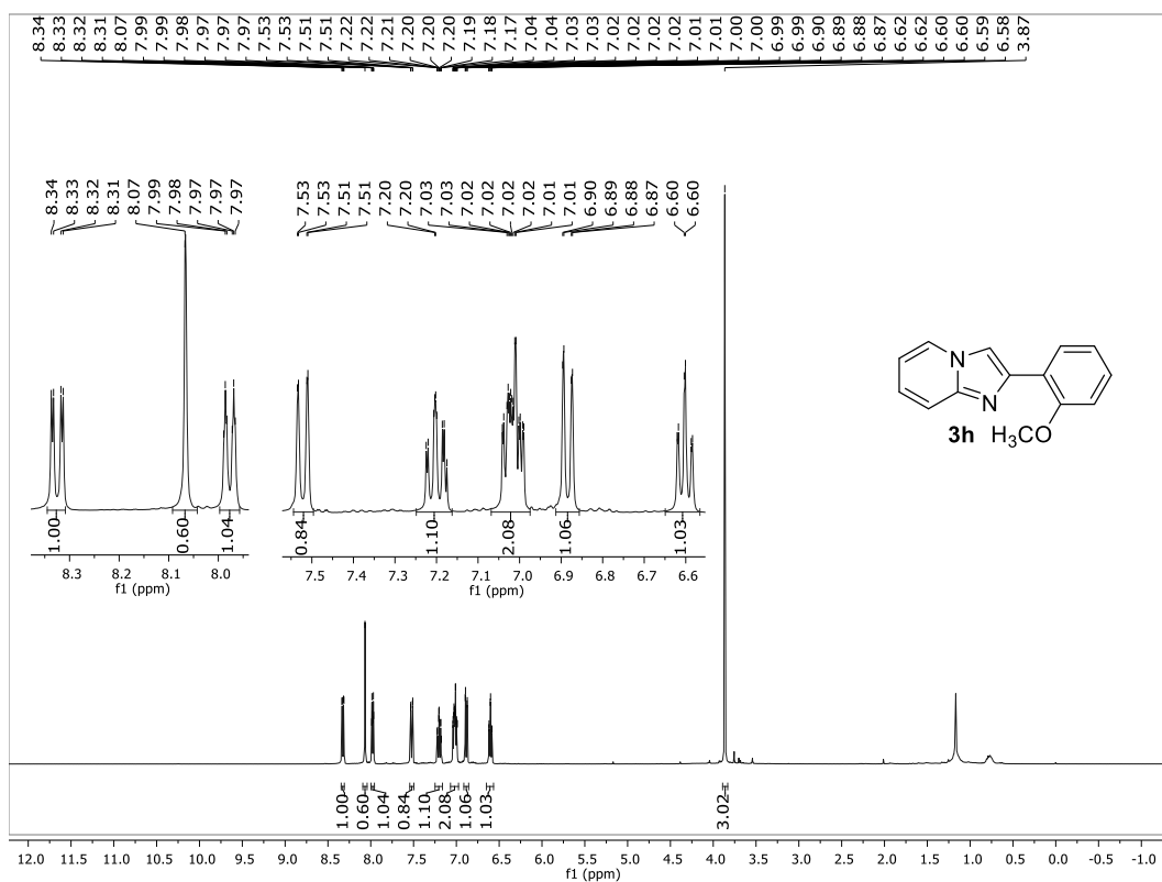
1 H NMR (400 MHz, CDCl 3 ) spectrum of 2-(2-methoxyphenyl)imidazo[1,2-a]pyridine ( 3h ).
