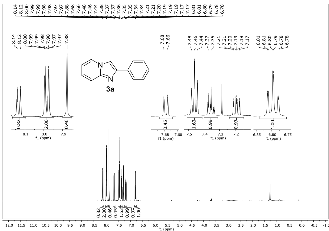
1 H NMR (400 MHz, CDCl 3 ) spectrum of 2-phenylimidazo[1,2-a]pyridine (3a).
