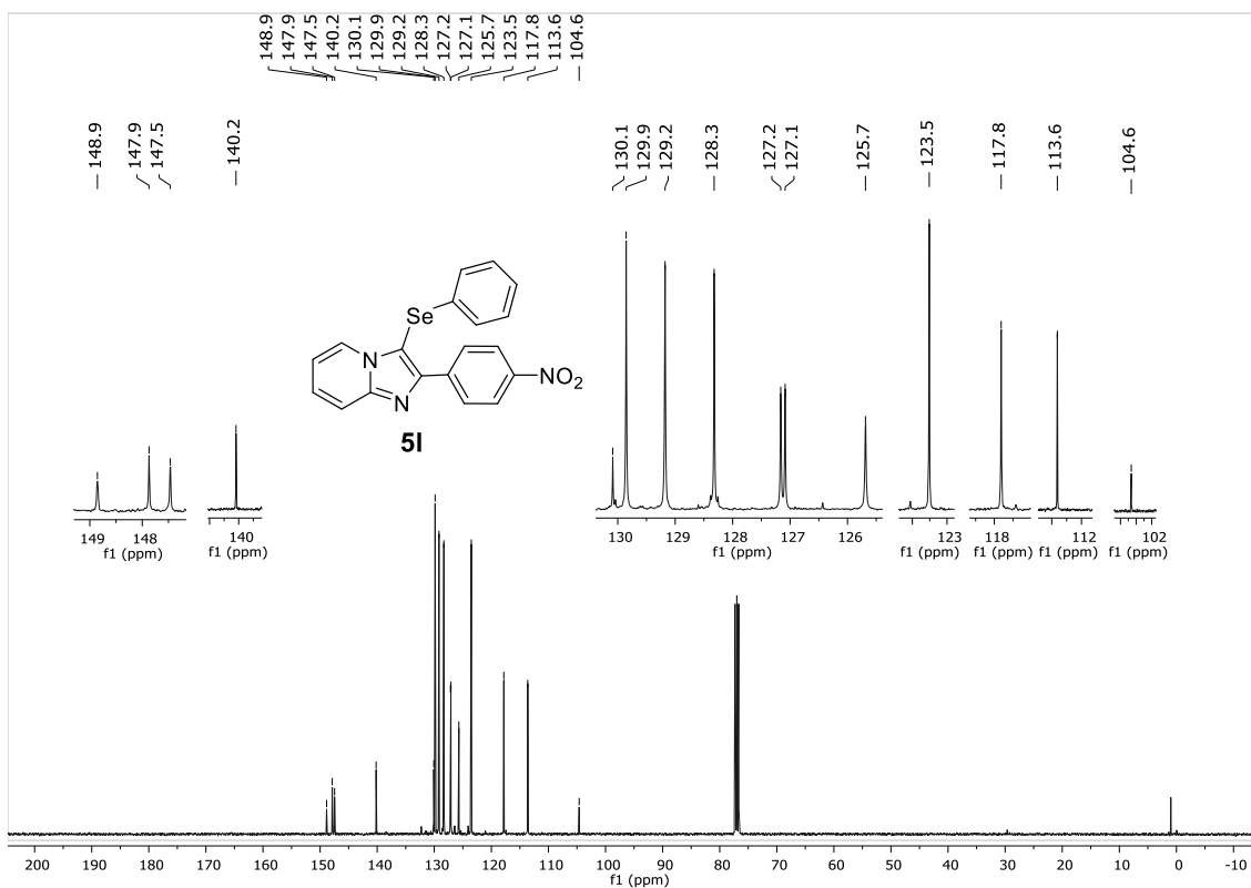
13 C NMR (100 MHz, CDCl 3 ) spectrum of 2-(4-nitrophenyl)-3-(phenylselanyl)imidazo[1,2- a ]pyridine ( 5I ).
