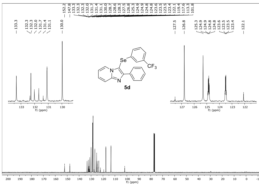
13 C NMR (100 MHz, CDCl 3 ) spectrum of 2-phenyl-3-[[3-(trifluoromethyl)phenyl]selanyl]imidazo[1,2-a]pyridine (5d).
