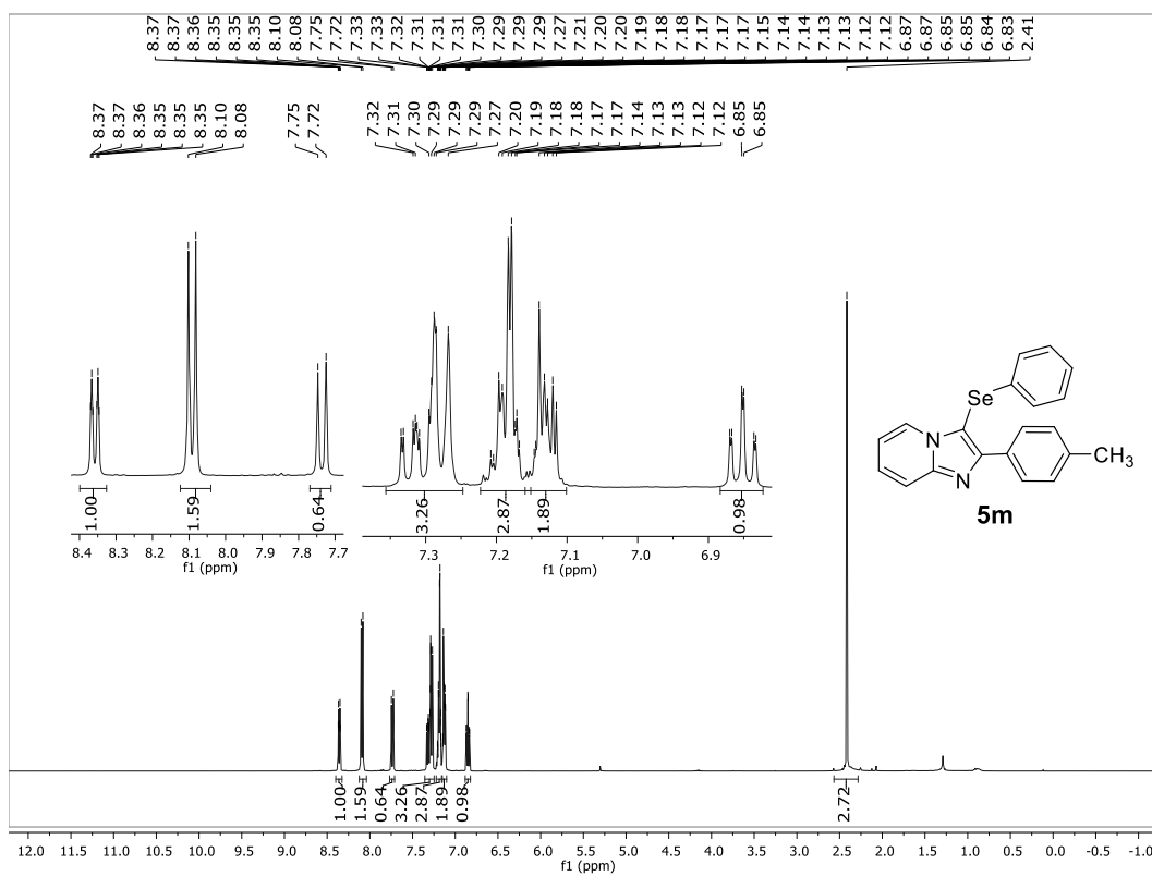
1 H NMR (400 MHz, CDCl 3 ) spectrum of 3-(phenylselanyl)-2-( p -tolyl)imidazo[1,2- a ]pyridine ( 5m ).
