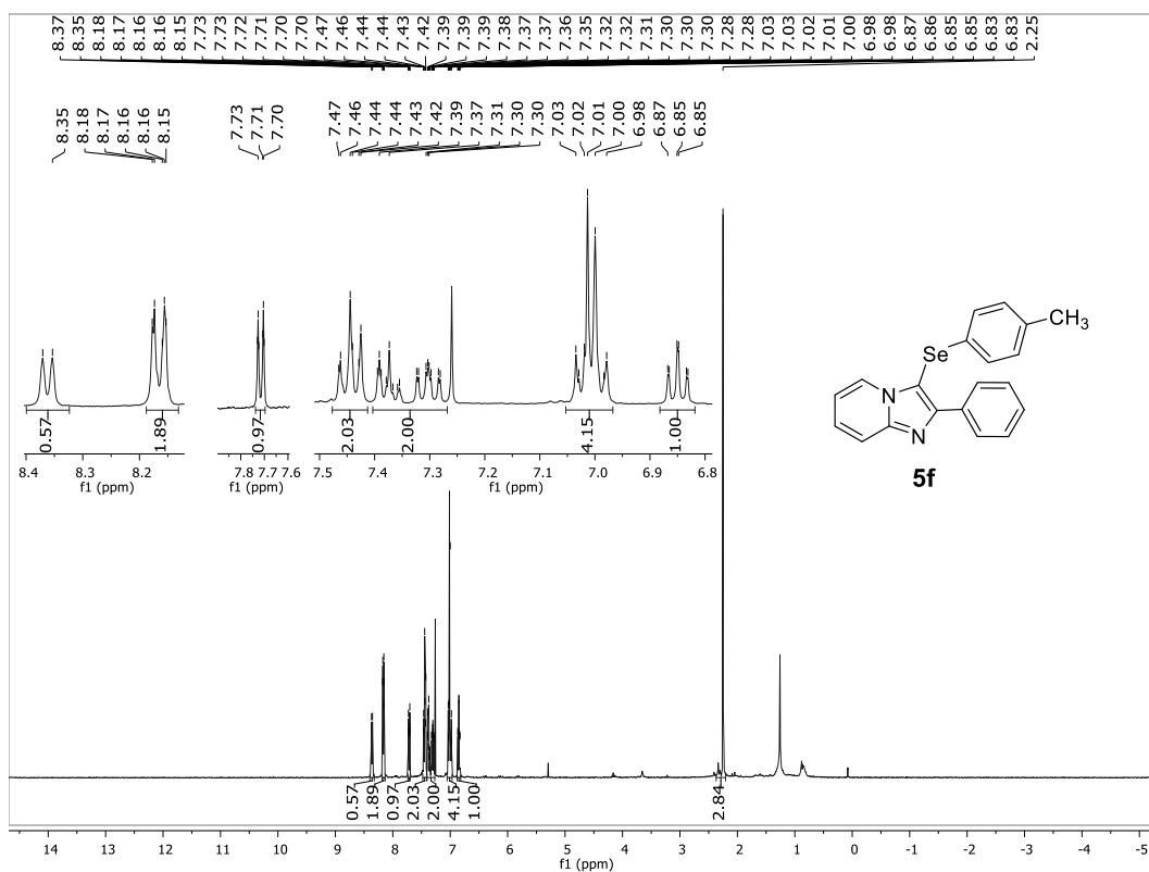
1 H NMR (400 MHz, CDCl 3 ) spectrum of 2-phenyl-3-( p -tolylselanyl)imidazo[1,2- a ]pyridine (5f).
