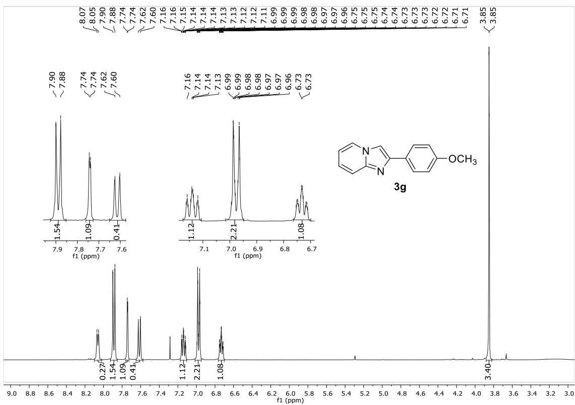
1 H NMR (400 MHz, CDCl 3 ) spectrum of 2-(4-methoxyphenyl)imidazo[1,2-a]pyridine ( 3g ).
