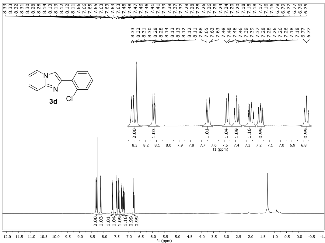
1 H NMR (400 MHz, CDCl 3 ) spectrum of 2-(2-chlorophenyl)imidazo[1,2-a]pyridine (3d).
