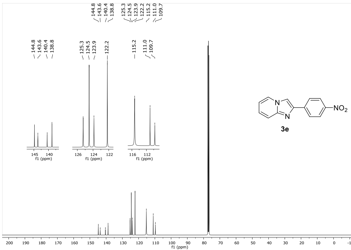
13 C NMR (100 MHz, CDCl 3 /DMSO- d 6 ) spectrum of 2-(4-nitrophenyl)imidazo[1,2- a ]pyridine ( 3e ).
