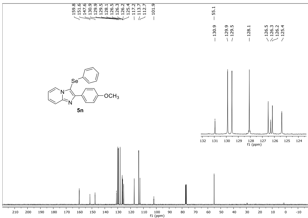
13 C NMR (100 MHz, CDCl 3 ) spectrum of 2-(4-methoxyphenyl)-3-(phenylselanyl)imidazo[1,2-a]pyridine ( 5n ).
