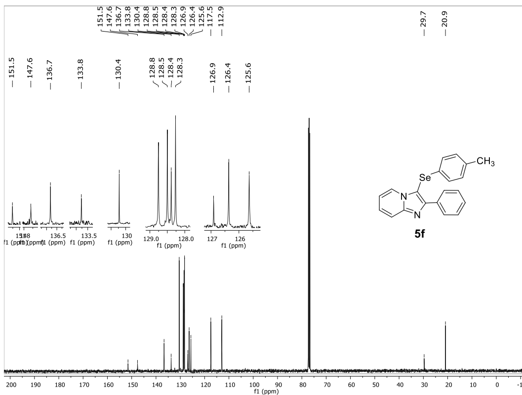
13 C NMR (100 MHz, CDCl 3 ) spectrum of 2-phenyl-3-( p -tolylselanyl)imidazo[1,2- a ]pyridine (5f).
