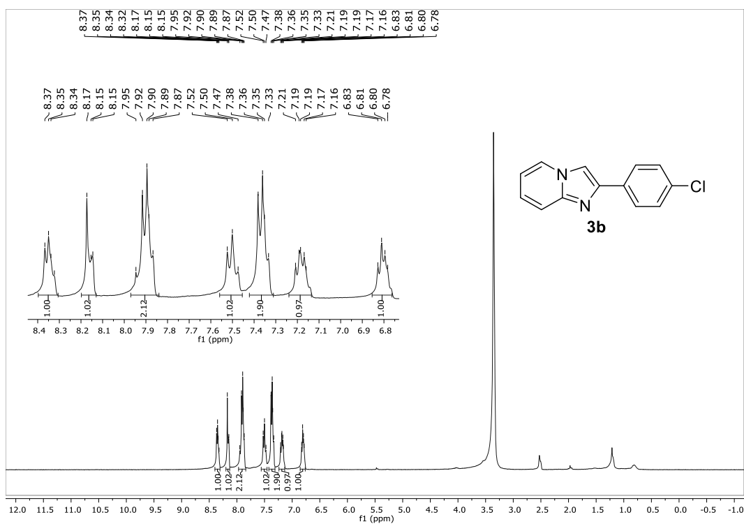
1 H NMR (400 MHz, CDCl 3 /DMSO- d 6 ) spectrum of 2-(4-chlorophenyl)imidazo[1,2- a ]pyridine ( 3b ).
