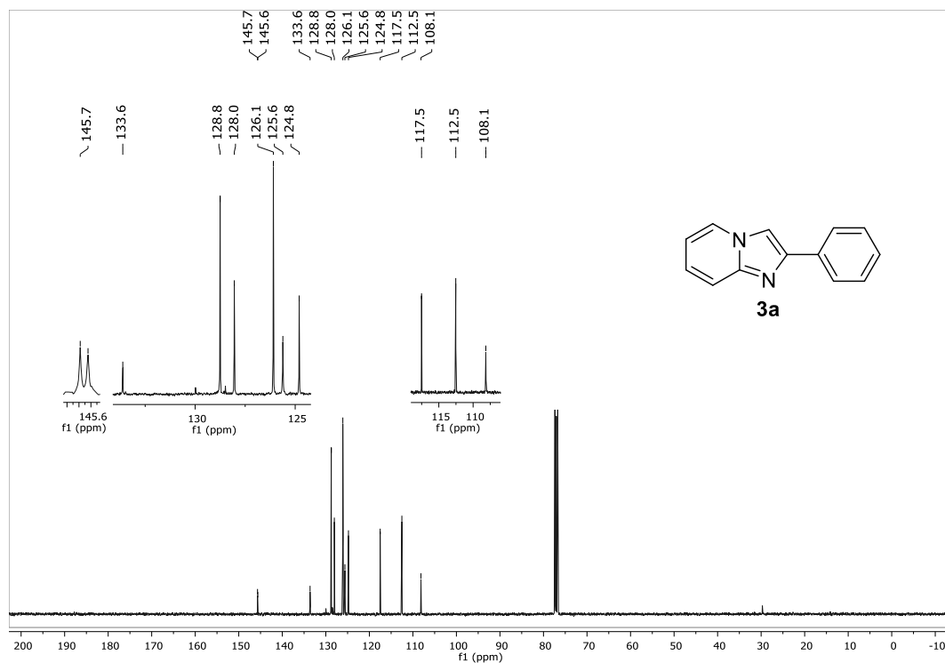
13 C NMR (100 MHz, CDCl 3 ) spectrum of 2-phenylimidazo[1,2-a]pyridine (3a).
