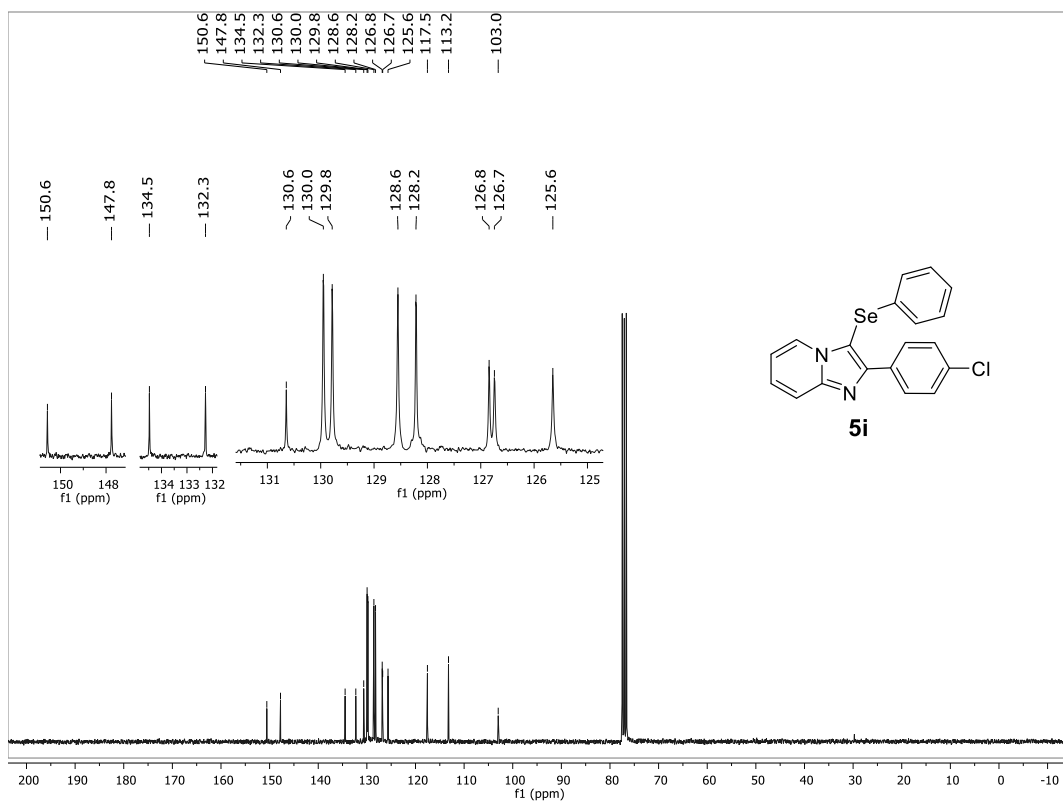
13 C NMR (100 MHz, CDCl 3 ) spectrum of 2-(4-chlorophenyl)-3-(phenylselanyl)imidazo[1,2-a]pyridine ( 5i ).
