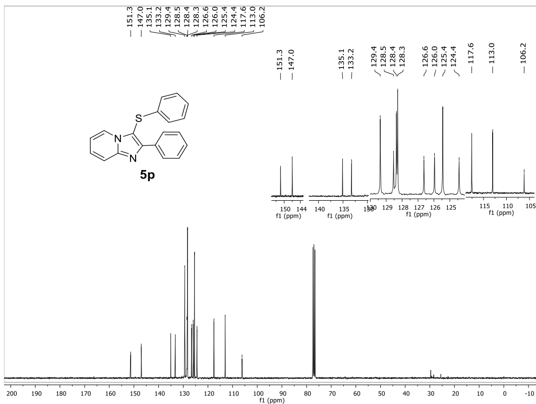
13 C NMR (100 MHz, CDCl 3 ) spectrum of 2-phenyl-3-(phenylthio)imidazo[1,2- a ]pyridine ( 5p ).
