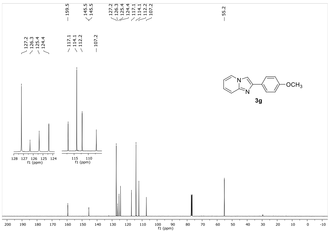
13 C NMR (100 MHz, CDCl 3 ) spectrum of 2-(4-methoxyphenyl)imidazo[1,2-a]pyridine ( 3g ).
