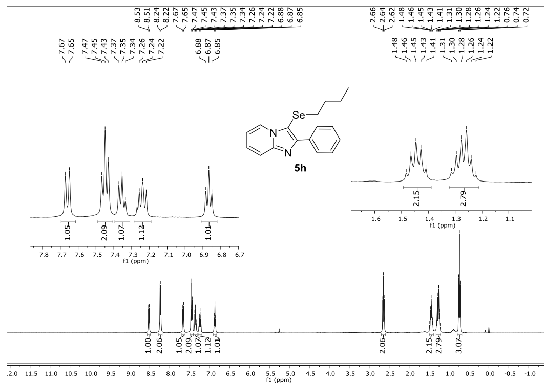
1 H NMR (400 MHz, CDCl 3 ) spectrum of 3-(butylselanyl)-2-phenylimidazo[1,2-a]pyridine ( 5h ).
