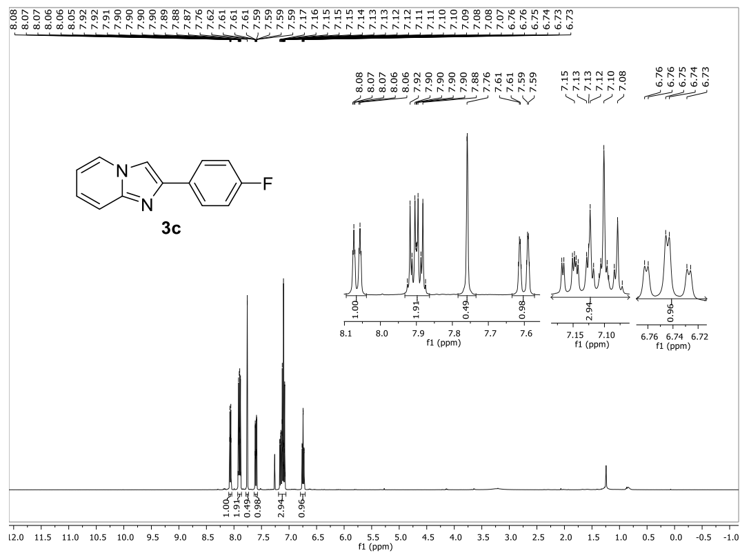
^1\text{H} NMR (400 MHz, \text{CDCl}_3 ) spectrum of 2-(4-fluorophenyl)imidazo[1,2-a]pyridine ( 3c ).
