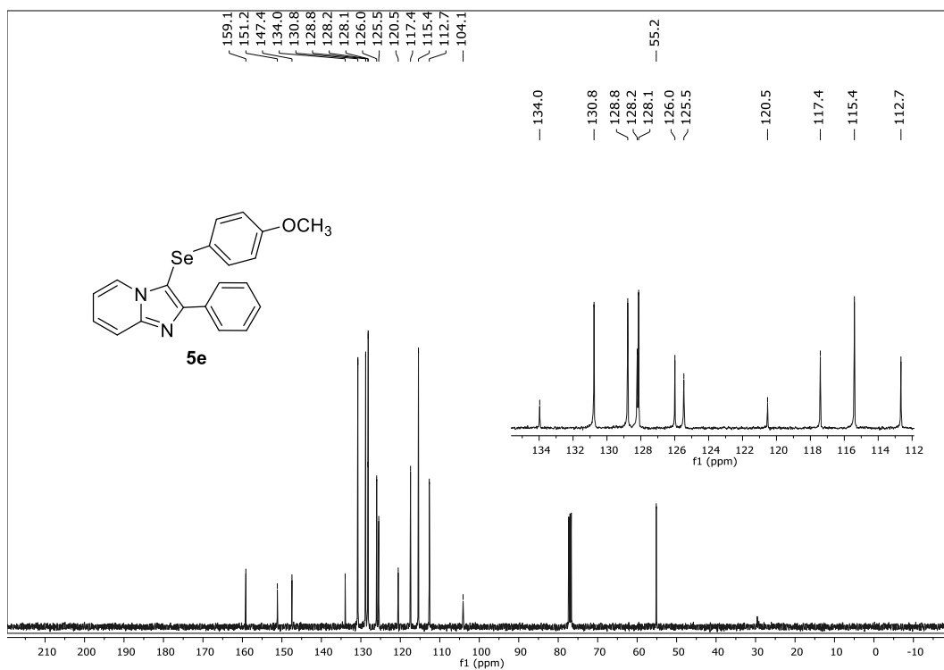
13 C NMR (100 MHz, CDCl 3 ) spectrum of 3-[(4-methoxyphenyl)selanyl]-2-phenylimidazo[1,2-a]pyridine ( 5e ).
