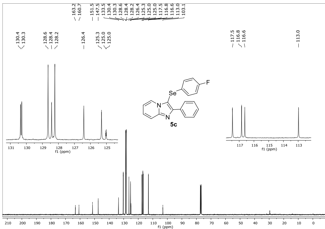
13 C NMR (100 MHz, CDCl 3 ) spectrum of 3-[(4-fluorophenyl)selenanyl]-2-phenylimidazo[1,2-a]pyridine ( 5c ).
