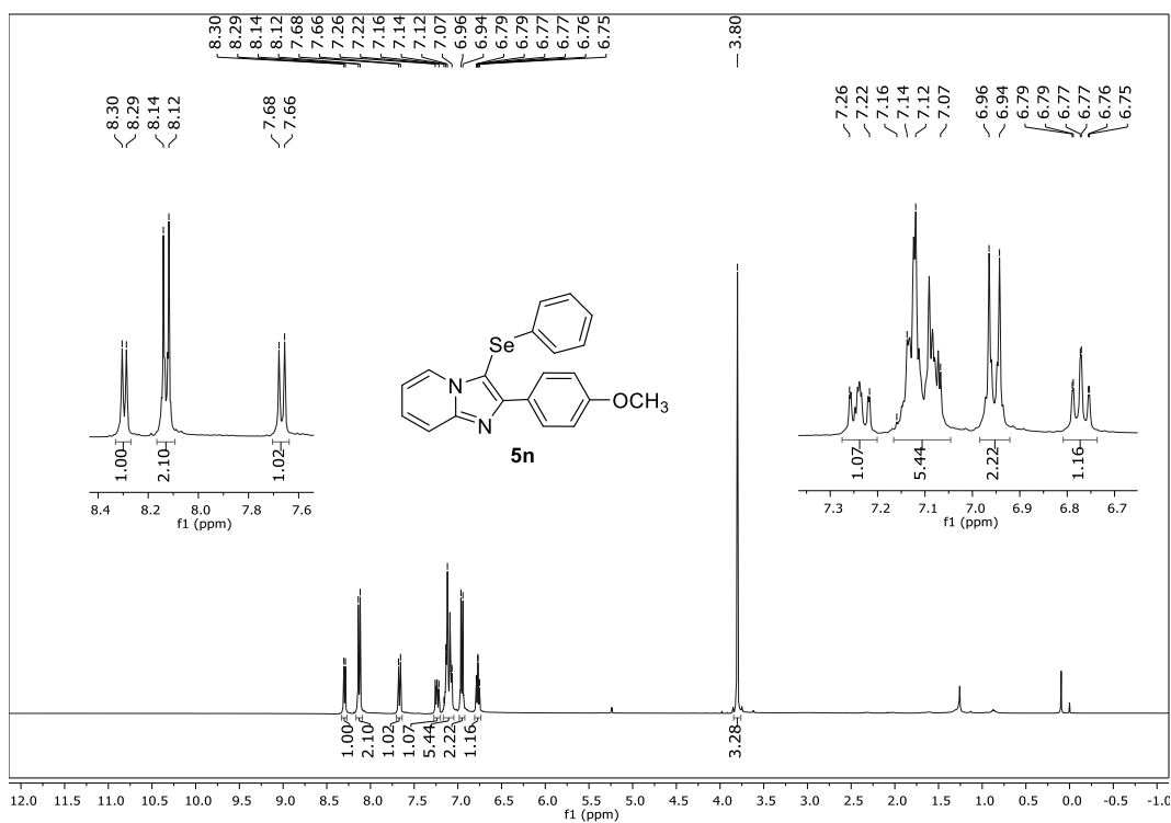
1 H NMR (400 MHz, CDCl 3 ) spectrum of 2-(4-methoxyphenyl)-3-(phenylselanyl)imidazo[1,2-a]pyridine ( 5n ).
