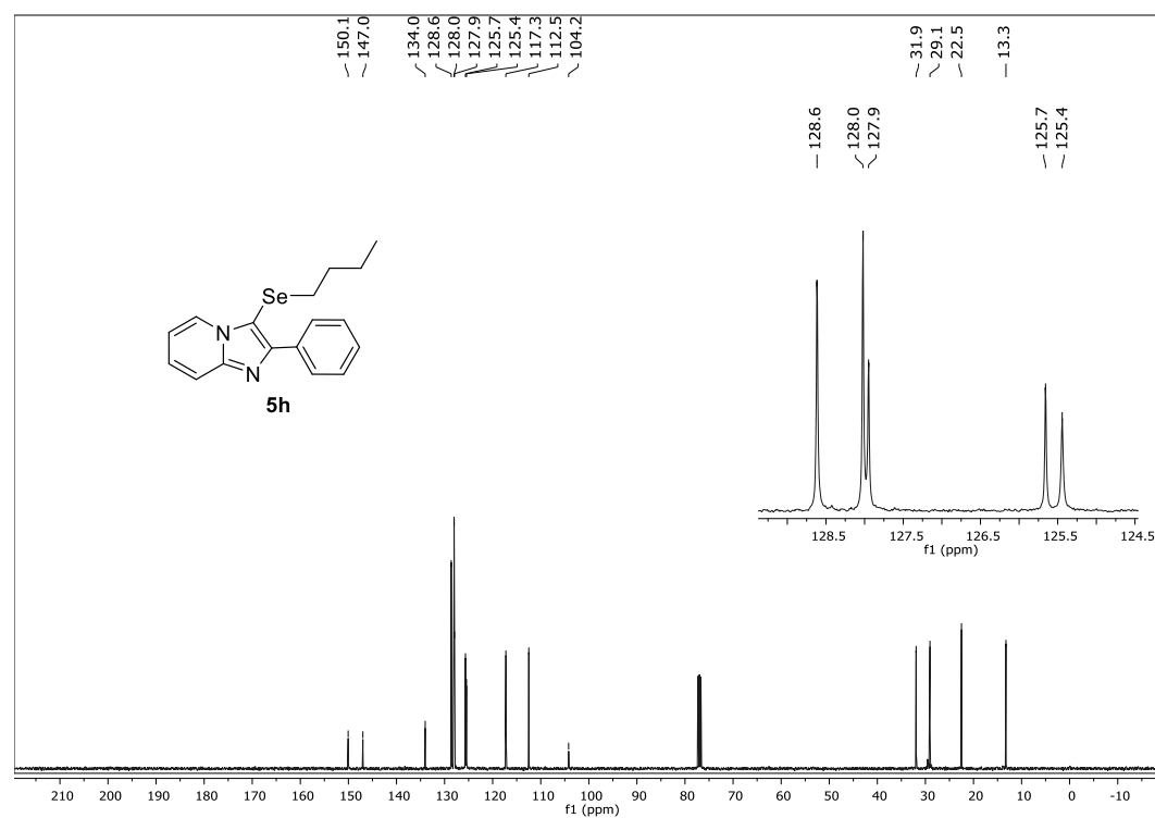
13 C NMR (100 MHz, CDCl 3 ) spectrum of 3-(butylselanyl)-2-phenylimidazo[1,2-a]pyridine ( 5h ).
