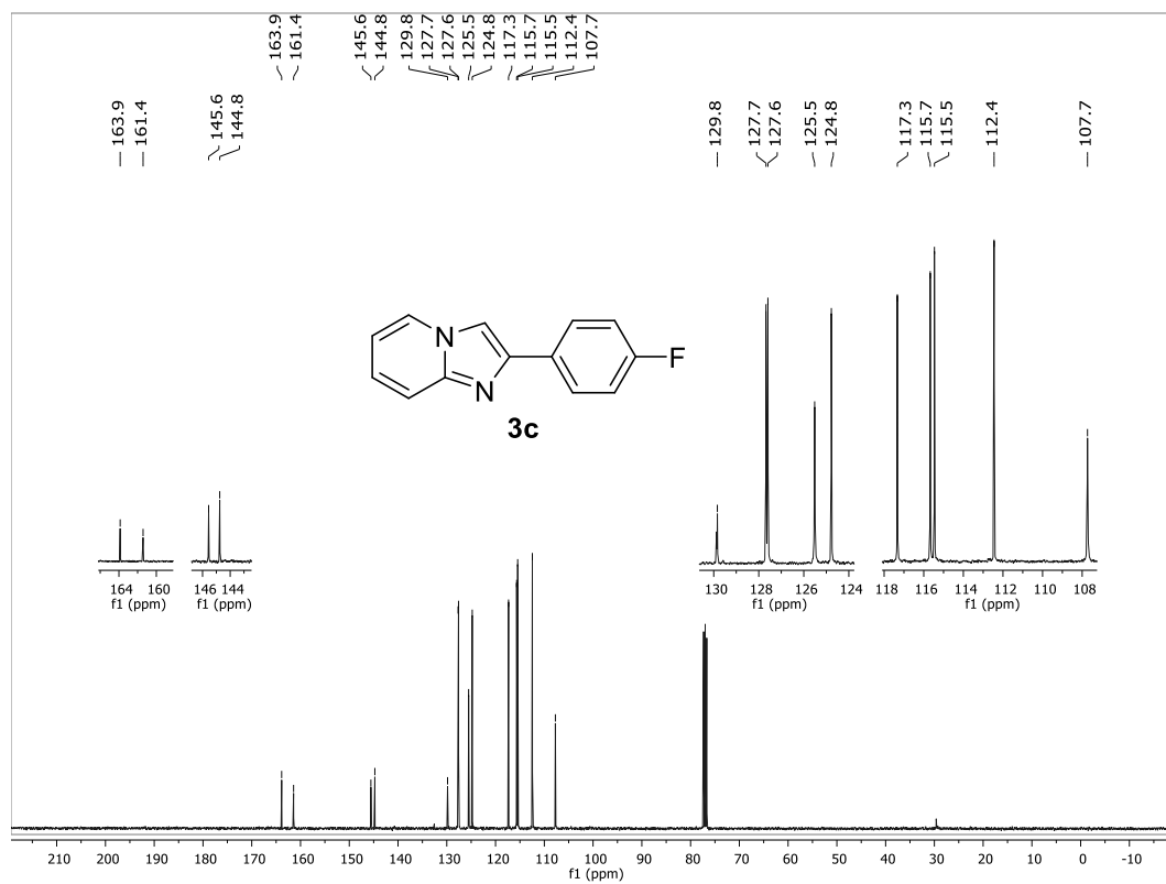
^{13}\text{C} NMR (100 MHz, \text{CDCl}_3 ) spectrum of 2-(4-fluorophenyl)imidazo[1,2-a]pyridine ( 3c ).
