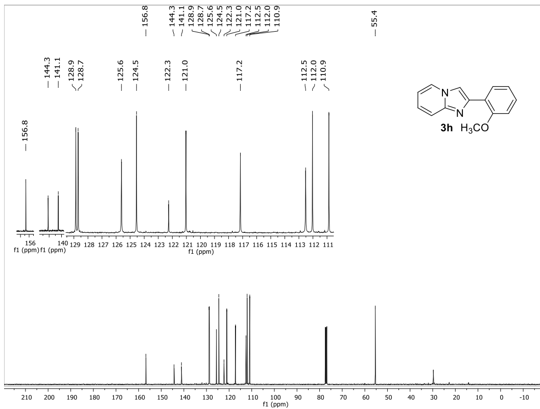
13 C NMR (100 MHz, CDCl 3 ) spectrum of 2-(2-methoxyphenyl)imidazo[1,2-a]pyridine ( 3h ).
