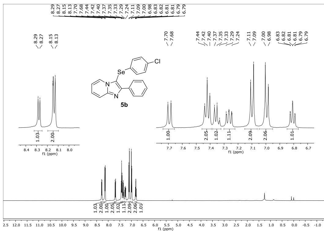
1 H NMR (400 MHz, CDCl 3 ) spectrum of 3-[(4-chlorophenyl)selanyl]-2-phenylimidazo[1,2- a ]pyridine ( 5b ).
