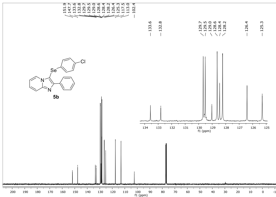
13 C NMR (100 MHz, CDCl 3 ) spectrum of 3-[(4-chlorophenyl)selanyl]-2-phenylimidazo[1,2- a ]pyridine ( 5b ).
