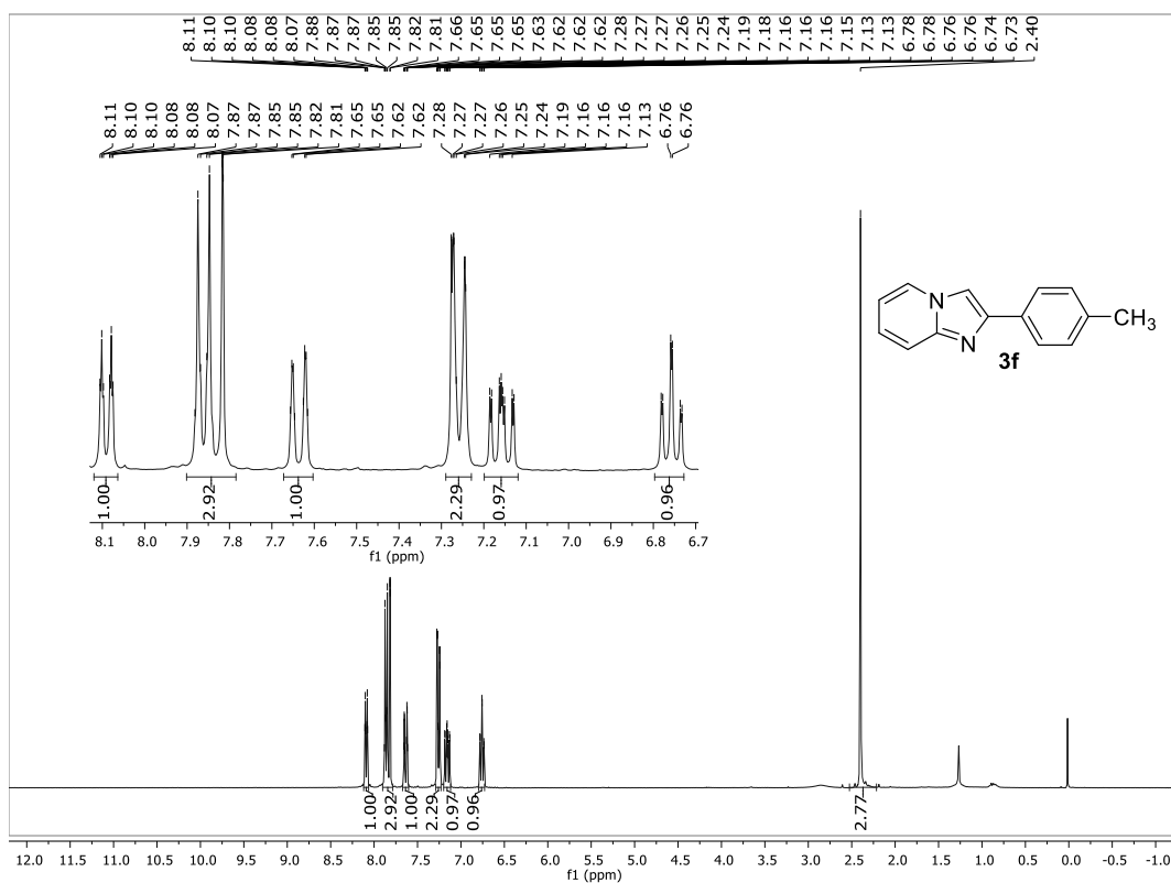
1 H NMR (400 MHz, CDCl 3 ) spectrum of 2-( p -tolyl)imidazo[1,2- a ]pyridine ( 3f ).
