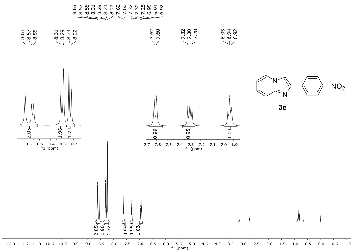
1 H NMR (400 MHz, CDCl 3 /DMSO- d 6 ) spectrum of 2-(4-nitrophenyl)imidazo[1,2- a ]pyridine ( 3e ).
