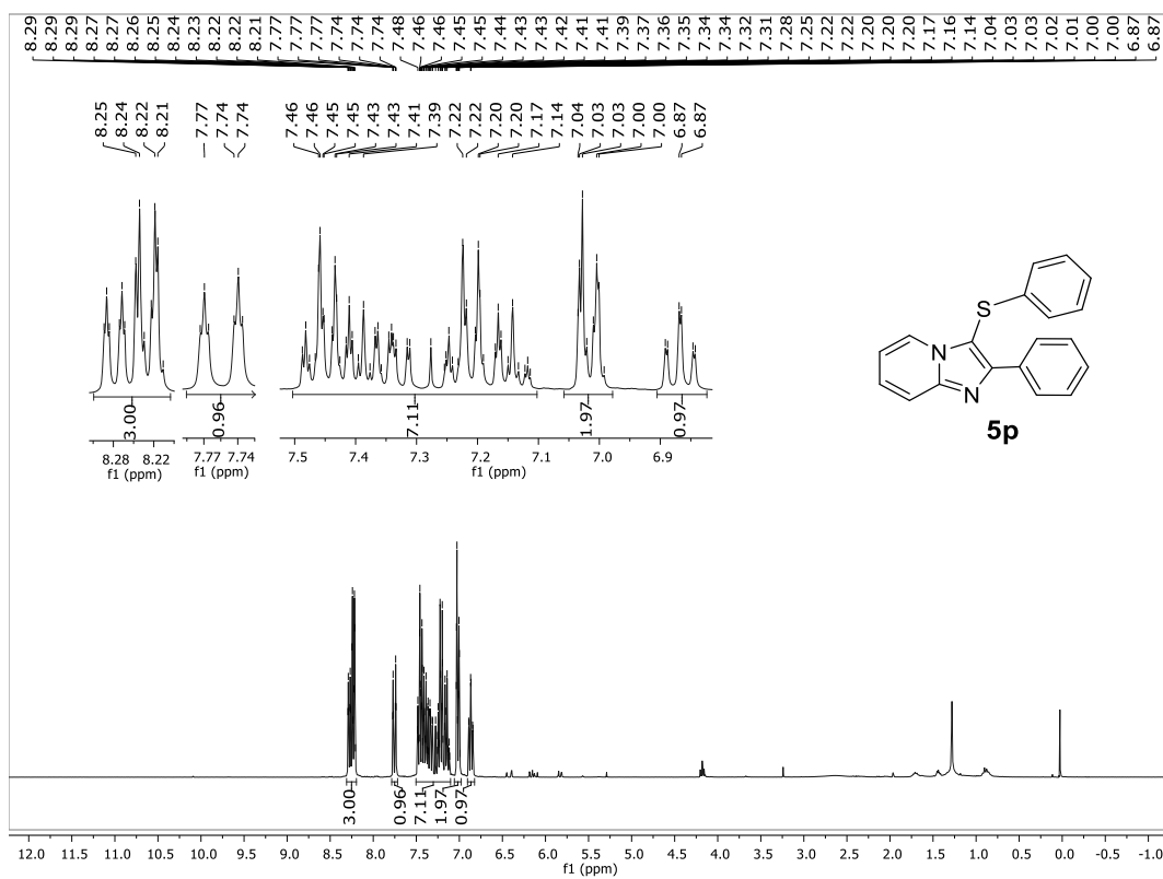
1 H NMR (400 MHz, CDCl 3 ) spectrum of 2-phenyl-3-(phenylthio)imidazo[1,2- a ]pyridine ( 5p ).
