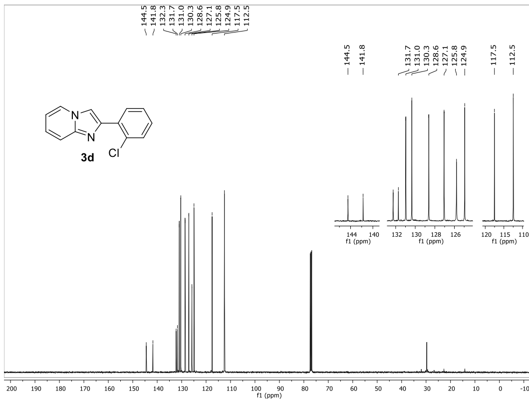
13 C NMR (100 MHz, CDCl 3 ) spectrum of 2-(2-chlorophenyl)imidazo[1,2-a]pyridine (3d).
