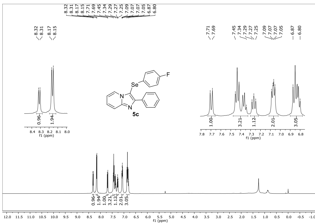
1 H NMR (400 MHz, CDCl 3 ) spectrum of 3-[(4-fluorophenyl)selenanyl]-2-phenylimidazo[1,2-a]pyridine ( 5c ).
