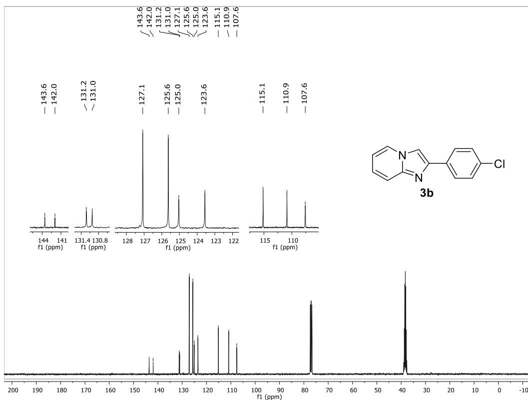
13 C NMR (100 MHz, CDCl 3 /DMSO- d 6 ) spectrum of 2-(4-chlorophenyl)imidazo[1,2- a ]pyridine ( 3b ).
