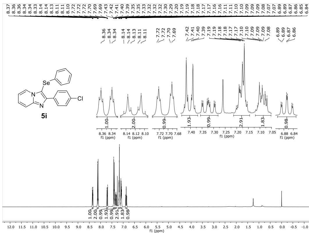
1 H NMR (400 MHz, CDCl 3 ) spectrum of 2-(4-chlorophenyl)-3-(phenylselanyl)imidazo[1,2-a]pyridine ( 5i ).
