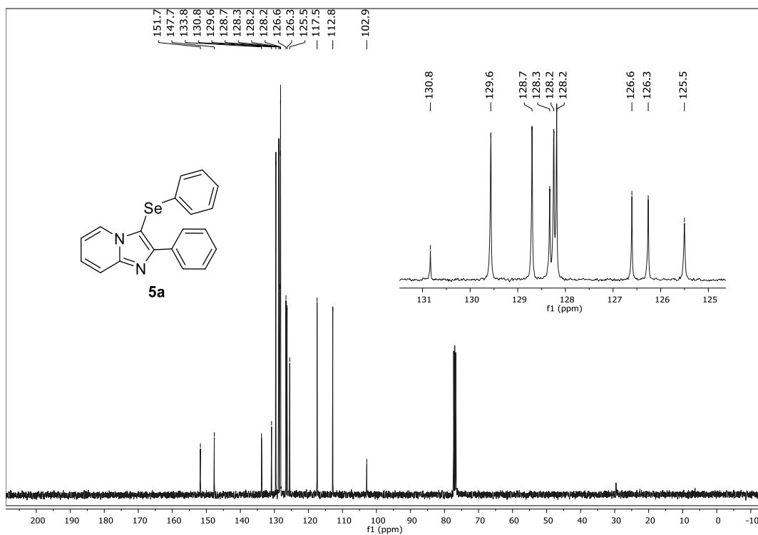
13 C NMR (100 MHz, CDCl 3 ) spectrum of 2-phenyl-3-(phenylselanyl)imidazo[1,2- a ]pyridine (5a).
