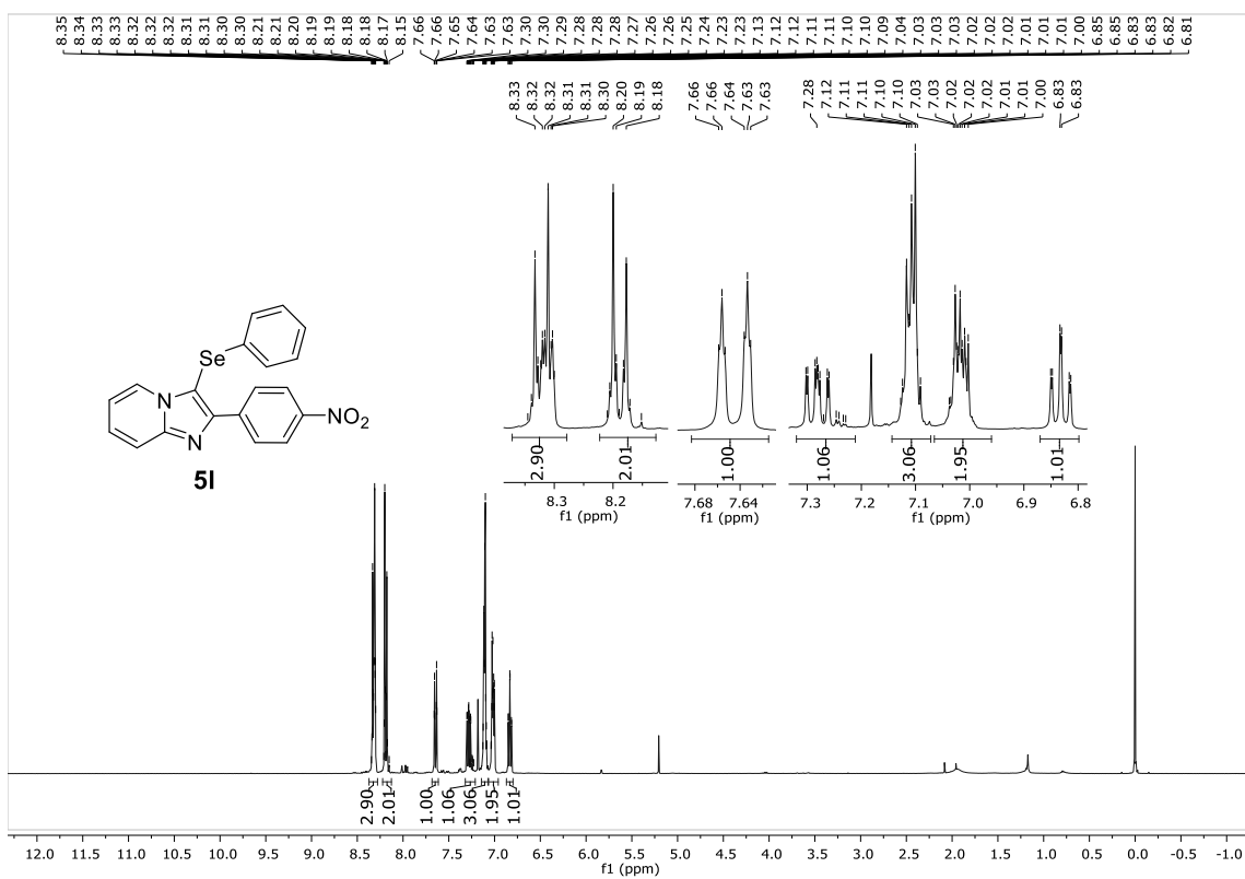
1 H NMR (400 MHz, CDCl 3 ) spectrum of 2-(4-nitrophenyl)-3-(phenylselanyl)imidazo[1,2- a ]pyridine ( 5I ).
