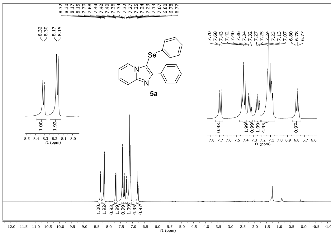
1 H NMR (400 MHz, CDCl 3 ) spectrum of 2-phenyl-3-(phenylselanyl)imidazo[1,2- a ]pyridine (5a).
