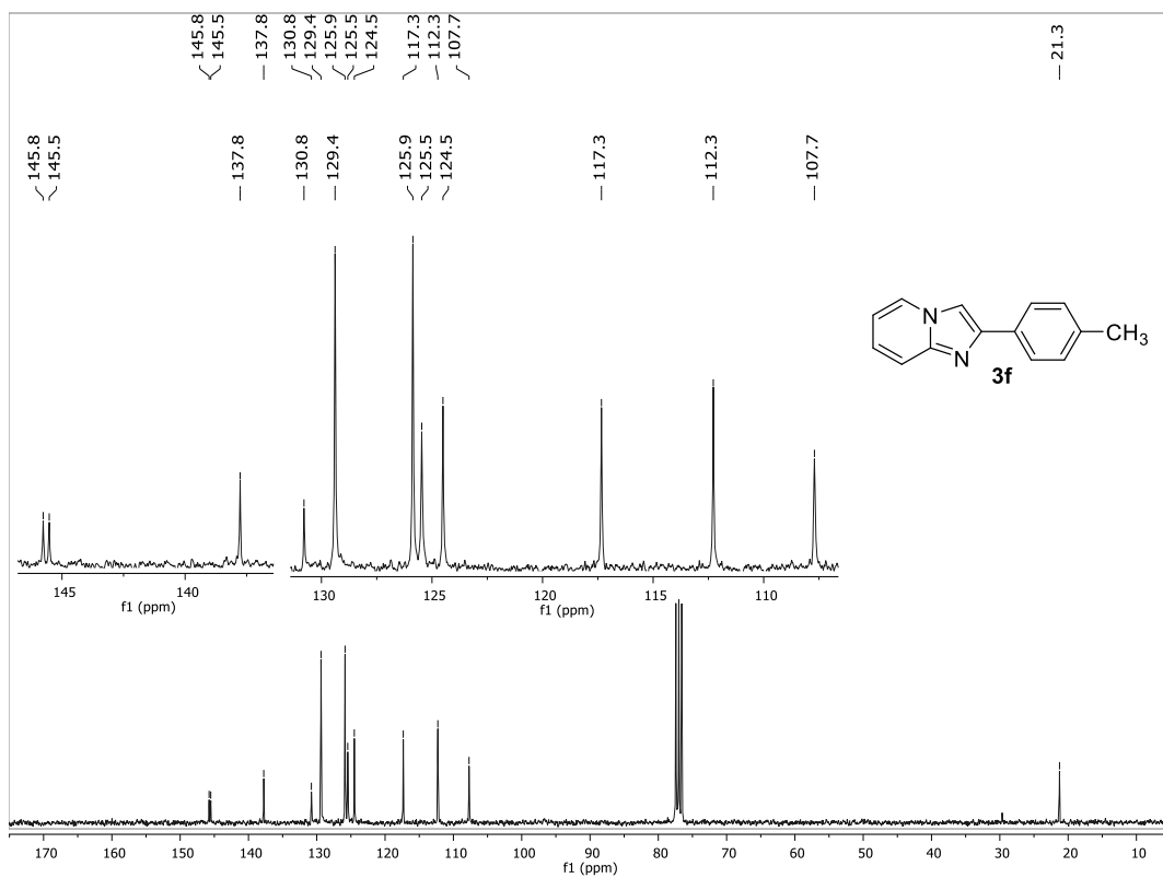
13 C NMR (100 MHz, CDCl 3 ) spectrum of 2-( p -tolyl)imidazo[1,2- a ]pyridine ( 3f ).
