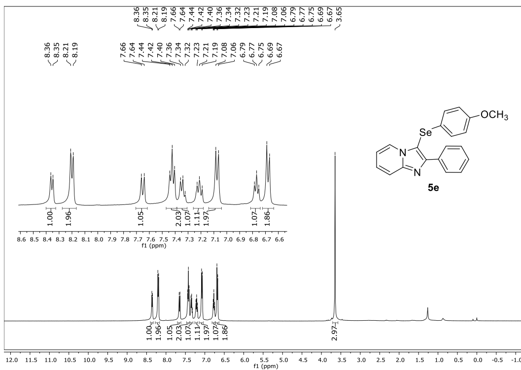
1 H NMR (400 MHz, CDCl 3 ) spectrum of 3-[(4-methoxyphenyl)selanyl]-2-phenylimidazo[1,2-a]pyridine ( 5e ).
