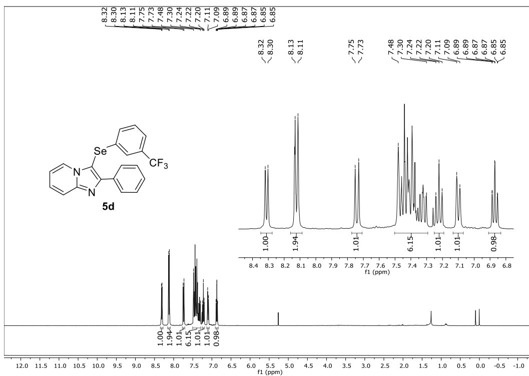
1 H NMR (400 MHz, CDCl 3 ) spectrum of 2-phenyl-3-[[3-(trifluoromethyl)phenyl]selanyl]imidazo[1,2-a]pyridine (5d).
