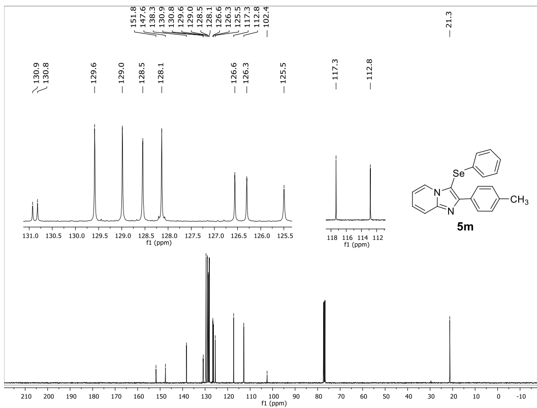
13 C NMR (100 MHz, CDCl 3 ) spectrum of 3-(phenylselanyl)-2-( p -tolyl)imidazo[1,2- a ]pyridine ( 5m ).
