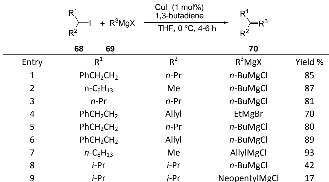
Scheme 21. Cross-coupling reaction of unactivated secondary alkyl iodides with alkyl Grignard reagents.
