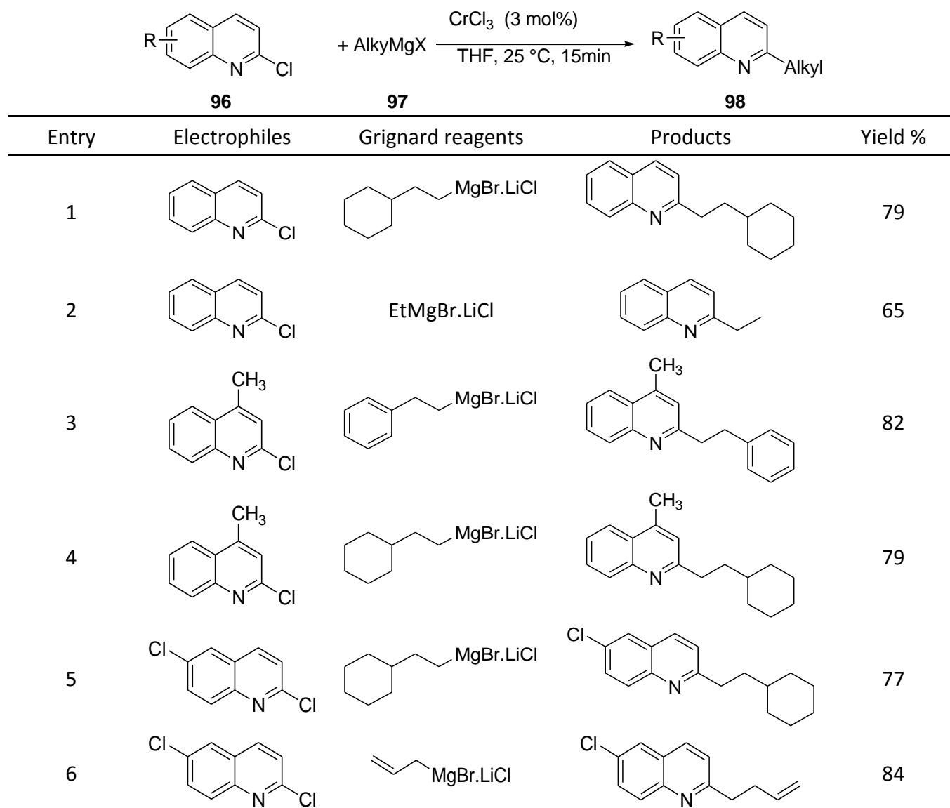
Scheme 31. Chromium-catalyzed cross coupling reaction of Grignard reagents with chloroquinolines.
