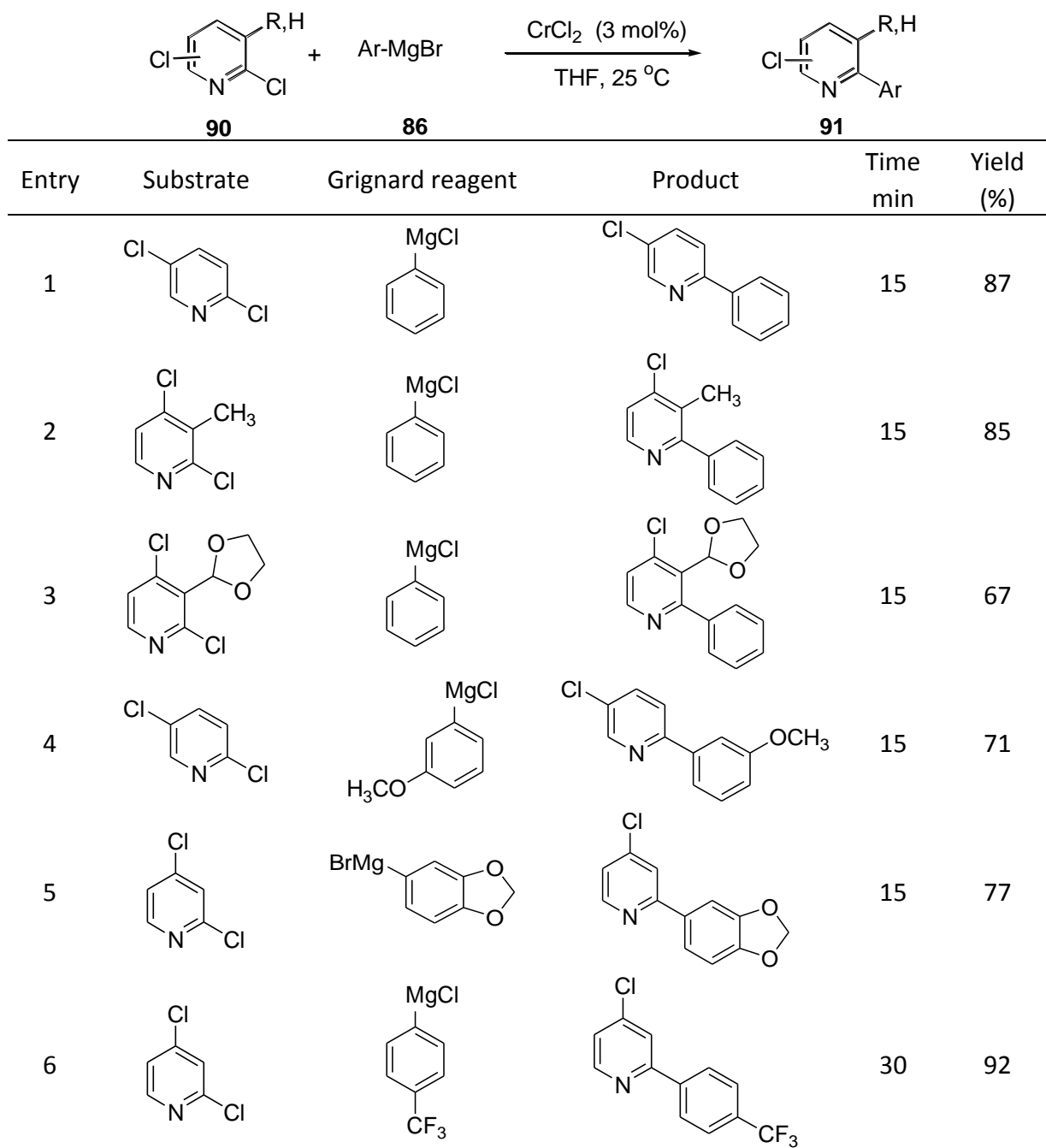
Scheme 29. Chemoselective reactions between dichlorinated pyridines and aromatic Grignard reagents.
