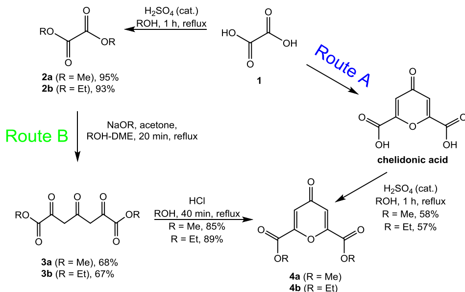
Scheme 1. Synthesis of dialkyl 4-oxo-4H-pyran-2,6-carboxylates 4 via the traditional method (Route A); 24 and via the modified procedure (Route B). 25
