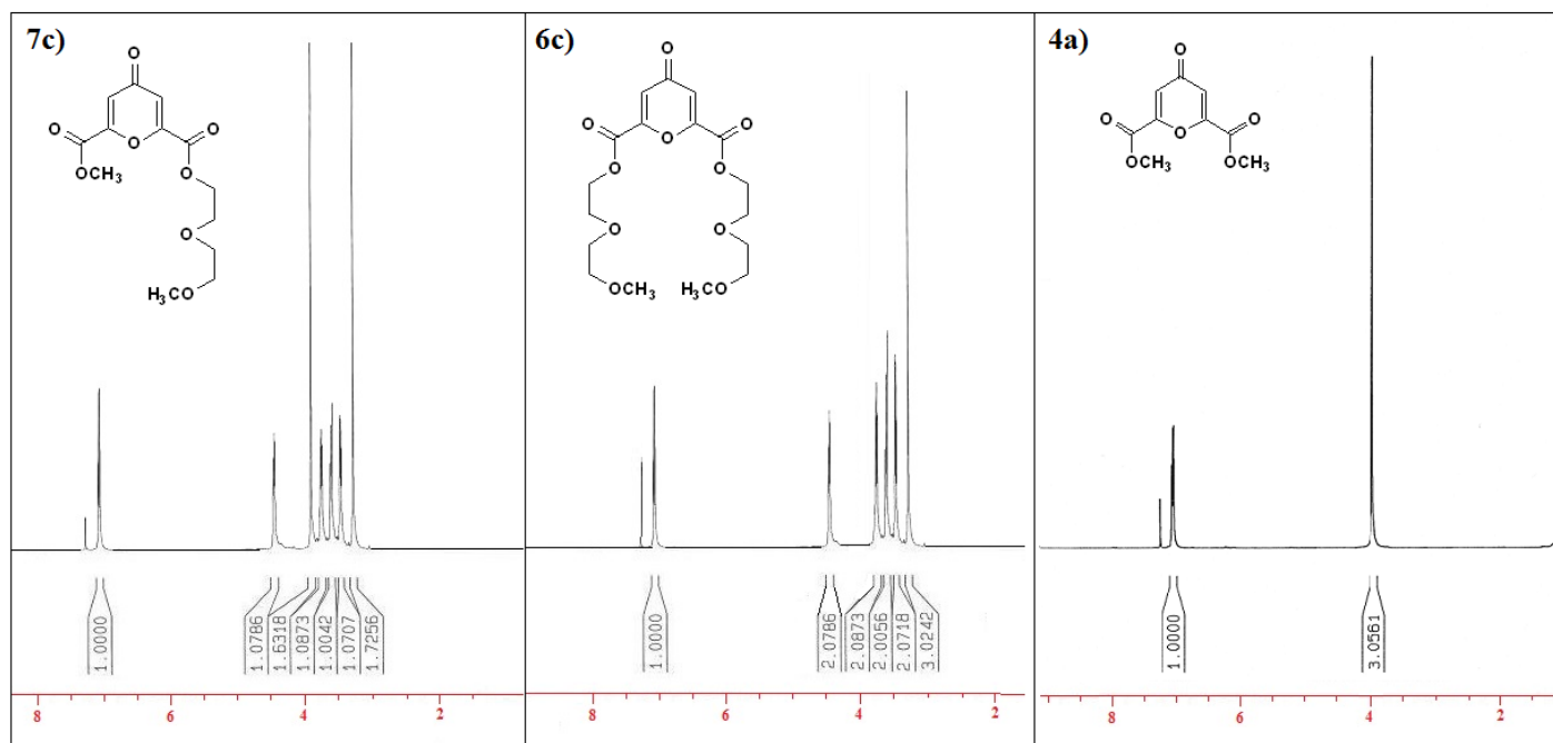
Figure 2. 1 H NMR spectra of the 6c and 7c as representative of synthesized podands.
