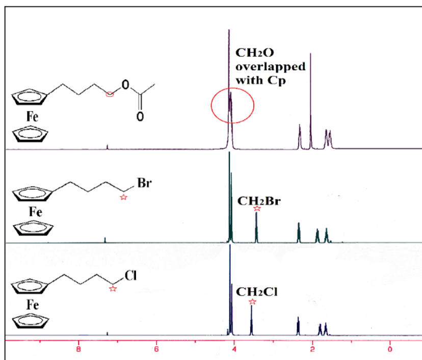
Figure 3. 1 H NMR spectra of 4-halobutylferrocenes 8a and 8b and 4-ferrocenylbutyl acetate 9 .
