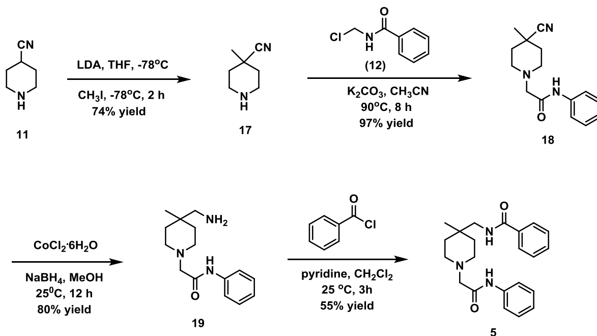
Scheme 2. Synthesis of compound 5
