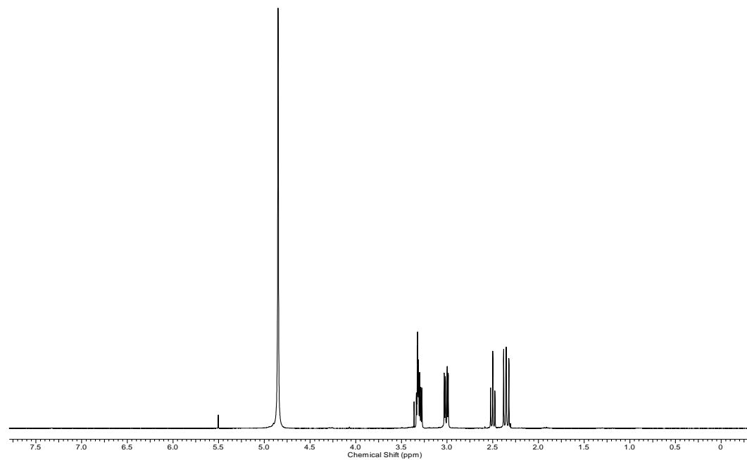
^1\text{H} NMR spectrum (400 MHz, \text{CD}_3\text{OD} ) of 4-aminopiperidine-3,5-diol ( 11 ).
