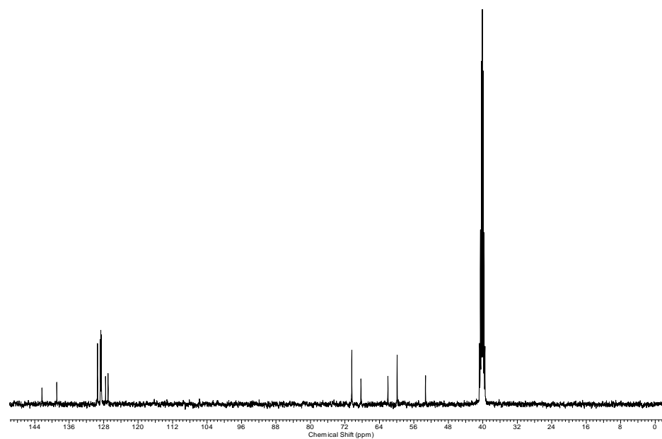
^{13}\text{C} NMR spectrum (100 MHz, \text{CD}_3\text{OD} , \text{DMSO}-d_6 ) of 1-benzyl-4-benzylaminopiperidine-3,5-diol ( 10a ).
