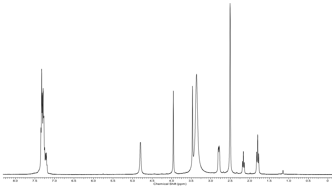
^1\text{H} NMR spectrum (400 MHz, \text{CD}_3\text{OD} , \text{DMSO } d_6 ) of 1-benzyl-4-benzylaminopiperidine-3,5-diol ( 10a ).
