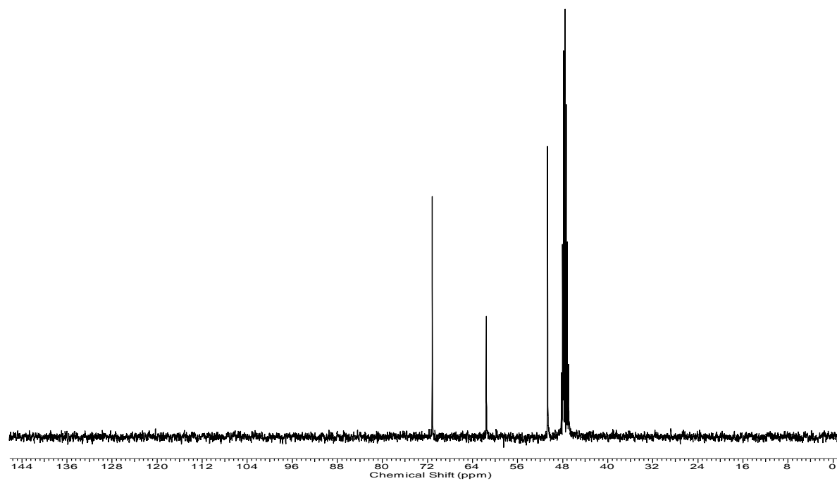
^{13}\text{C} NMR spectrum (100 MHz, \text{CD}_3\text{OD} ) of 4-aminopiperidine-3,5-diol ( 11 ).
