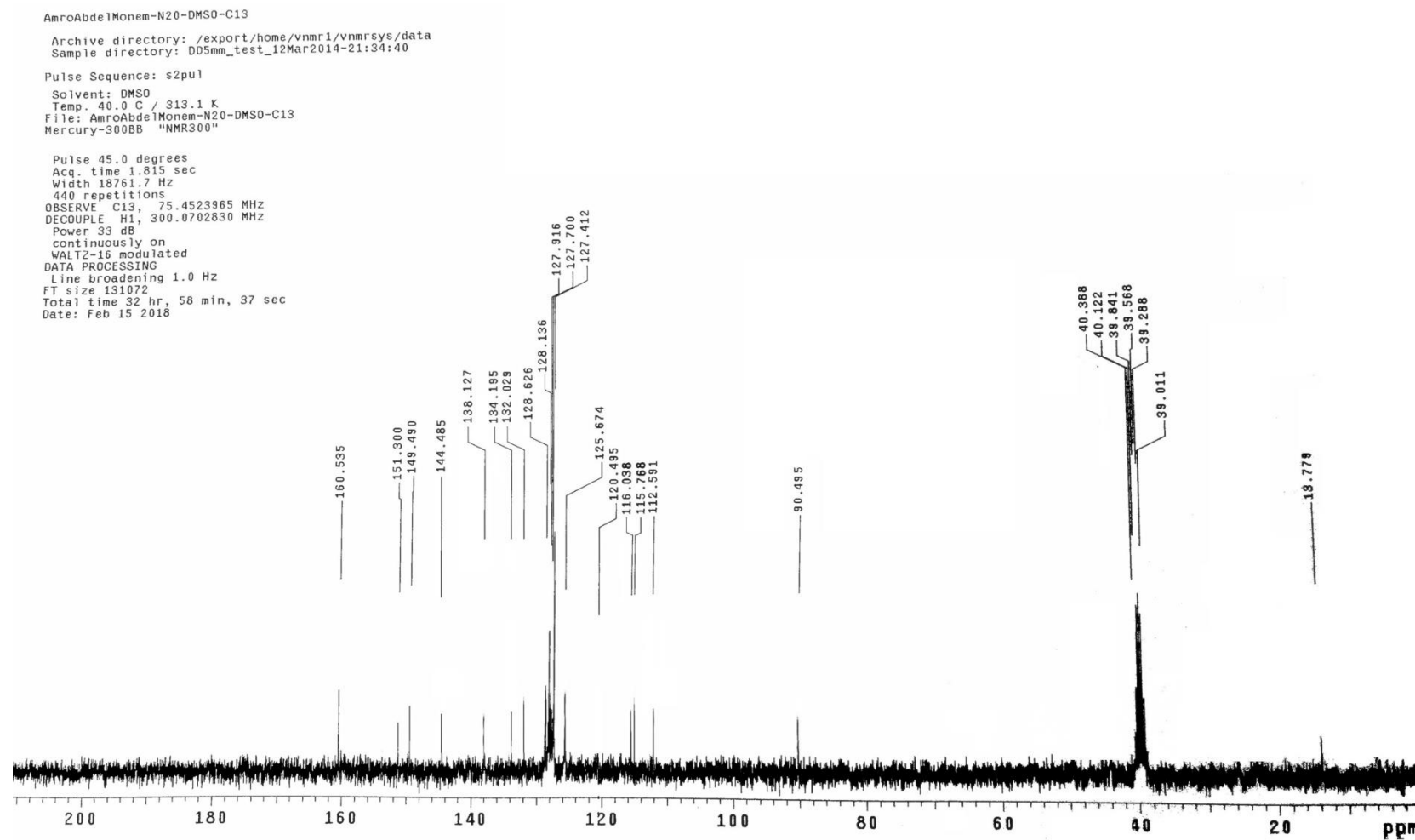
Figure 4. The ^{13}\text{C} NMR spectrum of compound 7a .
