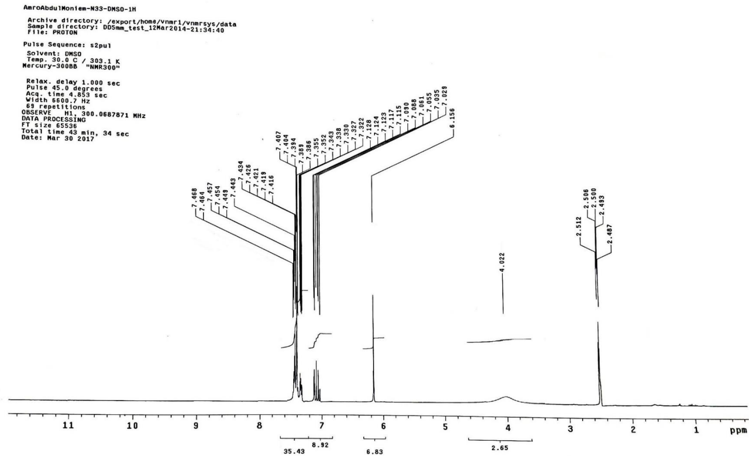
Figure 28. The ^1\text{H} NMR spectrum of compound 21f .
