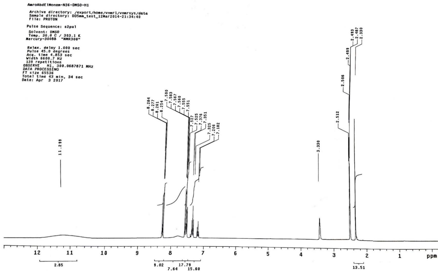
Figure 7. The ^1\text{H} NMR spectrum of compound 7c.
