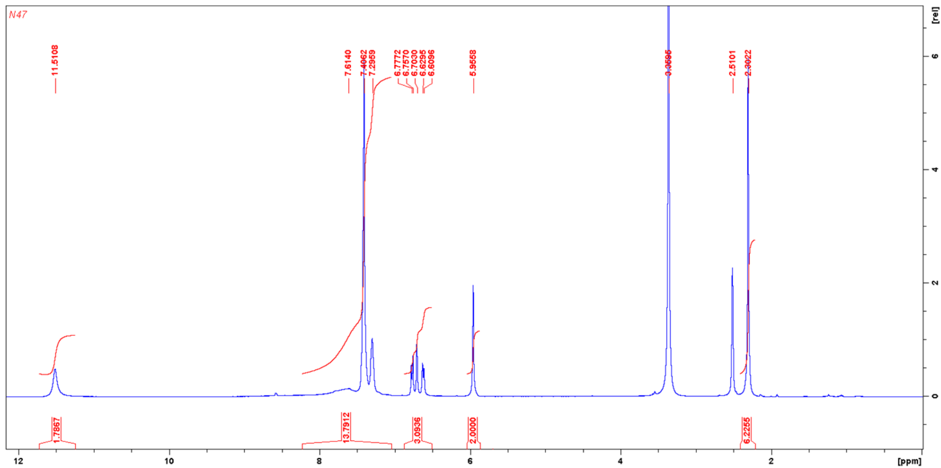
Figure 12. The ^1\text{H} NMR spectrum of compound 7f.
