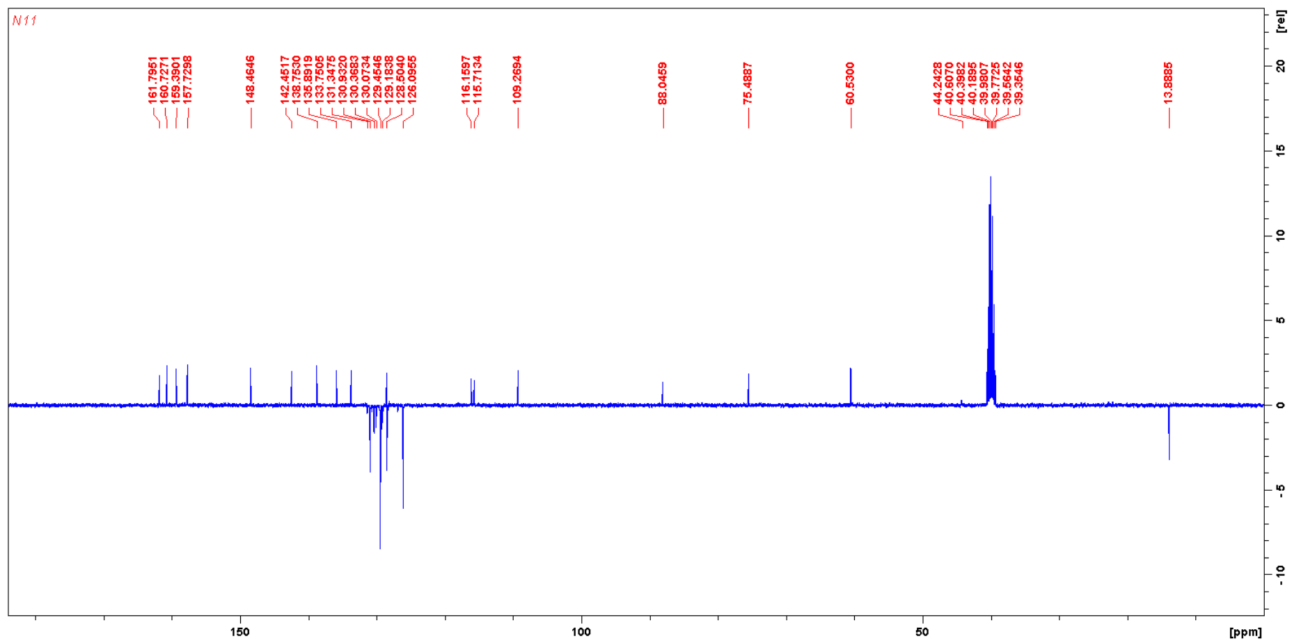
Figure 19. The ^{13}\text{C} NMR spectrum of compound 20b .
