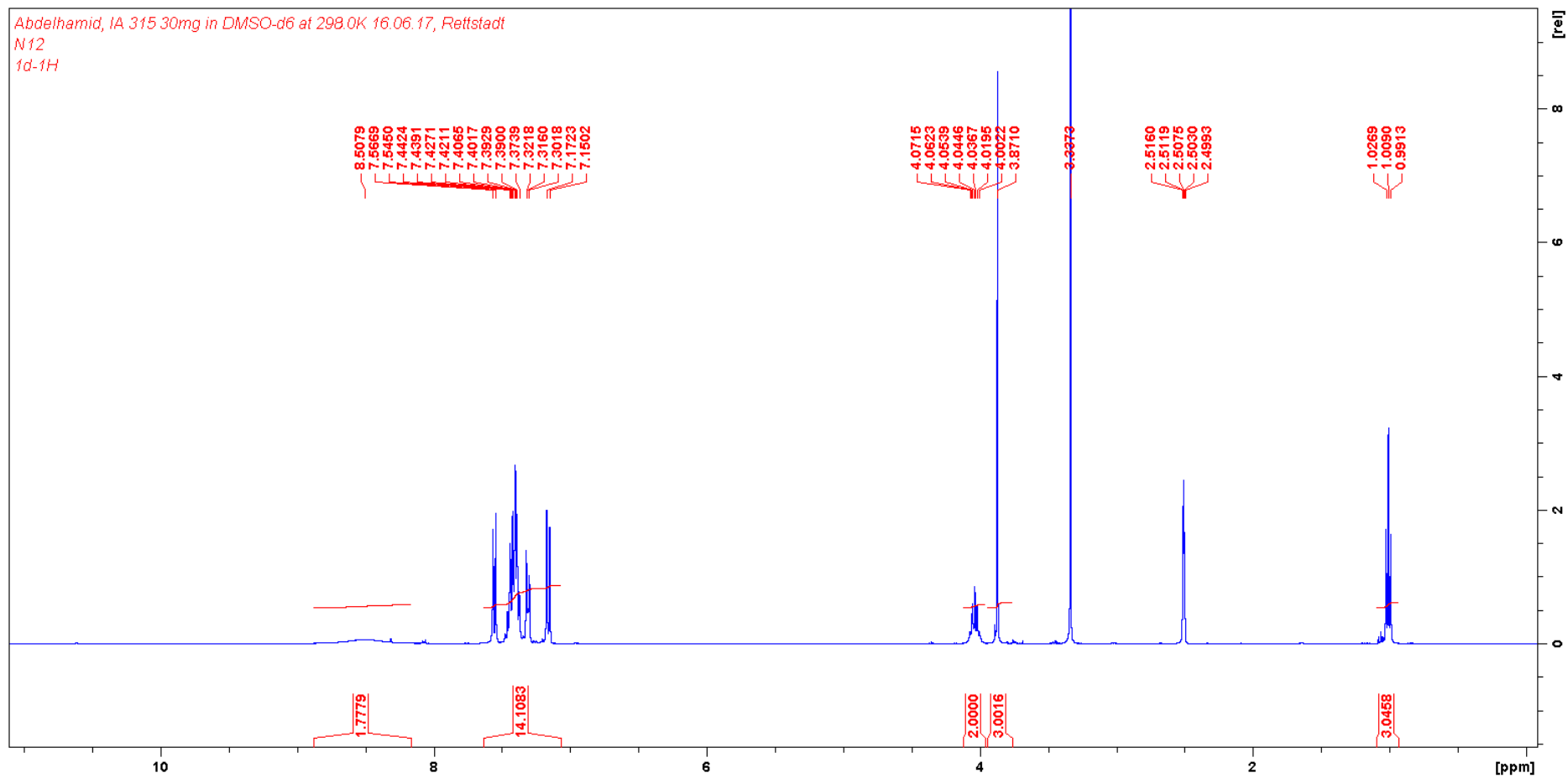
Figure 22. The ^1\text{H} NMR spectrum of compound 20e .
