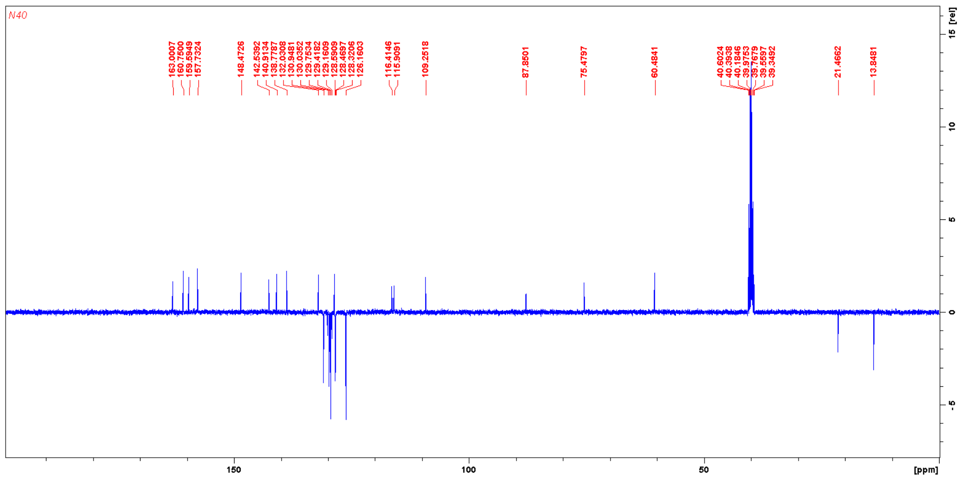
Figure 21. The ^{13}\text{C} NMR spectrum of compound 20d.
