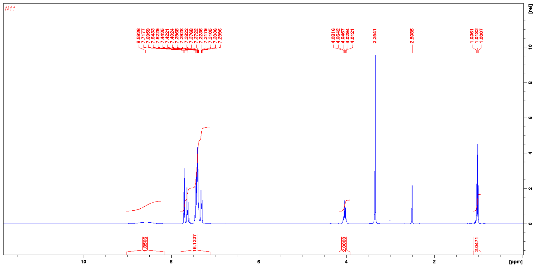
Figure 18. The ^1\text{H} NMR spectrum of compound 20b .
