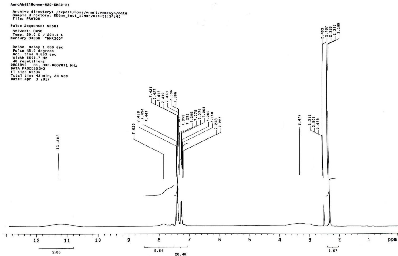
Figure 3. The ^1\text{H} NMR spectrum of compound 7a .
