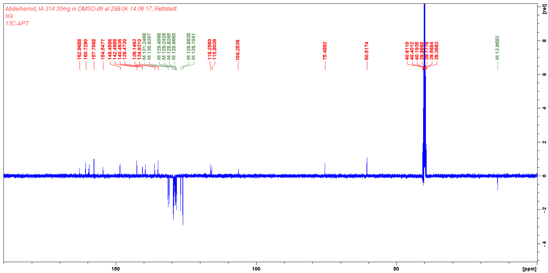
Figure 17. The ^{13}\text{C} NMR spectrum of compound 20a.
