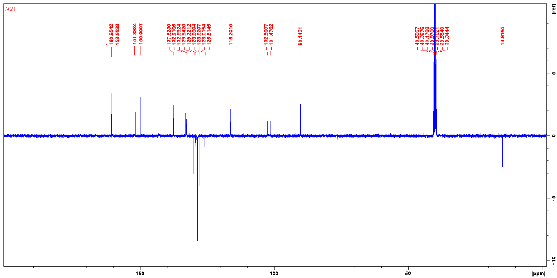
Figure 6. The ^{13}\text{C} NMR spectrum of compound 7b .
