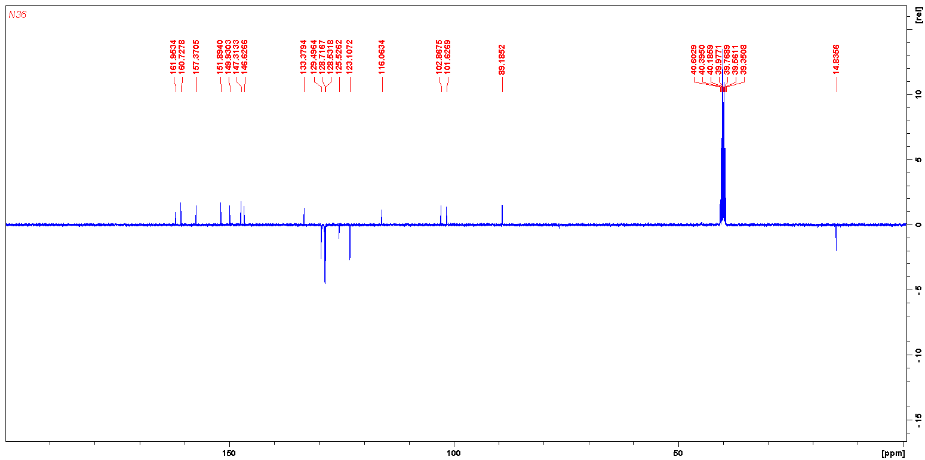
Figure 8. The ^{13}\text{C} NMR spectrum of compound 7c.
