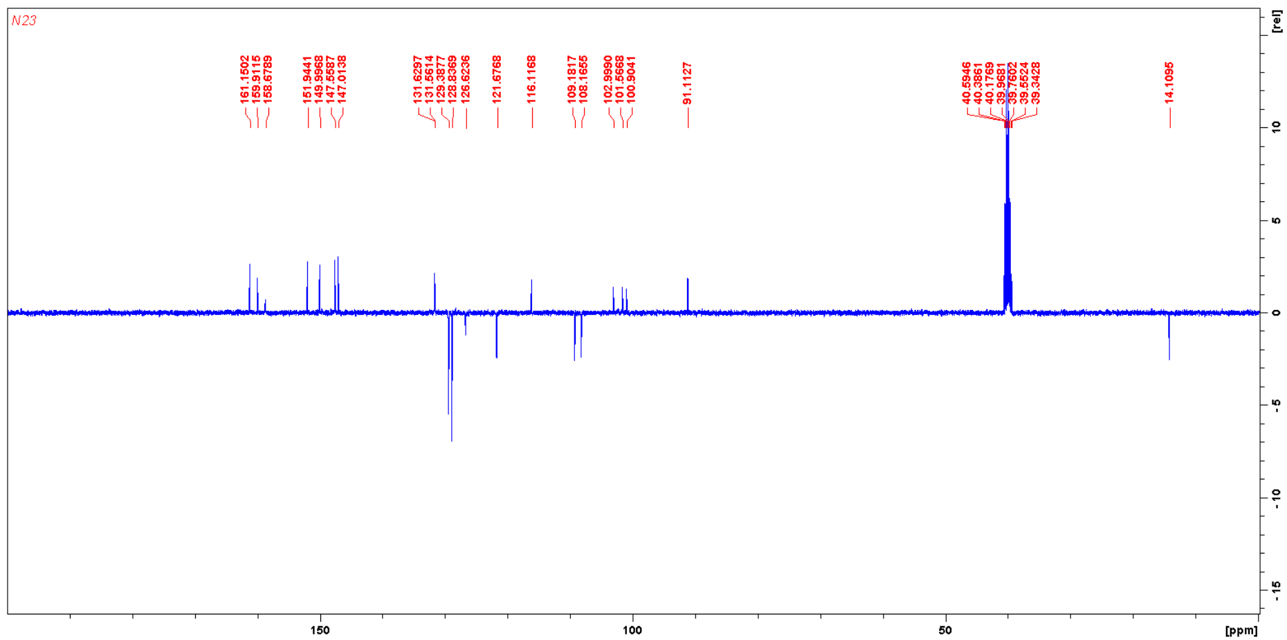
Figure 13. The ^{13}\text{C} NMR spectrum of compound 7f.
