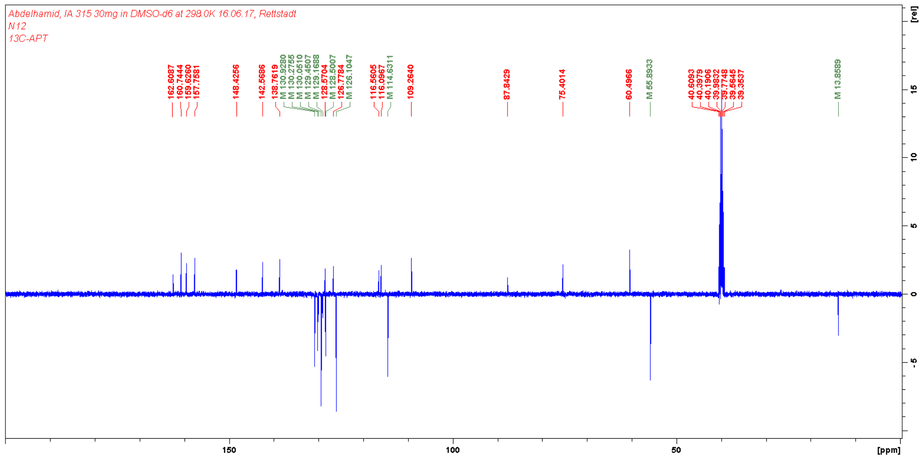
Figure 23. The ^{13}\text{C} NMR spectrum of compound 20e .
