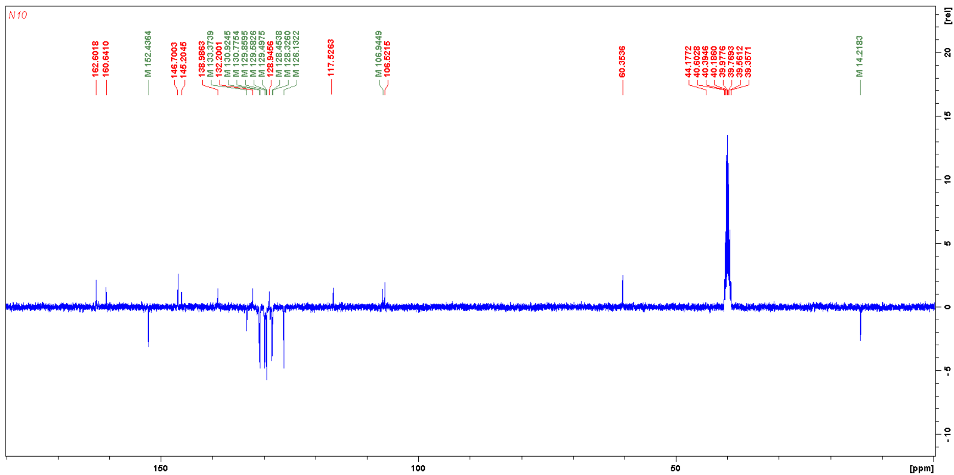
Figure 31. The ^{13}\text{C} NMR spectrum of compound 24a.
