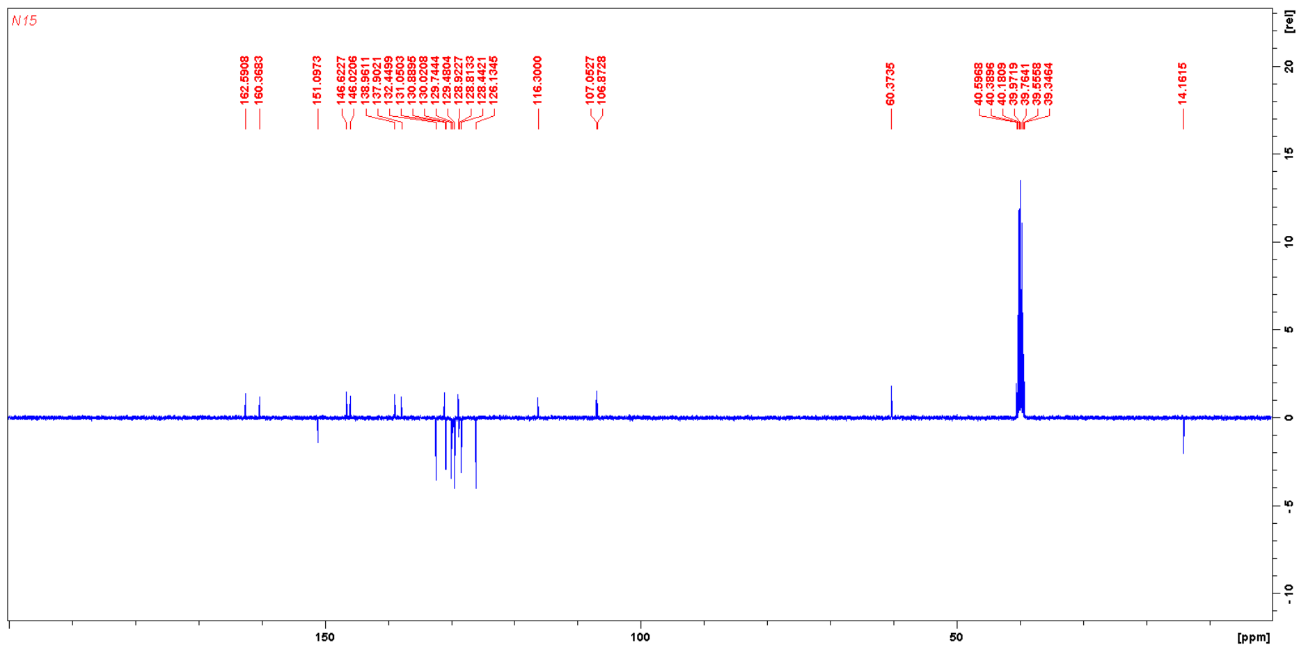
Figure 33. The ^{13}\text{C} NMR spectrum of compound 24b
