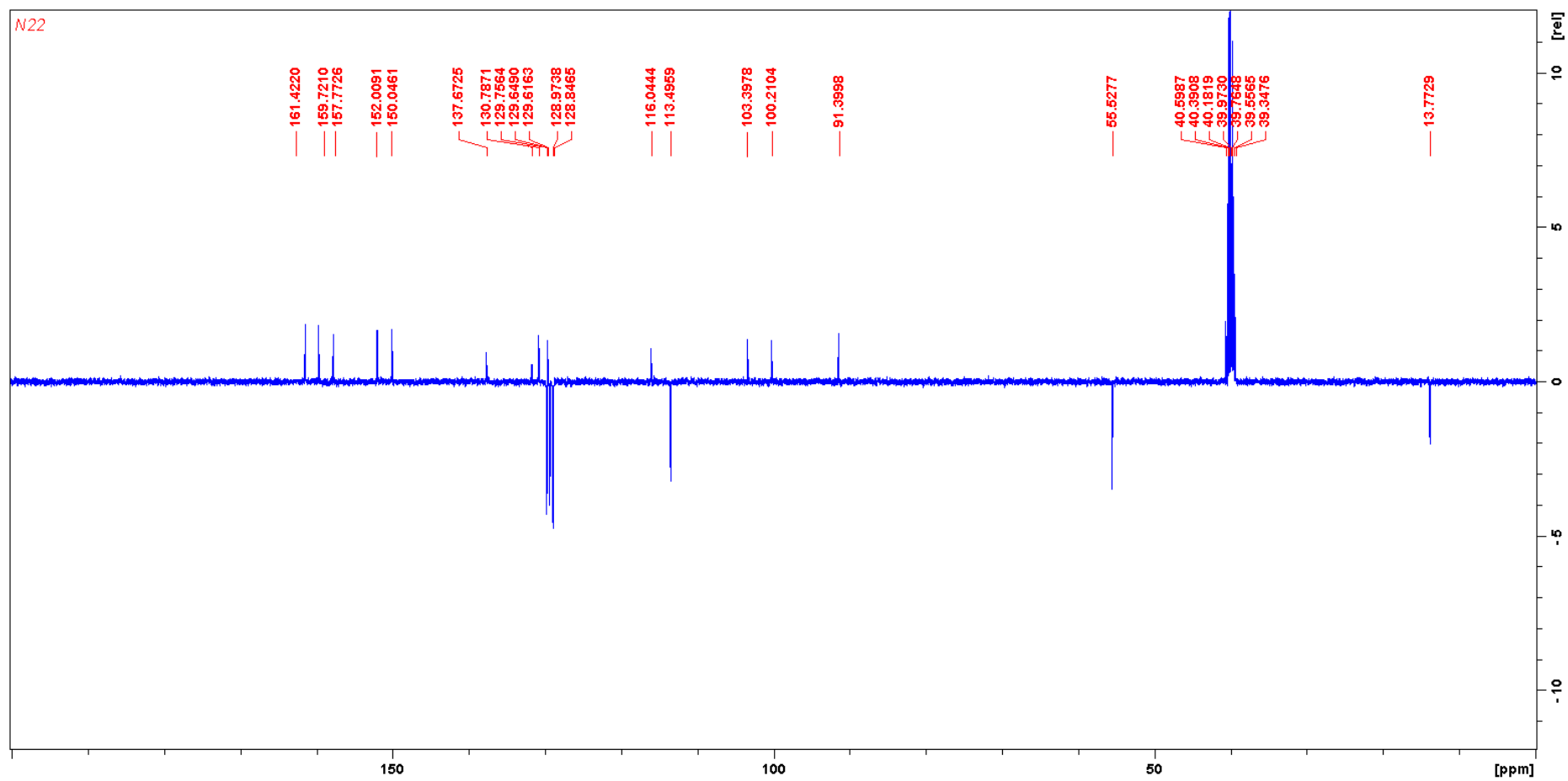
Figure 11. The ^{13}\text{C} NMR spectrum of compound 7e.
