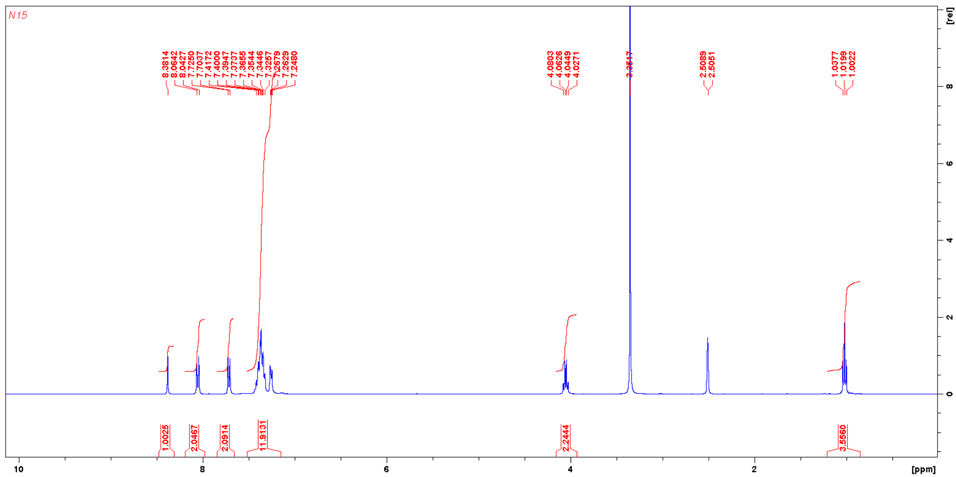
Figure 32. The ^1\text{H} NMR spectrum of compound 24b .
