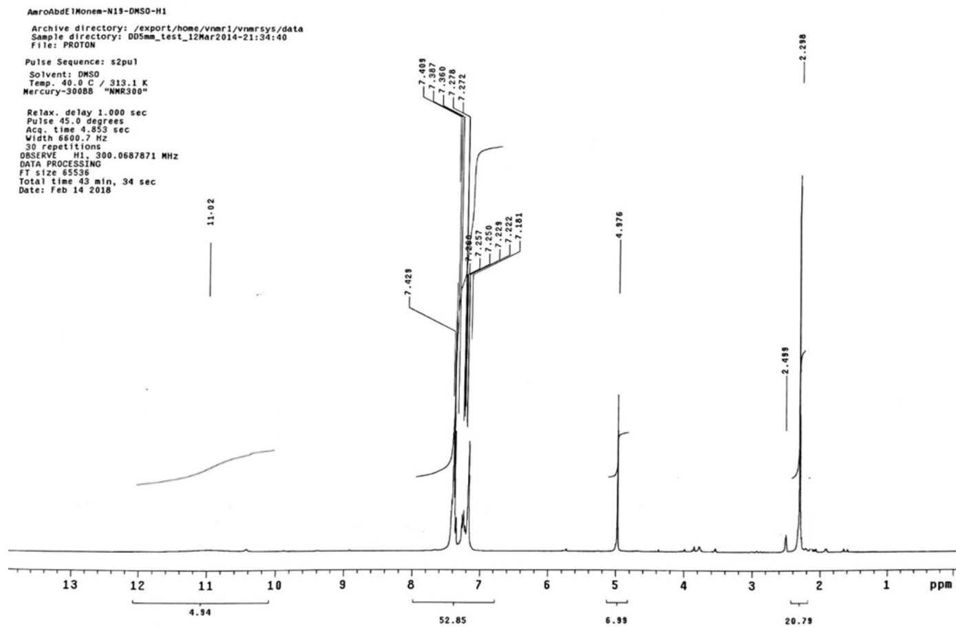
Figure 1. The ^1\text{H} NMR spectrum of compound 5.
