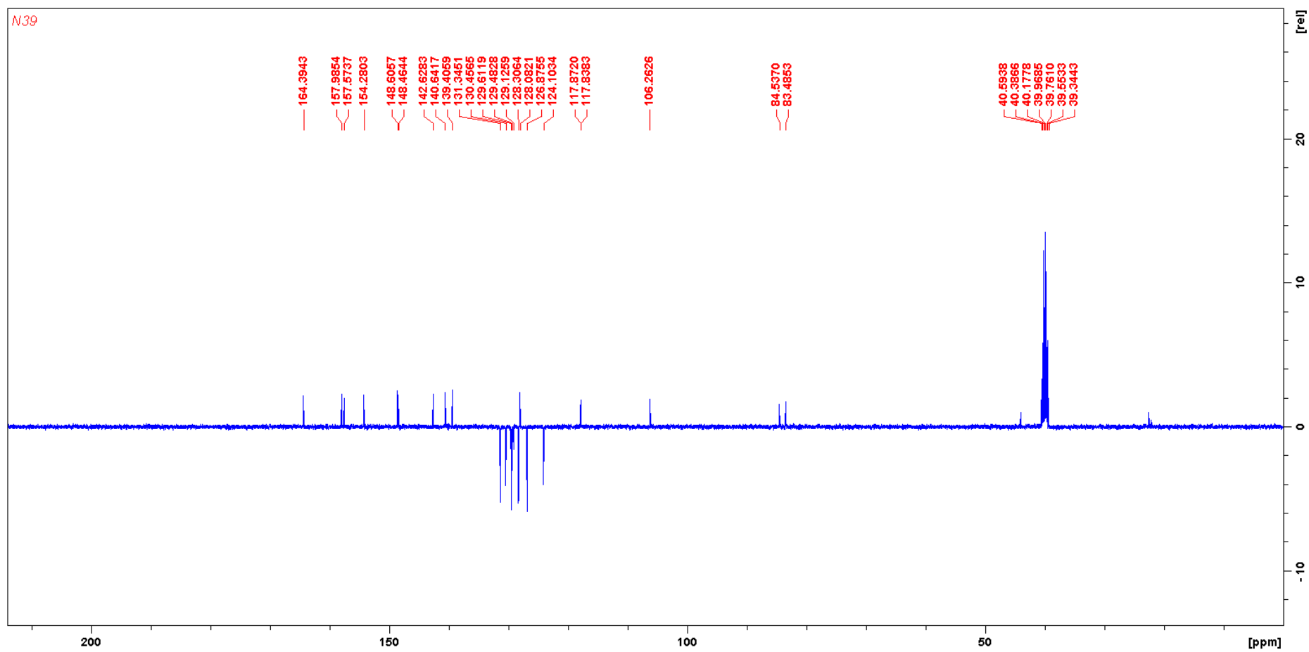
Figure 27. The ^{13}\text{C} NMR spectrum of compound 21c .
