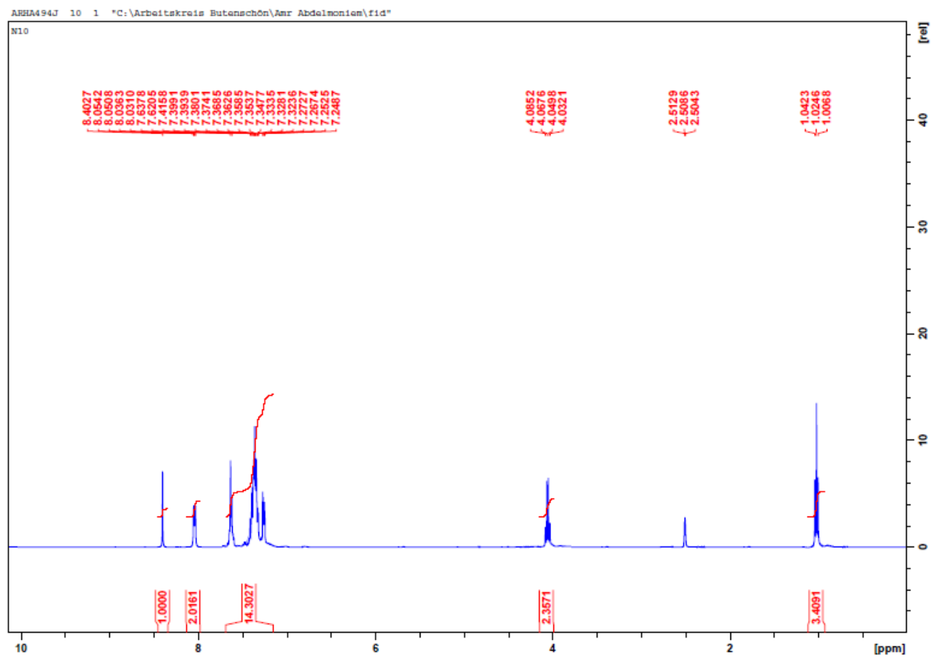
Figure 30. The ^1\text{H} NMR spectrum of compound 24a.
