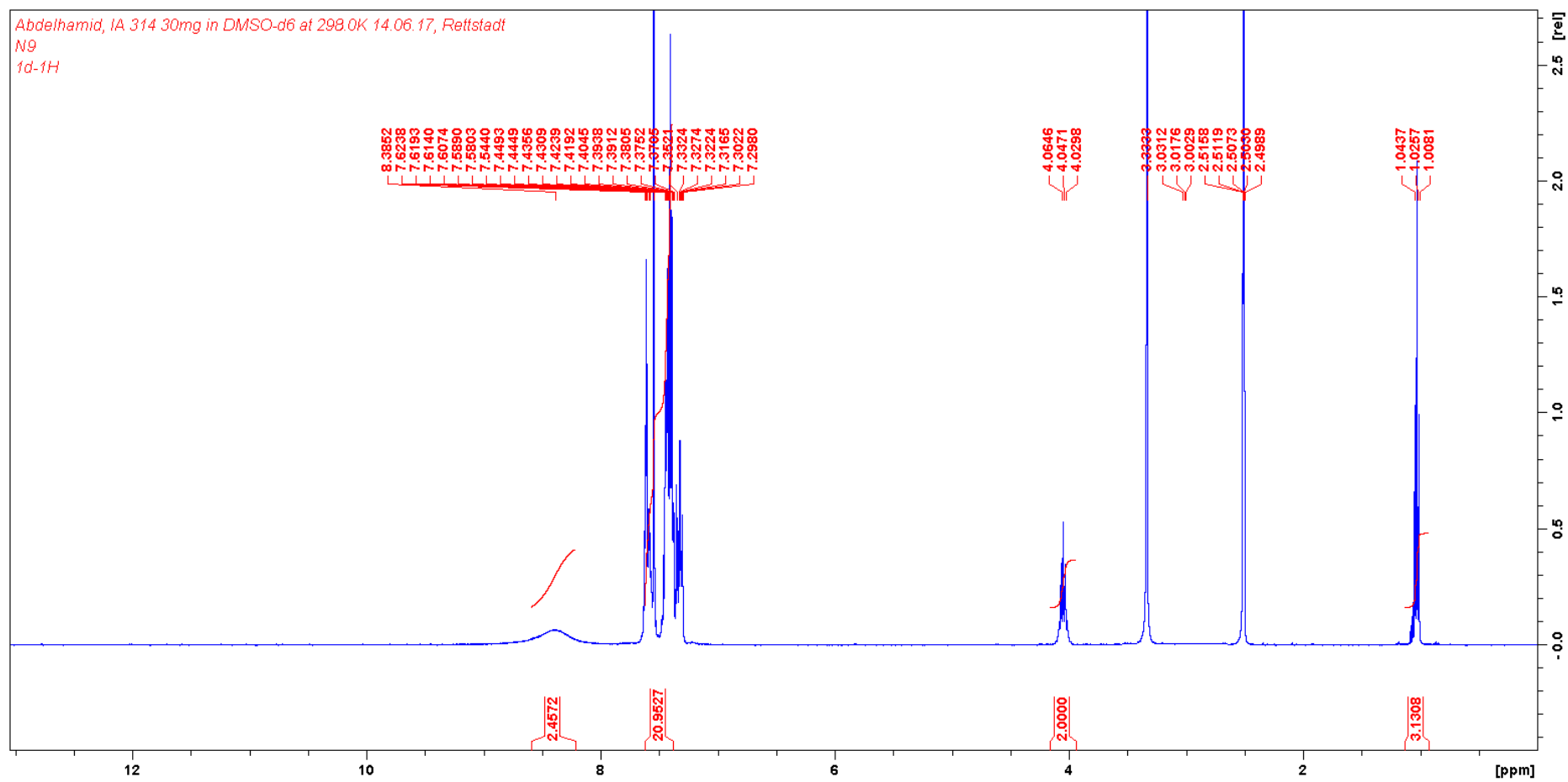
Figure 16. The ^1\text{H} NMR spectrum of compound 20a.
