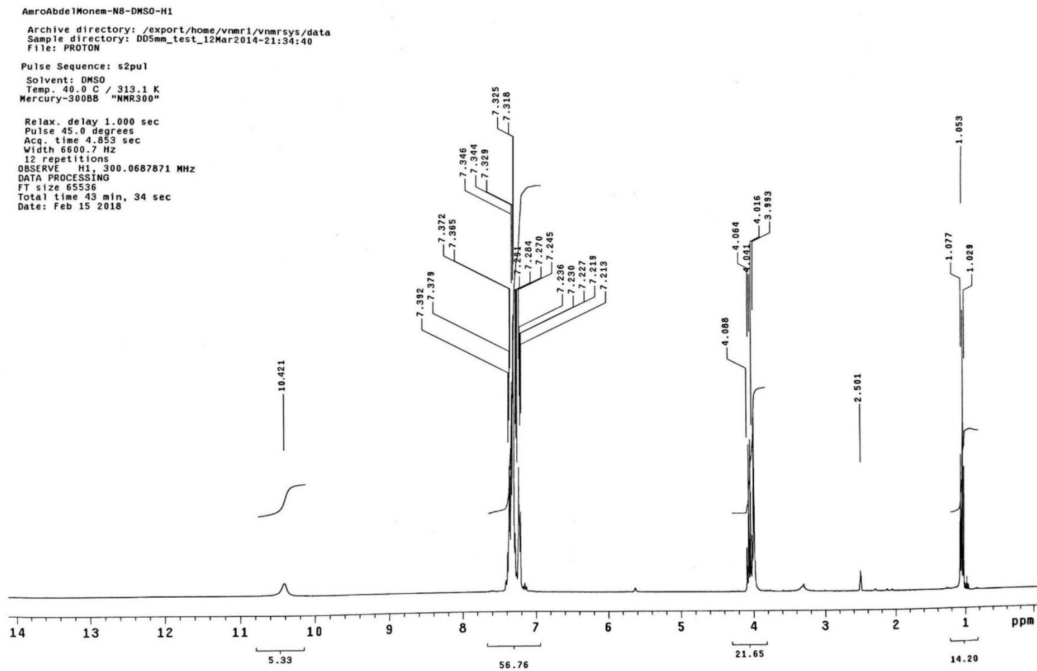
Figure 14. The ^1\text{H} NMR spectrum of compound 18 .
