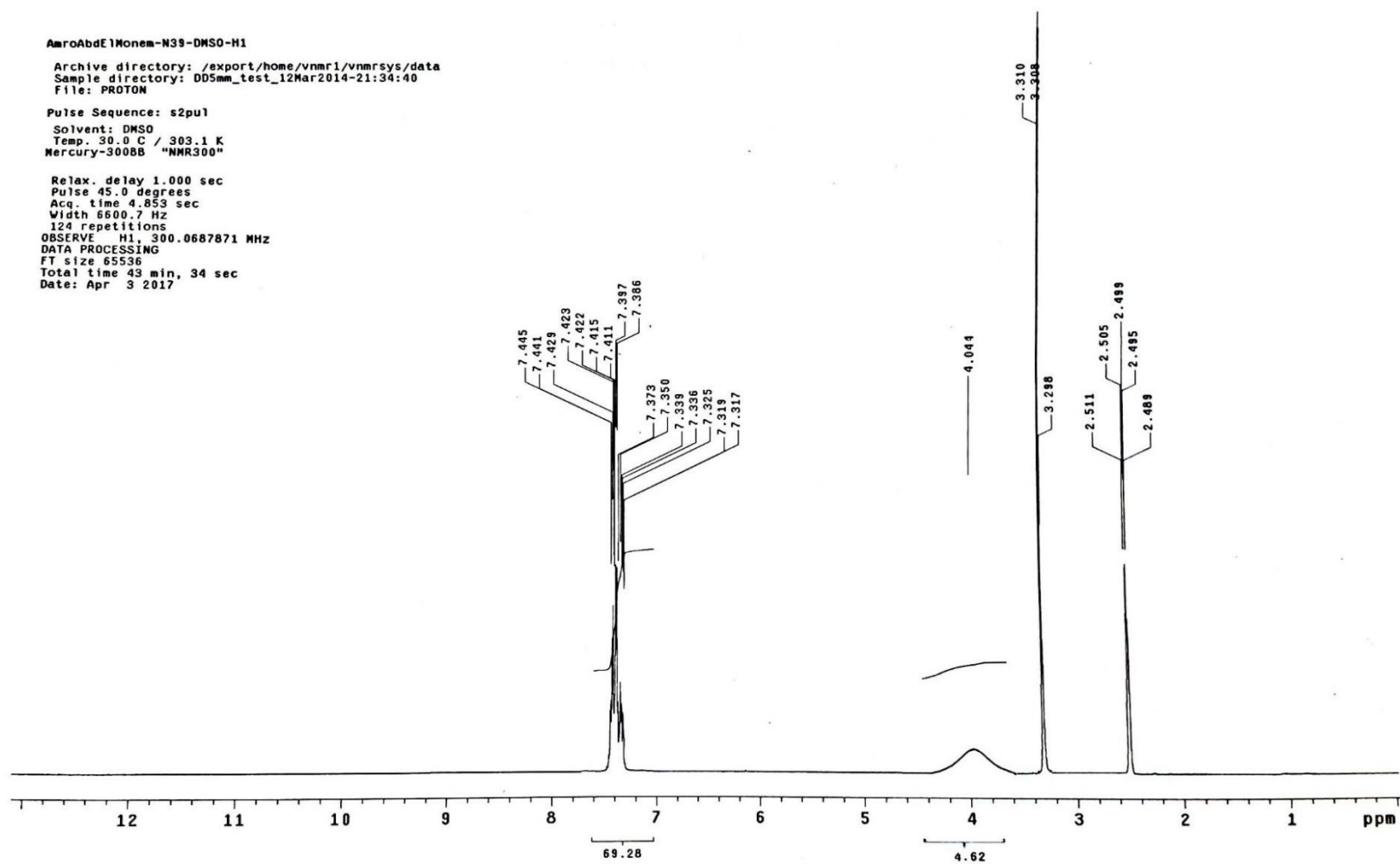
Figure 26. The ^1\text{H} NMR spectrum of compound 21c.
