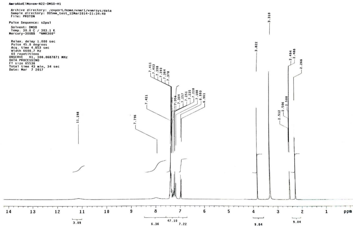
Figure 10. The ^1\text{H} NMR spectrum of compound 7e .
