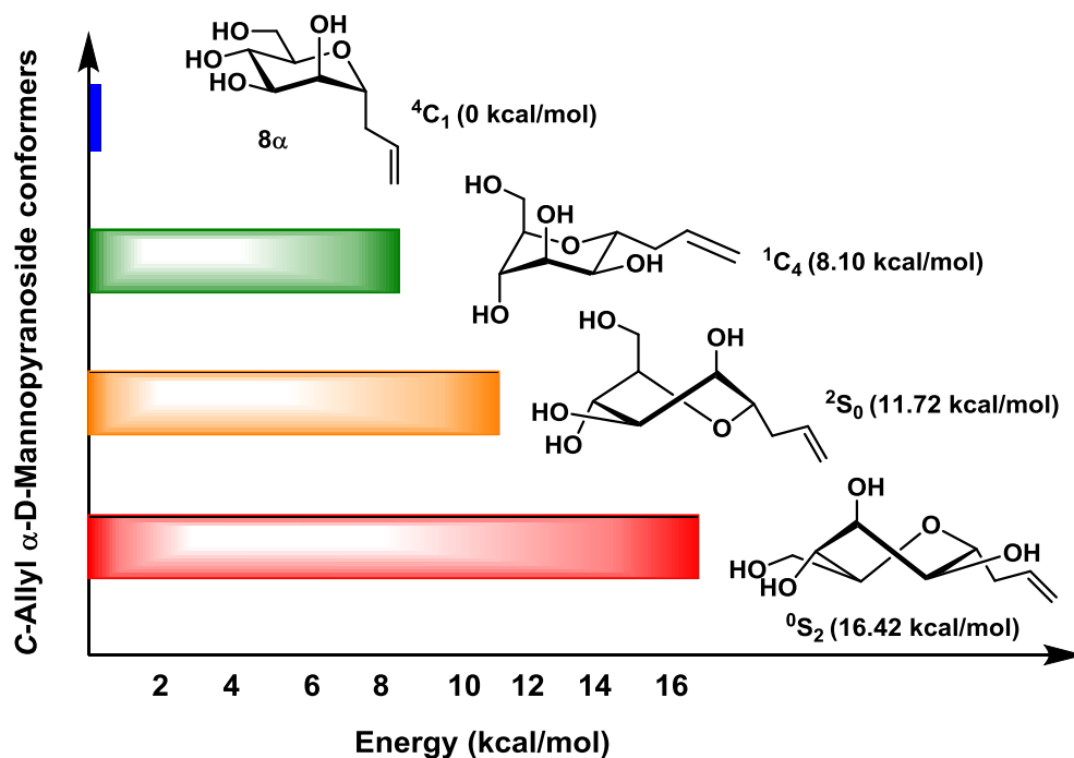
Figure 1. Relative energy level of C-allyl \alpha -D-mannopyranoside ( 8a ) conformers.
