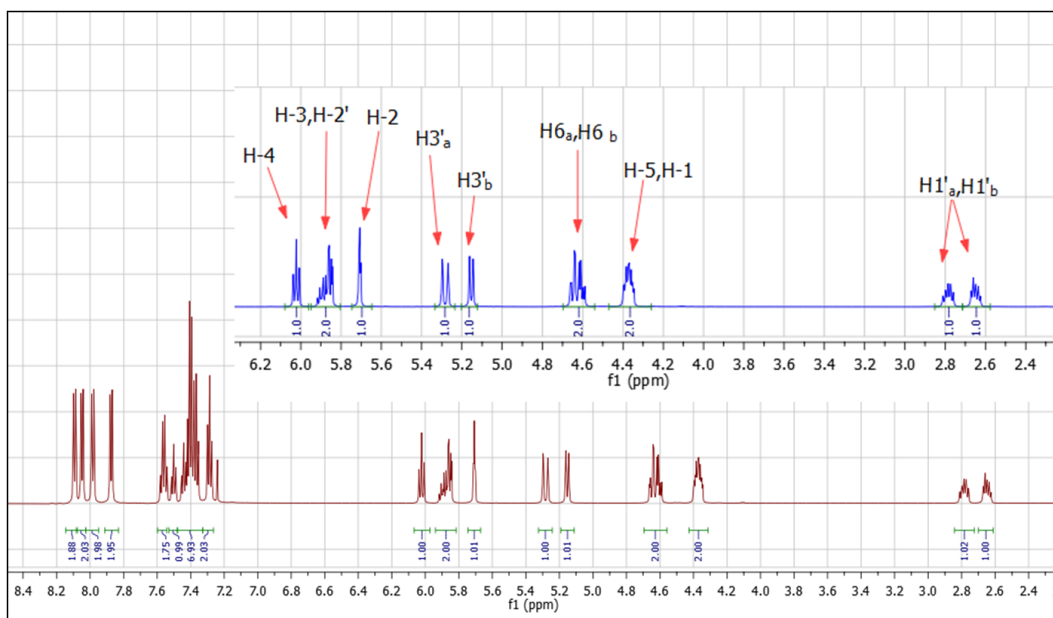
Figure 2. {}^1H NMR ( CDCl_3 , 600 MHz) of perbenzoylated C-allyl \alpha -D-mannopyranoside 5a .
