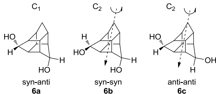
Figure 1. Isomerism and symmetry of 4,7-disubstituted- D 3 -trishomocubane with the same substituents.
