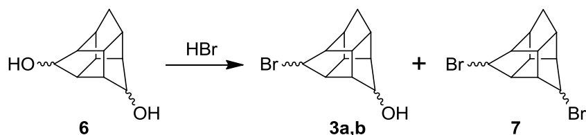
Scheme 2. Reaction of D_3 -trishomocubane-4,7-diol ( 6 ) with HBr.
