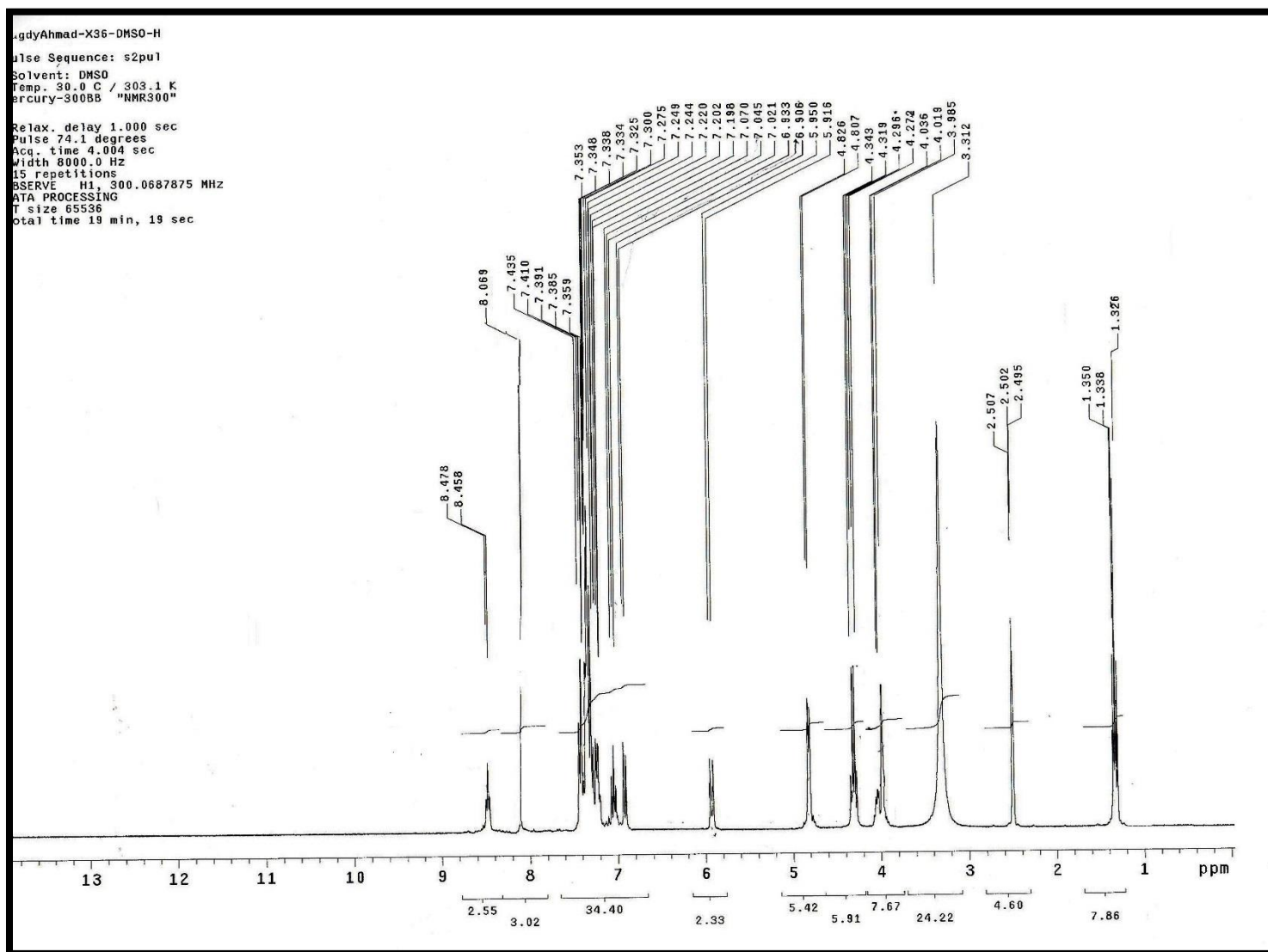
Figure 18. ^1\text{H} NMR spectrum of compound 9 (DMSO)
