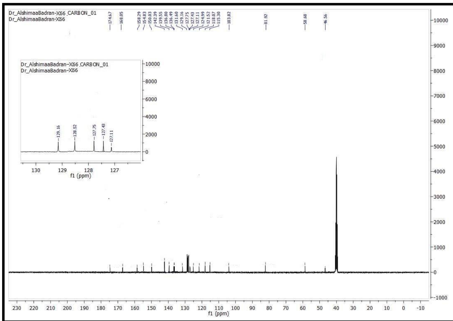
Figure 29. ^{13}\text{C} NMR spectrum of compound 11
