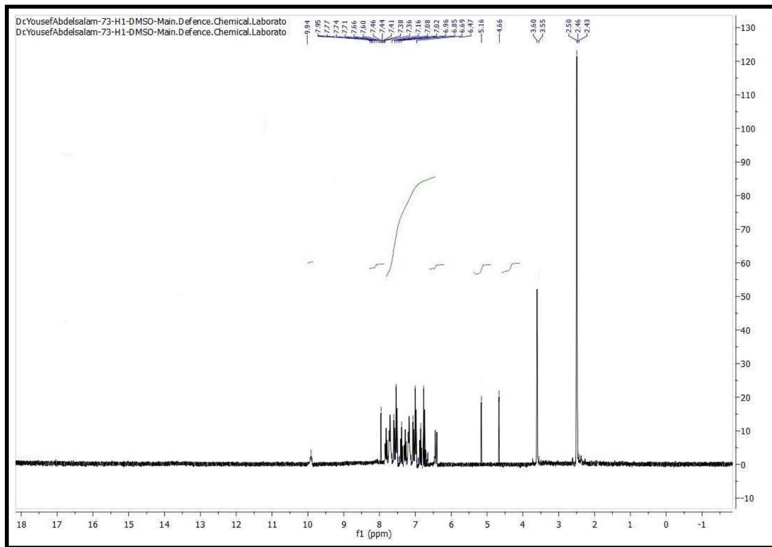
Figure 2. ^1\text{H} NMR spectrum of compound 5
