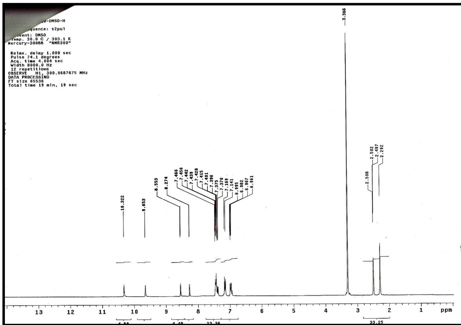
Figure 14. ^1\text{H} NMR spectrum of compound 8
