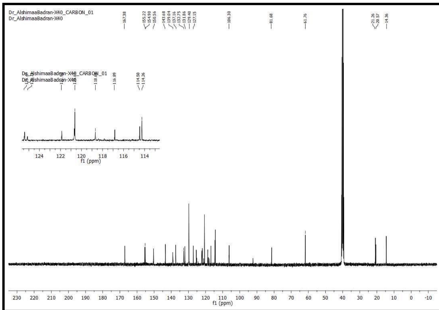
Figure 25. ^{13}\text{C} NMR spectrum of compound 10
