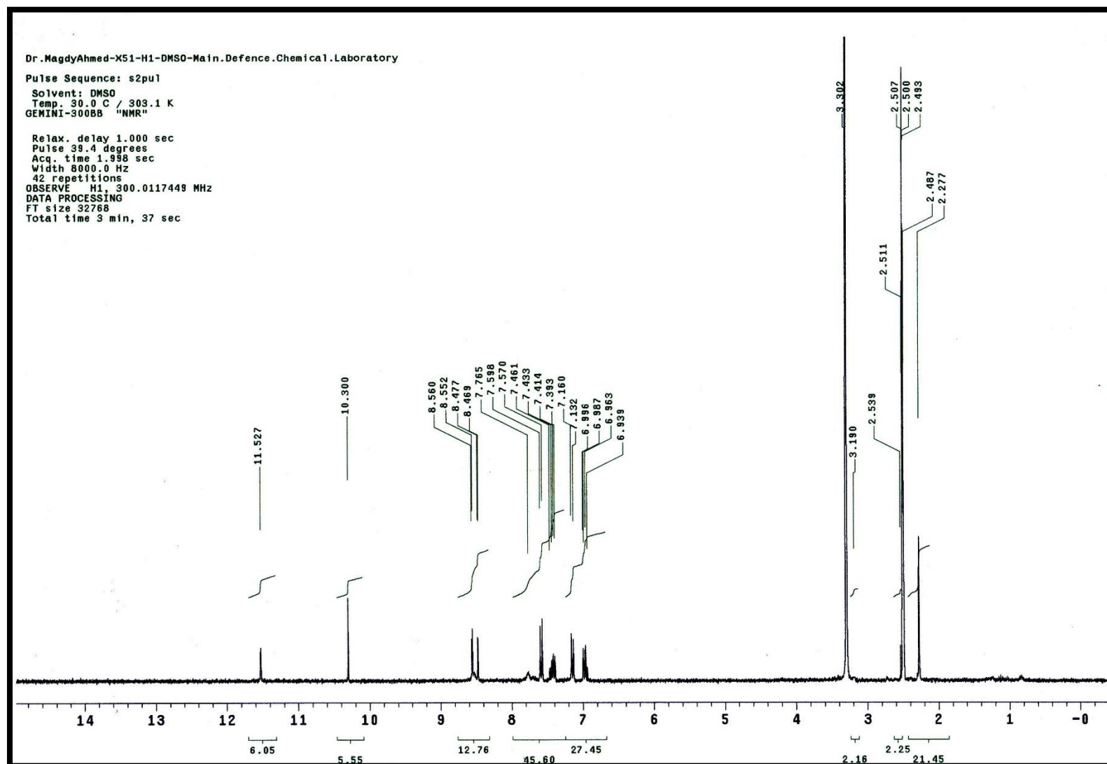
Figure 32. ^1\text{H} NMR spectrum of compound 12
