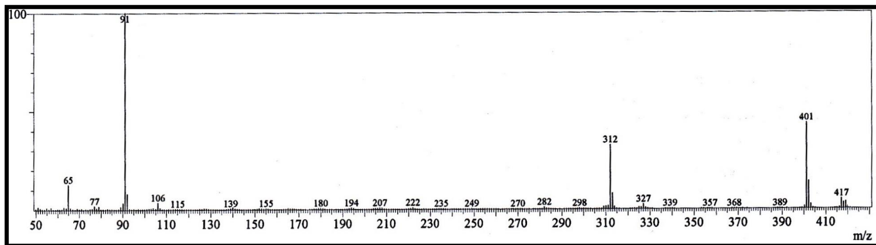
Figure 12. Mass spectrum of compound 7
