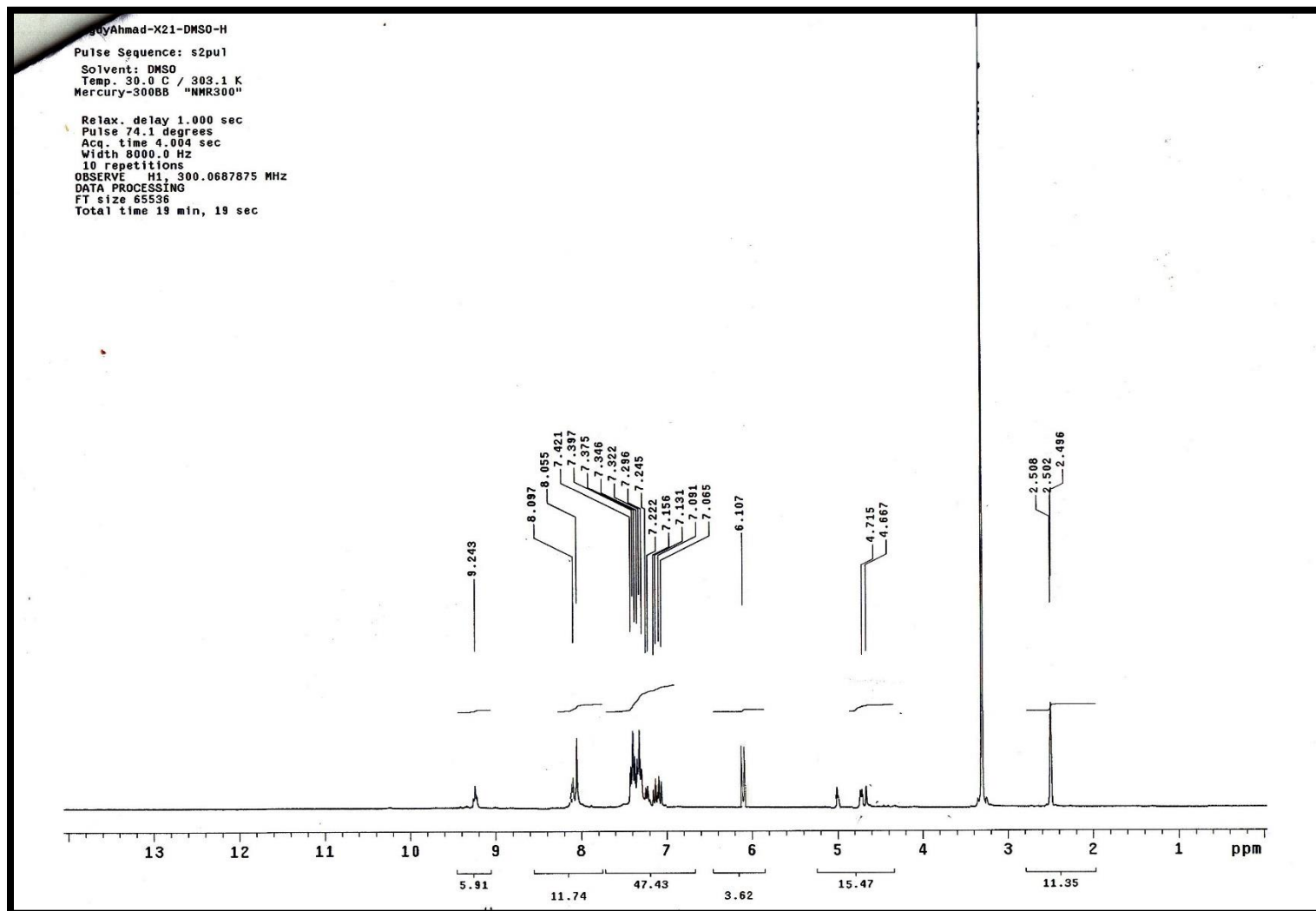
Figure 28. ^1\text{H} NMR spectrum of compound 11
