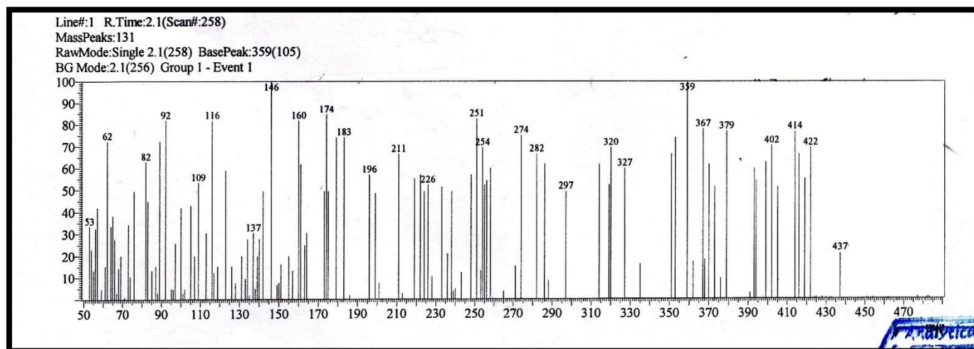
Figure 30. Mass spectrum of compound 11
