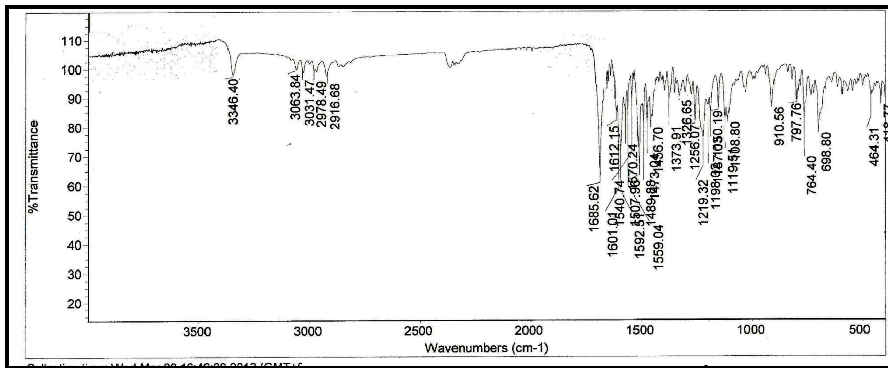
Figure 17. IR spectrum of compound 9
