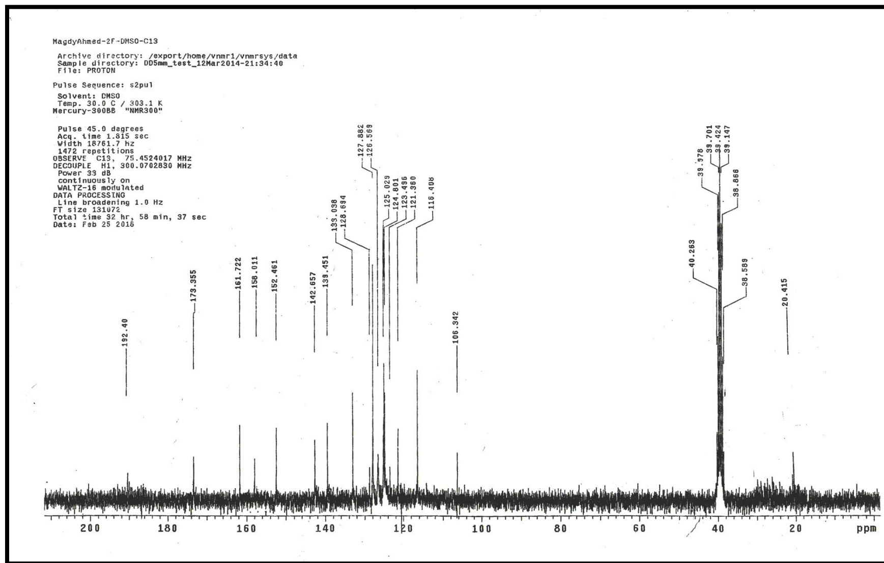
Figure 33. ^{13}\text{C} NMR spectrum of compound 12
