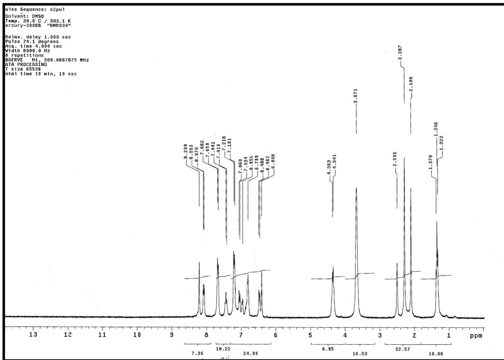
Figure 24. ^1\text{H} NMR spectrum of compound 10 (DMSO + \text{D}_2\text{O} )
