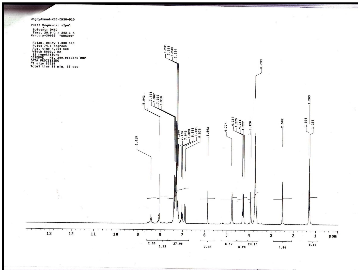
Figure 19. ^1\text{H} NMR spectrum of compound 9 (DMSO+ \text{D}_2\text{O} )
