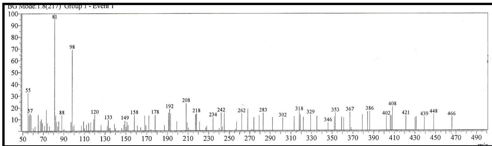
Figure 21. Mass spectrum of compound 9
