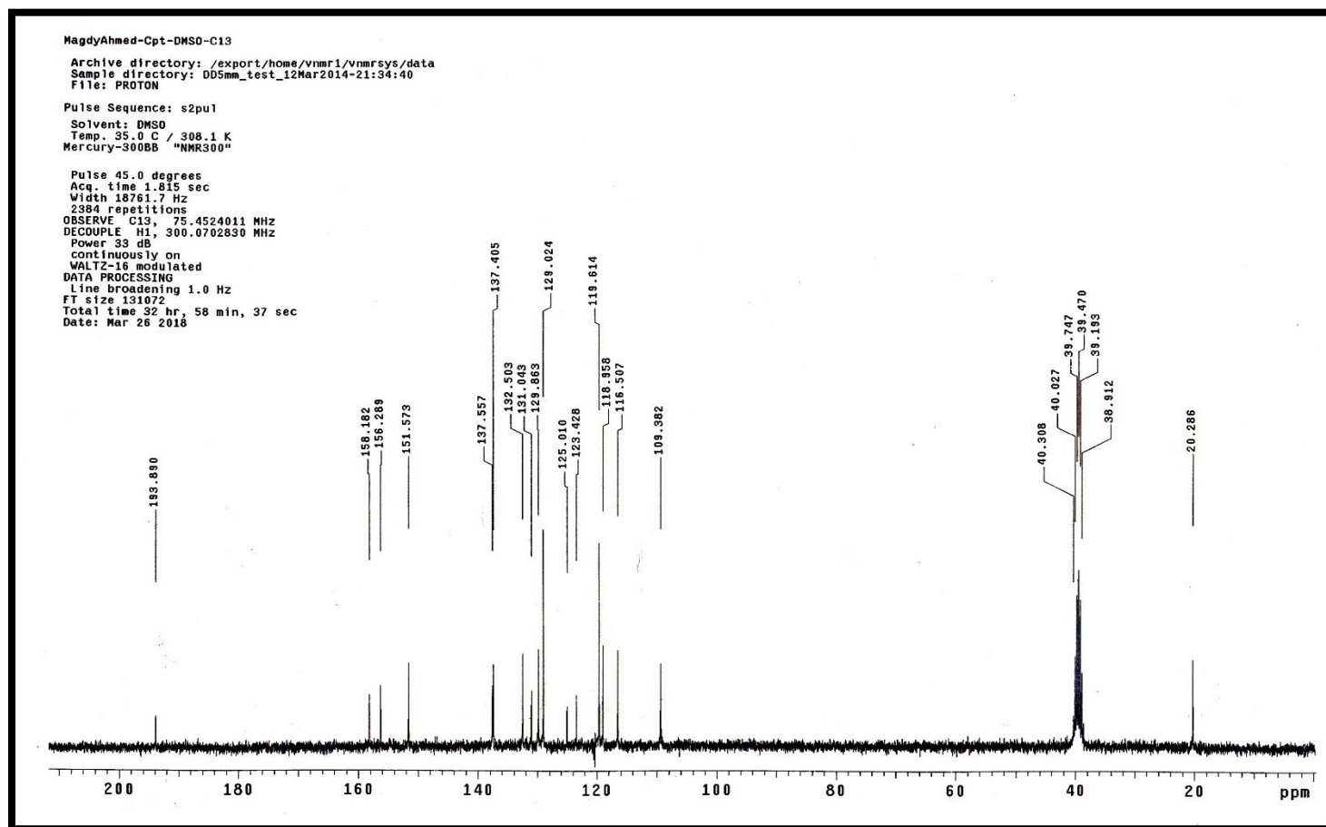
Figure 6. ^{13}\text{C} NMR spectrum of compound 6
