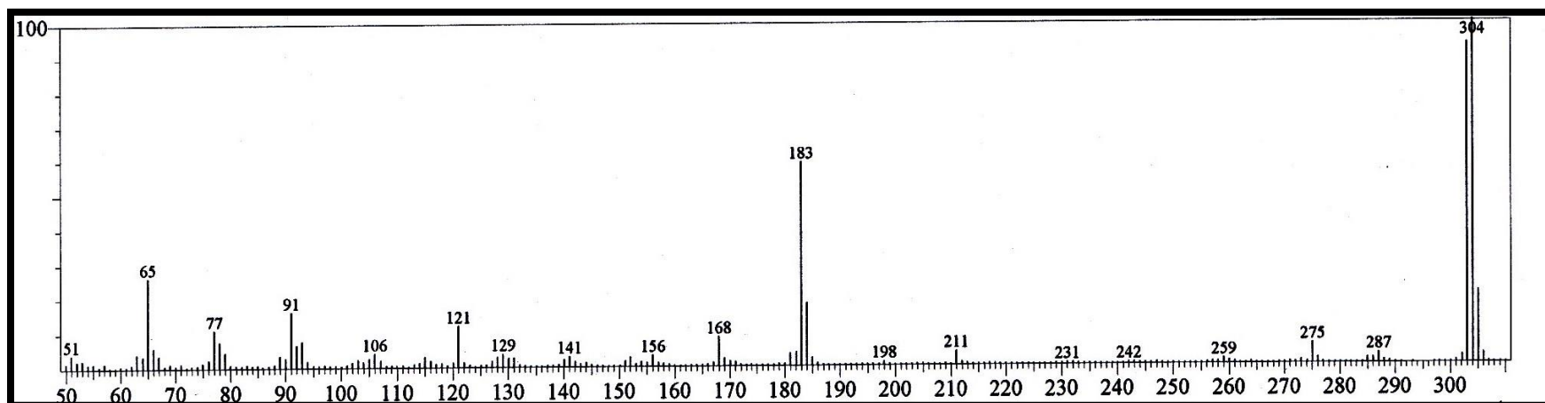
Figure 7. Mass spectrum of compound 6
