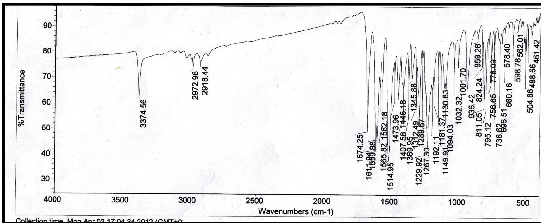
Figure 22. IR spectrum of compound 10
