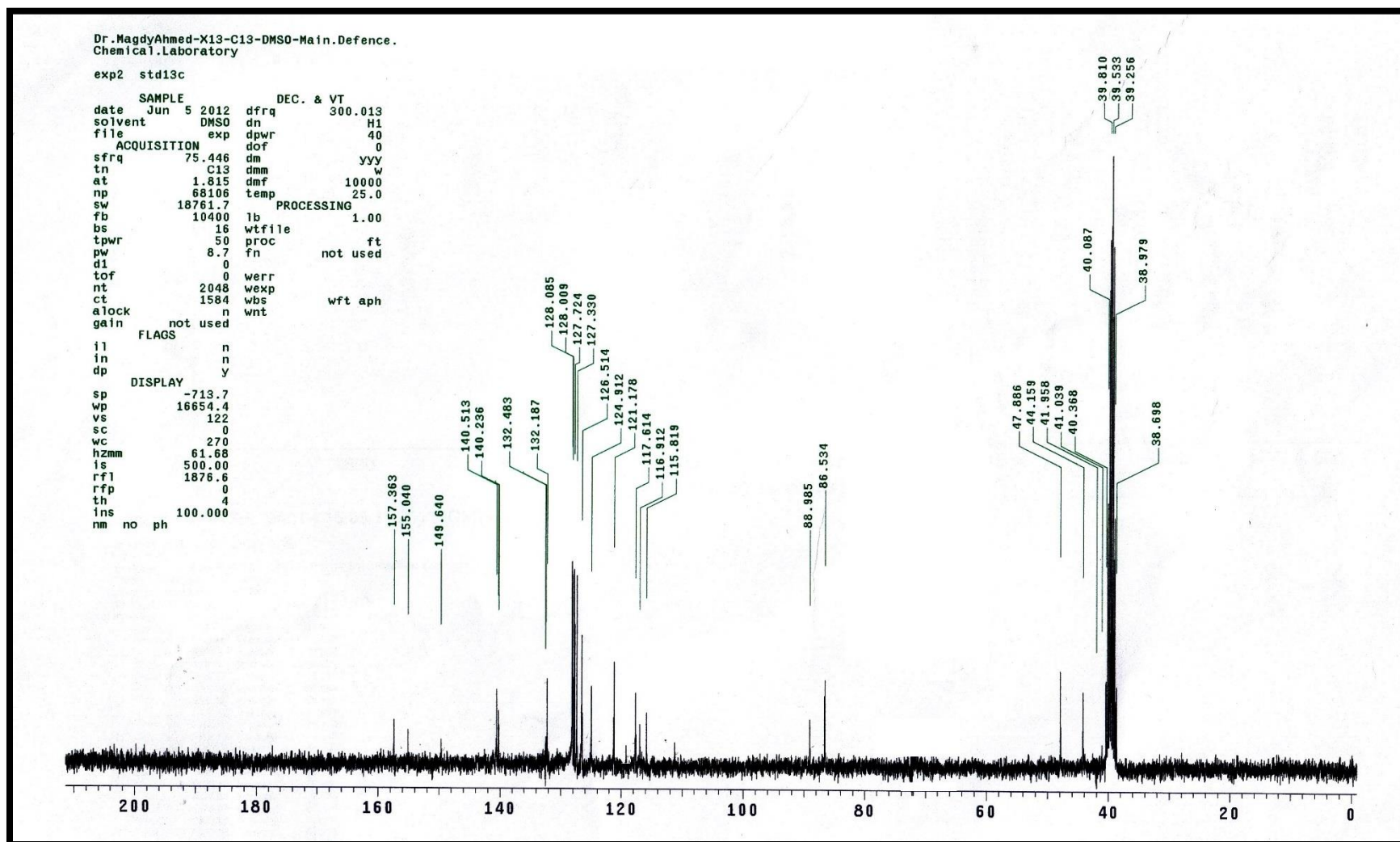
Figure 11. ^{13}\text{C} NMR spectrum of compound 7
