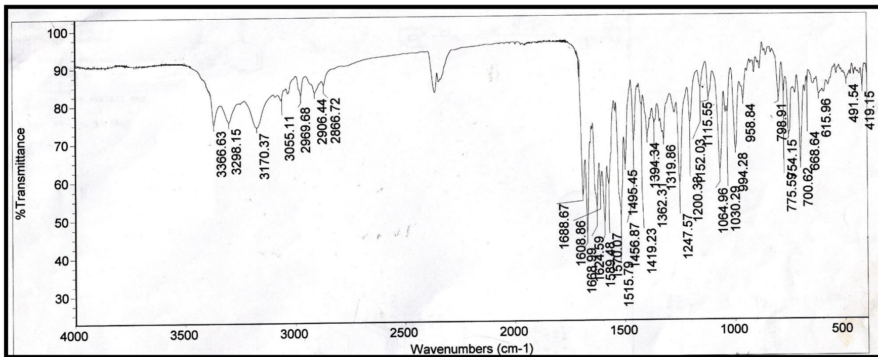
Figure 27. IR spectrum of compound 11
