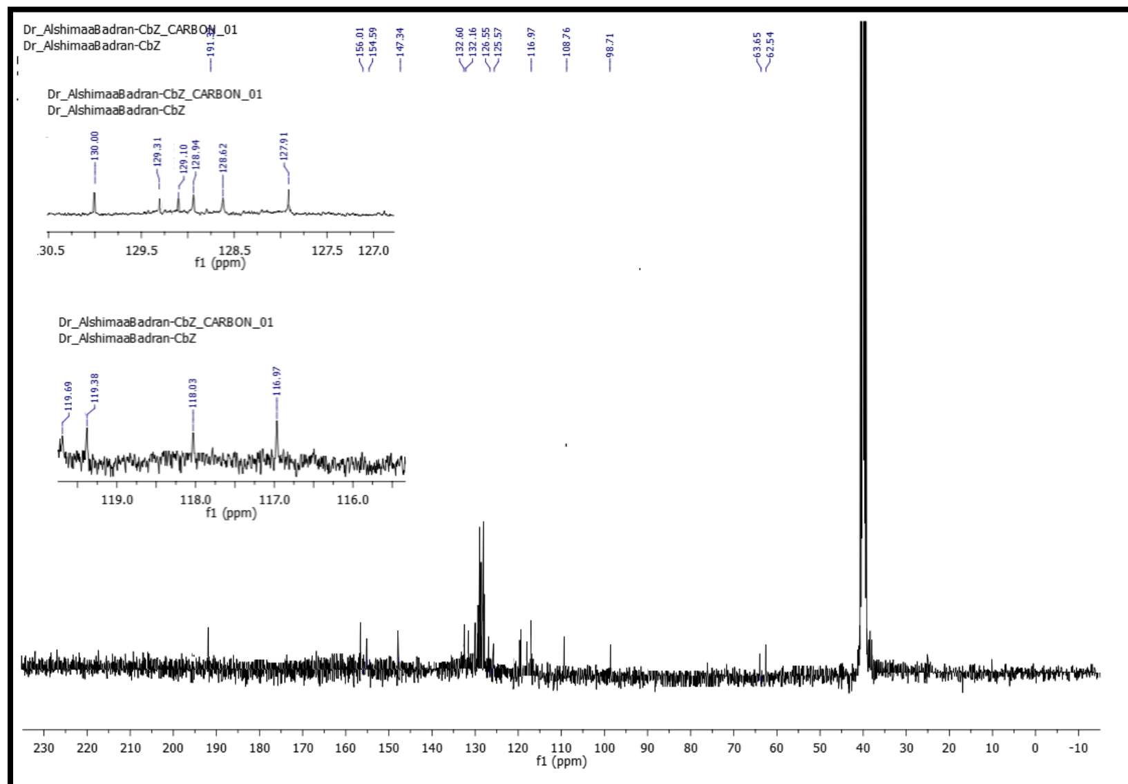
Figure 3. ^{13}\text{C} NMR spectrum of compound 5
