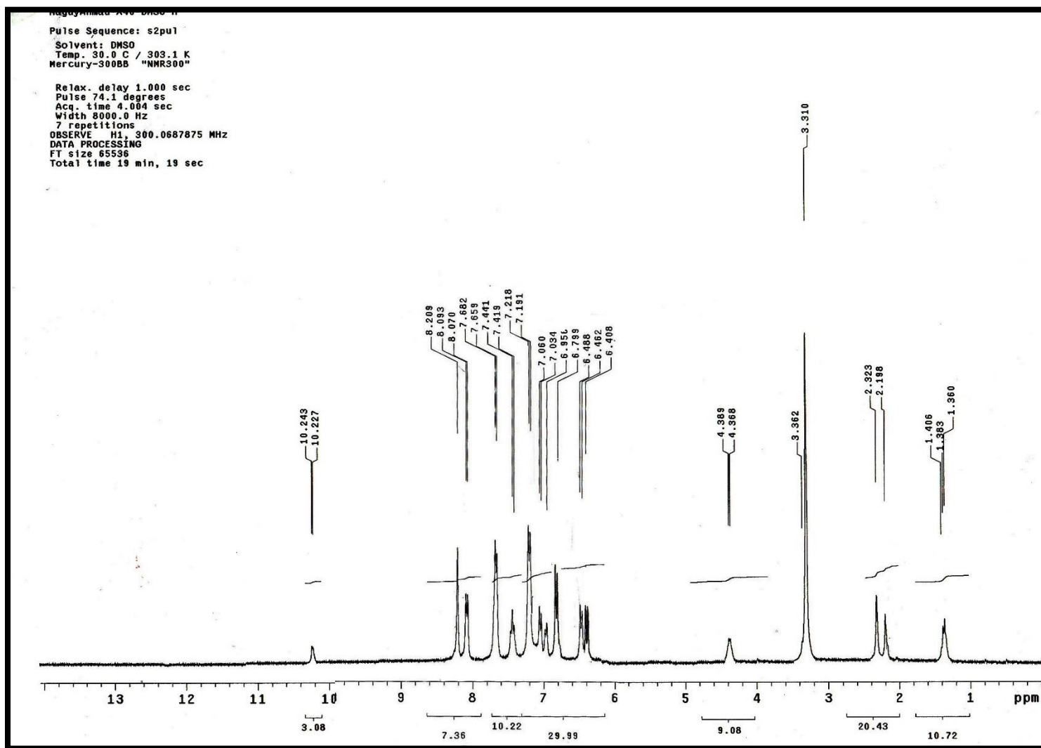
Figure 23. ^1\text{H} NMR spectrum of compound 10 (DMSO)
