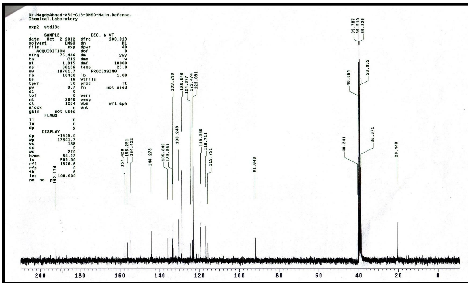
Figure 15. ^{13}\text{C} NMR spectrum of compound 8
