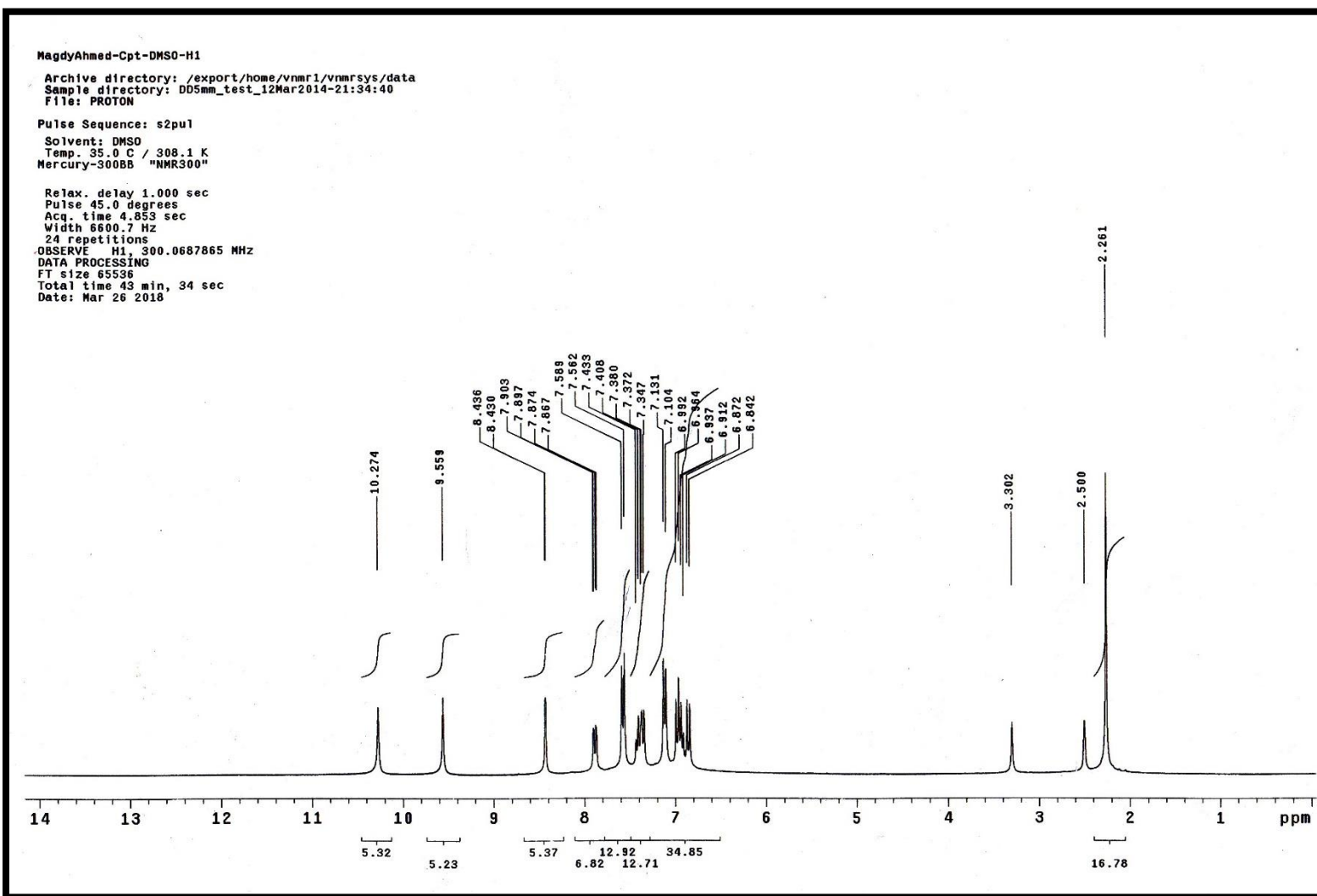
Figure 5. ^1\text{H} NMR spectrum of compound 6
