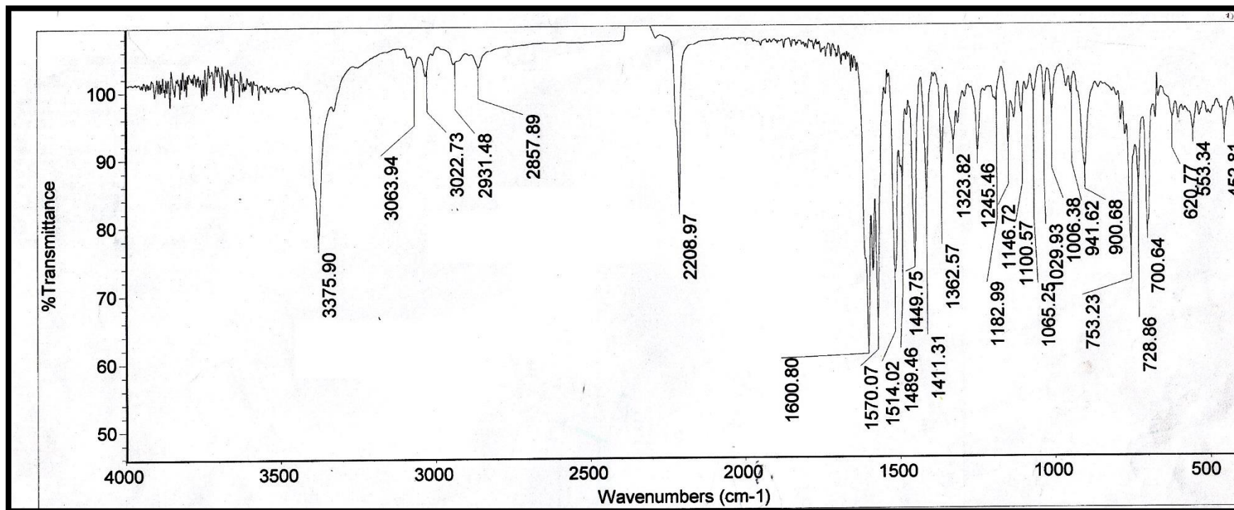
Figure 8. IR spectrum of compound 7
