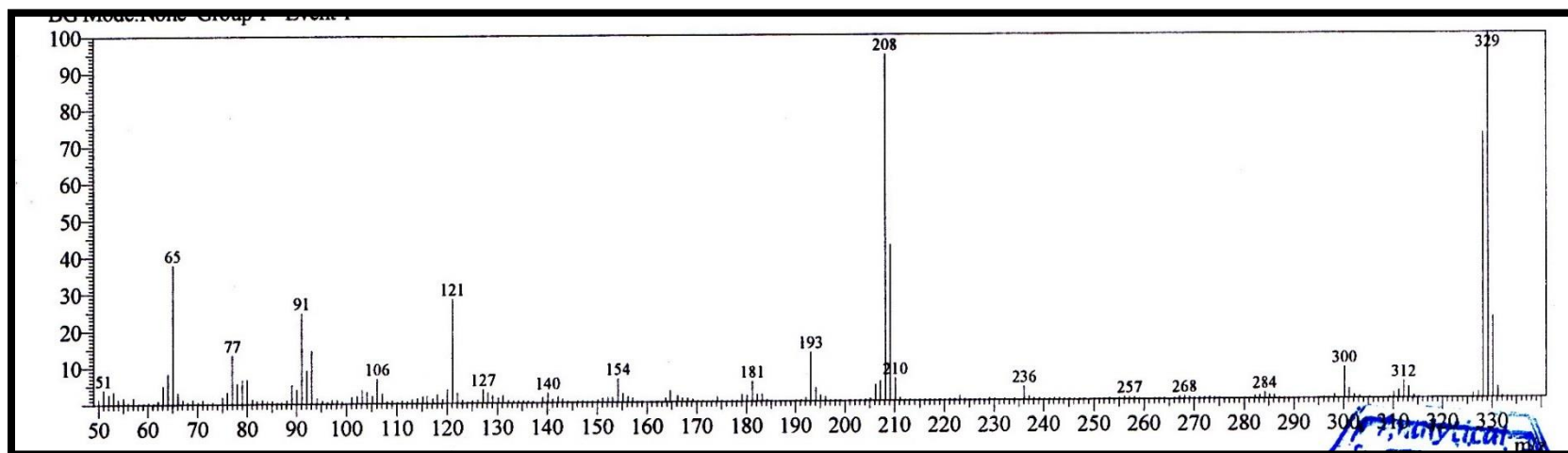
Figure 16. Mass spectrum of compound 8
