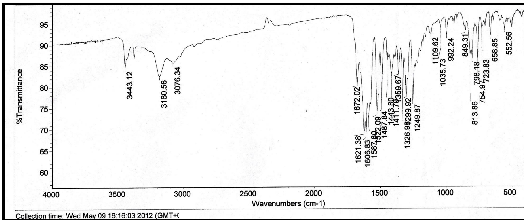
Figure 31. IR spectrum of compound 12
