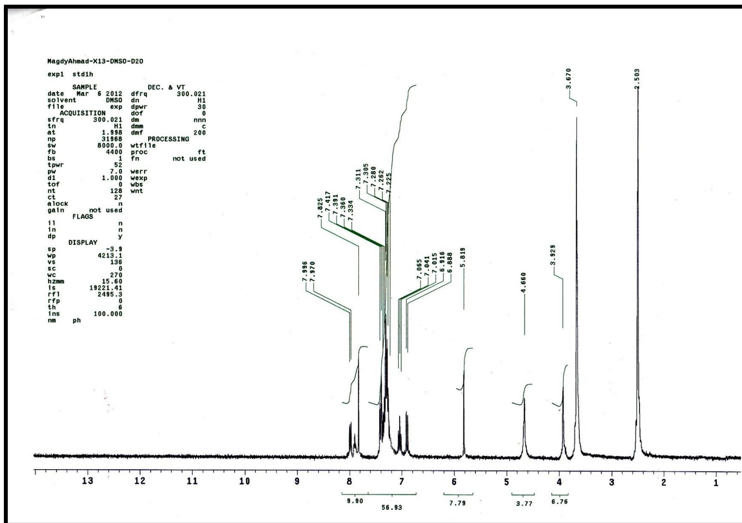
Figure 10. ^1\text{H} NMR spectrum of compound 7 (DMSO+ \text{D}_2\text{O} )
