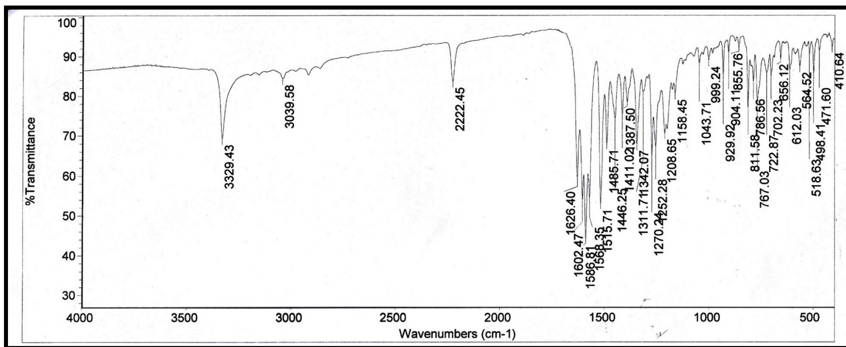
Figure 13. IR spectrum of compound 8
