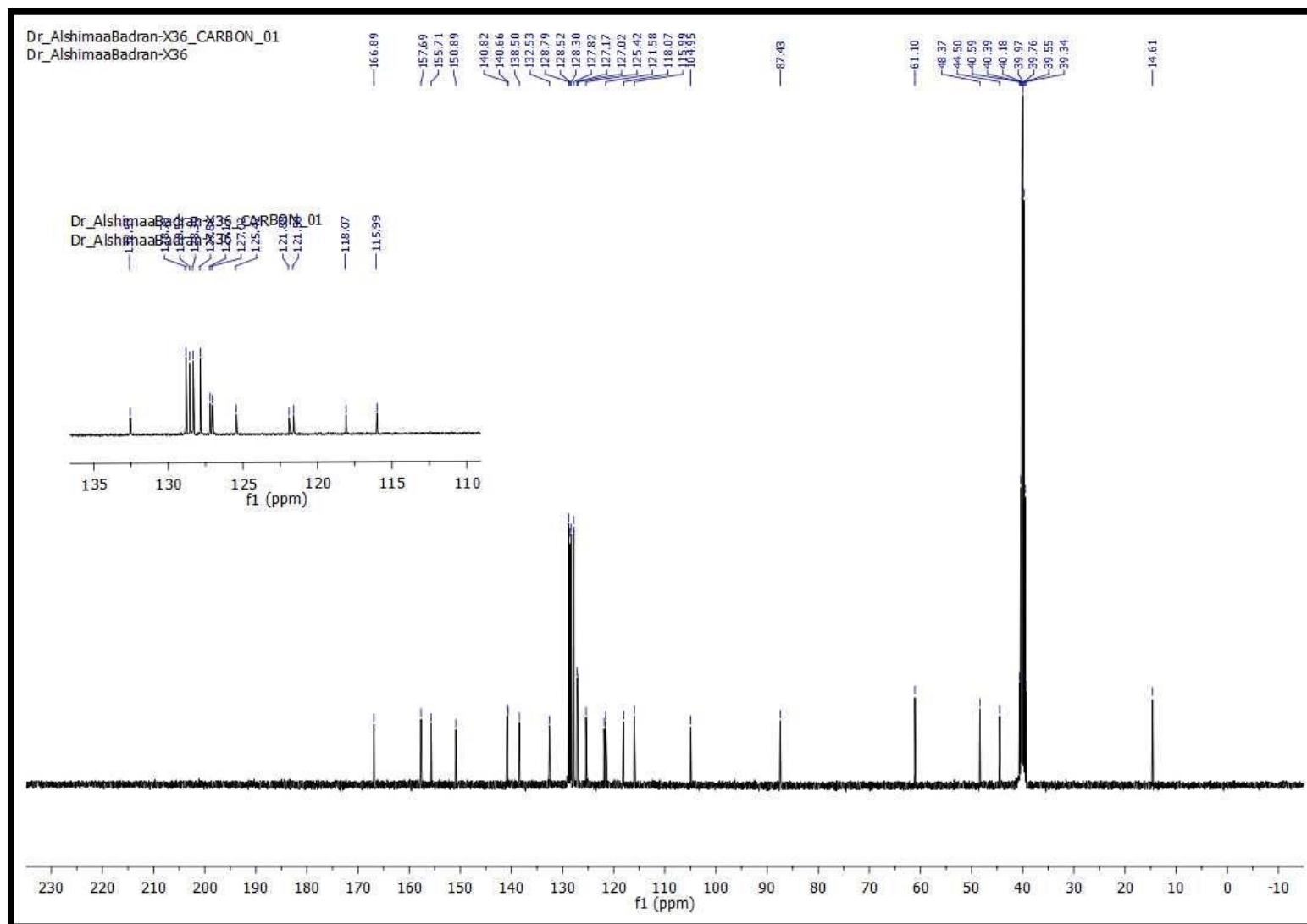
Figure 20. ^{13}\text{C} NMR spectrum of compound 9
