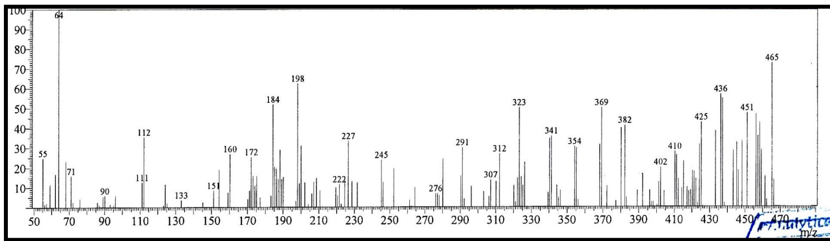
Figure 26. Mass spectrum of compound 10
