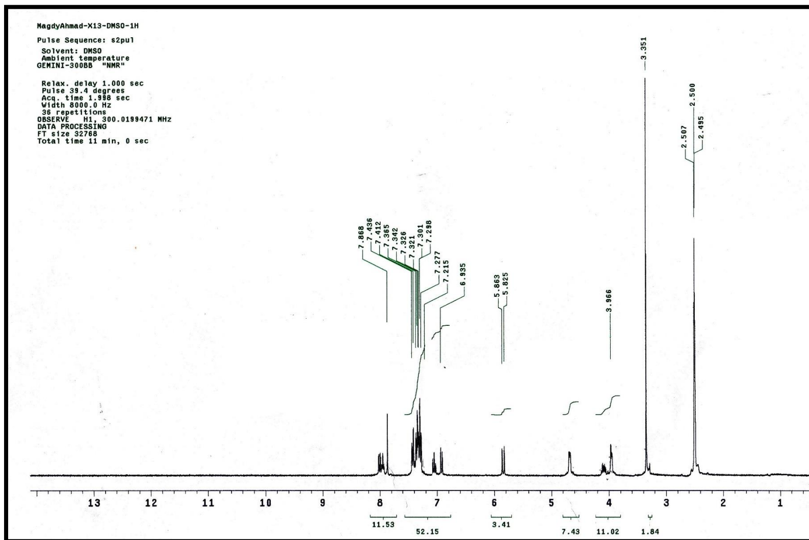
Figure 9. ^1\text{H} NMR spectrum of compound 7 (DMSO)
