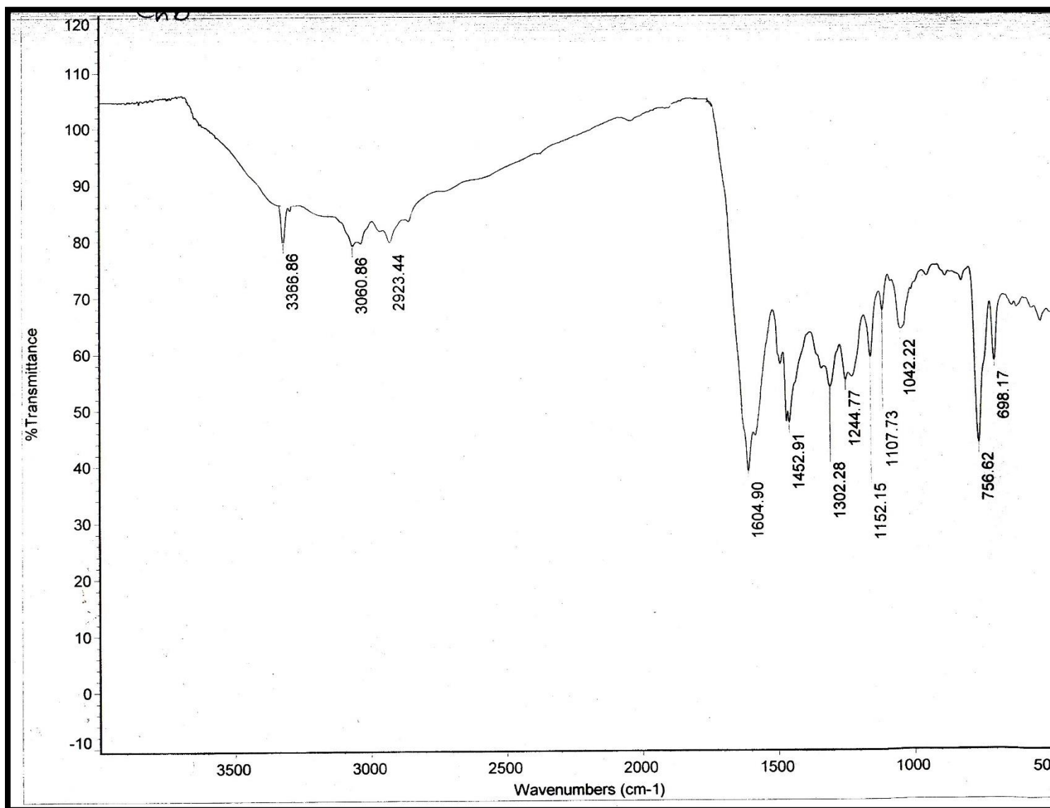
Figure 1. IR spectrum of compound 5
