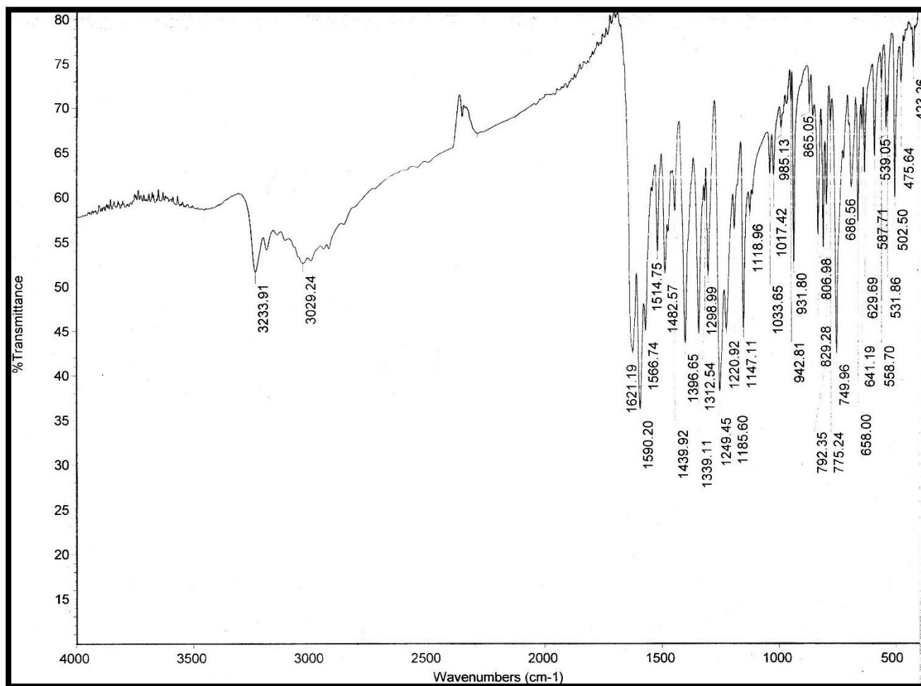
Figure 4. IR spectrum of compound 6
