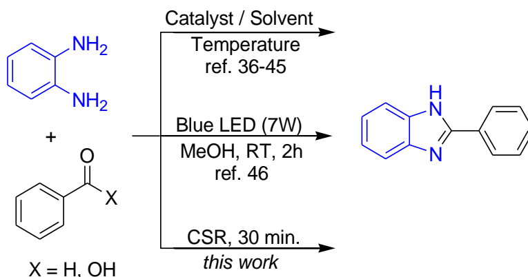
Scheme 1. Synthesis of benzimidazoles.
