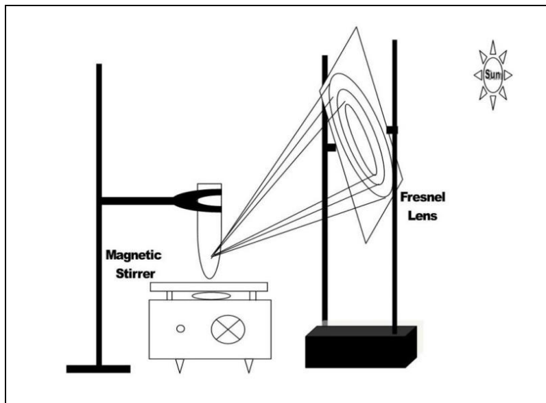
Figure 2: Schematic representation of experimental CSR Photochemical setup. a
