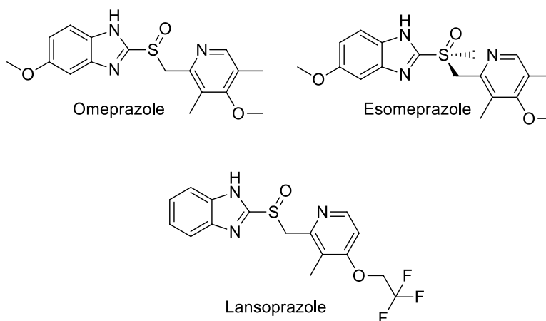
Figure 1. Some important benzimidazoles.
