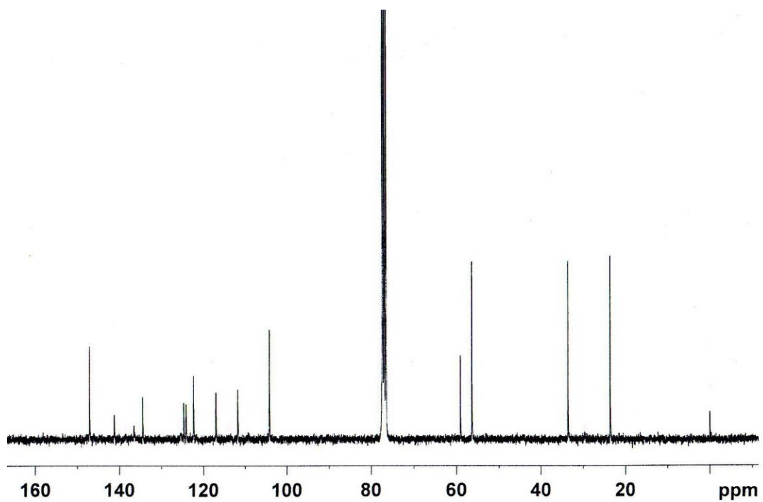
Figure S2. ^{13}\text{C} NMR spectrum of compound a .
