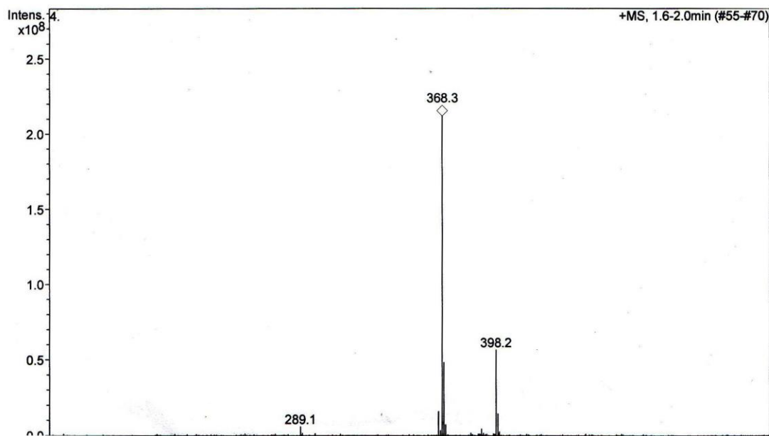
Figure S6. HPLC-ESI-MS spectrum of compound g.
