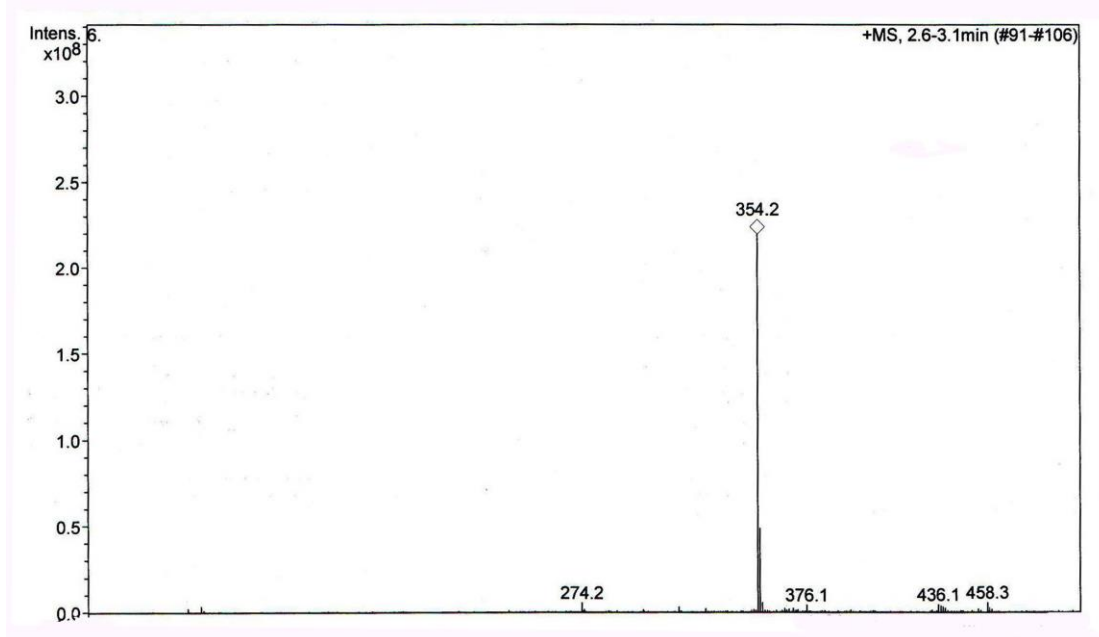
Figure S3. HPLC-ESI-MS spectrum of compound a.
