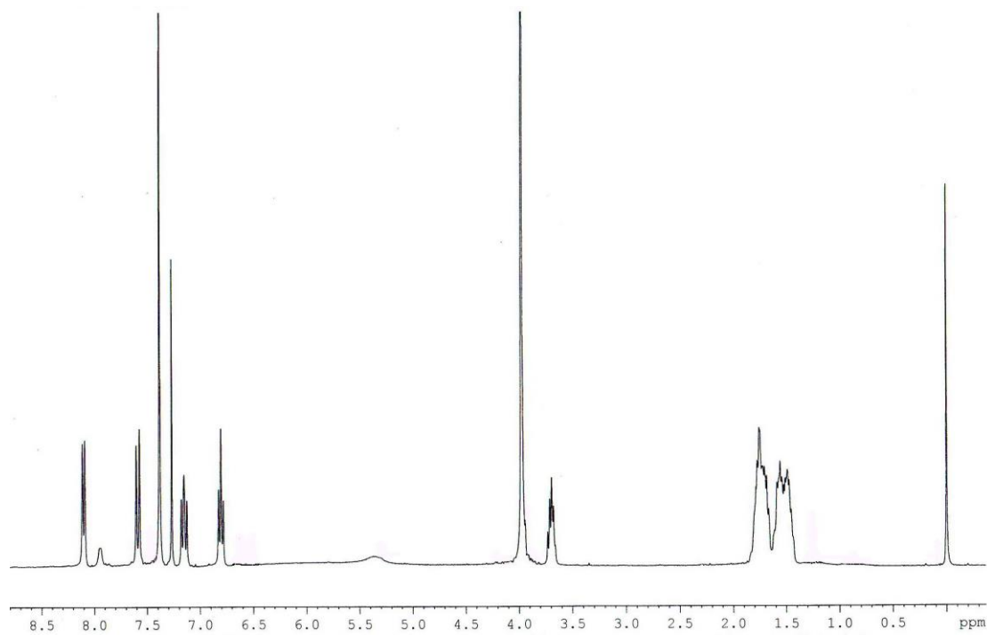
Figure S1. ^1\text{H} NMR spectrum of compound a .
