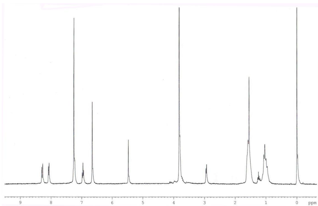
Figure S4. 1 H NMR spectrum of compound g.
