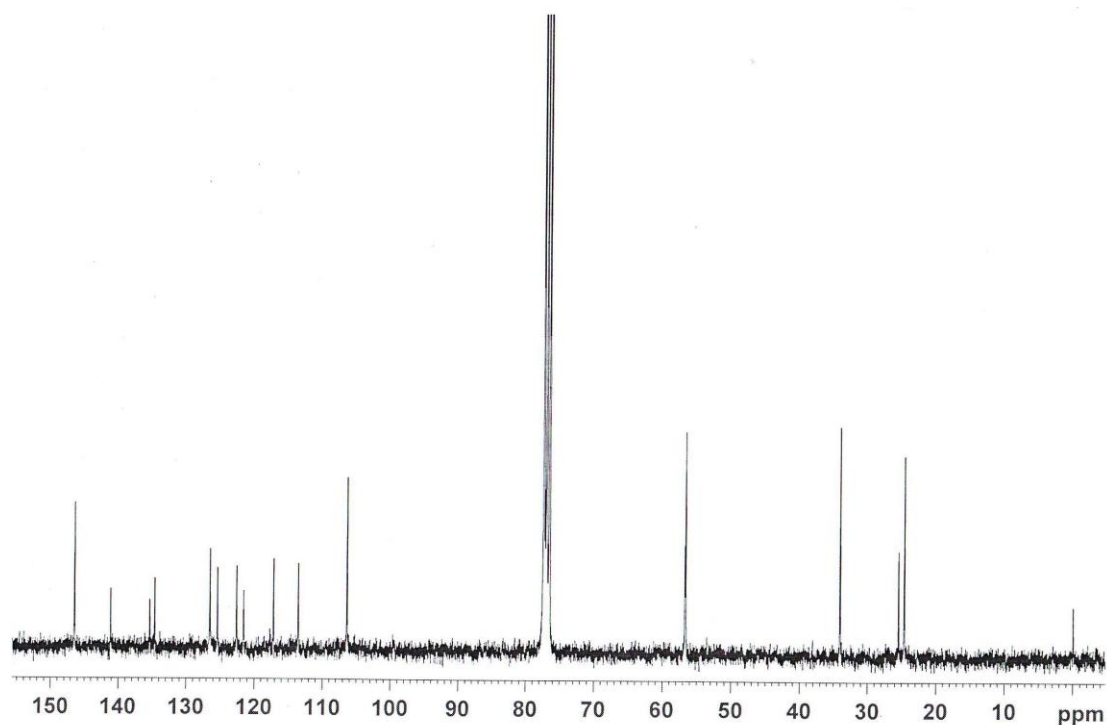
Figure S5. ^{13}\text{C} NMR spectrum of compound g.
