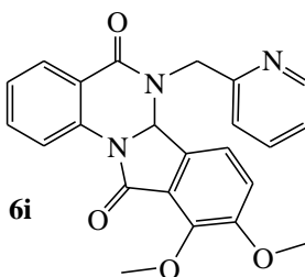
6,6a-Dihydro-9,10-dimethoxy-6-(pyridin-2-ylmethyl)isoindolo[2,1-a]quinazoline-5,11-dione (6i)
