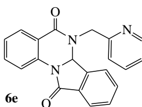
6,6a-Dihydro-6-(pyridin-2-ylmethyl)isoindolo[2,1-a]quinazoline-5,11-dione (6e)
