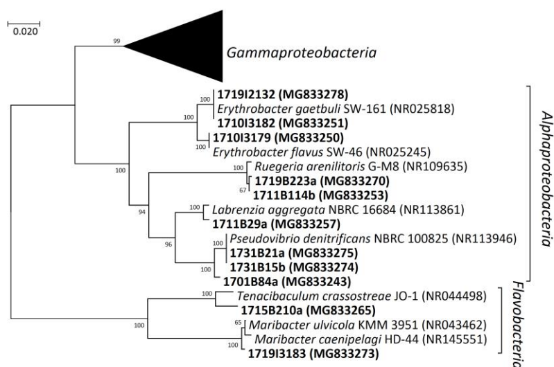
Figure 4. Neighbour-joining phylogenetic tree based on 16S rRNA gene sequences from Alphaproteobacteria and Flavobacteria strains isolated from Jaspis cf. coriacea and Jaspis splendens (in bold ), as well as reference type strains. Evolutionary distances were computed using the Maximum Composite Likelihood method, a total of 745 nucleotide positions were used. Bootstrap values are expressed as percentages of 1000 replicated; bootstrap values of \leq 50\% are not shown. Bar, 2 substitutions 100 base pairs.
