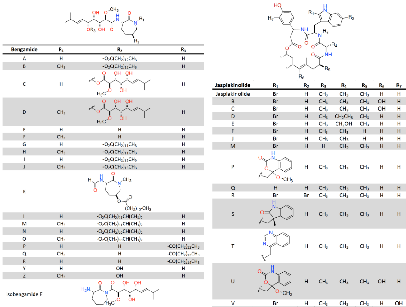
Scheme 1. Structures of bengamide and jasplakinolide analogues.
