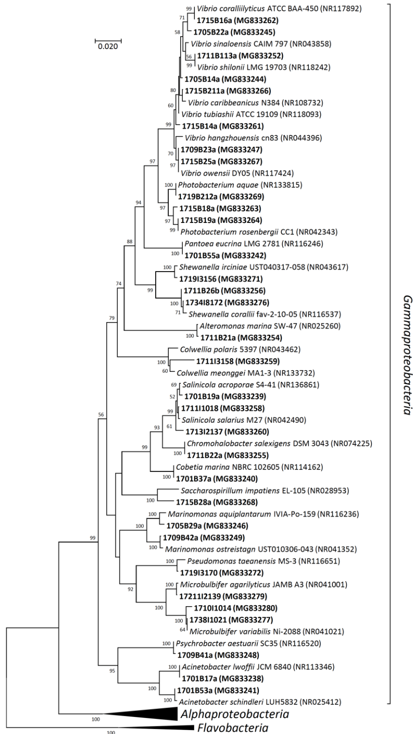
Figure 3. Neighbour-joining phylogenetic tree based on 16S rRNA gene sequences from Gammaproteobacteria strains isolated from Jaspis cf. coriacea and Jaspis splendens (in bold ), as well as reference type strains. Evolutionary distances were computed using the Maximum Composite Likelihood method, a total of 745 nucleotide positions were used. Bootstrap values are expressed as percentages of 1000 replicated; bootstrap values of \leq 50\% are not shown. Bar, 2 substitutions 100 base pairs.
