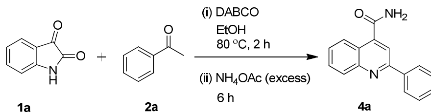
Scheme 3. One pot synthesis of 2-phenylquinoline-4-carboxamide ( 4a ).
