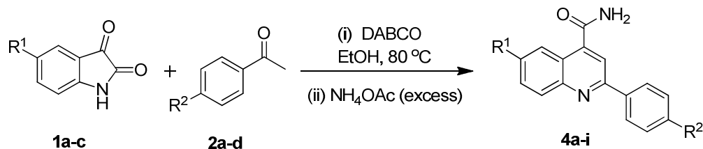
Scheme 4. Synthesis of 4-arylquinoline-4-carboxamides 4a-i .
