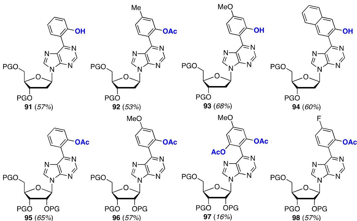
Figure 5. Oxidation of 6-aryl purine nucleosides with Pd(OAc) 2 and PIDA (PG = t -BuMe 2 Si).
