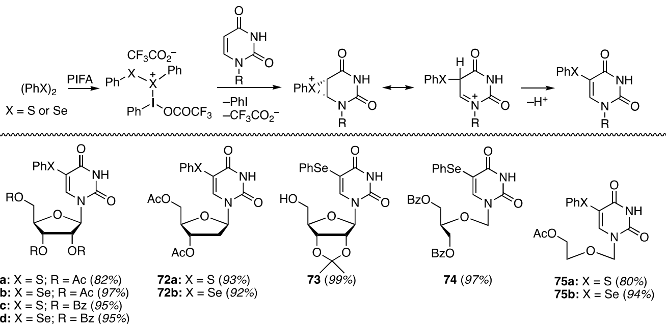
Scheme 18. Sulfenylation and selenation of uracil derivatives and uridine nucleosides, and analogues.
