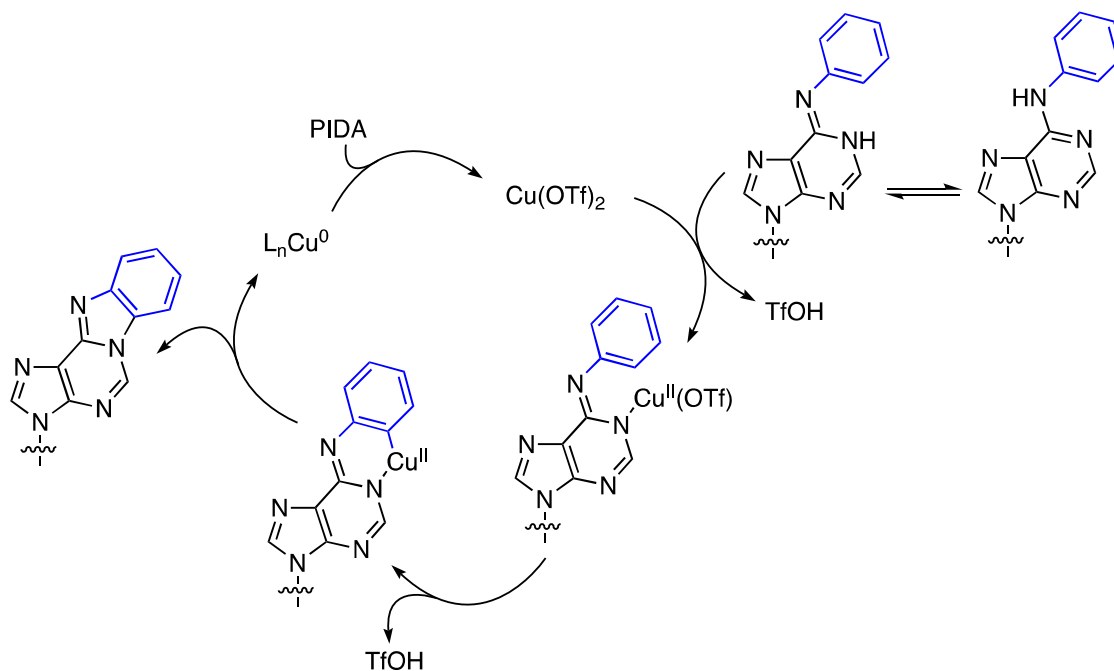
Scheme 24. A possible catalytic cycle for the \text{Cu}(\text{OTf})_2/\text{PIDA} -mediated cyclization
