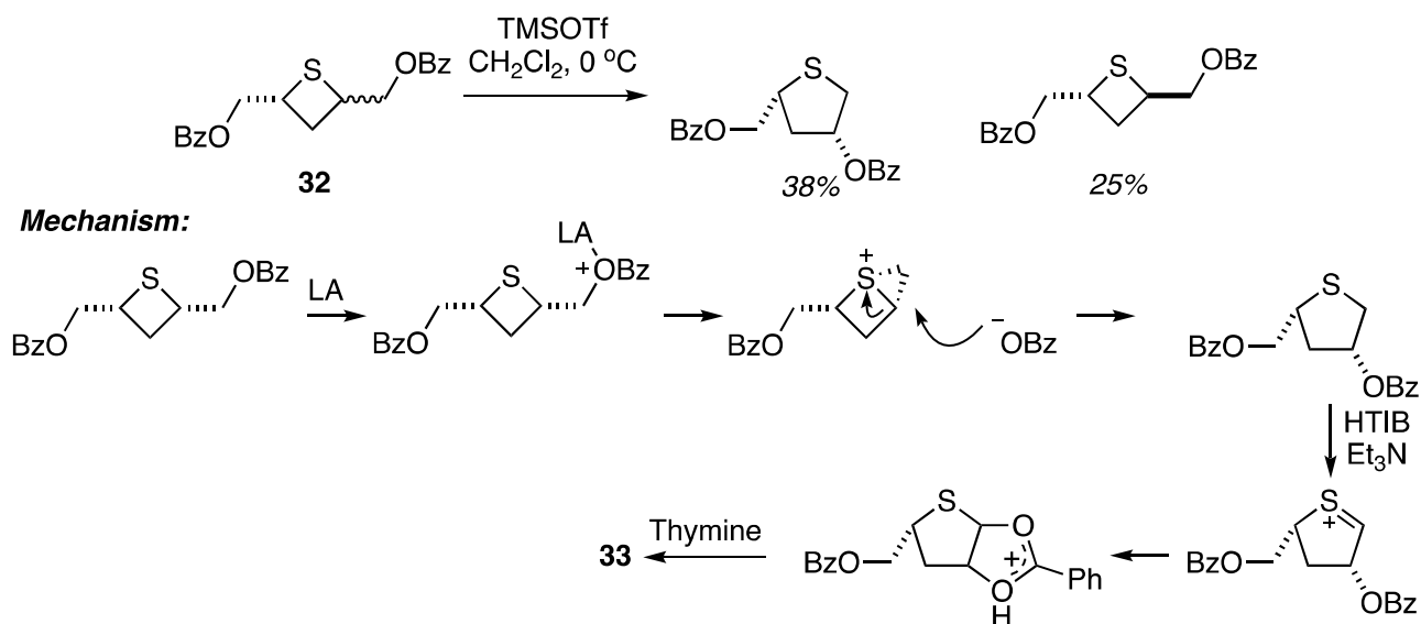
Scheme 7. Isomerization of cis - 32 and a mechanism for the formation of product 33 .
