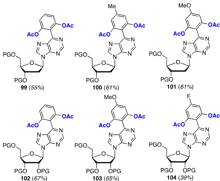
Figure 6. Diacetoxylation of 6-aryl purine nucleosides with Pd(OAc) 2 and PIDA (PG = t -BuMe 2 Si).
