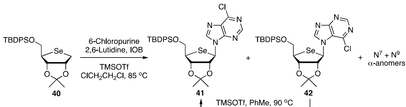
Scheme 9. Synthesis of the seleno analogue of 6-chloropurine riboside.
