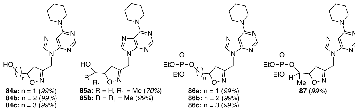
Figure 4. Examples of isoxazoline-substituted 6-pyrrolidinyl purine derivatives via PIFA oxidation.
