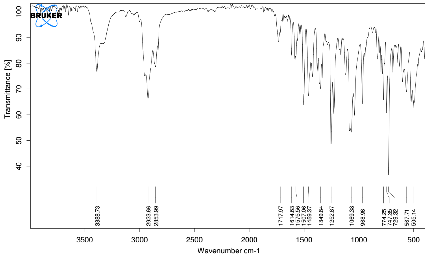
Figure S63. IR spectrum of compound 8u
