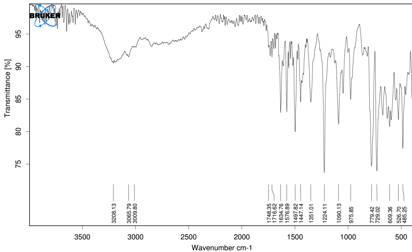
Figure S47. IR spectrum of compound 8q
