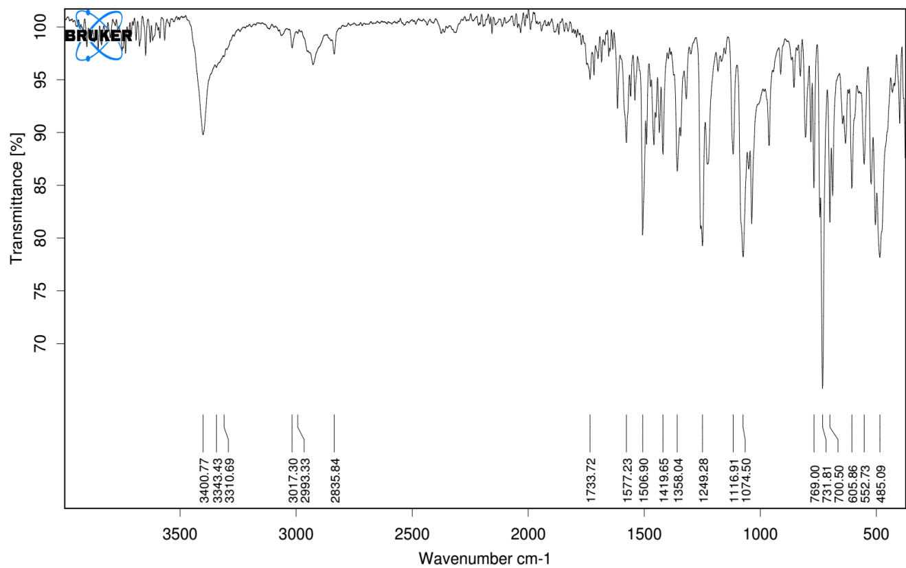
Figure S3. IR spectrum of compound 8a
