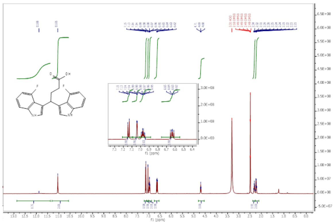
Figure S80. ^{13}\text{C} NMR spectrum of compound 8y
