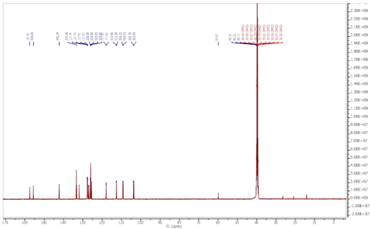
13 C NMR spectrum of compound 8j
