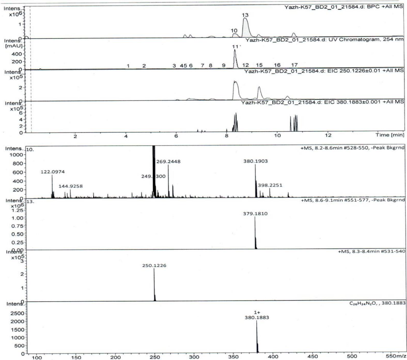
Figure S16. HRMS spectrum of compound 8g
