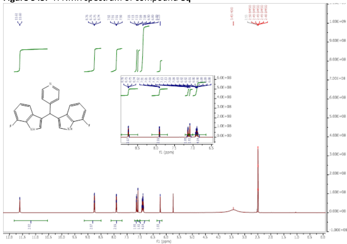
Figure S45. ^1\text{H} NMR spectrum of compound 8q
