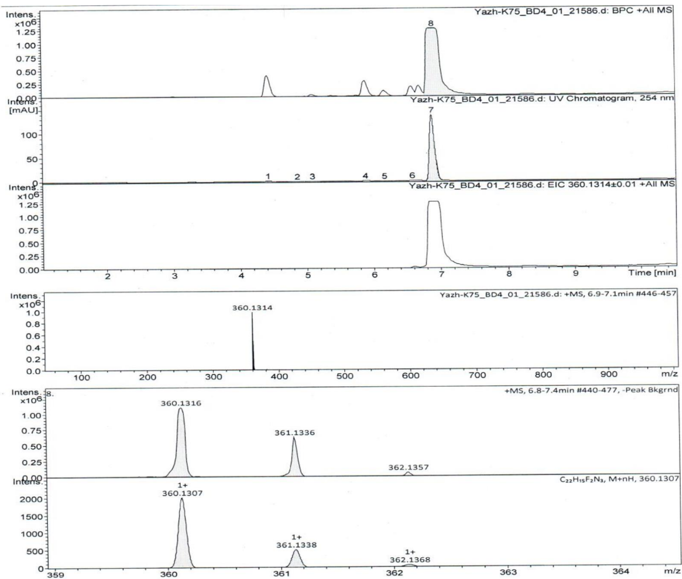
Figure S24. HRMS spectrum of compound 8i
