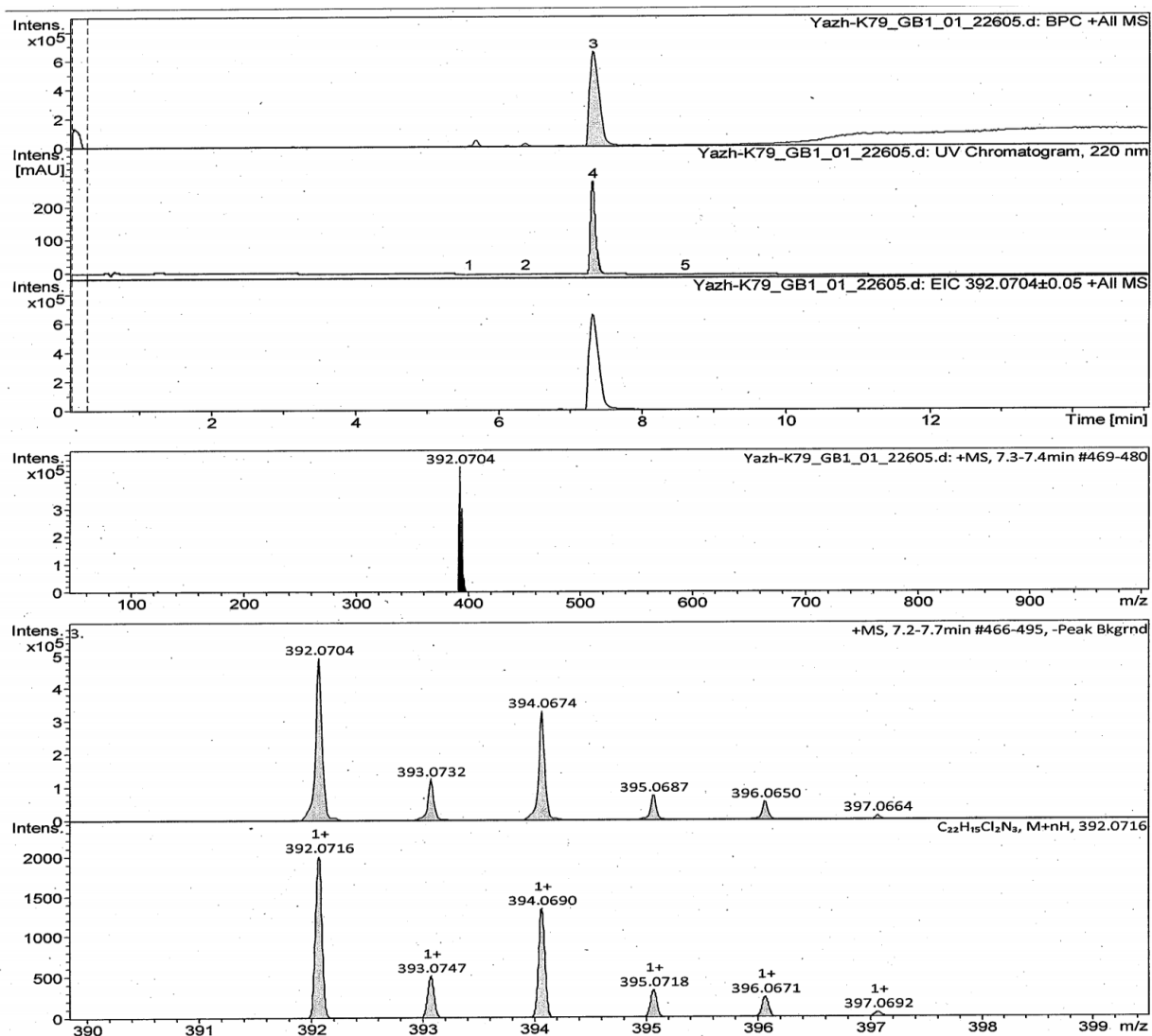
Figure S52. HRMS spectrum of compound 8r
