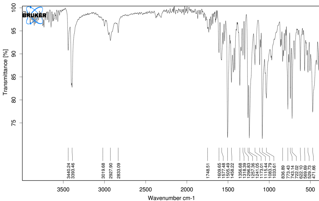
Figure S19. IR spectrum of compound 8h
