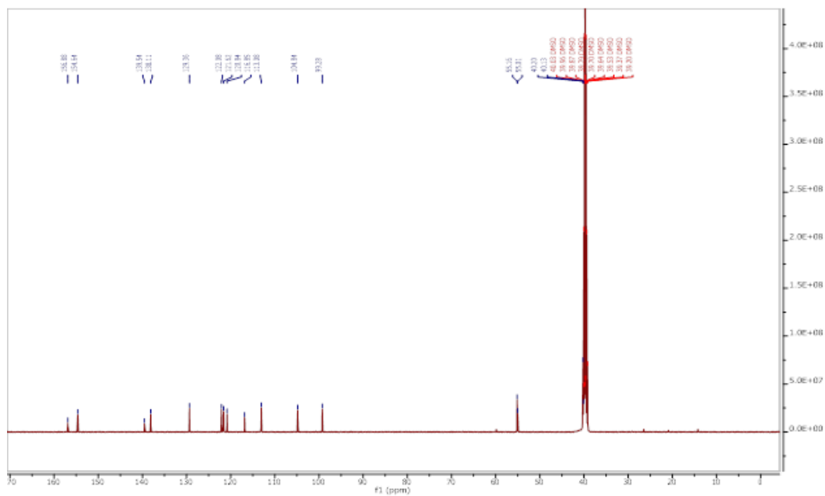
Figure S18. ^{13}\text{C} NMR spectrum of compound 8h
