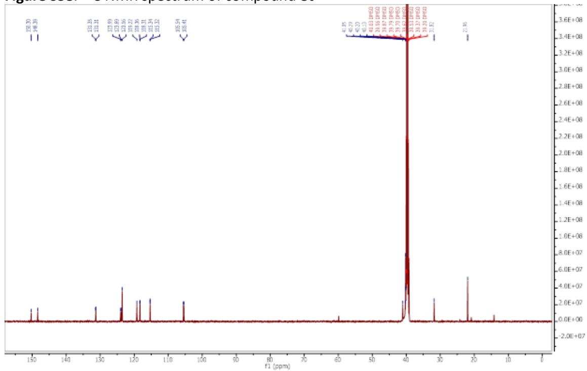
Figure S58. 13 C NMR spectrum of compound 8t
