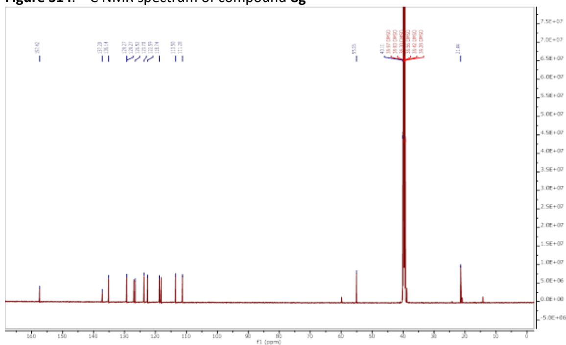
Figure S14. 13 C NMR spectrum of compound 8g
