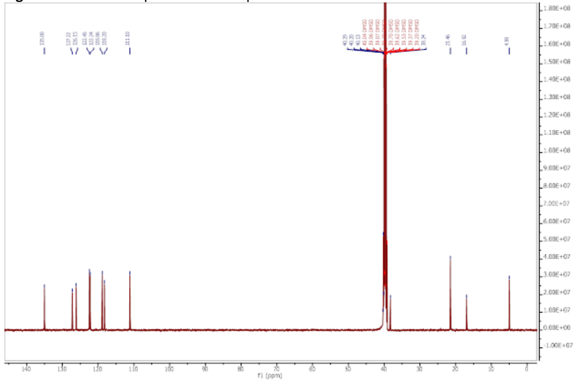
Figure S68. ^{13}\text{C} NMR spectrum of compound 8v
