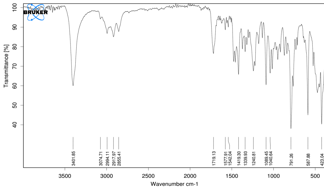
Figure S69. IR spectrum of compound 8v
