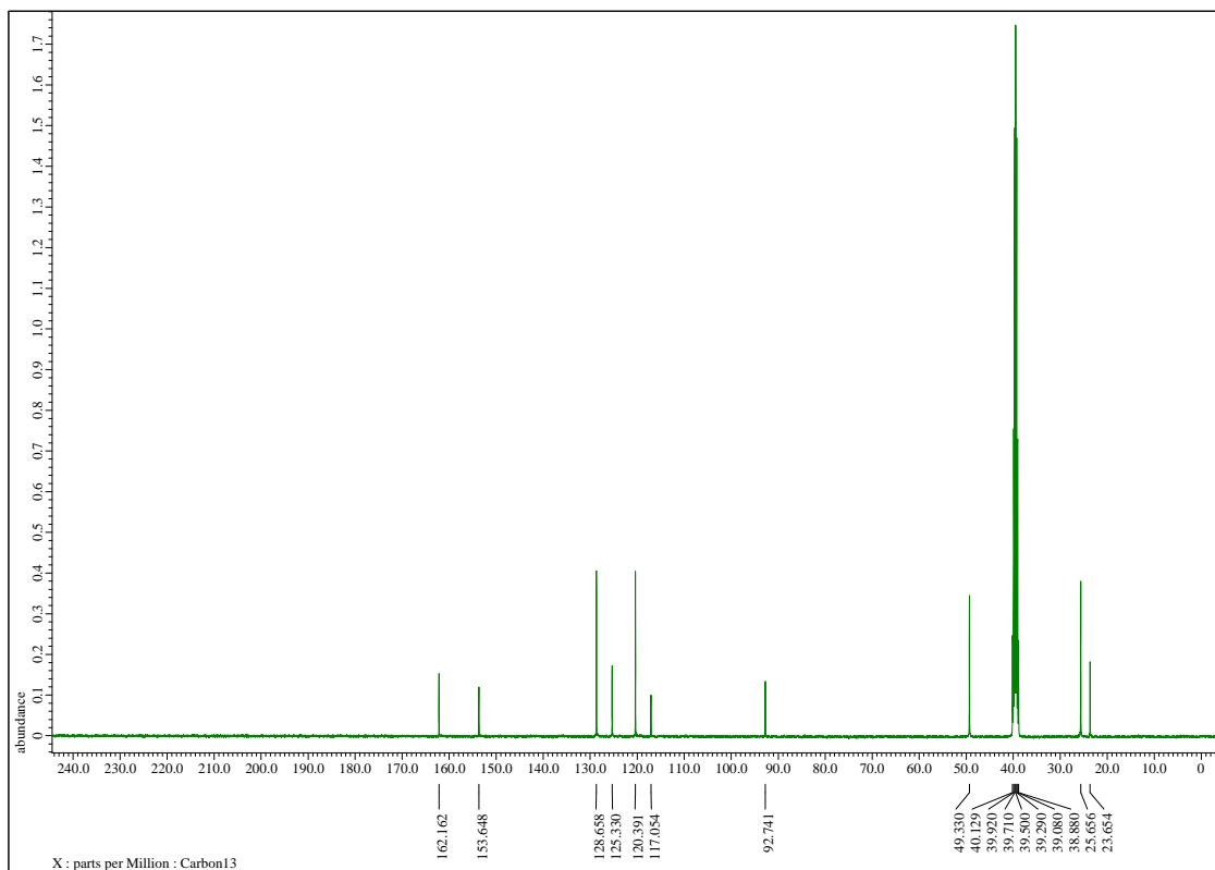
^1\text{H} and ^{13}\text{C} NMR spectra of compound 6g (DMSO- d_6 )
