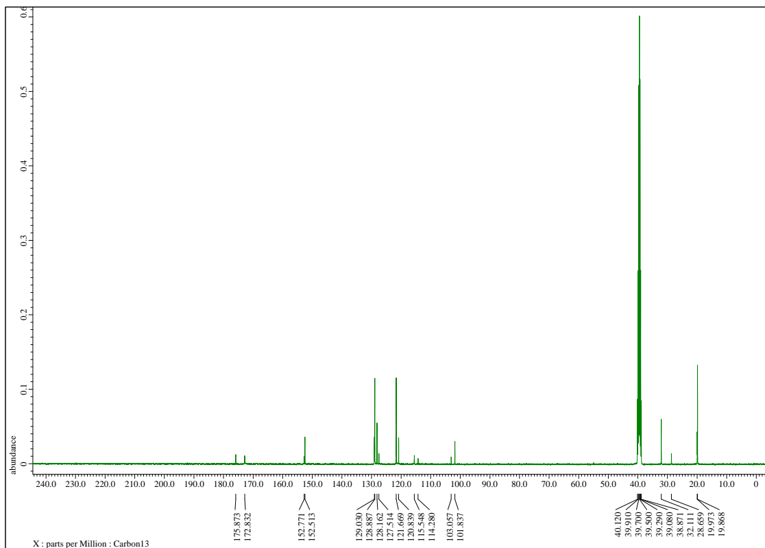
^1\text{H} and ^{13}\text{C} NMR spectra of compound 8k (CDCl 3 )
