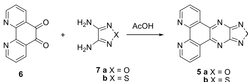
Scheme 1. Synthesis of [1,2,5]chalcogenadiazolo[3',4':5,6]pyrazino[2,3-f][1,10]phenanthrolines.
