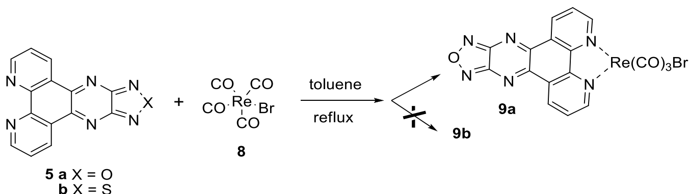
Scheme 2. Synthesis of \text{Re}(\text{I}) bromocarbonyl complexes.
