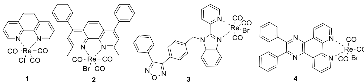
Figure 1. Some Re(I) halocarbonyl complexes with bidentate N,N -ligands.
