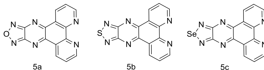
Figure 2. Some polycyclic ligands bearing chalcogenadiazole moiety.
