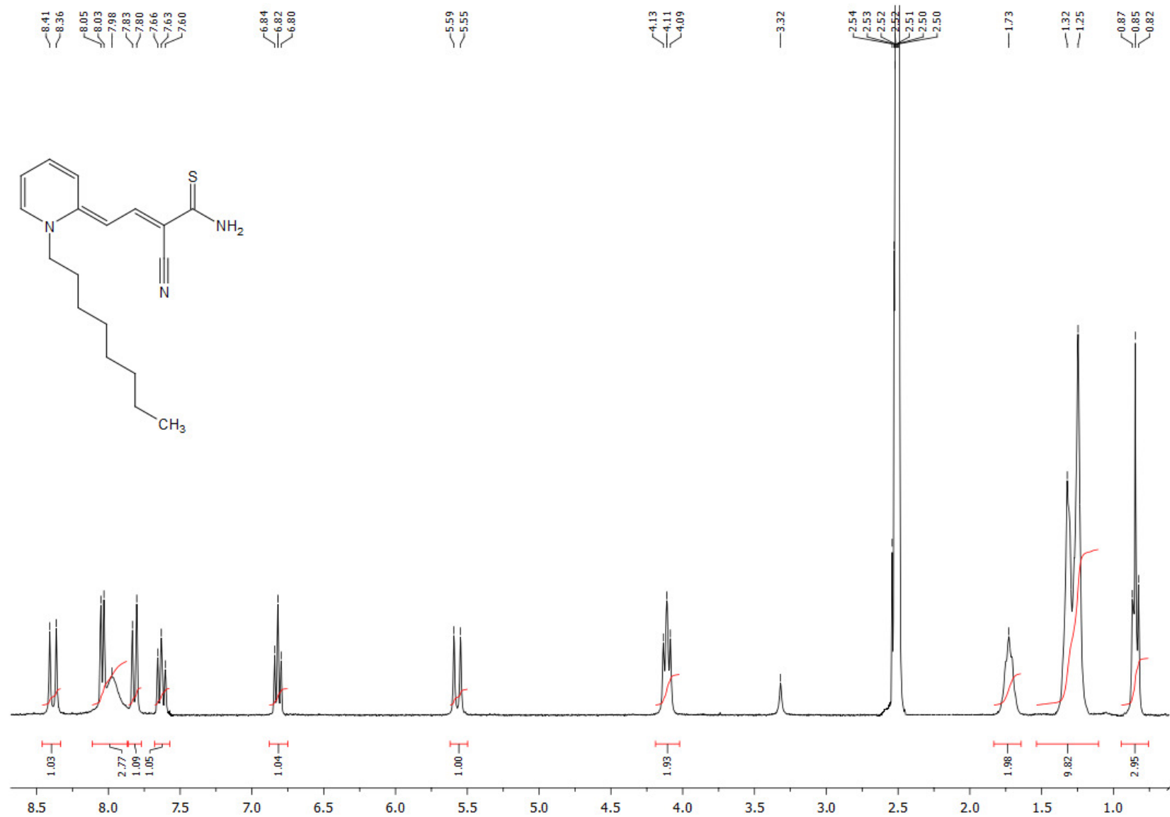
1 H NMR (300.1 MHz, DMSO- d 6 ) spectrum of (2E,4E)-4-(1'-octylpyridin-2'(1'H)-ylidene)-2-cyanobut-2-enethioamide 6i
