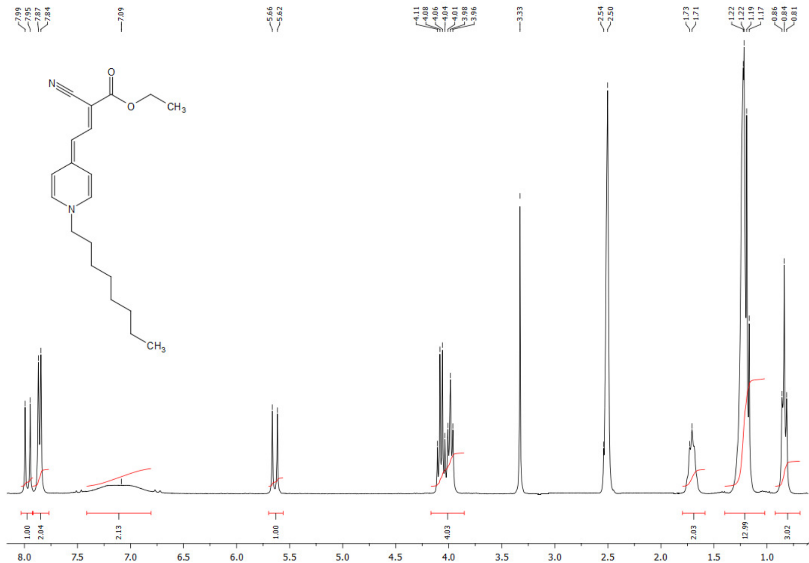
1 H NMR (300.1 MHz, DMSO- d 6 ) spectrum of ethyl (Z)-2-cyano-4-(1'-octylpyridin-4'(1'H)-ylidene)but-2-enoate 7h
