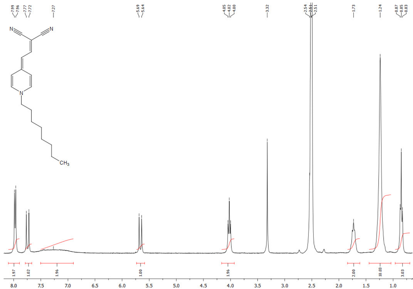
1 H NMR (300.1 MHz, DMSO- d 6 ) spectrum of 2-(2-(1'-octylpyridin-4'(1' H )-ylidene)ethylidene)malononitrile 7g
