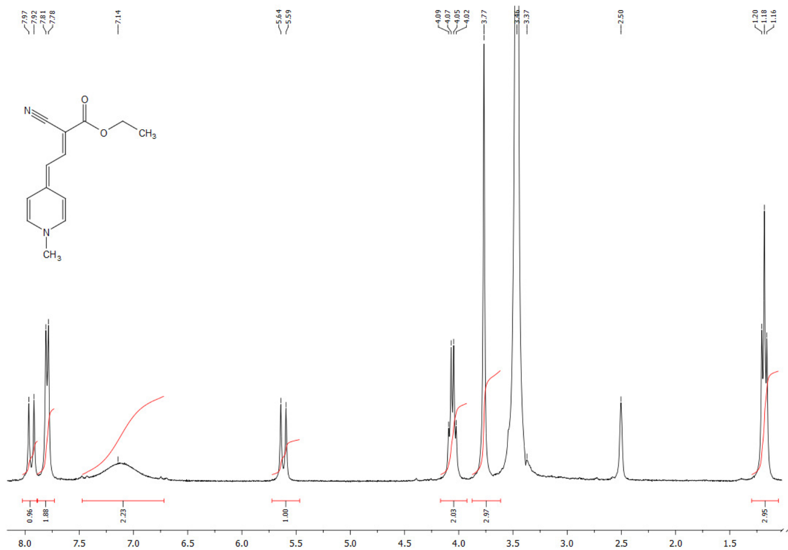
^1\text{H} NMR (300.1 MHz, \text{DMSO-}d_6 ) spectrum of ethyl (Z)-2-cyano-4-(1'-methylpyridin-4'(1'H)-ylidene)but-2-enoate 7b
