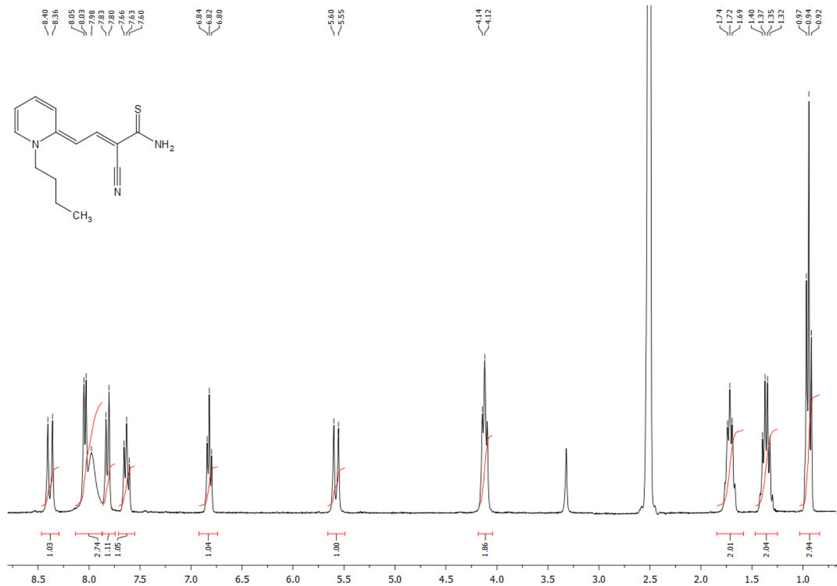
^1\text{H} NMR (300.1 MHz, \text{DMSO-}d_6 ) spectrum of (2E,4E)-4-(1'-butylpyridin-2'(1'H)-ylidene)-2-cyanobut-2-enethioamide 6f
