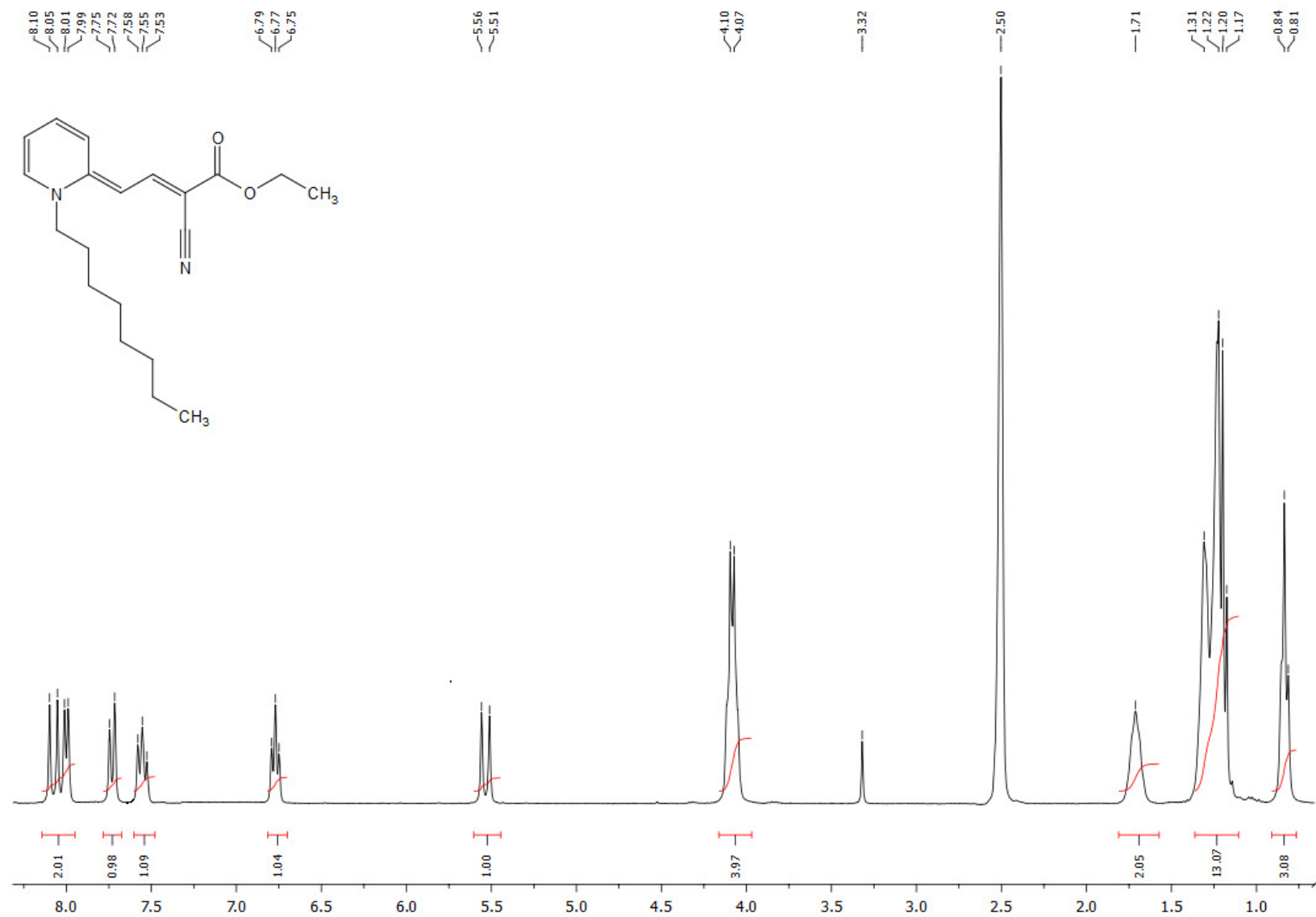
^1\text{H} NMR (300.1 MHz, \text{DMSO}-d_6 ) spectrum of ethyl (2E,4E)-2-cyano-4-(1'-octylpyridin-2'(1'H)-ylidene)but-2-enoate 6h
