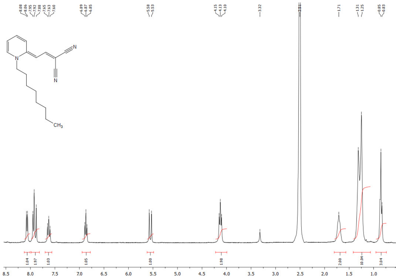
1 H NMR (300.1MHz, DMSO- d 6 ) spectrum of (E)-2-(2-(1'-octylpyridin-2'(1' H )-ylidene)ethylidene)malononitrile 6g
