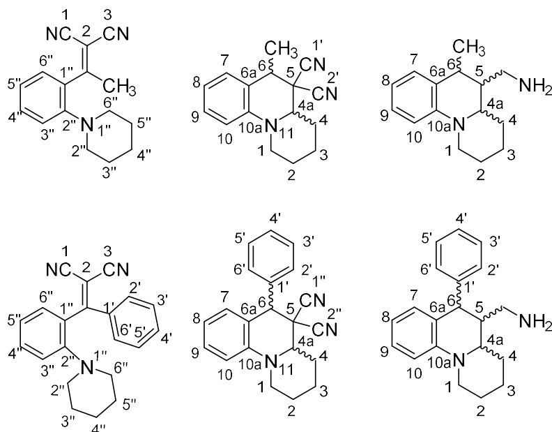
Scheme 5. The scheme of the atom numbering for NMR assignment.
