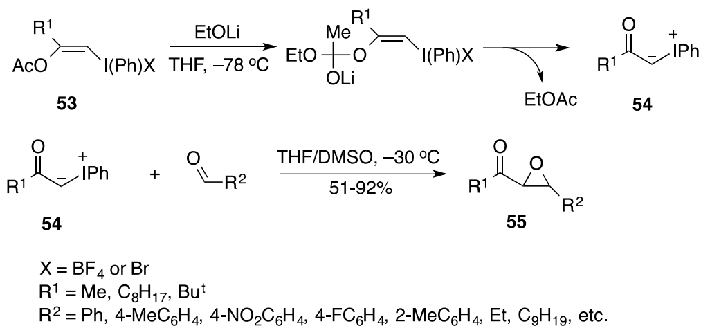
Scheme 17. Reactions of monocarbonyl iodonium ylides 54 with aldehydes.
