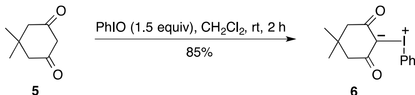
Scheme 2. Synthesis of dimedone-derived iodonium ylide 6 .
