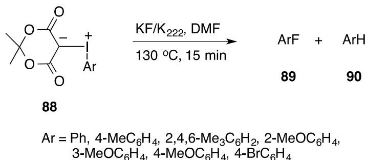
Scheme 31. Reaction of iodonium ylides with fluoride anion in DMF.
