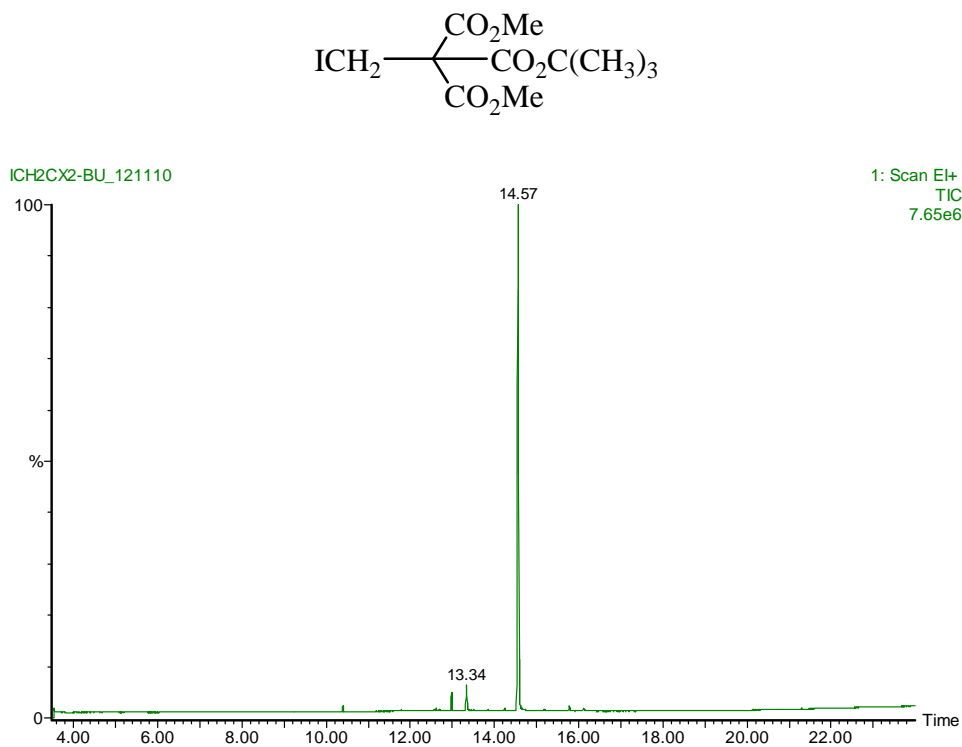
Figure S30. GC chromatogram.
