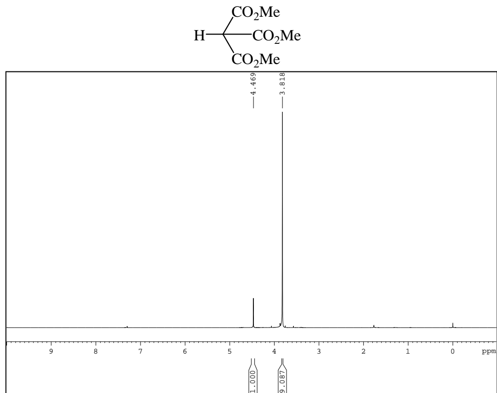
Figure S1. 1 H NMR spectrum.
