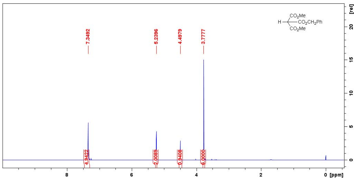
Figure S7. ^1\text{H} NMR spectrum.
