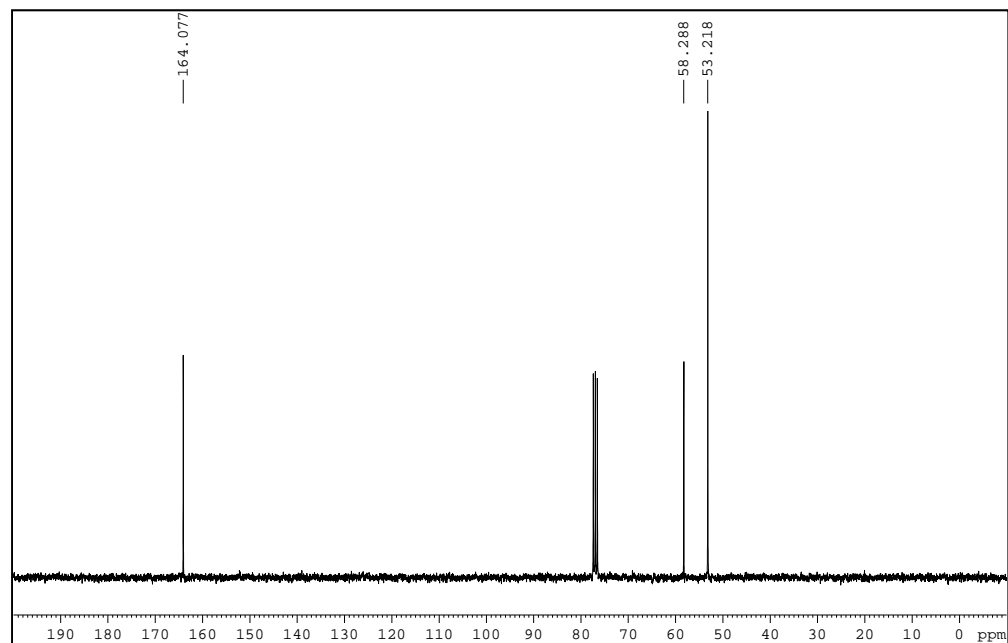
Figure S2. 13 C NMR spectrum.
