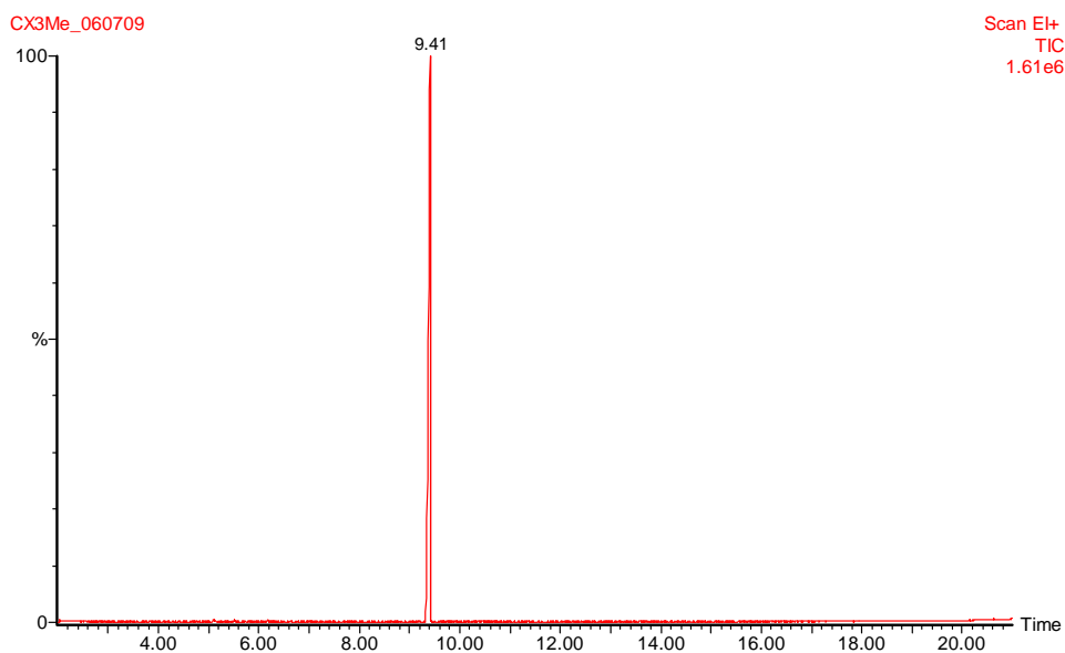
Figure S18. GC chromatogram.
