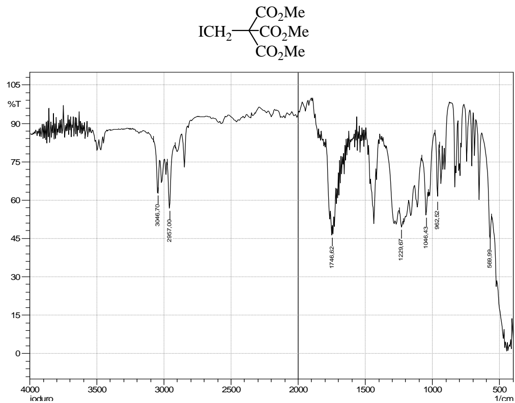
Figure S40. IR spectrum.
