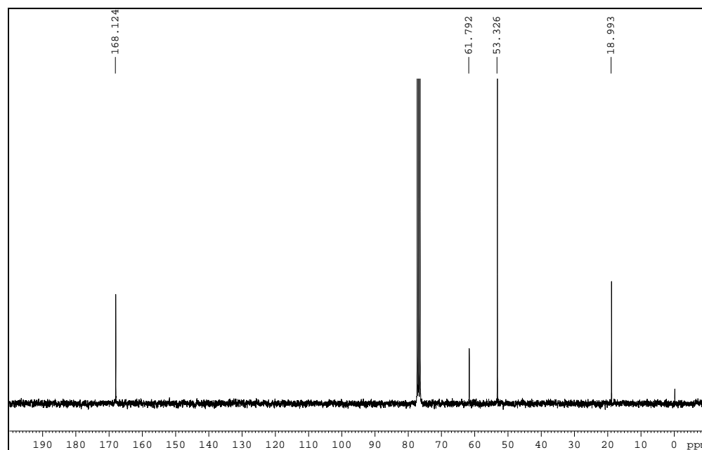
Figure S4. 13 C NMR spectrum.
