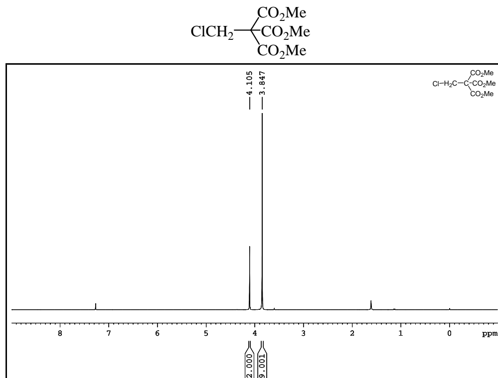
Figure S9. ^1\text{H} NMR spectrum.
