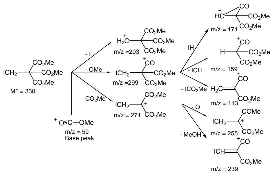
Figure S29. Proposed fragmentation pathway.
