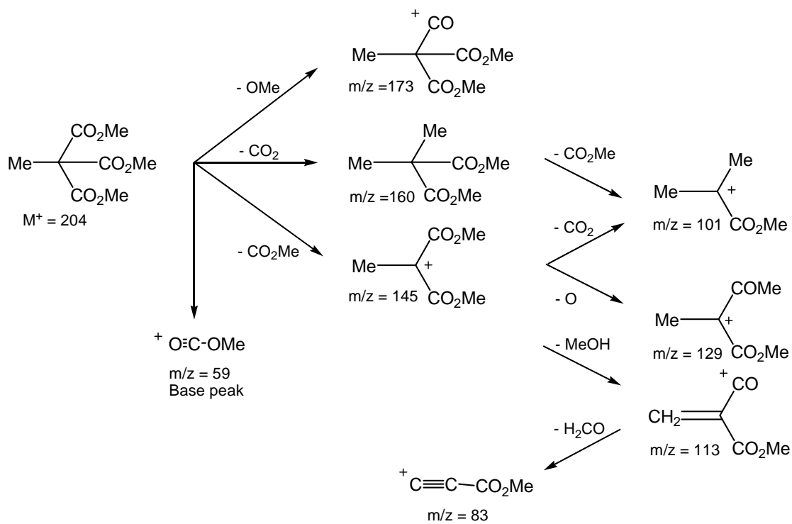
Figure S20. Proposed fragmentation pathway.
