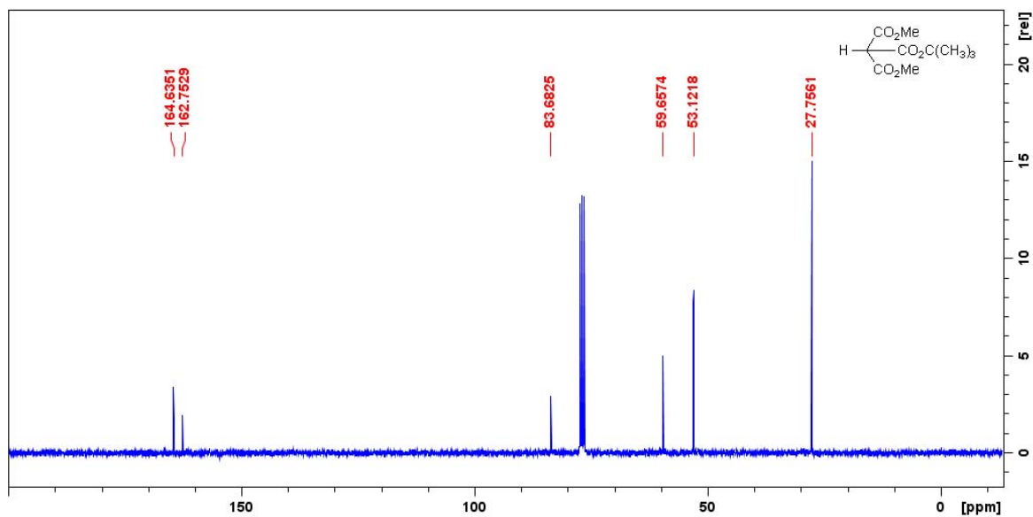
Figure S6. ^{13}\text{C} NMR spectrum.
