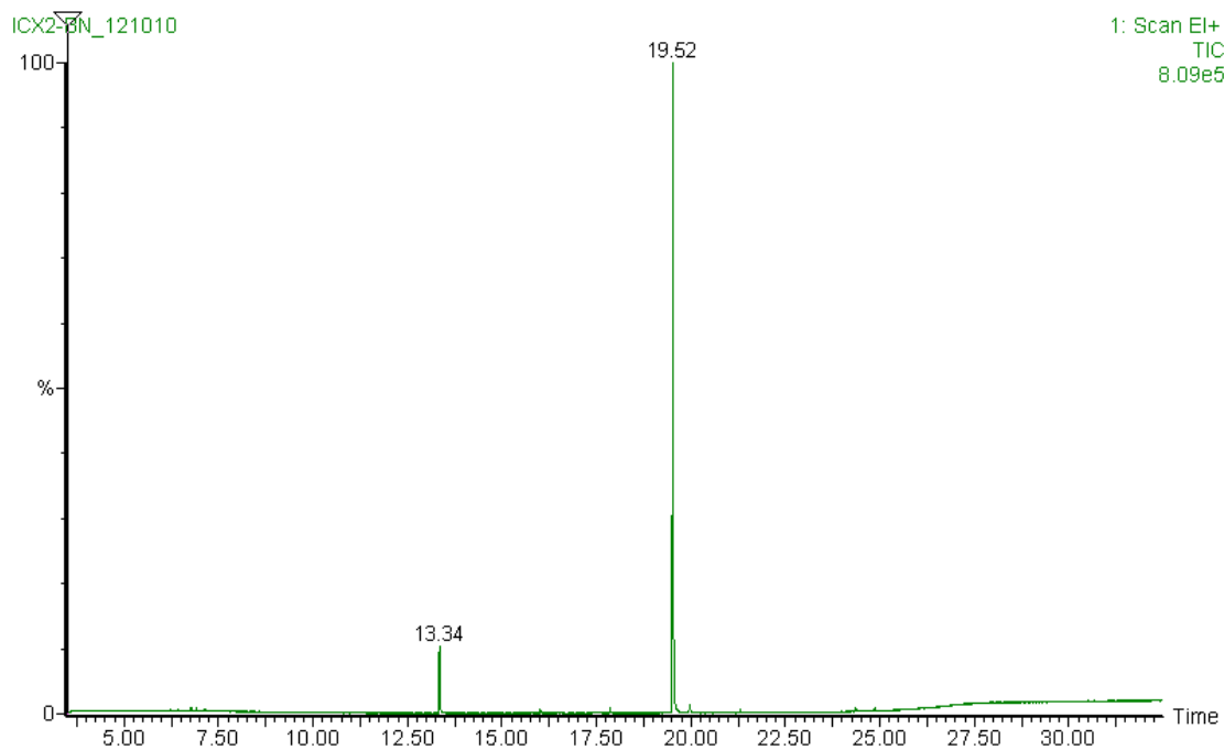
Figure S33. GC chromatogram.
