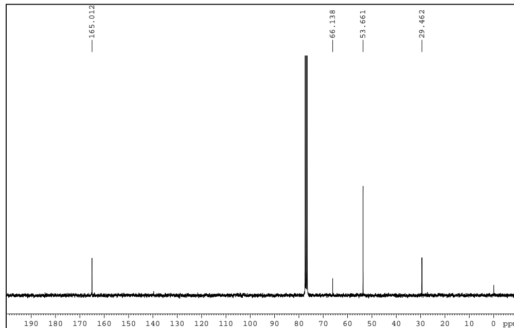
Figure S12. 13 C NMR spectrum.
