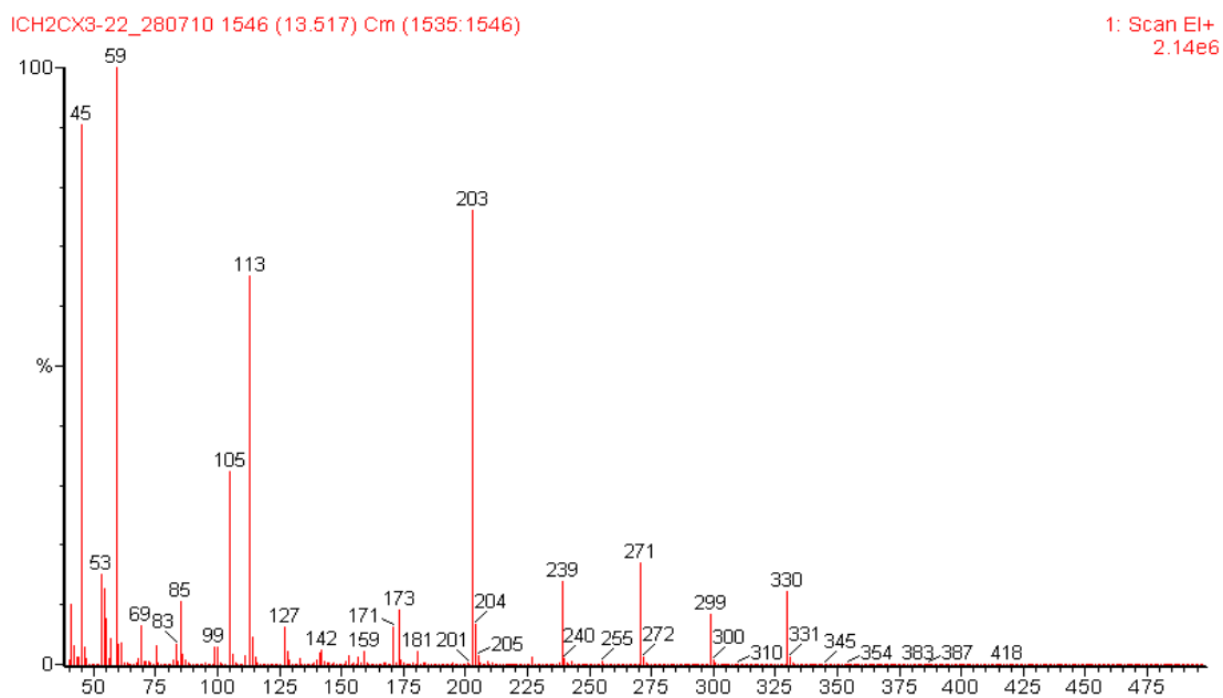
Figure S28. Mass spectrum rt 13.53 min.
