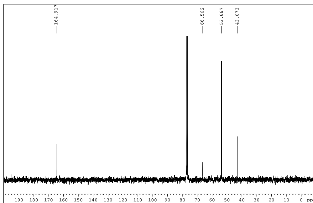
Figure S10. ^{13}\text{C} NMR spectrum.
