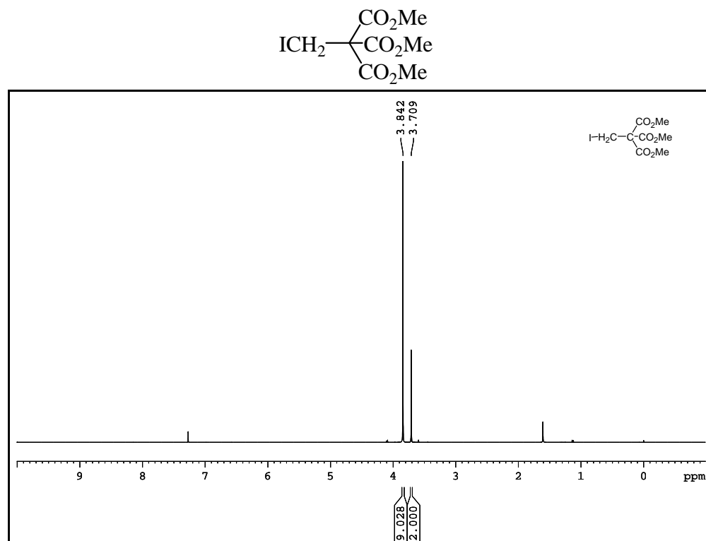
Figure S13. ^1\text{H} NMR spectrum.
