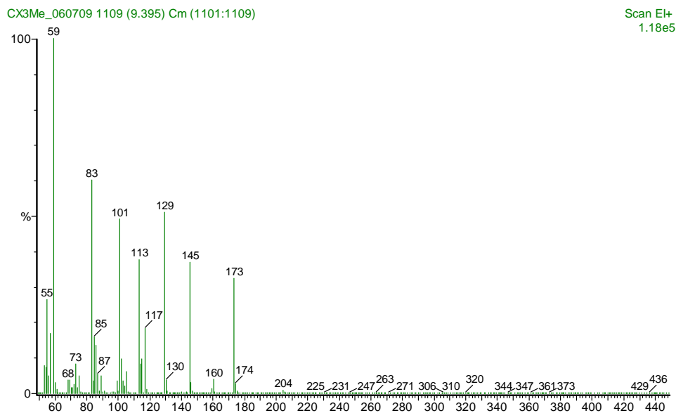
Figure S19. Mass spectrum rt 9.41 min.
