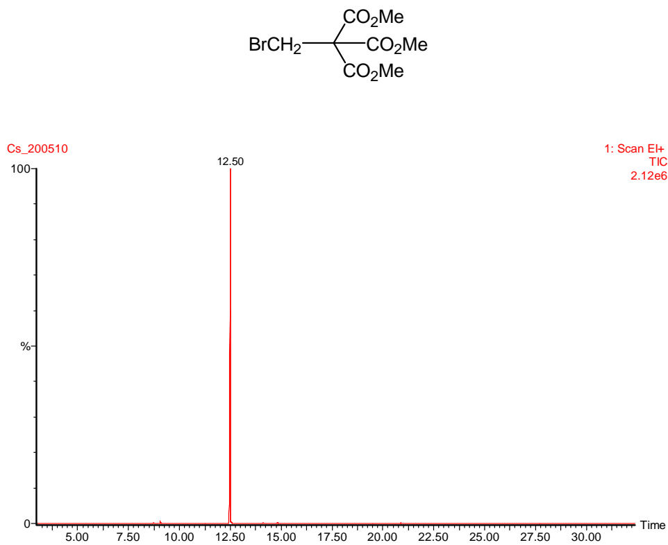
Figure S24. GC chromatogram.
