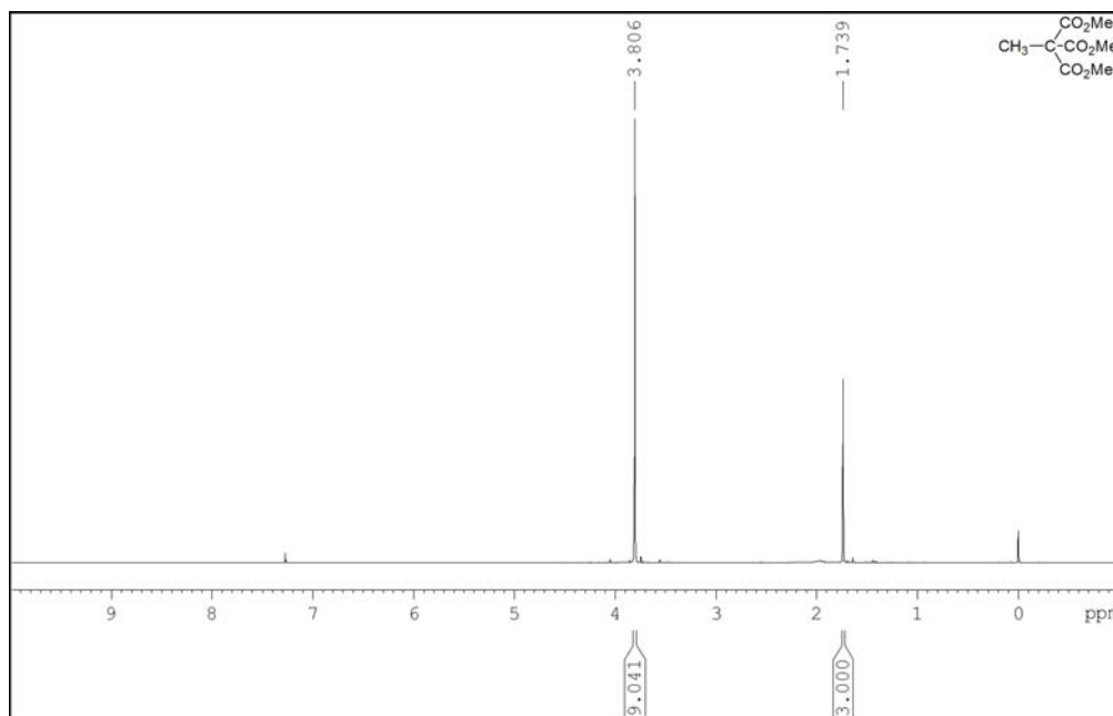
Figure S3. 1 H NMR spectrum.
