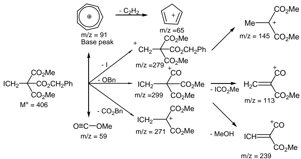
Figure S35. Proposed fragmentation pathway.
