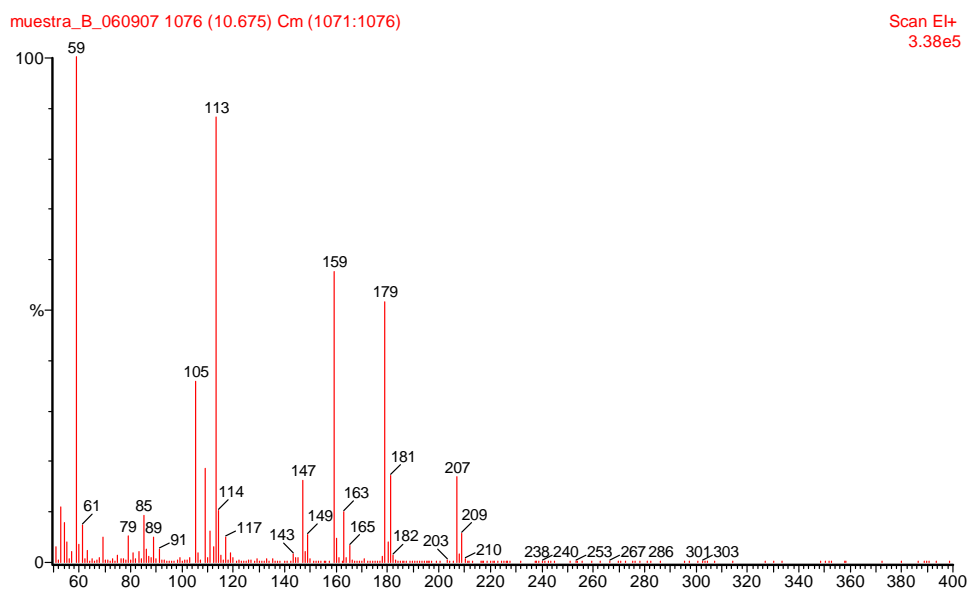
Figure S22. Mass spectrum rt 10.67 min.
