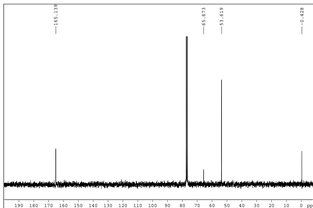
Figure S14. ^{13}\text{C} NMR spectrum.
