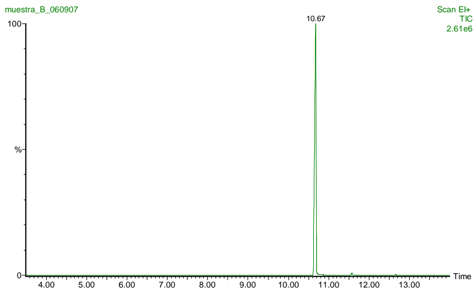
Figure S21. GC chromatogram.
