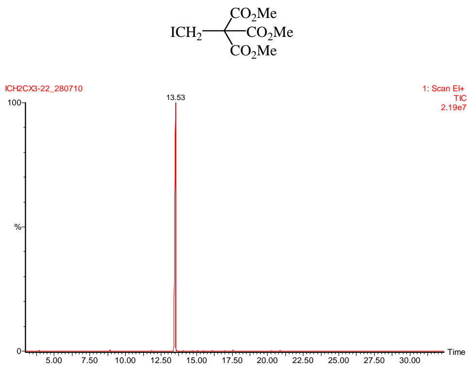
Figure S27. GC chromatogram.
