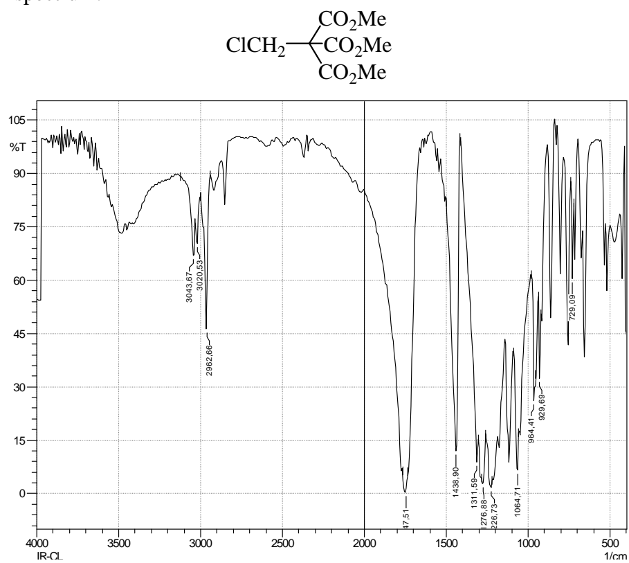
Figure S38. IR spectrum.
