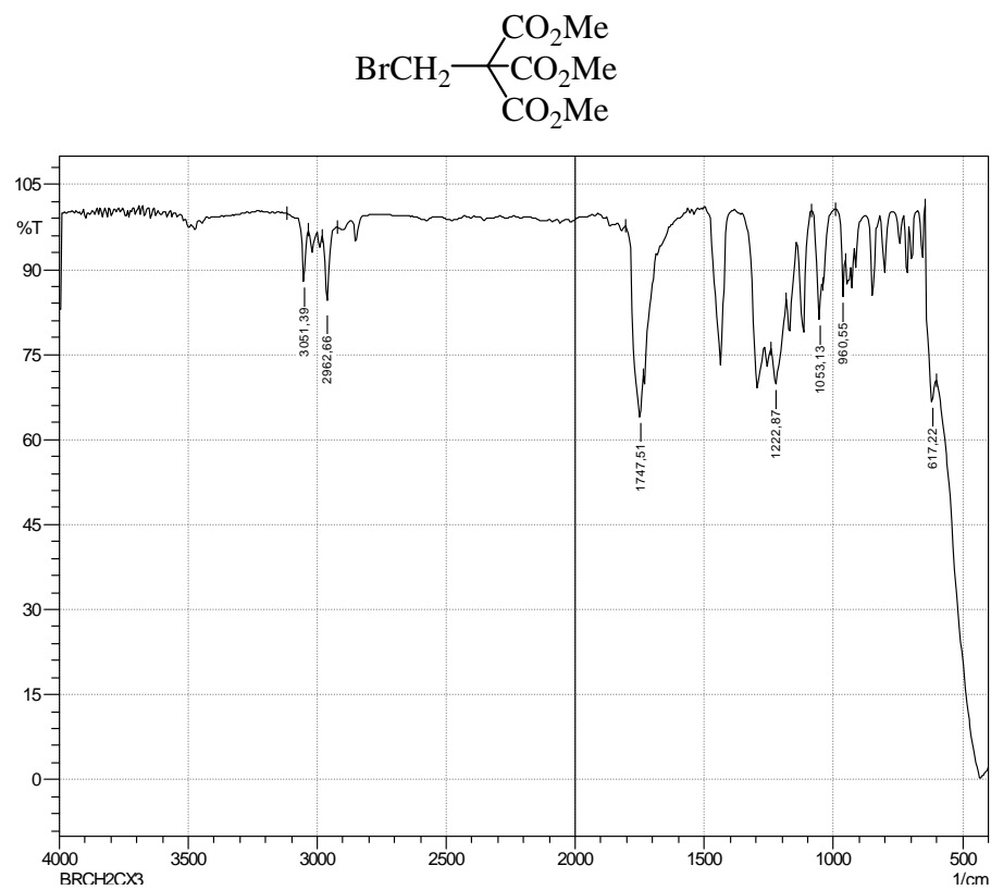
Figure S39. IR spectrum.
