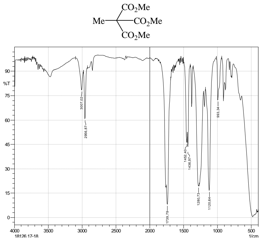
Figure S37. IR spectrum.
