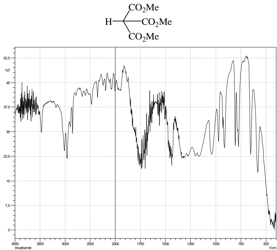
Figure S36. IR spectrum.
