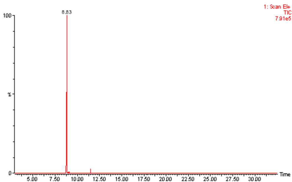
Figure S15. GC chromatogram.
