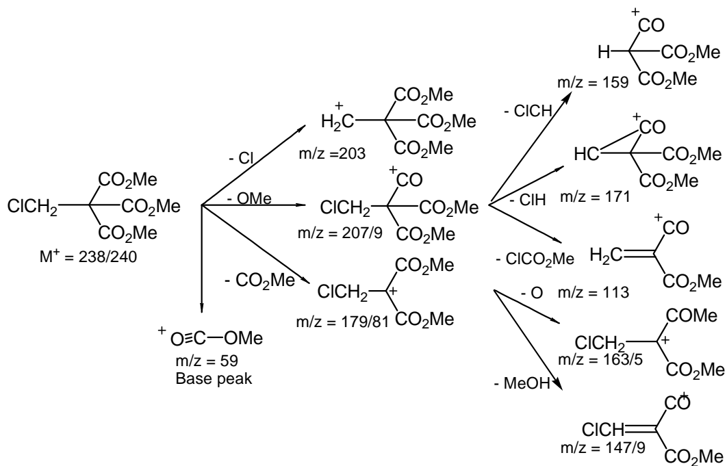
Figure S23. Proposed fragmentation pathway .
