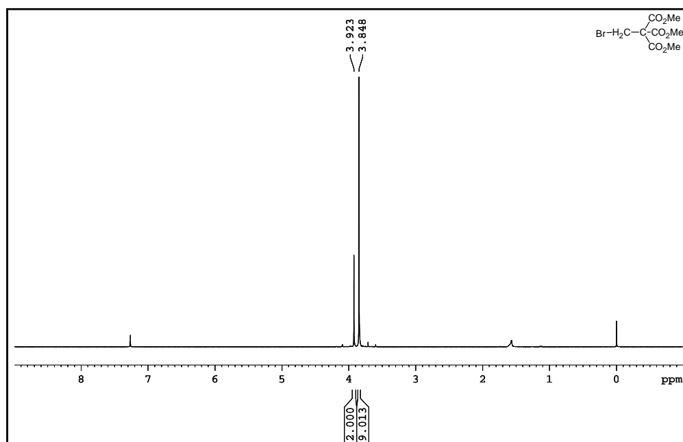
Figure S 11. 1 H NMR spectrum.
