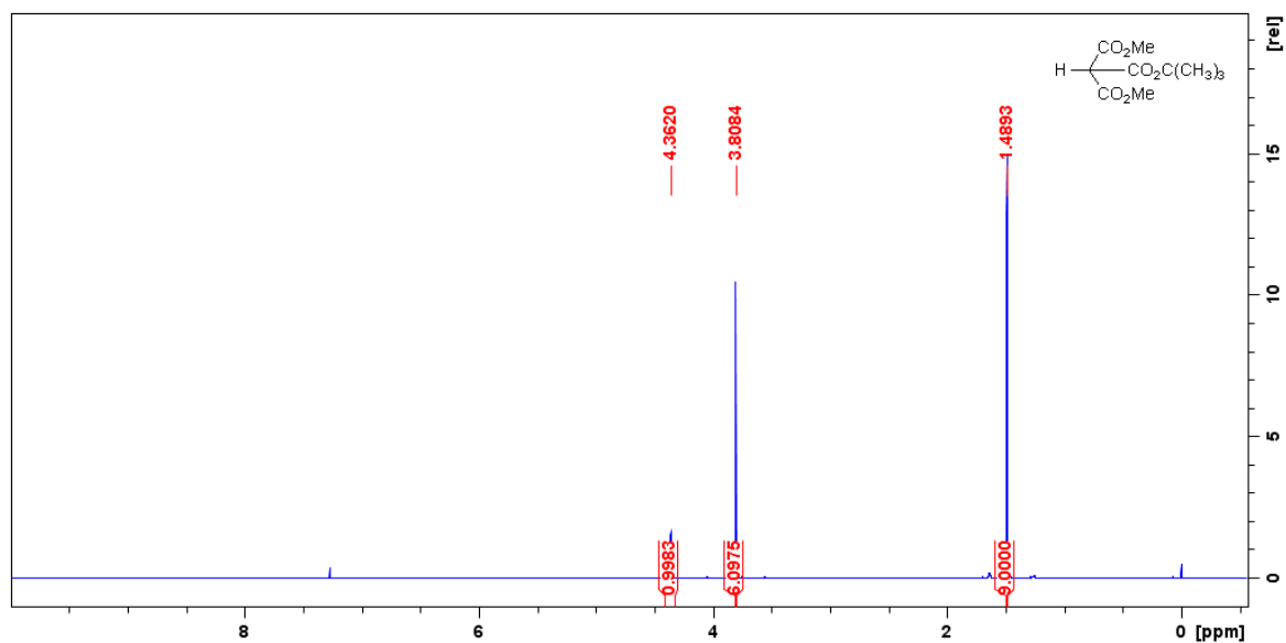
Figure S5. ^1\text{H} NMR spectrum.
