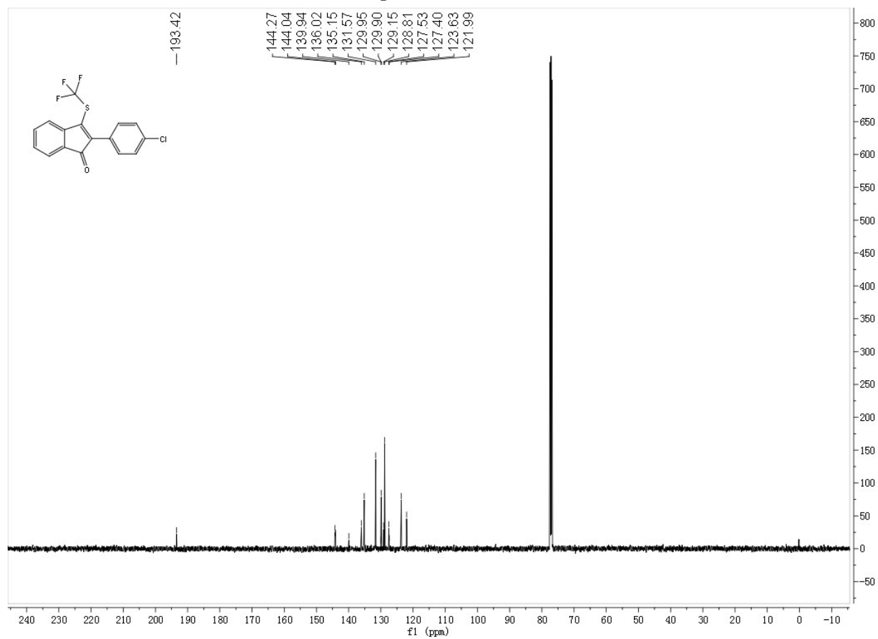
19 F NMR spectrum of 2b
