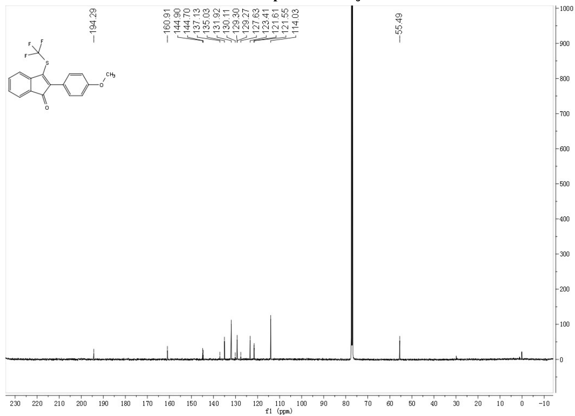
19 F NMR spectrum of 2j
