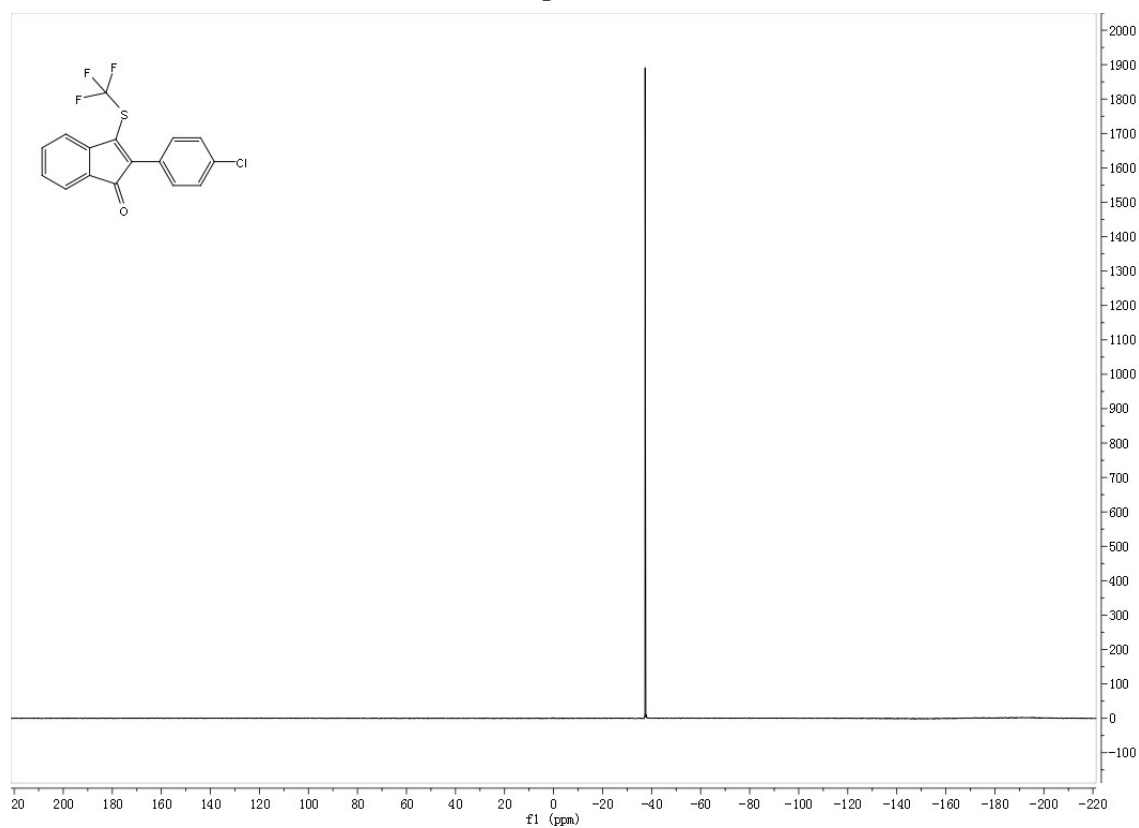
19 F NMR spectrum of 2b
