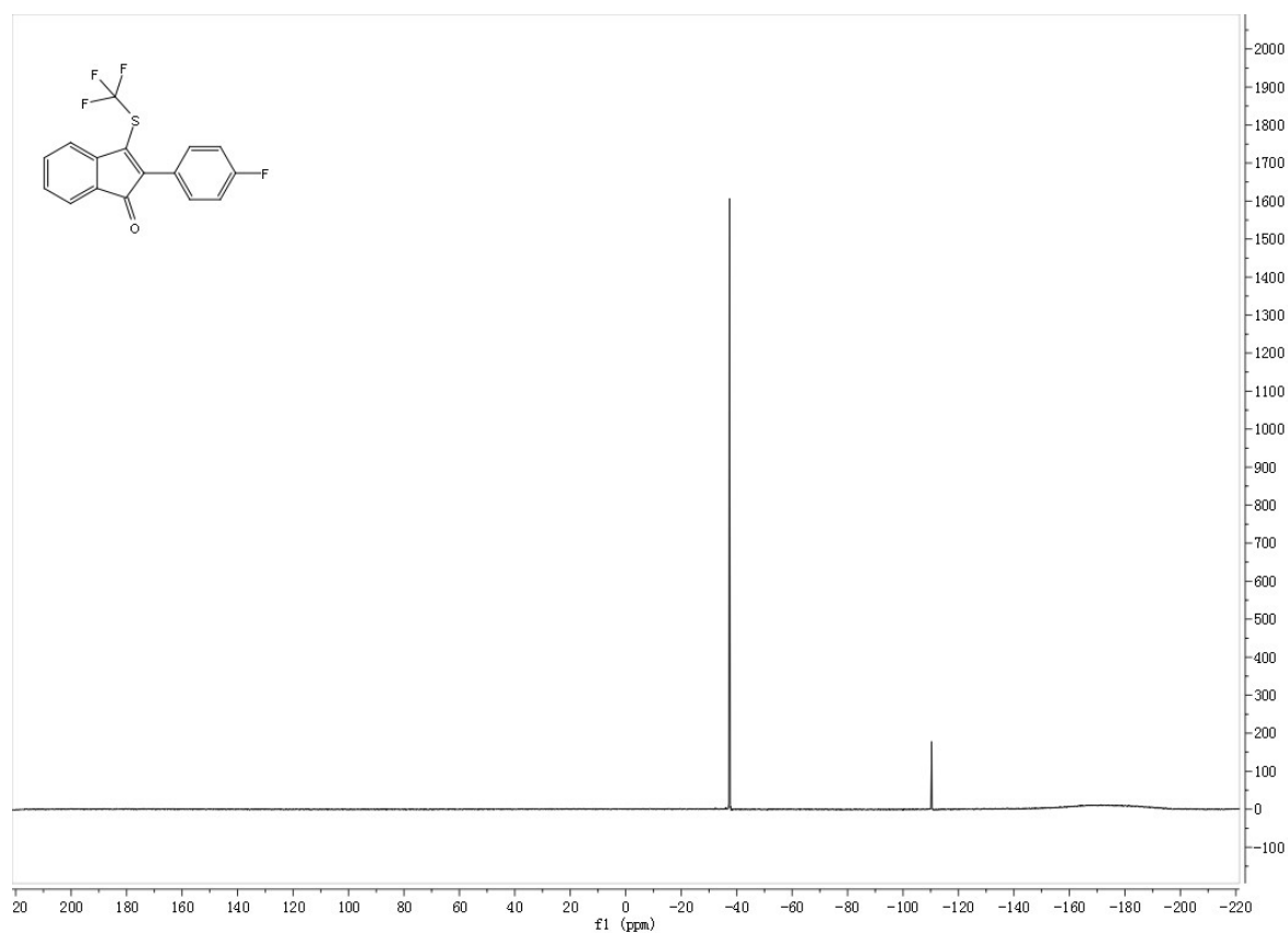
19 F NMR spectrum of 2d
