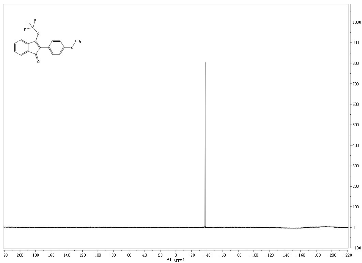
19 F NMR spectrum of 2j
