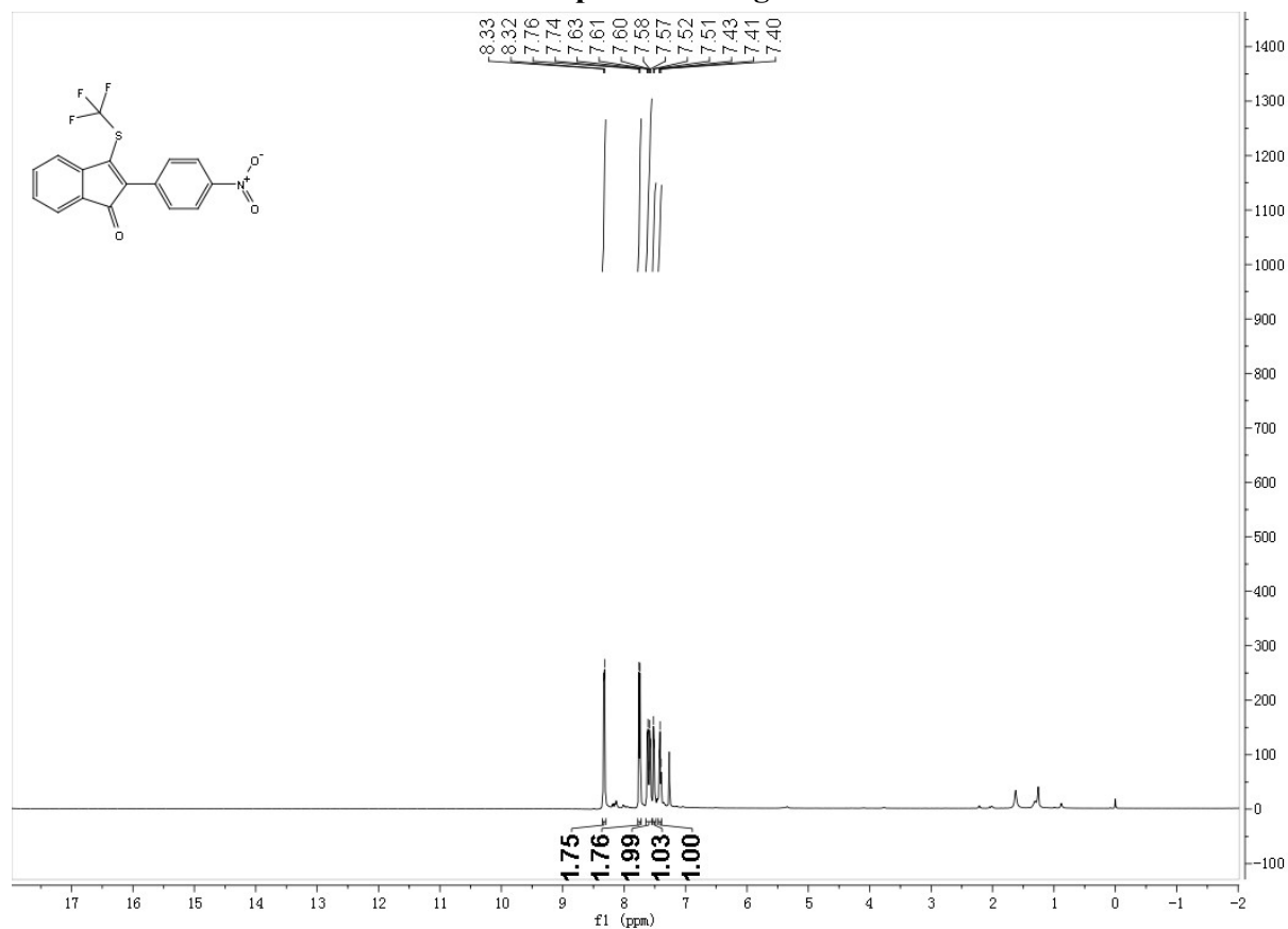
13 C NMR spectrum of 2g
