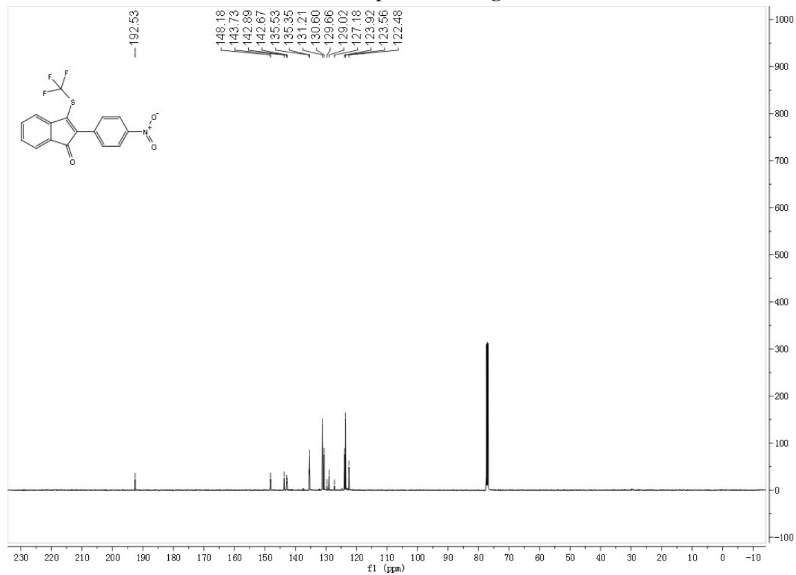
13 C NMR spectrum of 2g
