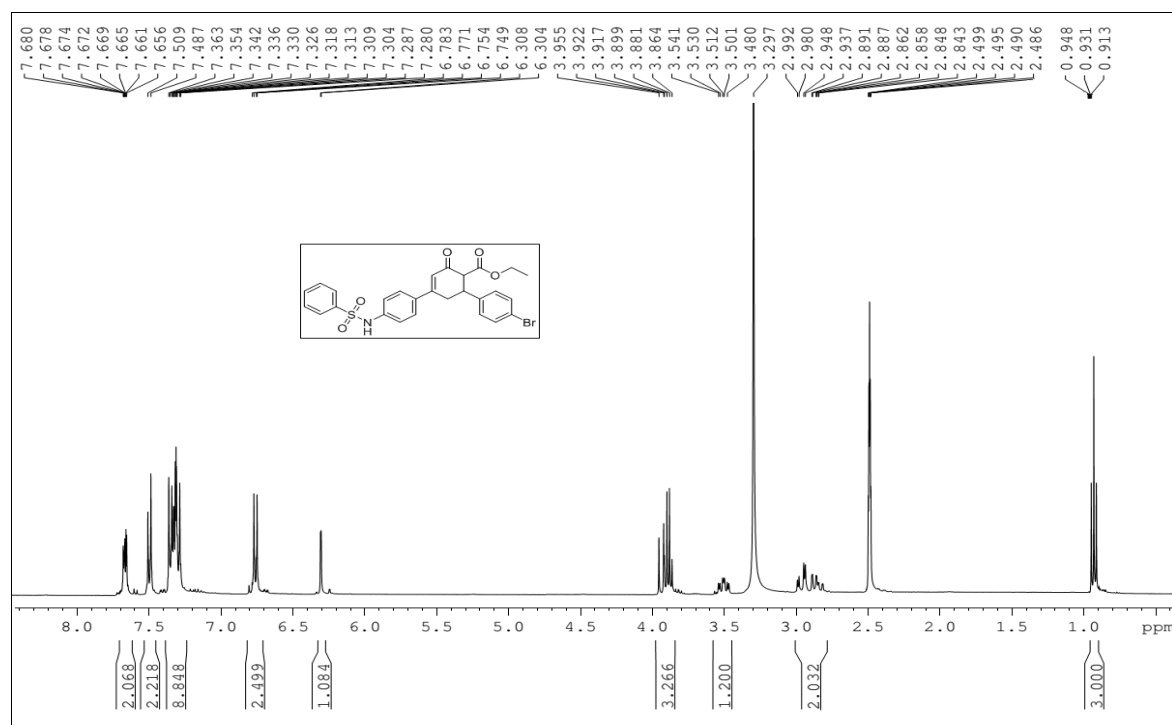
Fig. S43. 1 H spectrum of Ethyl 6-(4-bromophenyl)-2-oxo-4-((4-phenylsulfonamido)phenyl)-cyclohex-3-enecarboxylate (7d)
