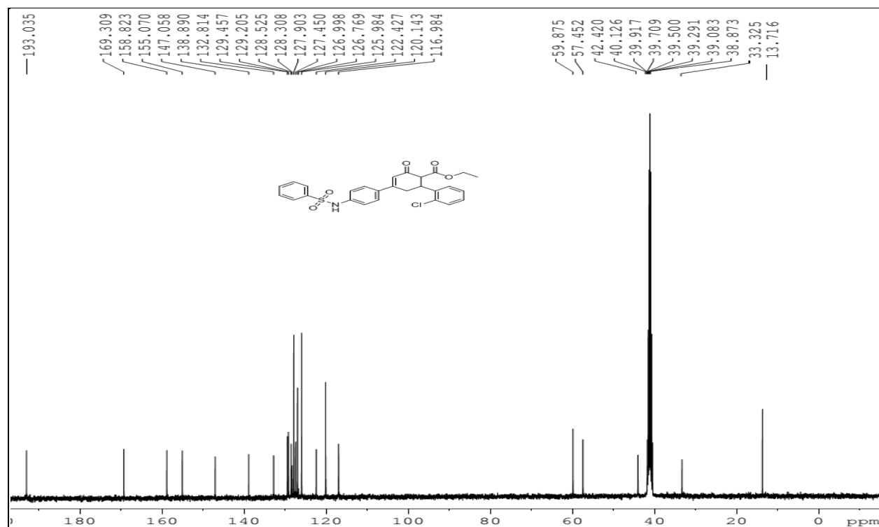
Fig. S52. 13 C spectrum of Ethyl 6-(2-chlorophenyl)-2-oxo-4-((4-phenylsulfonamido)phenyl)-cyclohex-3-enecarboxylate (7h)
