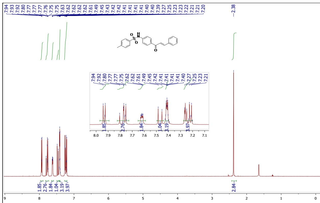
Fig. S23. 1 H spectrum of N -(4-(3-(3-chlorophenyl)acryloyl)phenyl)benzenesulfonamide (5l)
