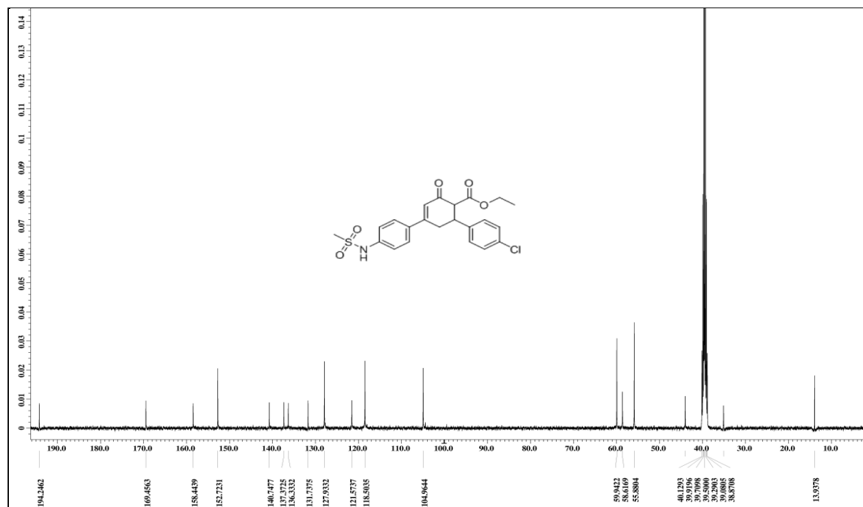
Fig. S70. ^{13}\text{C} spectrum of Ethyl 6-(4-chlorophenyl)-2-oxo-4-(4-methylsulfonamidophenyl)-cyclohex-3-ene carboxylate (7q)
