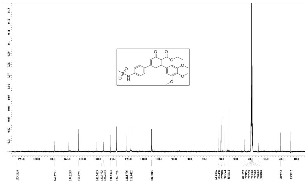
Fig. S72. ^{13}\text{C} spectrum of Ethyl 6-(3,4,5-trimethoxyphenyl)-2-oxo-4-(4-methylsulfonamido -phenyl)-cyclohex-3-ene carboxylate (7r)
