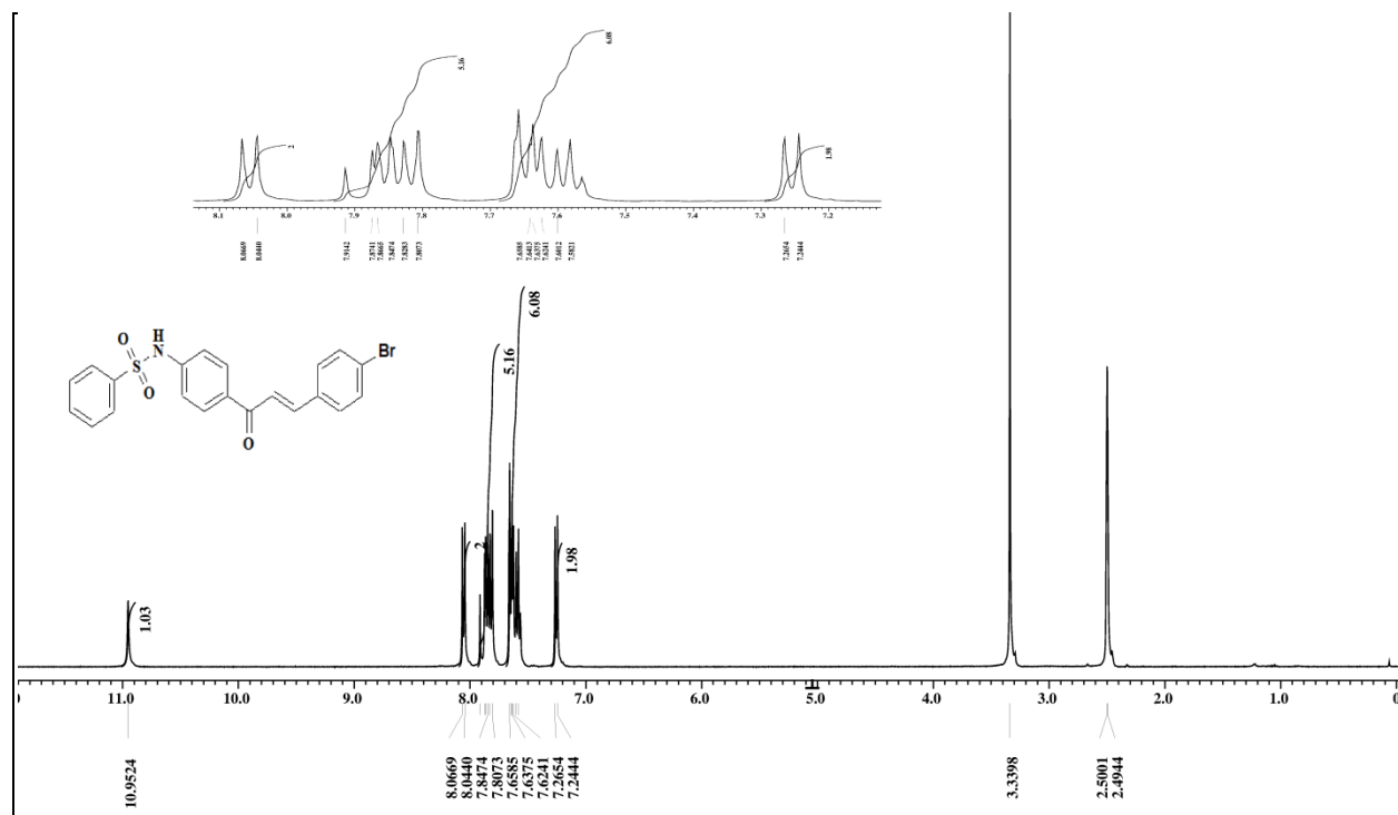
Fig. S7. 1 H spectrum of N -[4-(3-(4-bromophenyl)-acryloyl)-phenyl]-benzenesulfonamide (5d)
