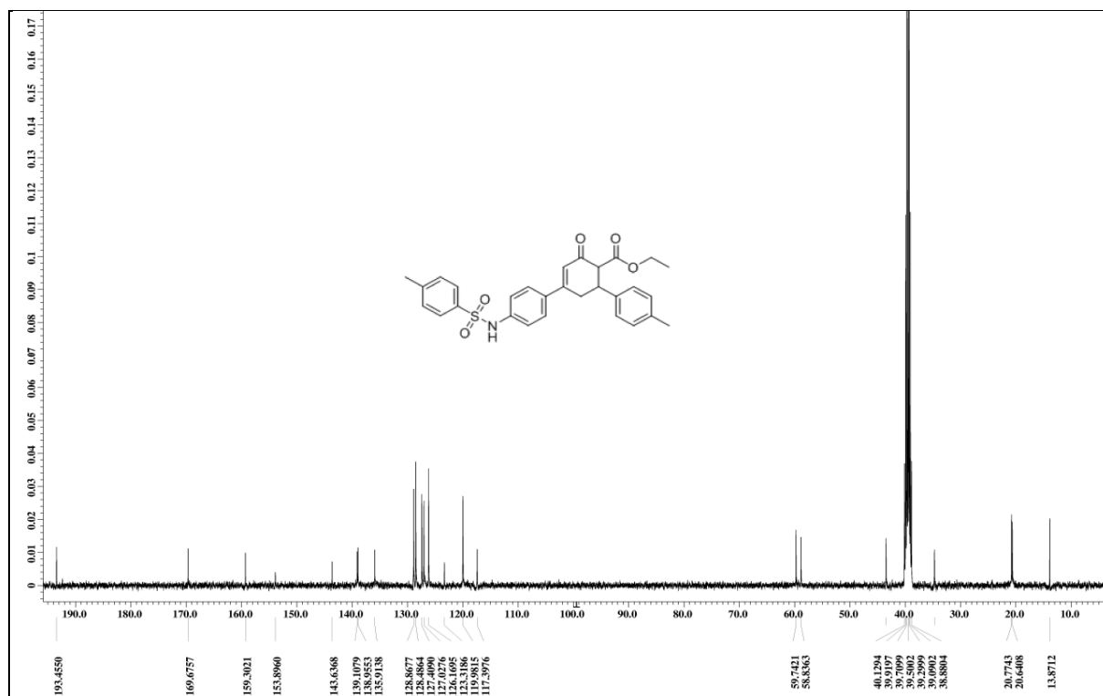
Fig. S66. 13 C spectrum of Ethyl 6-(4-methylphenyl)-2-oxo-4-((4-(4-methylphenylsulfonamido)-phenyl))-cyclohex-3-ene carboxylate (7o)
