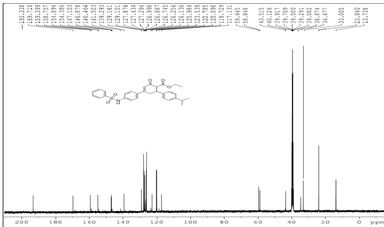
Fig. S46. 13 C Spectrum of Ethyl 6-(4-isopropylphenyl)-2-oxo-4-((4-phenylsulfonamido)phenyl)-cyclohex-3-enecarboxylate (7e)
