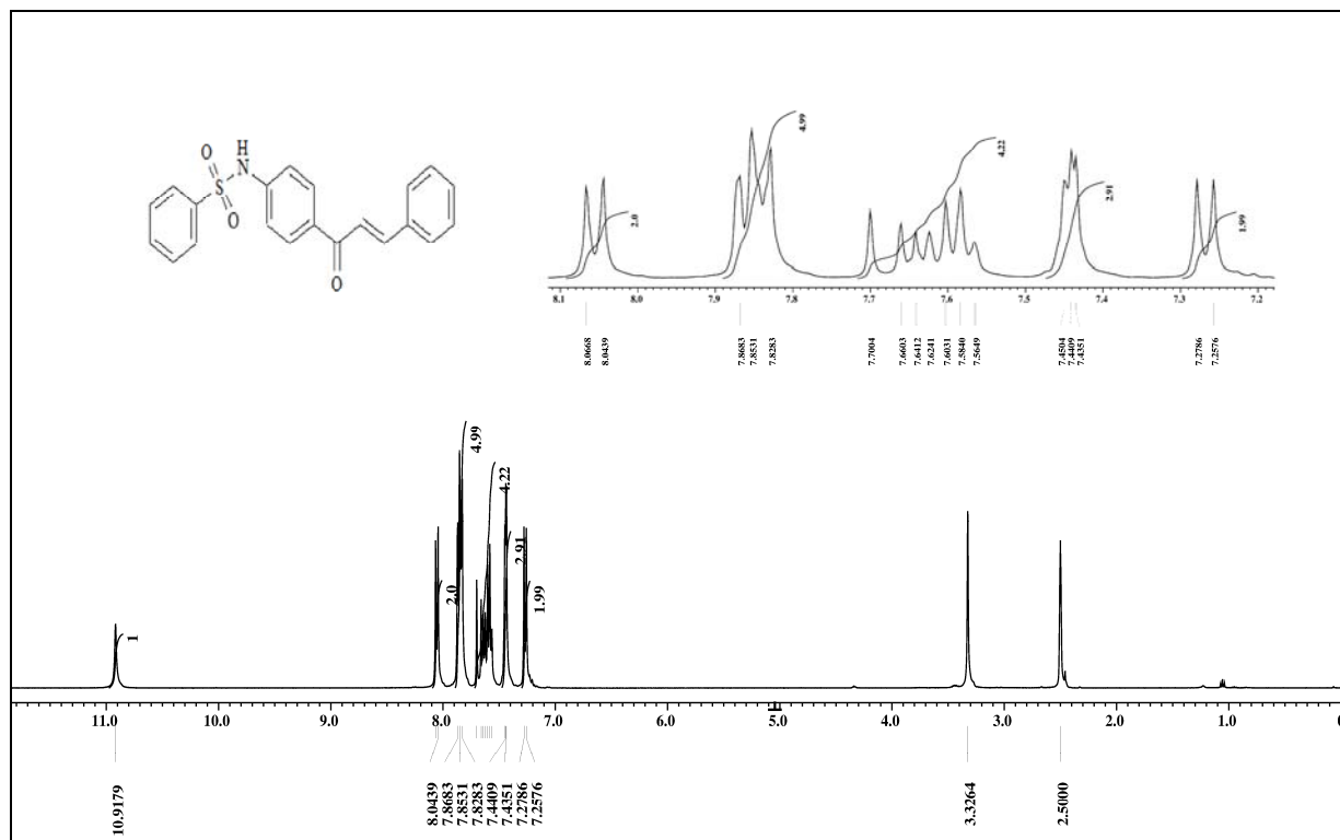
Fig. S1. 1 H spectrum of N -(4-cinnamoylphenyl)benzenesulfonamide (5a)
