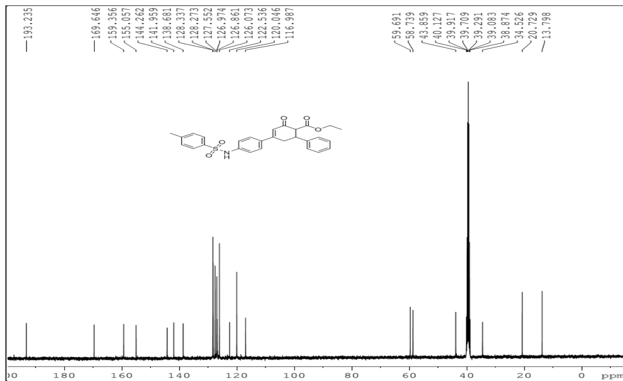
Fig. S60. 13 C spectrum of Ethyl 6-phenyl-2-oxo-4-((4-(4-methylphenylsulfonamido)phenyl))-cyclohex-3-enecarboxylate (7l)
