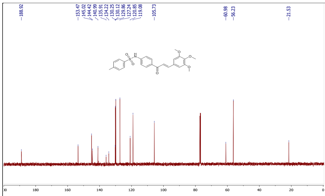
Fig. S28. 13 C spectrum of 4-methyl- N -(4-(3-(3,4,5-trimethoxyphenyl)acryloyl)phenyl)benzenesulfonamide (5n)
