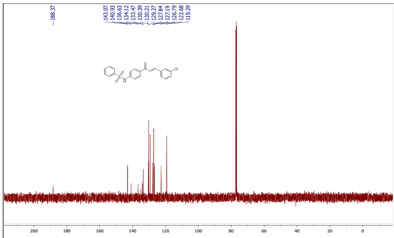
Fig. S22. 13 C spectrum of N -(4-(3-(3-chlorophenyl)acryloyl)phenyl)benzenesulfonamide (5k)
