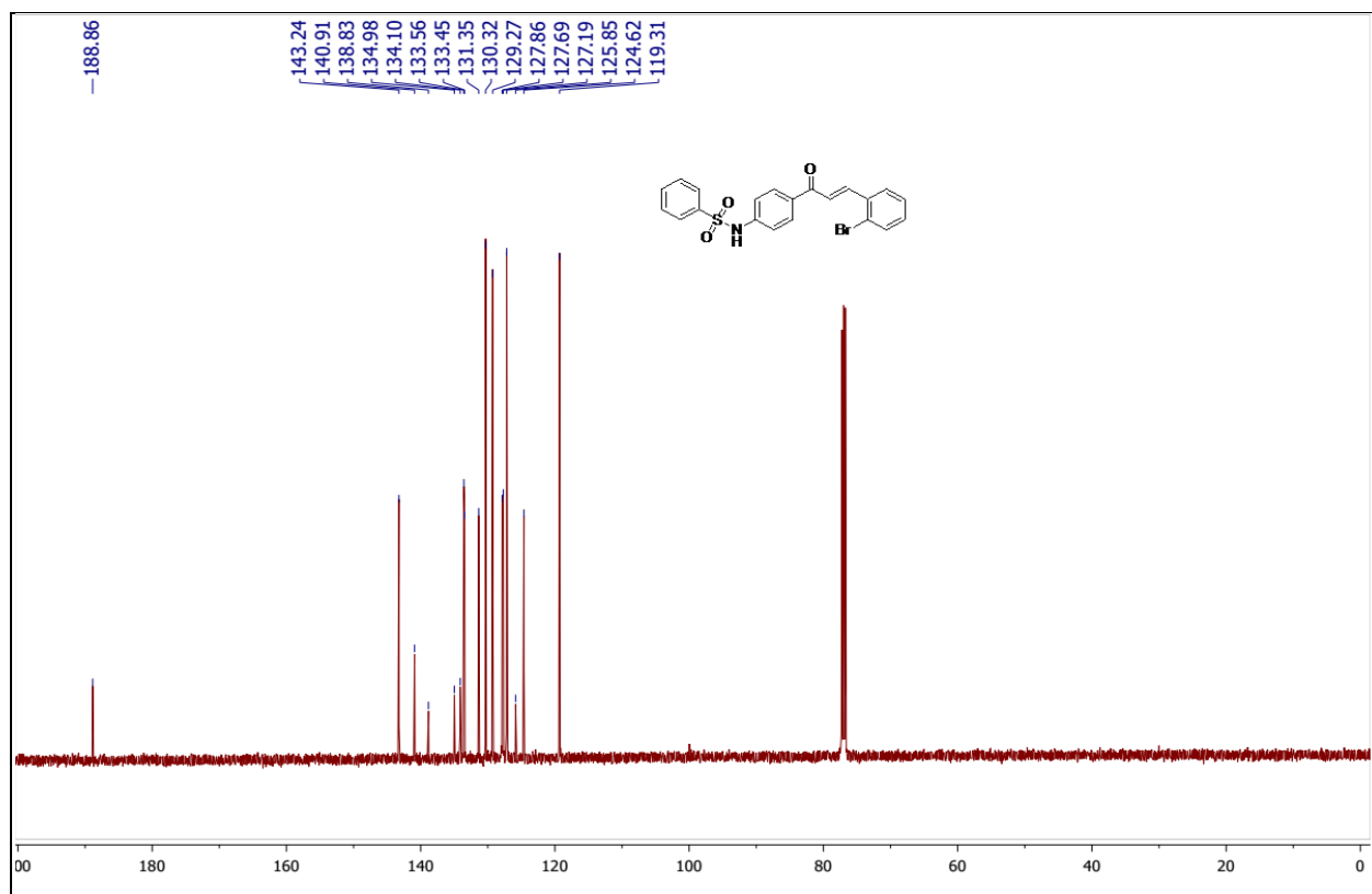
Fig. S18. ^{13}\text{C} spectrum of N -(4-(3-(2-bromophenyl)acryloyl)phenyl)benzenesulfonamide (5i)
