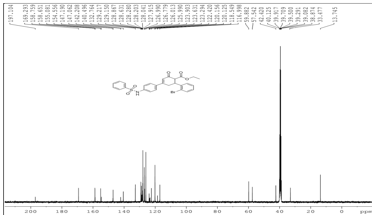
Fig. S54. ^{13}\text{C} spectrum of Ethyl 6-(2-bromophenyl)-2-oxo-4-((4-phenylsulfonamido)phenyl)-cyclohex-3-ene carboxylate (7i)
