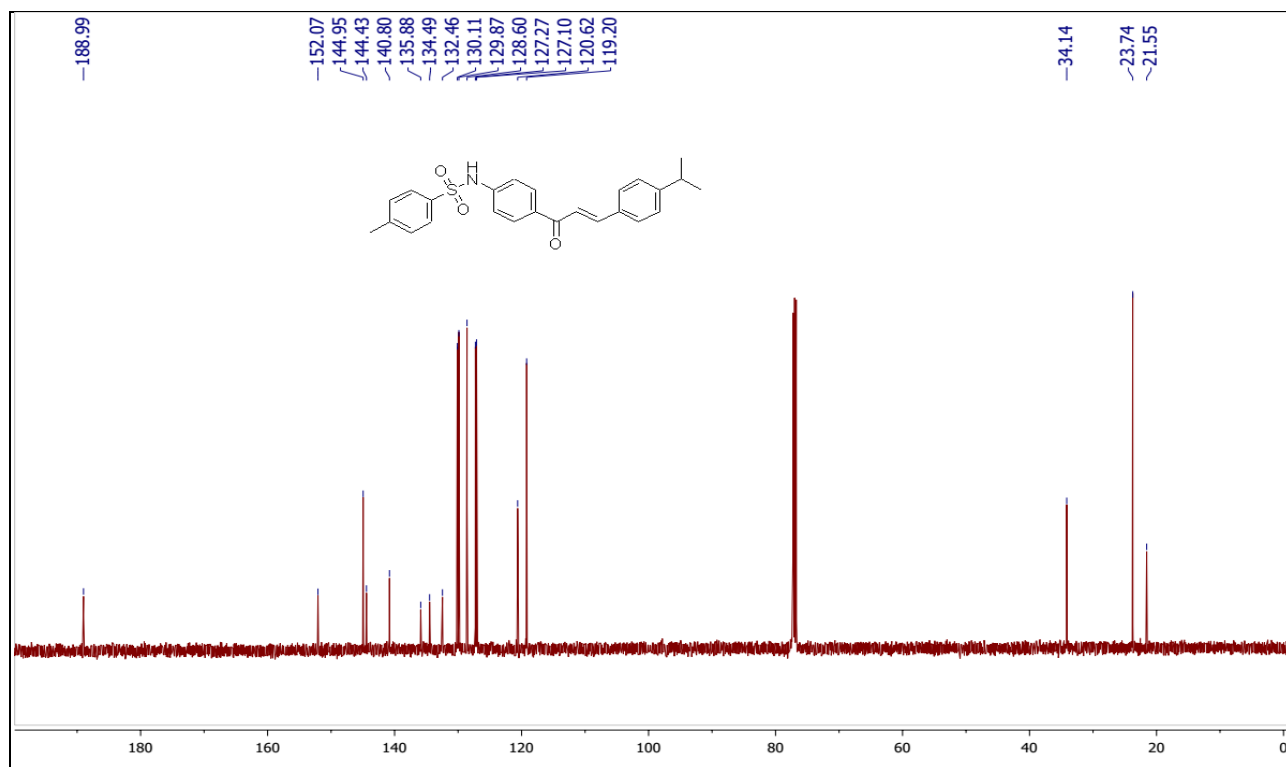
Fig. S26. ^{13}\text{C} spectrum of N -(4-(3-(4-isopropylphenyl)acryloyl)phenyl)-4-methylbenzenesulfonamide (5m)
