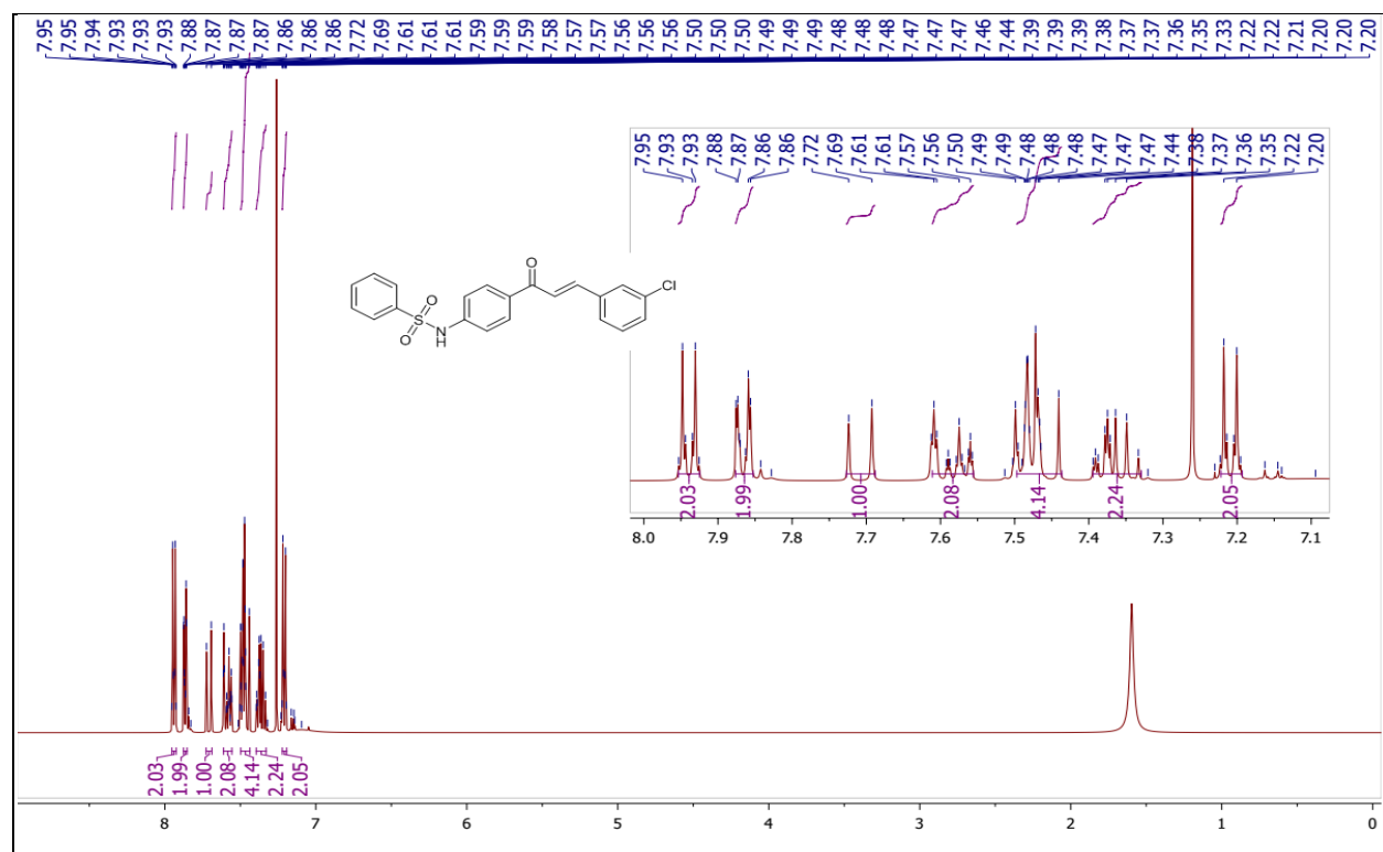
Fig. S21. ^1\text{H} spectrum of N -(4-(3-(3-chlorophenyl)acryloyl)phenyl)benzenesulfonamide (5k)
