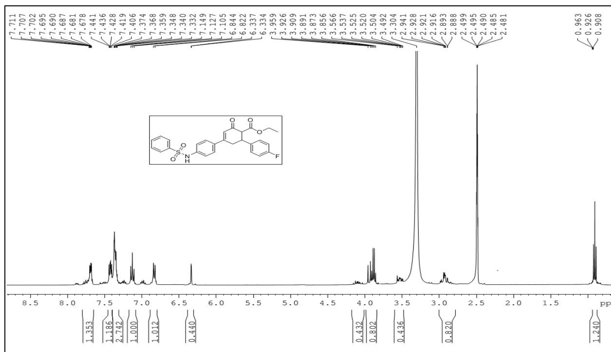
Fig. S41. 1 H Spectrum of Ethyl 6-(4-fluorophenyl)-2-oxo-4-((4-phenylsulfonamido)phenyl)-cyclohex-3-enecarboxylate (7c)
