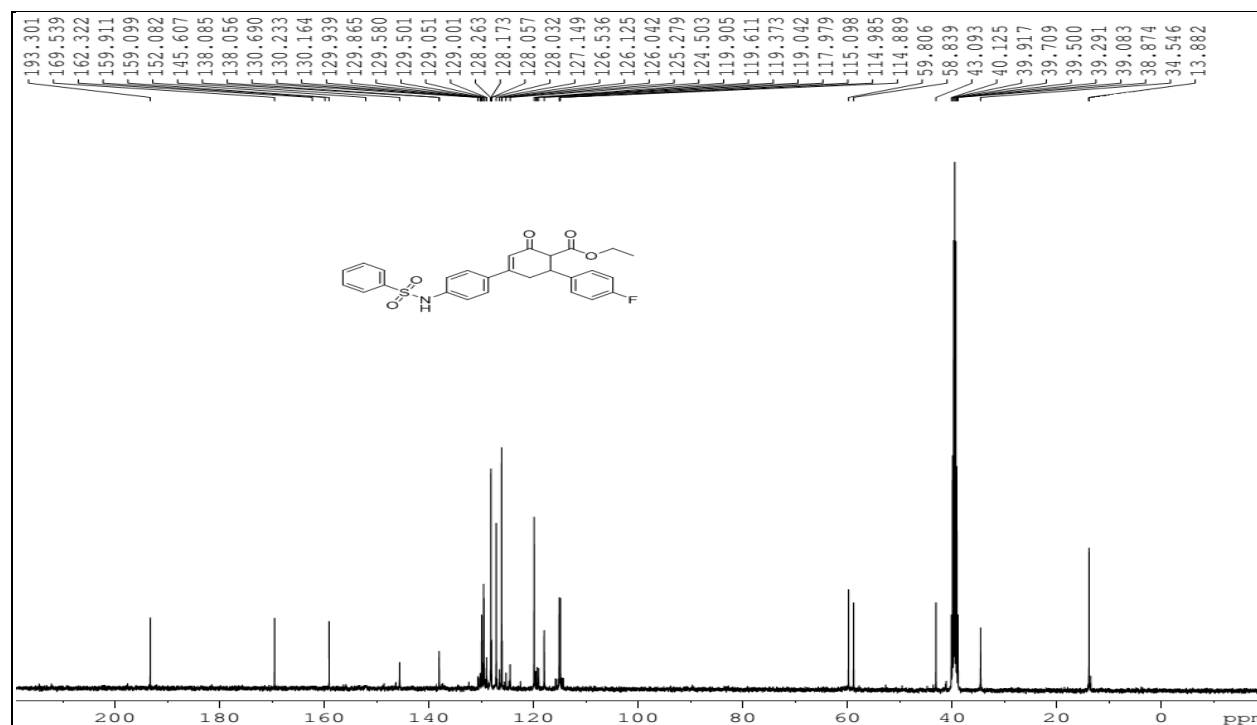
Fig. S42. 13 C Spectrum of Ethyl 6-(4-fluorophenyl)-2-oxo-4-((4-phenylsulfonamido)phenyl)-cyclohex-3-enecarboxylate (7c)
