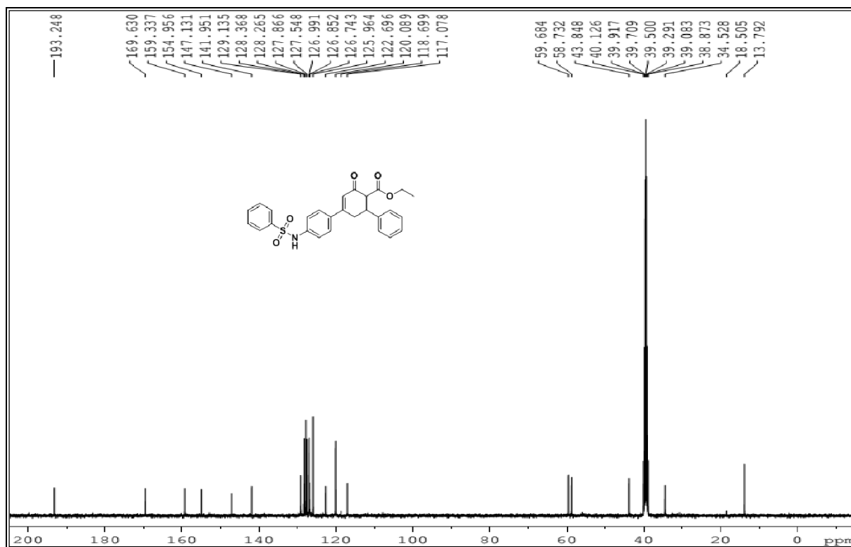
Fig. S38. ^{13}\text{C} spectrum of Ethyl 6-phenyl-2-oxo-4-((4-phenylsulfonamido)phenyl)-cyclohex-3-enecarboxylate (7a)
