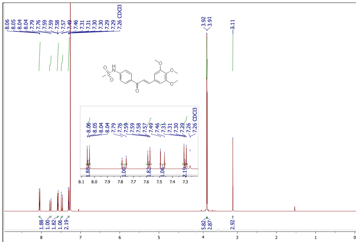
Fig. S35. ^1\text{H} spectrum of N -(4-(3-(3,4,5-trimethoxyphenyl)acryloyl)phenyl)methanesulfonamide (5r)
