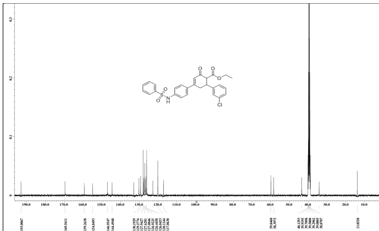
Fig. S58. 13 C spectrum of Ethyl 6-(3-chlorophenyl)-2-oxo-4-((4-phenylsulfonamido)phenyl)-cyclohex-3-enecarboxylate (7k)
