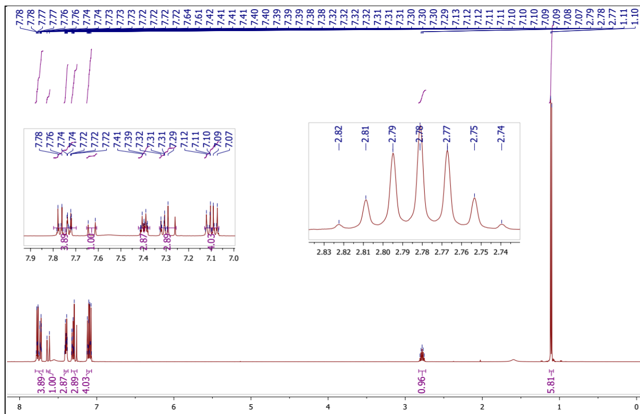
Fig. S9. 1 H spectrum of N -(4-(3-(4-isopropylphenyl)acryloyl)phenyl)benzenesulfonamide (5e)
