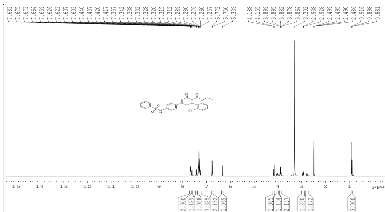
Fig. S51. ^1\text{H} spectrum of Ethyl 6-(2-chlorophenyl)-2-oxo-4-((4-phenylsulfonamido)phenyl)-cyclohex-3-enecarboxylate (7h)
