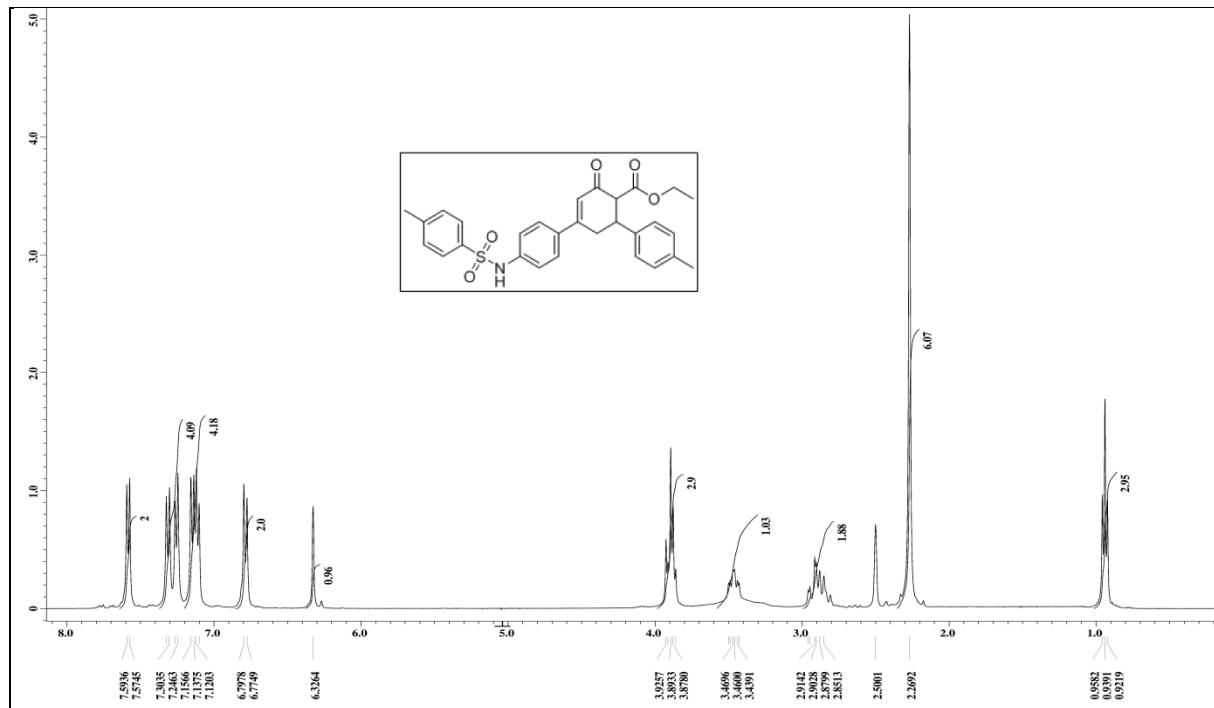
Fig. S65. 1 H spectrum of Ethyl 6-(4-methylphenyl)-2-oxo-4-((4-(4-methylphenylsulfonamido)phenyl)-cyclohex-3-ene carboxylate (7o)
