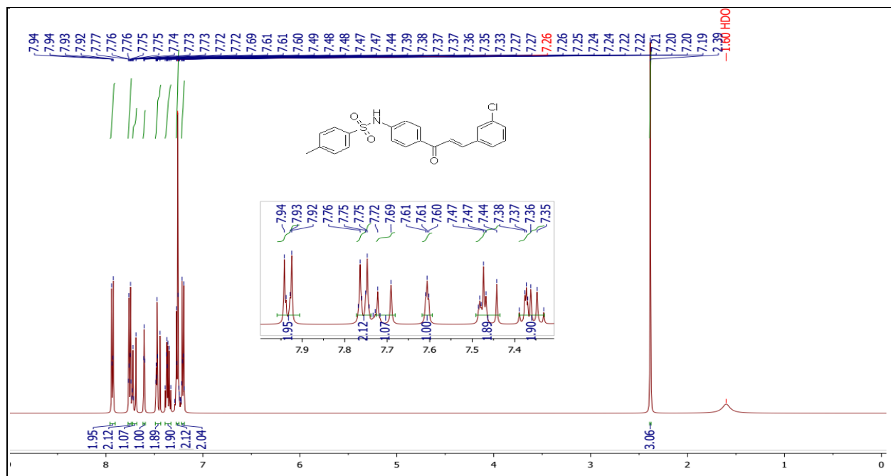
Fig. S31. ^1\text{H} spectrum of N -(4-(3-(3-chlorophenyl)acryloyl)phenyl)-4-methylbenzenesulfonamide (5p)
