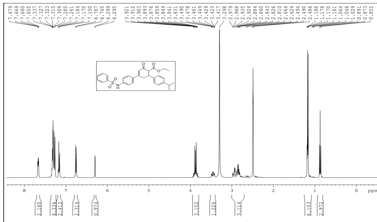
Fig. S45. 1 H Spectrum of Ethyl 6-(4-isopropylphenyl)-2-oxo-4-((4-phenylsulfonamido)phenyl)-cyclohex-3-enecarboxylate (7e)
