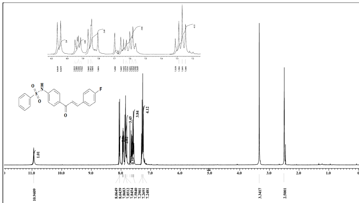
Fig. S5. 1 H spectrum of N -[4-(3-(4-fluorophenyl)acryloyl)phenyl]benzenesulfonamide (5c)
