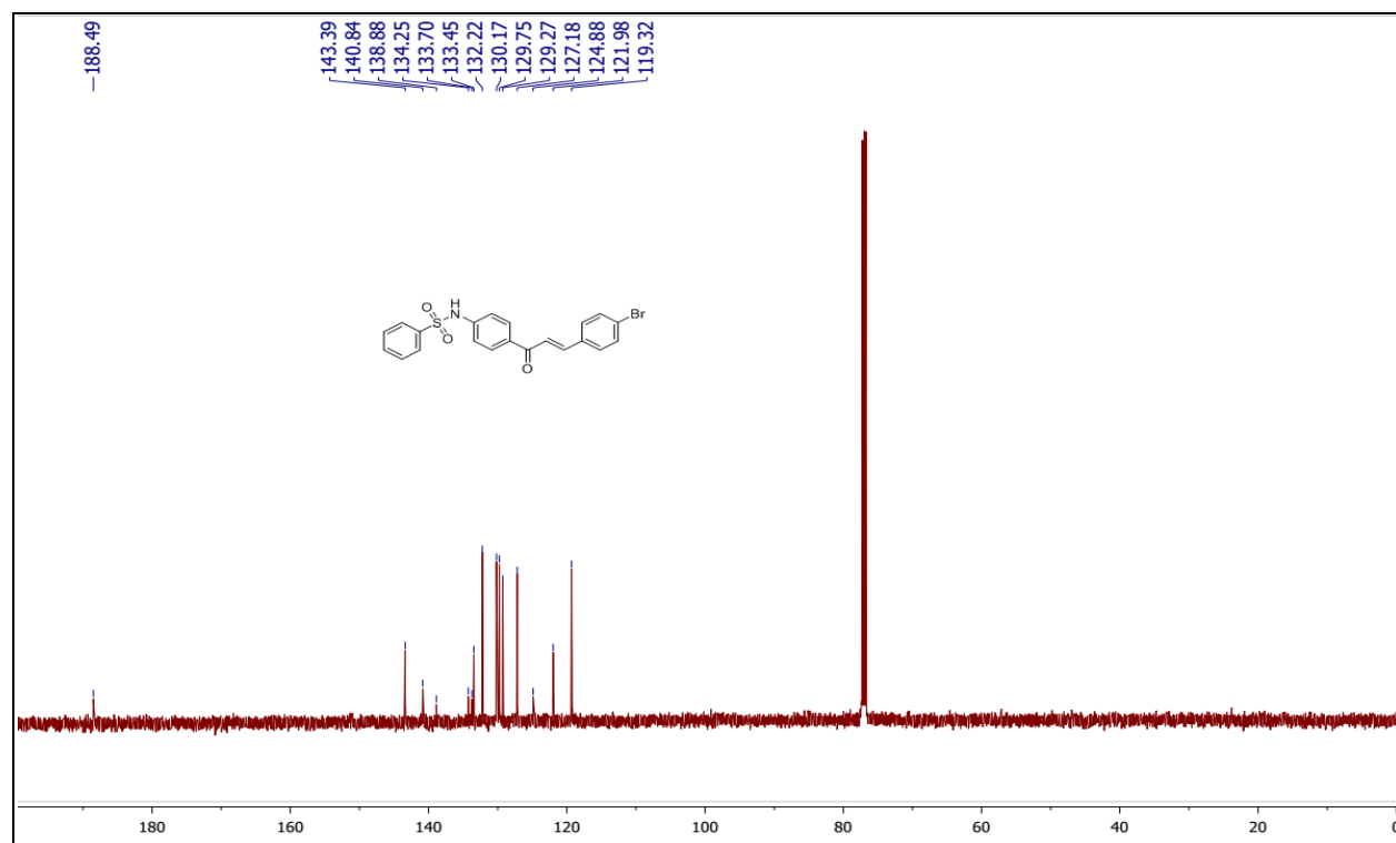
Fig. S8. 13 C spectrum of N -[4-(3-(4-bromophenyl)-acryloyl)-phenyl]-benzenesulfonamide (5d)
