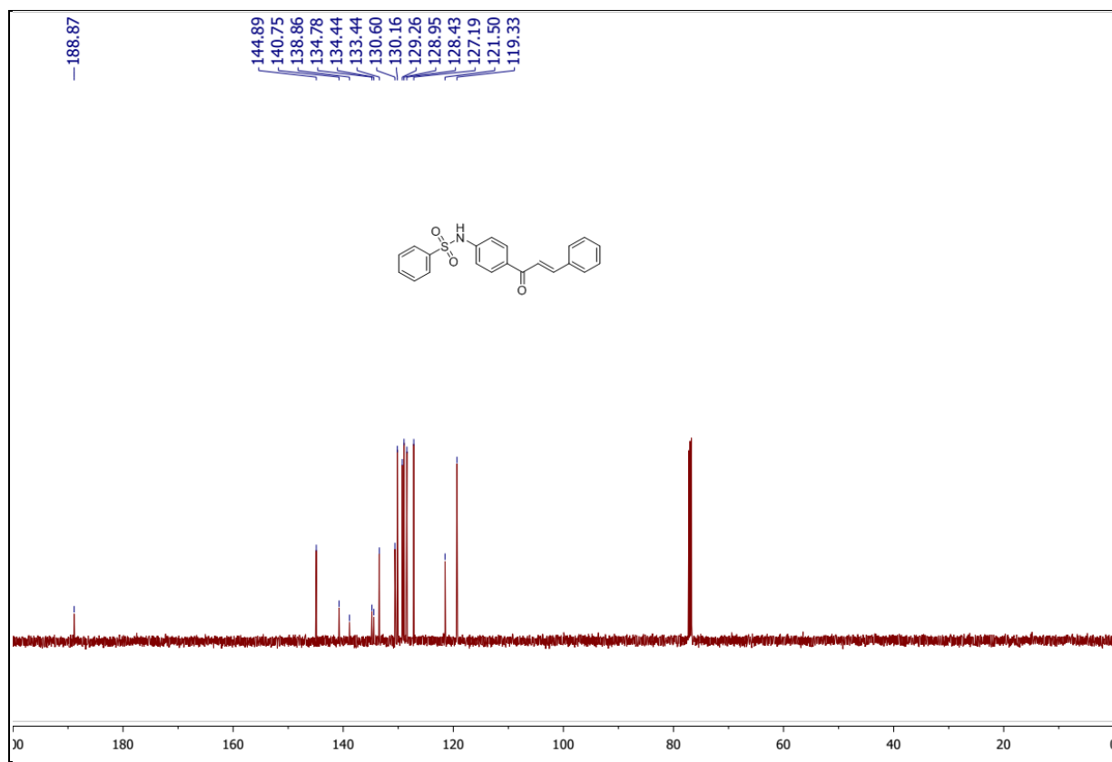
Fig. S2. 13 C spectrum of N -(4-cinnamoylphenyl)benzenesulfonamide (5a)
