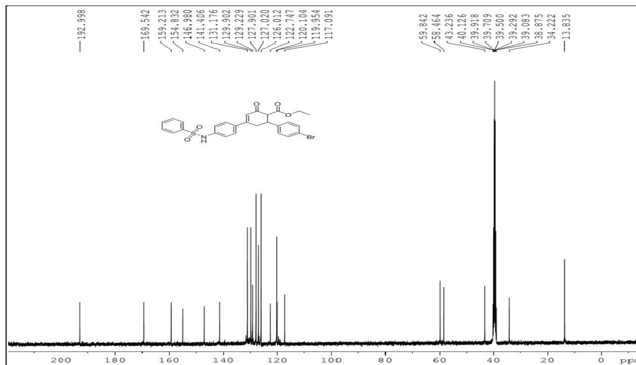
Fig. S44. 13 C Spectrum of Ethyl 6-(4-bromophenyl)-2-oxo-4-((4-phenylsulfonamido)phenyl)-cyclohex-3-enecarboxylate (7d)
