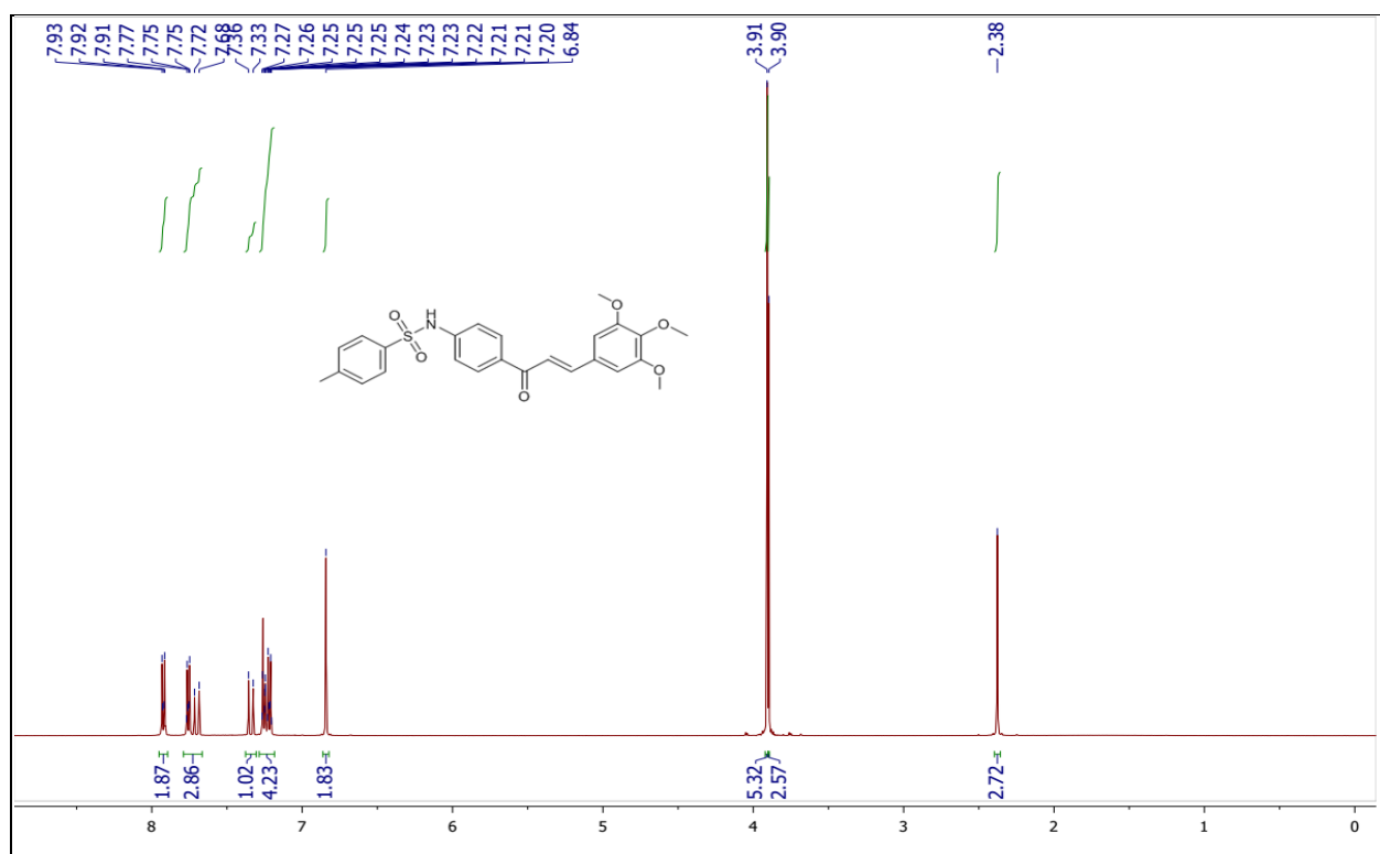
Fig. S27. ^1\text{H} spectrum of 4-methyl- N -(4-(3-(3,4,5-trimethoxyphenyl)acryloyl)phenyl)benzenesulfonamide (5n)
