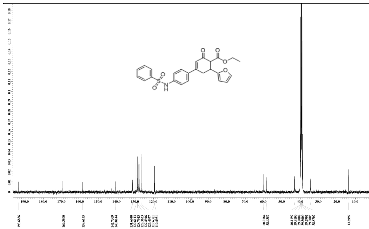
Fig. S48. 13 C Spectrum of Ethyl 6-(2-furyl)-2-oxo-4-((4-phenylsulfonamido)phenyl)-cyclohex-3-encarboxylate (7f)
