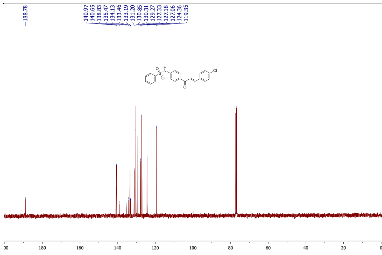
Fig. S4. 13 C spectrum of N -[4-(3-(4-chlorophenyl)-acryloyl)-phenyl]-benzenesulfonamide (5b)
