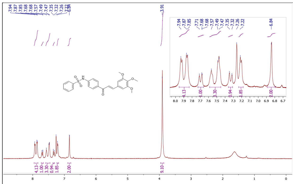
Fig. S13. 1 H spectrum of N -(4-(3-(3,4,5-trimethoxyphenyl)acryloyl)phenyl)benzenesulfonamide (5g)
