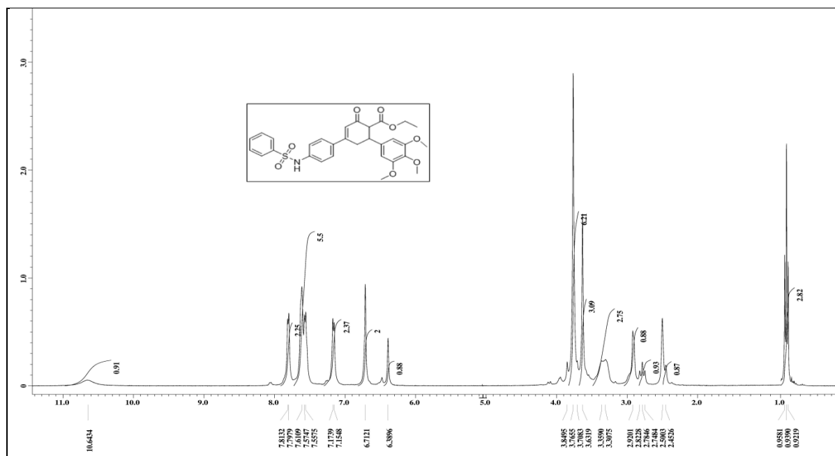
Fig. S49. 1 H Spectrum of Ethyl 6-(3,4,5-trimethoxyphenyl)-2-oxo-4-((4-phenylsulfonamido)phenyl)-cyclohex-3-encarboxylate (7g)
