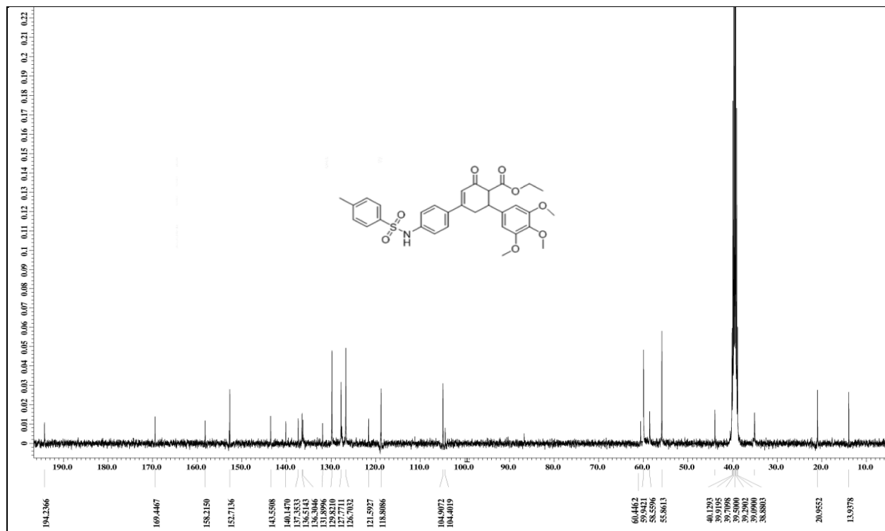
Fig. S64. 13 C spectrum of Ethyl 6-(3,4,5-trimethoxyphenyl)-2-oxo-4-((4-(4-methylphenylsulfonamido)phenyl)-cyclohex-3-enecarboxylate (7n)
