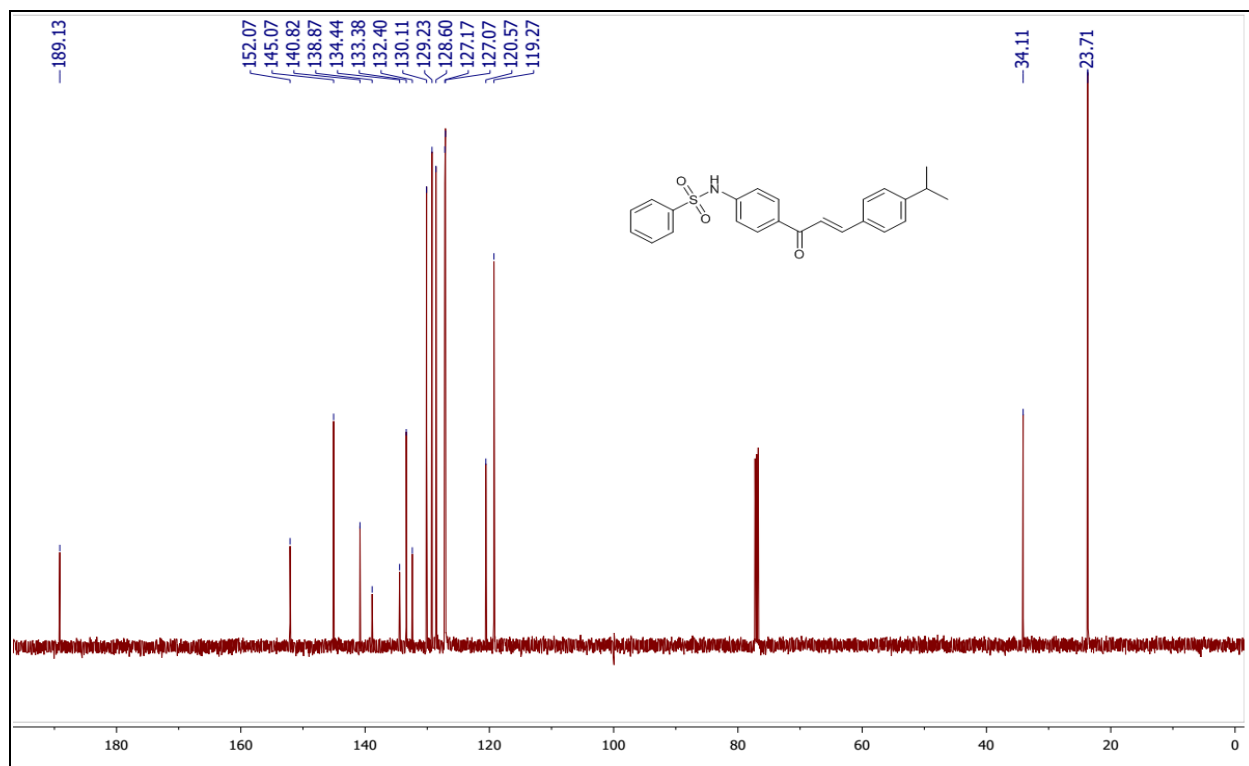
Fig. S10. 13 C spectrum of N -(4-(3-(4-isopropylphenyl)acryloyl)phenyl)benzenesulfonamide (5e)
