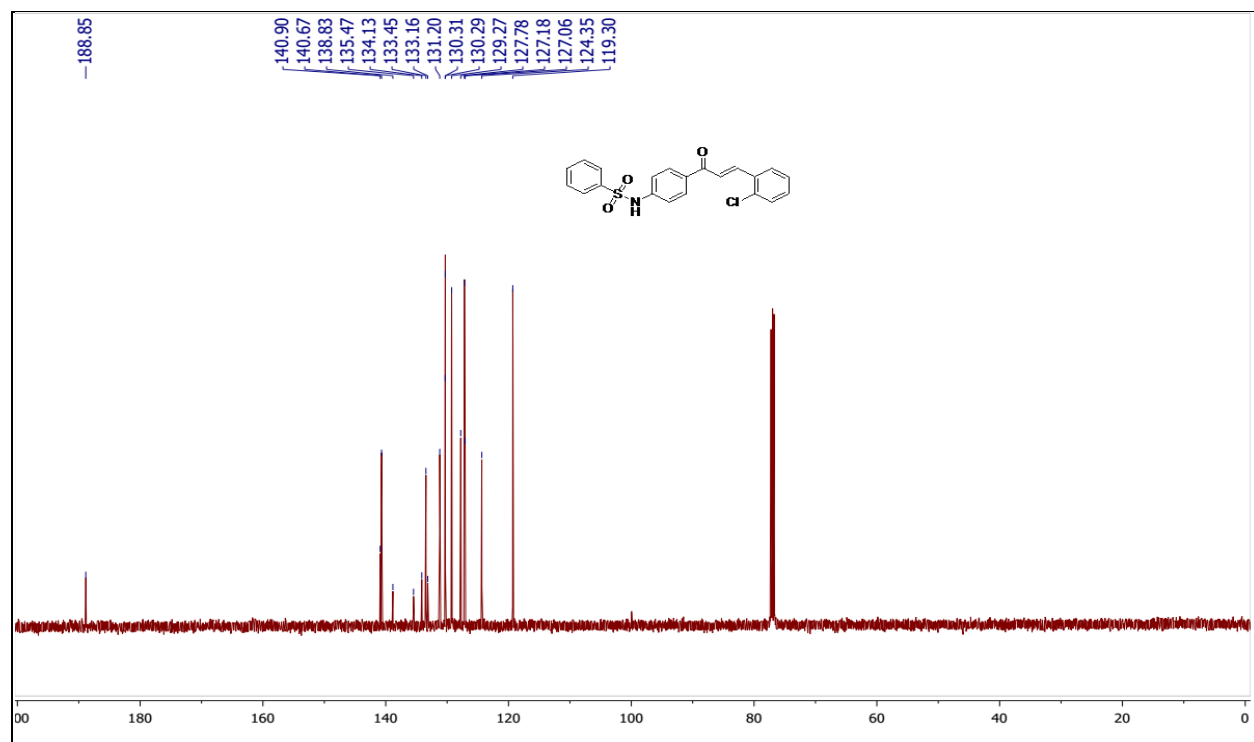
Fig. S16. 13 C spectrum of N -(4-(3-(2-chlorophenyl)acryloyl)phenyl)benzenesulfonamide (5h)
