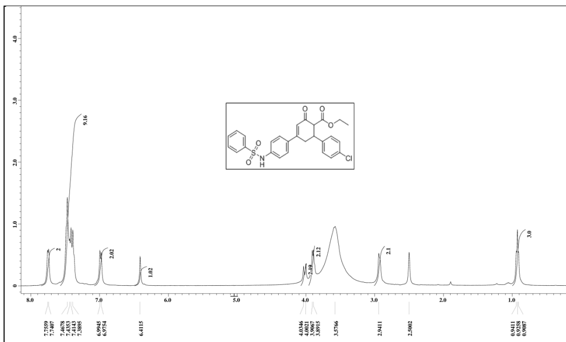
Fig. S39. ^1\text{H} Spectrum of Ethyl 6-(4-chlorophenyl)-2-oxo-4-((4-phenylsulfonamido)phenyl)-cyclohex-3-enecarboxylate (7b)
