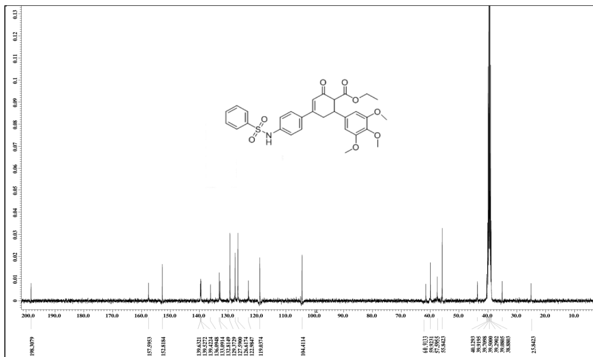
Fig. S50. ^{13}\text{C} Spectrum of Ethyl 6-(3,4,5-trimethoxyphenyl)-2-oxo-4-((4-phenylsulfonamido)-phenyl)-cyclohex-3-enecarboxylate (7g)
