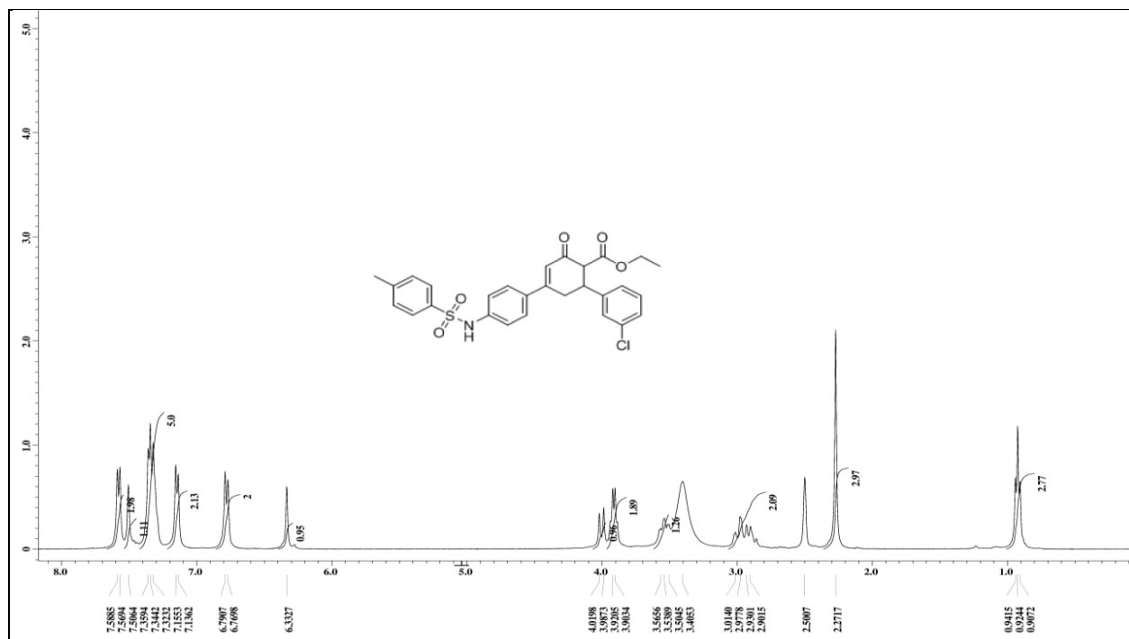
Fig. S67. 1 H spectrum of Ethyl 6-(3-chlorophenyl)-2-oxo-4-((4-(4-methylphenylsulfonamido)-phenyl))-cyclohex-3-ene carboxylate (7p)
