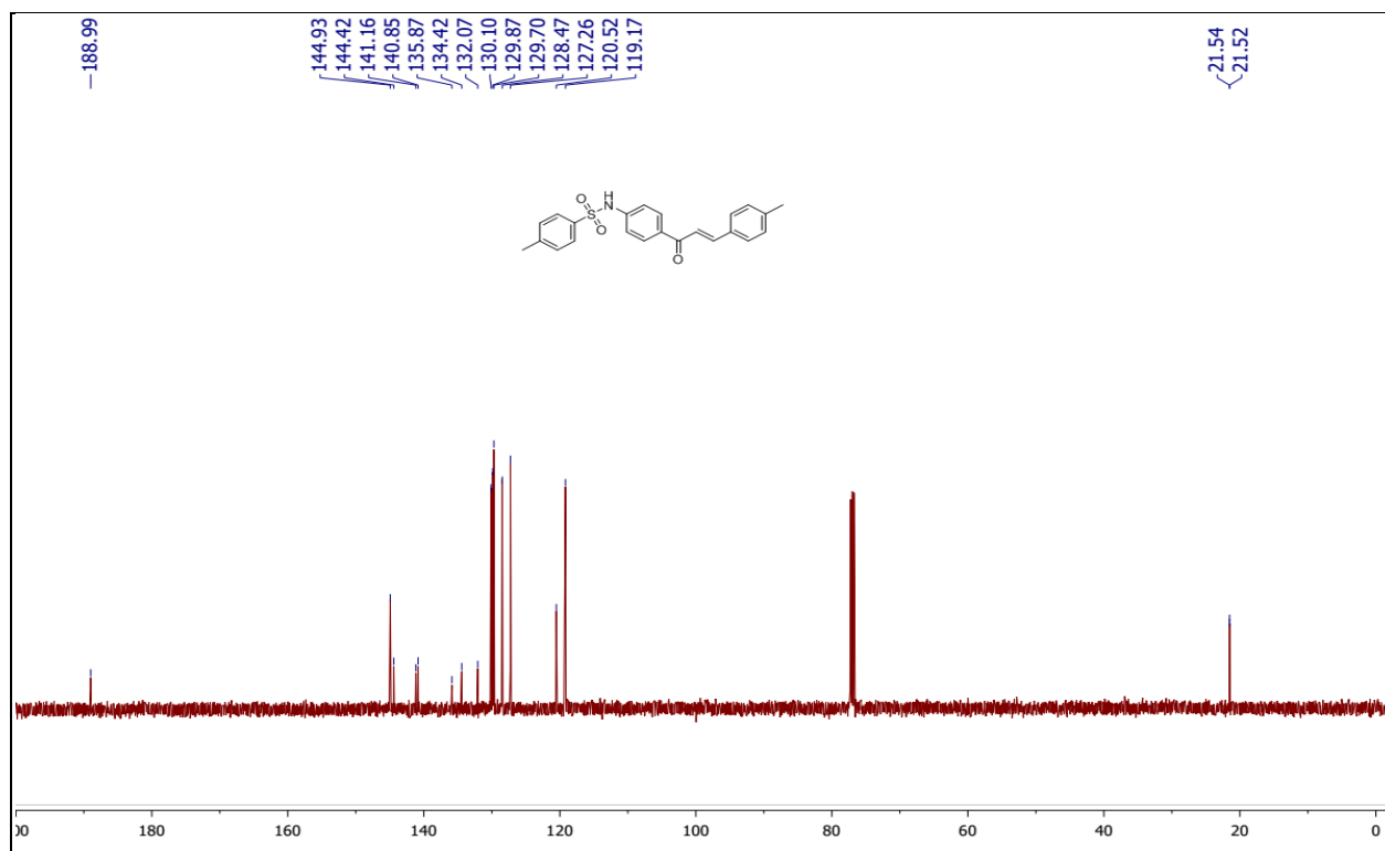
Fig. S30. ^{13}\text{C} spectrum of 4-methyl- N -(4-(3-( p -tolyl)acryloyl)phenyl)benzenesulfonamide (5o)
