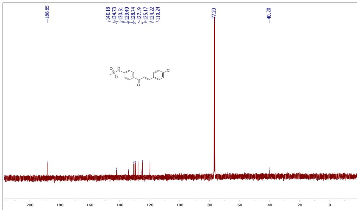
Fig. S34. ^{13}\text{C} spectrum of N -(4-(3-(4-chlorophenyl)acryloyl)phenyl)methanesulfonamide (5q)
