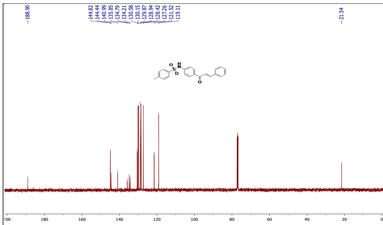
Fig. S24. 13 C spectrum of N -(4-cinnamoylphenyl)-4-methylbenzenesulfonamide (5l)
