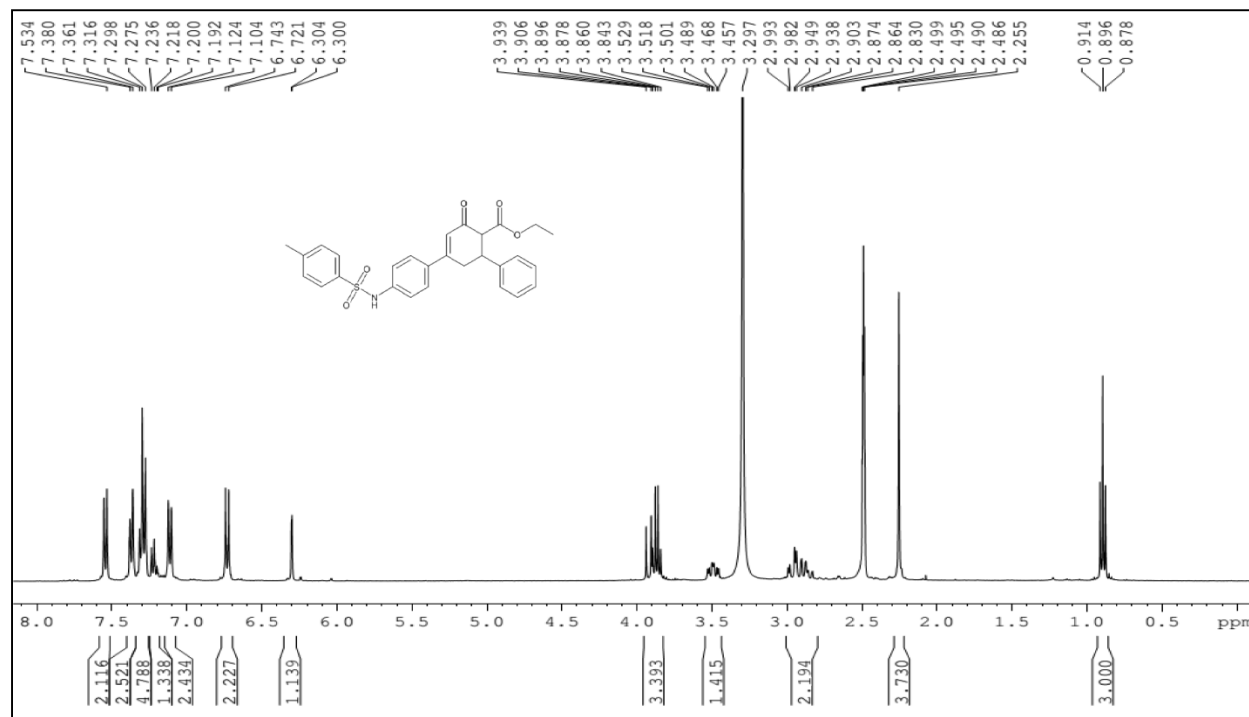
Fig. S59. 1 H spectrum of Ethyl 6-phenyl-2-oxo-4-((4-(4-methylphenylsulfonamido)phenyl)-cyclohex-3-enecarboxylate (7l)
