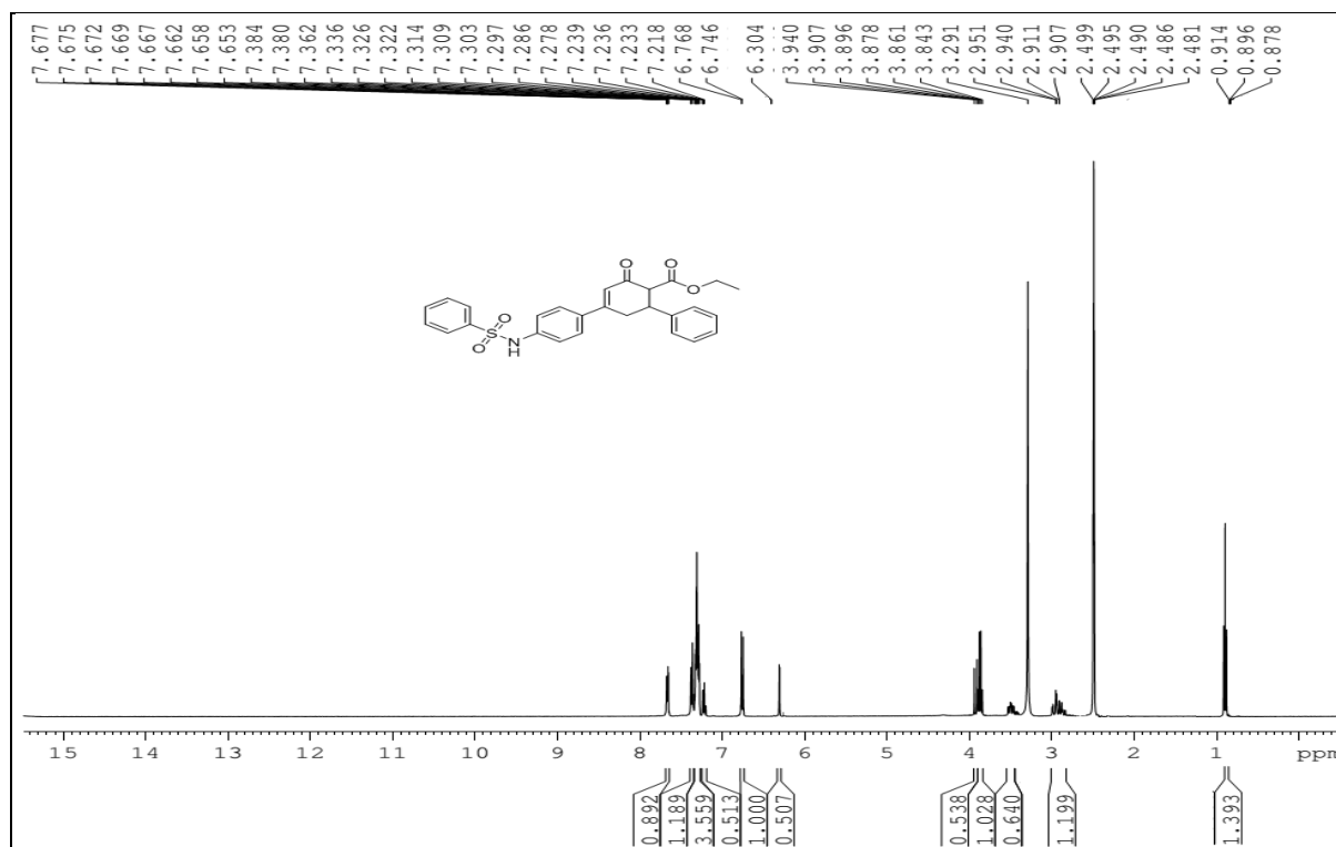
Fig. S37. 1 H spectrum of Ethyl 6-phenyl-2-oxo-4-((4-phenylsulfonamido)phenyl)-cyclohex-3-enecarboxylate (7a)
