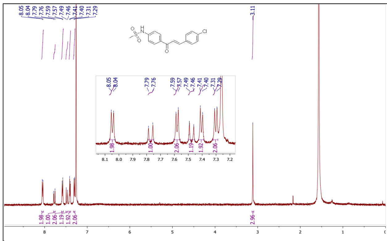
Fig. S33. 1 H spectrum of N -(4-(3-(4-chlorophenyl)acryloyl)phenyl)methanesulfonamide (5q)
