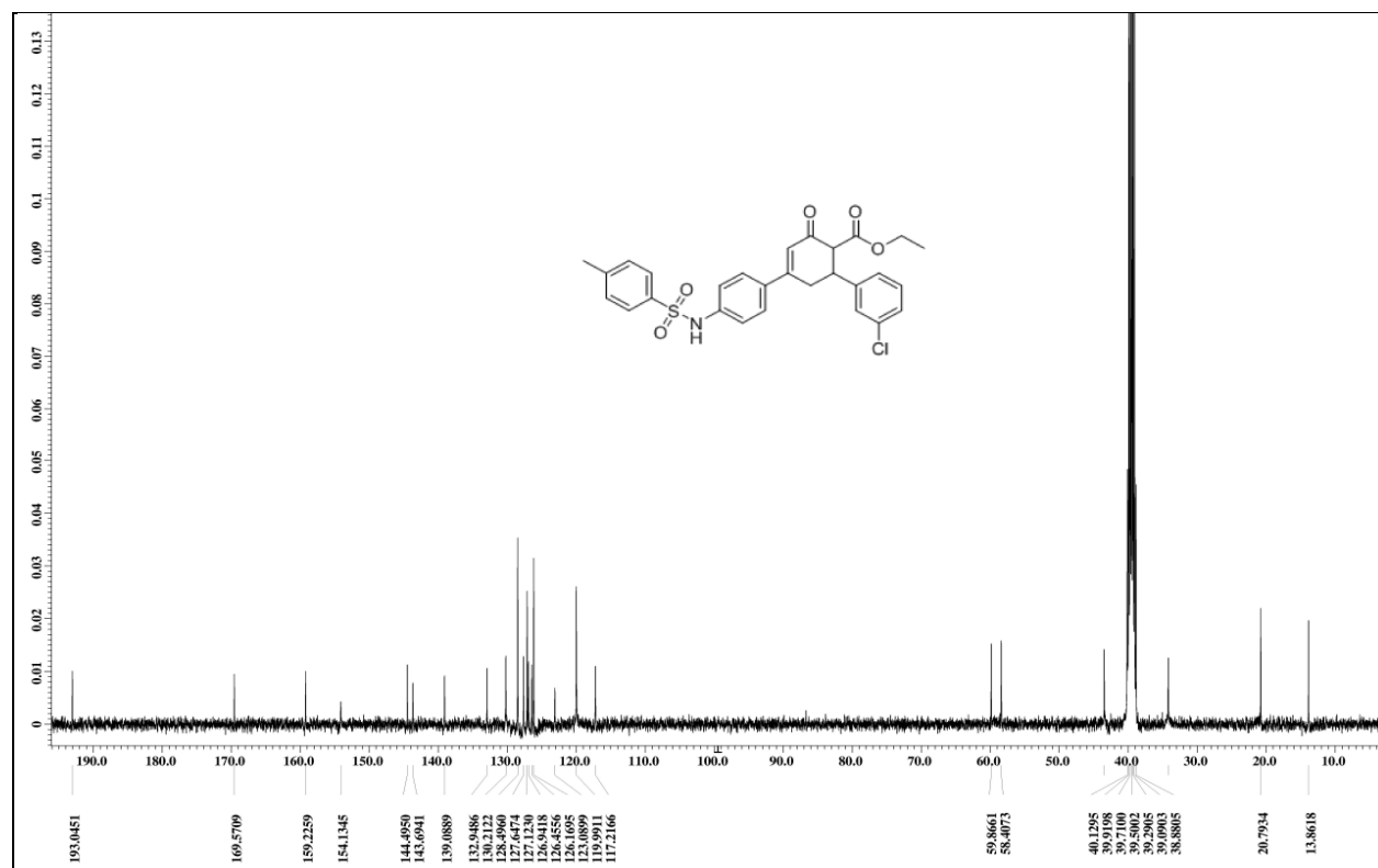
Fig. S68. ^{13}\text{C} spectrum of Ethyl 6-(3-chlorophenyl)-2-oxo-4-((4-(4-methylphenylsulfonamido)-phenyl))-cyclohex-3-ene carboxylate (7p)
