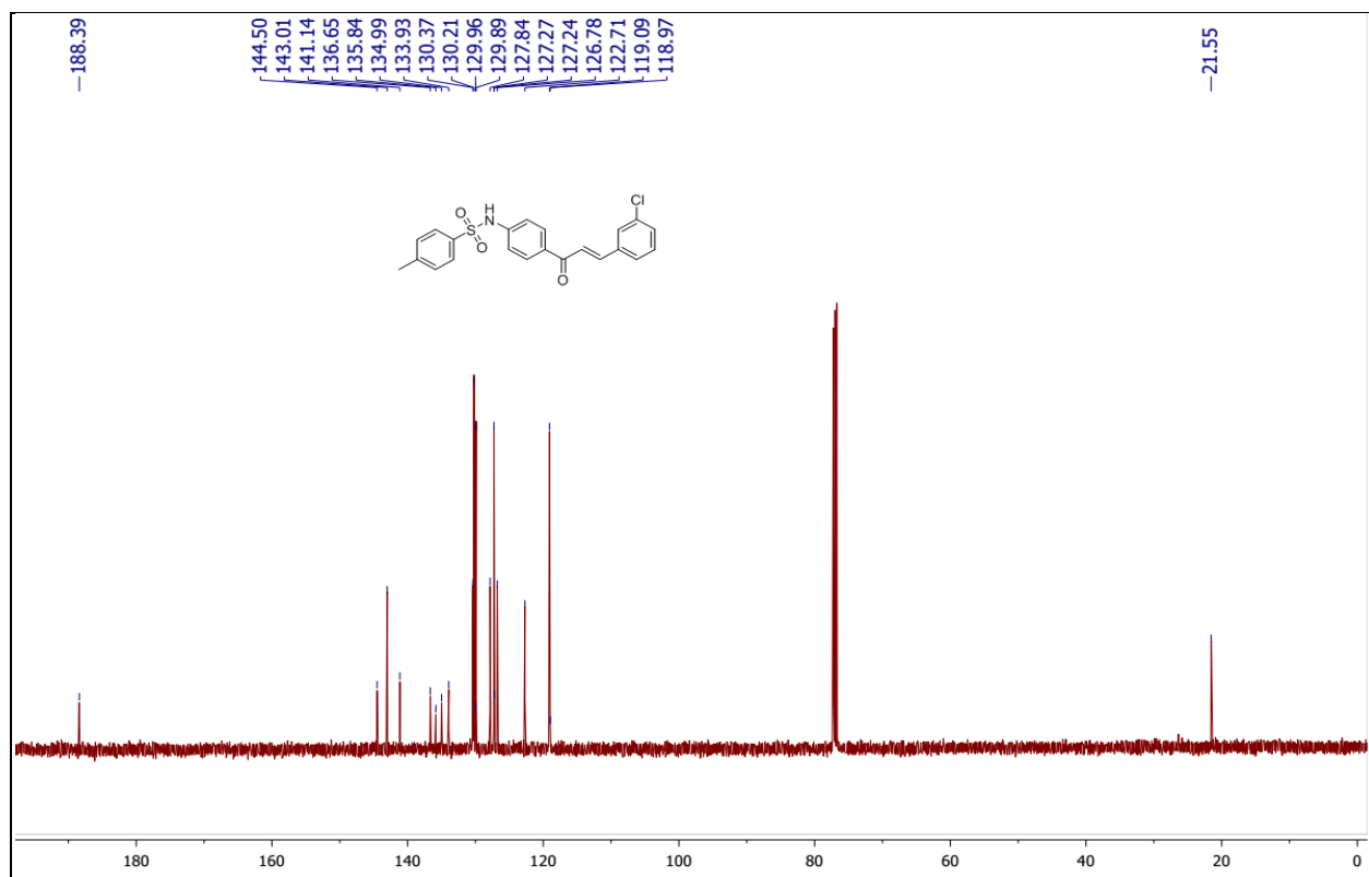
Fig. S32. 13 C spectrum of N -(4-(3-(3-chlorophenyl)acryloyl)phenyl)-4-methylbenzenesulfonamide (5p)
