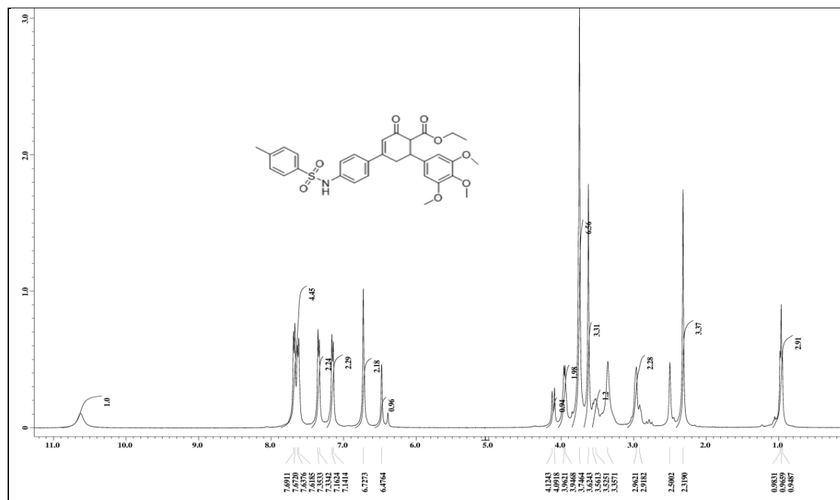
Fig. S63. 1 H spectrum of Ethyl 6-(3,4,5-trimethoxyphenyl)-2-oxo-4-((4-(4-methylphenylsulfonamido)phenyl)-cyclohex-3-enecarboxylate (7n)
