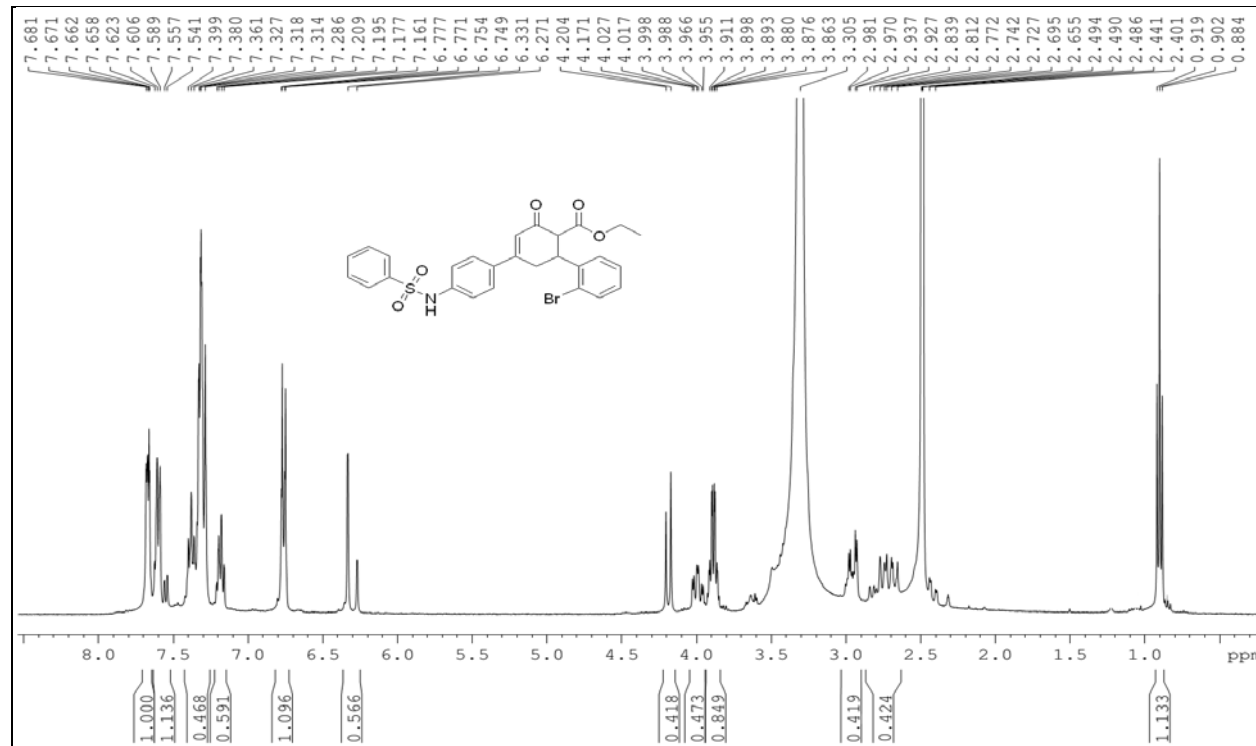
Fig. S53. 1 H spectrum of Ethyl 6-(2-bromophenyl)-2-oxo-4-((4-phenylsulfonamido)phenyl)-cyclohex-3-enecarboxylate (7i)
