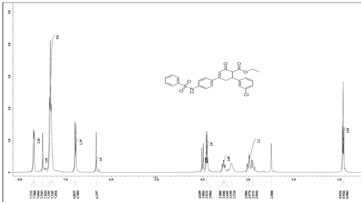
Fig. S57. 1 H spectrum of Ethyl 6-(3-chlorophenyl)-2-oxo-4-((4-phenylsulfonamido)phenyl)-cyclohex-3-enecarboxylate (7k)
