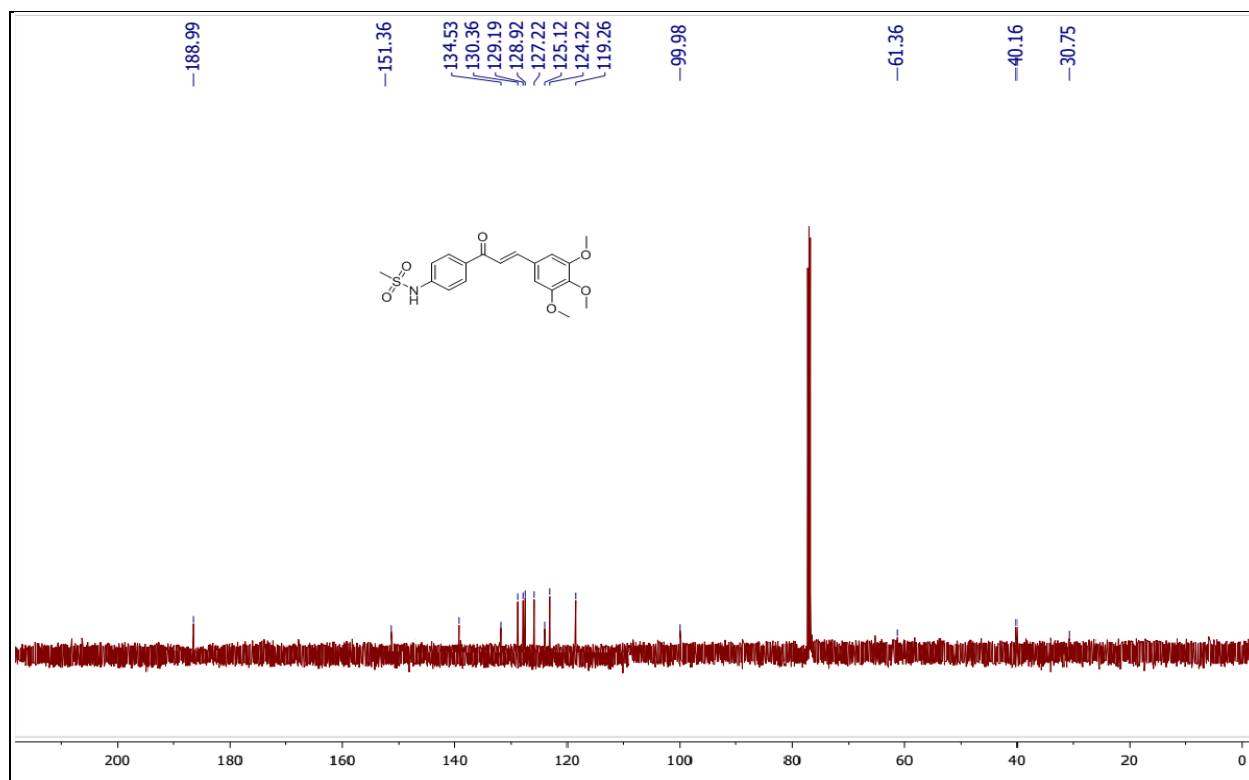
Fig. S36. 13 C spectrum of N -(4-(3-(3,4,5-trimethoxyphenyl)acryloyl)phenyl)methanesulfonamide (5r)
