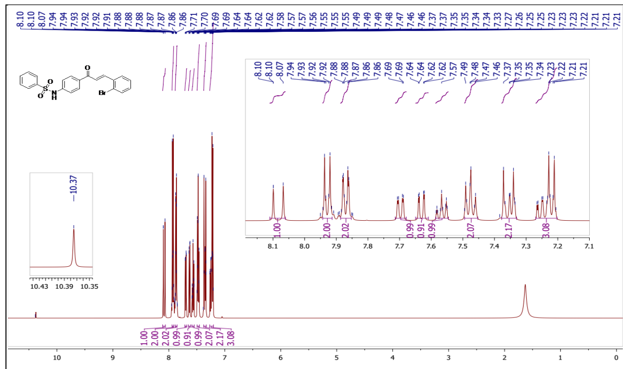
Fig. S17. 1 H spectrum of N -(4-(3-(2-bromophenyl)acryloyl)phenyl)benzenesulfonamide (5i)
