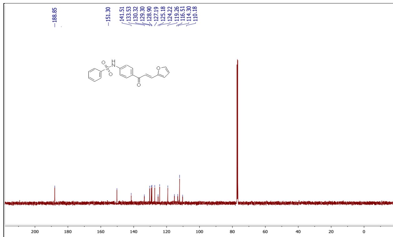
Fig. S12. 13 C spectrum of N -(4-(3-(furan-2-yl)acryloyl)phenyl)benzenesulfonamide (5f)
