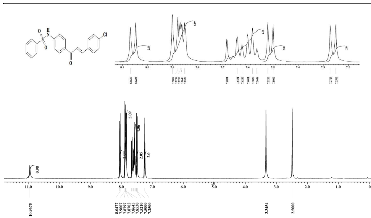
Fig. S3. 1 H spectrum of N -[4-(3-(4-chlorophenyl)-acryloyl)-phenyl]-benzenesulfonamide (5b)
