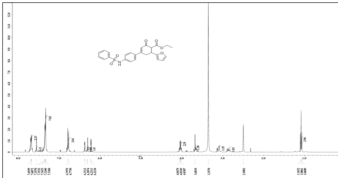
Fig. S47. 1 H Spectrum of Ethyl 6-(2-furyl)-2-oxo-4-((4-phenylsulfonamido)phenyl)-cyclohex-3-enecarboxylate (7f)
