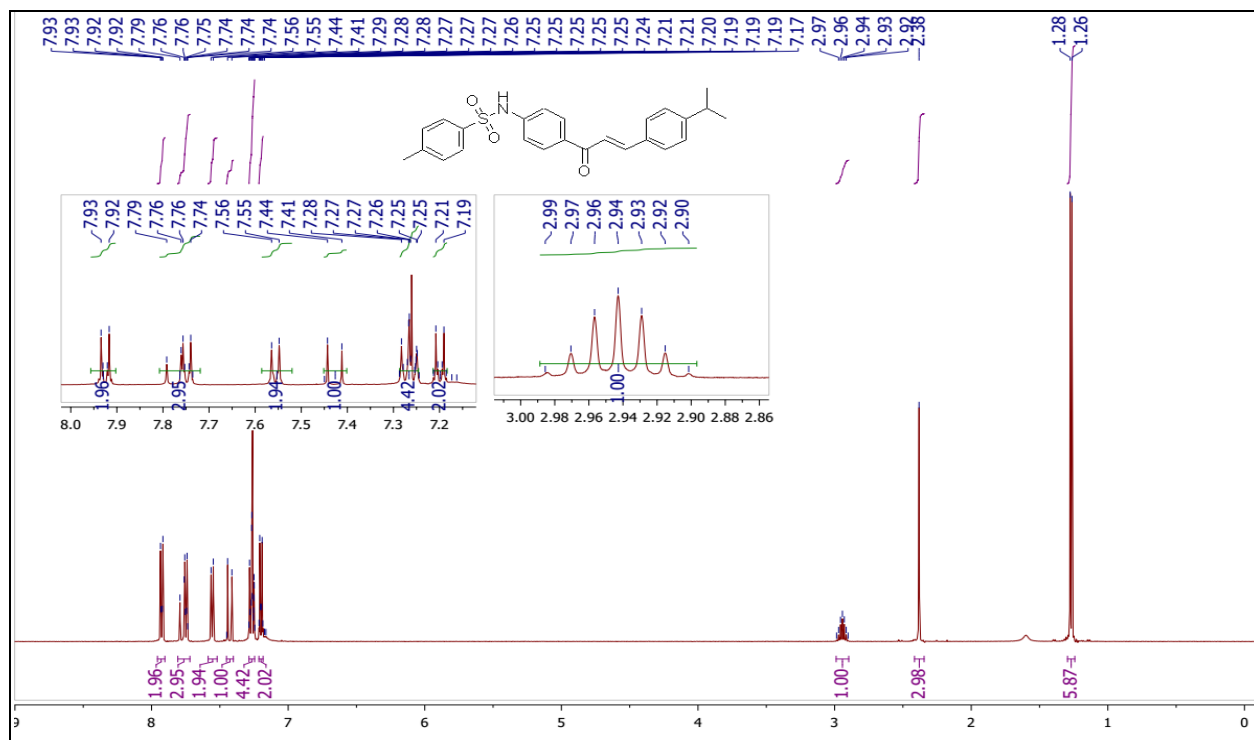
Fig. S25. 1 H spectrum of N -(4-(3-(4-isopropylphenyl)acryloyl)phenyl)-4-methylbenzenesulfonamide (5m)
