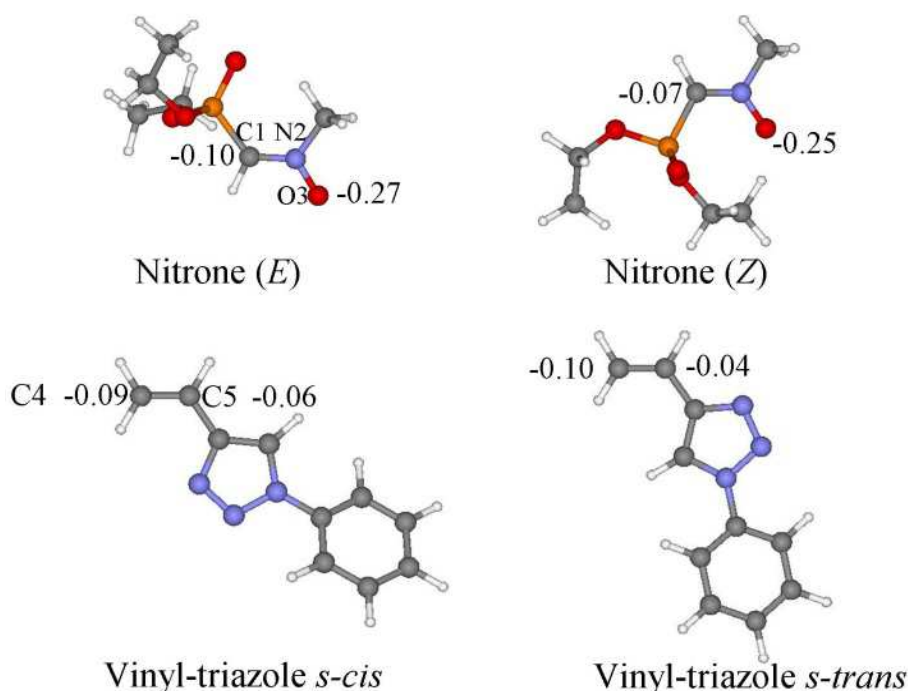
Figure 4. Hirshfeld charges (e.u.) on reactive atoms of reagent in the various conformations.
