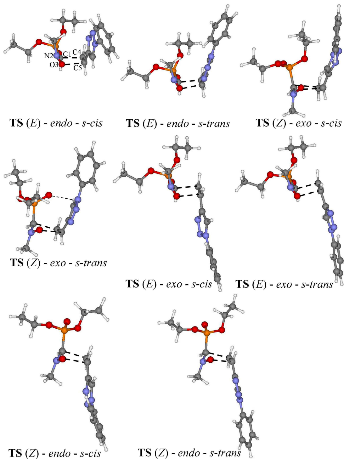
Figure 5. Molecular structures of the eight transition states for the formation of the cis and trans -adducts of the 3,5 regioisomer.
