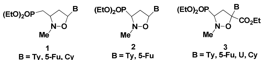
Figure 1. Phosphonated N,O -nucleosides.
