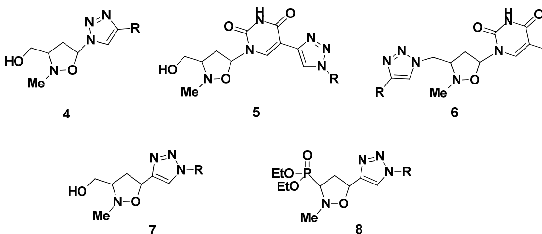
Figure 2. 1,2,3-Triazolyl- N,O -nucleosides.
