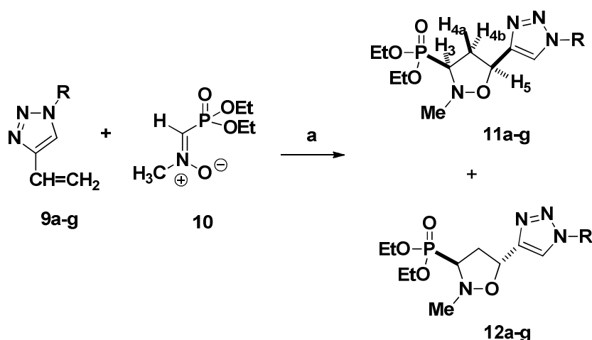
Scheme 1. Synthesis of 3-phosphonated 5-( 1H -1,2,3-triazol-4-yl)isoxazolidines 11a-g and 12a-g . Reagents and conditions: a) CH 2 Cl 2 , MW, 100 W, 2 h, 90 °C.
