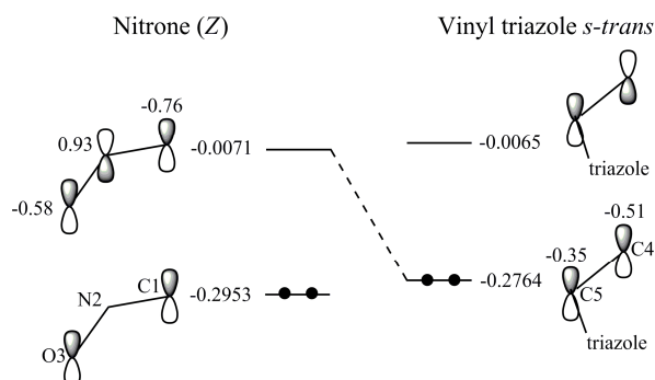
Figure 3. Energies (hartree) and coefficients of HOMO and LUMO, useful for the application of the Houk's rule (energies are not in scale).
