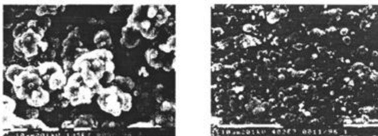
Effect of ultrasound (800kHz) on polypyrrole electrodeposition lefthand figure silent (SEM 1000x), righthand insonated (SEM 4000x).
