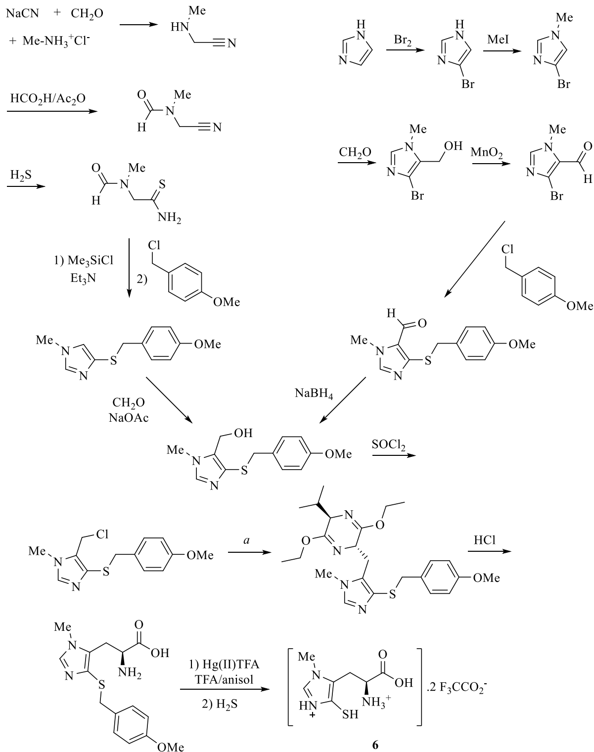
Scheme 1. The total synthesis routes proposed by Holler et al. 18,19 (left) and Ohba et al. 20,21 (right). a ( R )-2,5-Dihydro-3,6-diethoxy-2-isopropylpyrazine, n -butyllithium.
