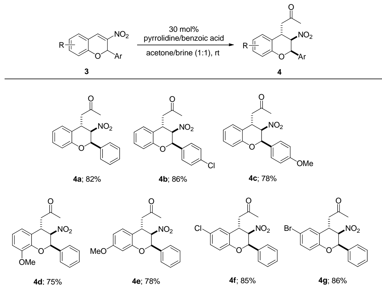
Scheme 1. Synthesis of 2,3,4-trisubstituted chromanes 4 in brine.
