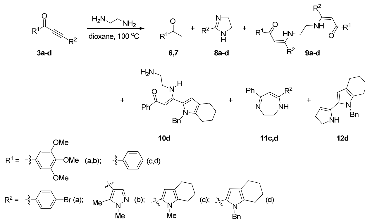
Scheme 4. Reaction of ketoacetylenes 3a-d with EDA in refluxing dioxane.
