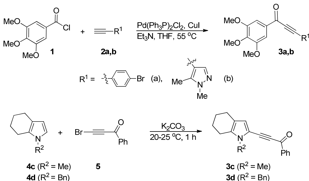
Scheme 3. Two approaches to the preparation of ketoalkynes 3a-d .
