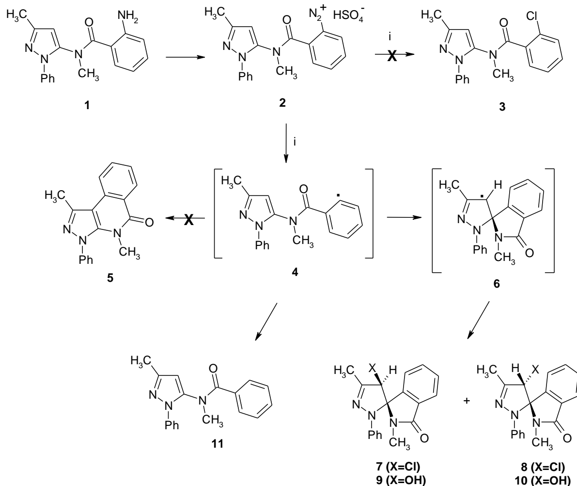
Scheme 1. i) \text{CuSO}_4 / ascorbic acid / \text{NaCl} .
