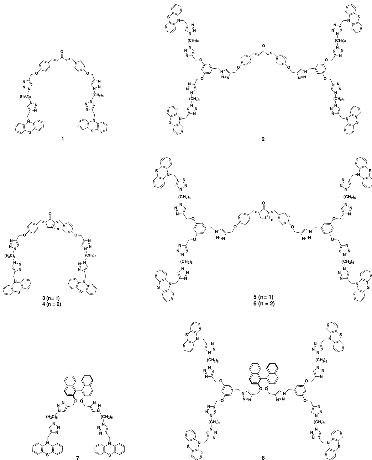
Figure 1. Molecular structure of phenthiazine dendrimers 1-8.
