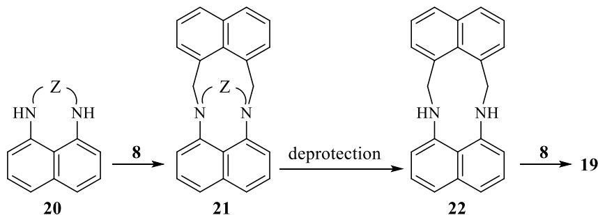
Scheme 3. Proposed synthesis of bicyclic derivative 19 .
