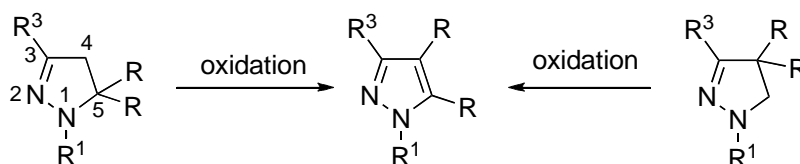
Scheme 1. The retropinacol rearrangement of 2-pyrazolines.
