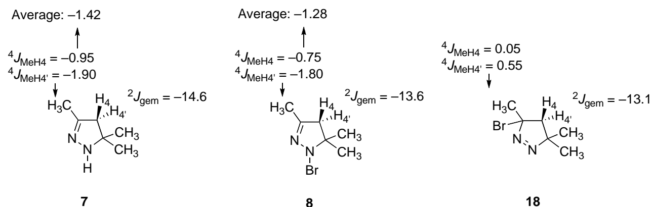
Scheme 7. Calculated [B3LYP/6-311++G(d,p)] ^1\text{H} - ^1\text{H} SSCC (in Hz).
