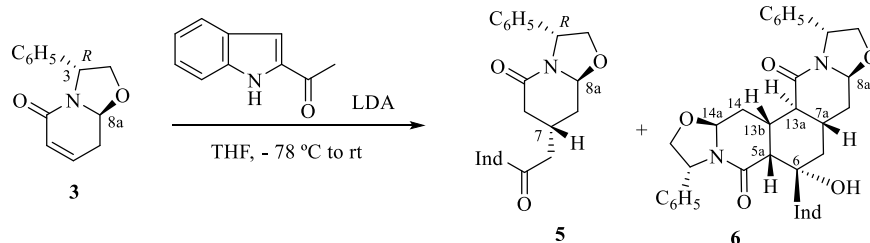
Scheme 2. Conjugate addition of 2-acetylindole enolate to unsaturated lactam 3 .
