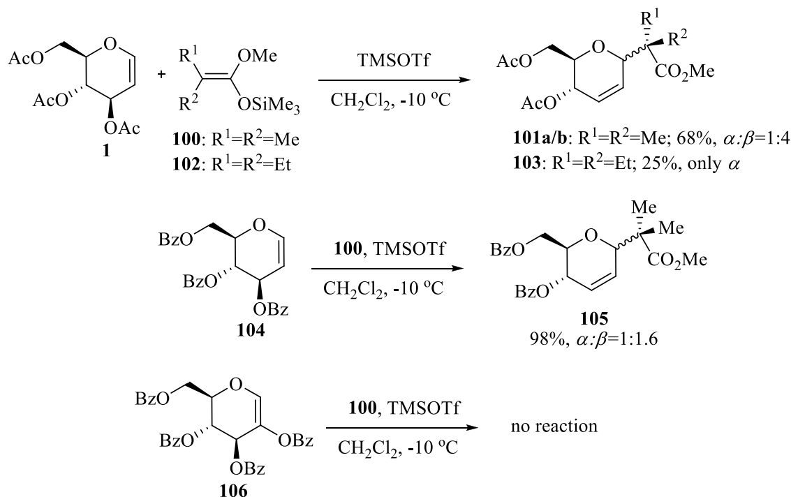
Scheme 48
