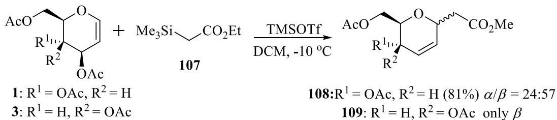
Scheme 49
