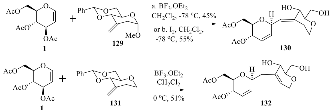
Scheme 57
