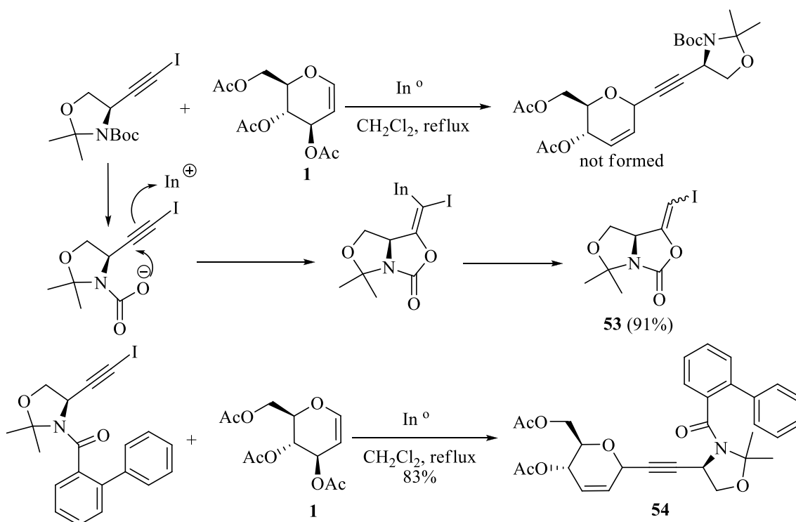
Scheme 24
