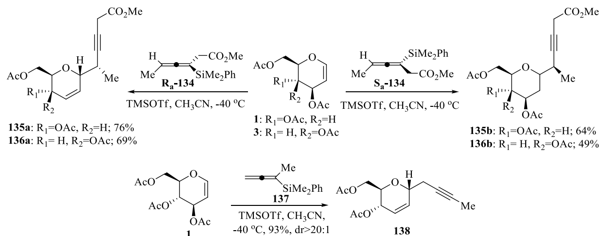
Scheme 59
