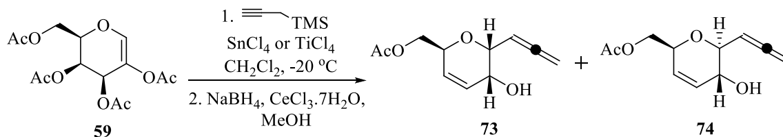
Scheme 33
