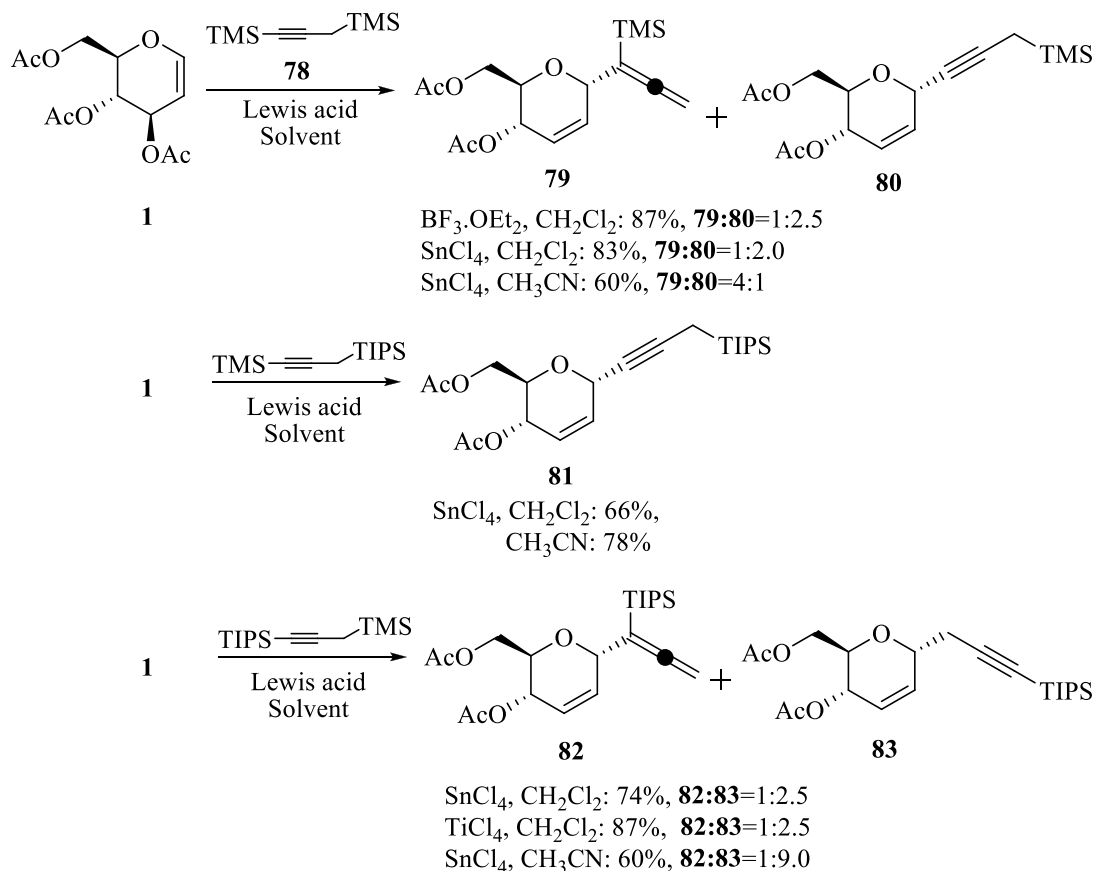
Scheme 36
