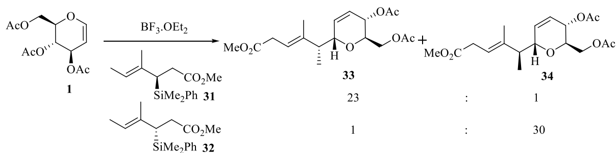
Scheme 16
