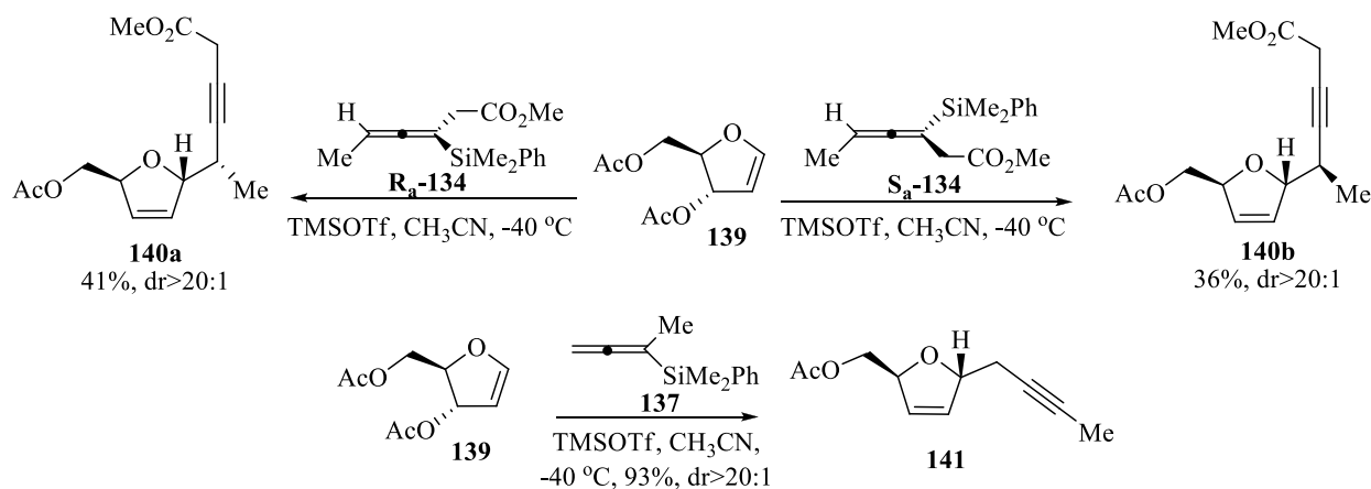
Scheme 60
