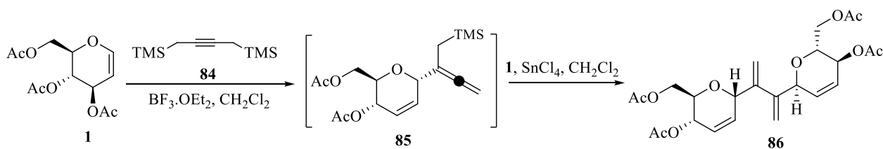
Scheme 38
