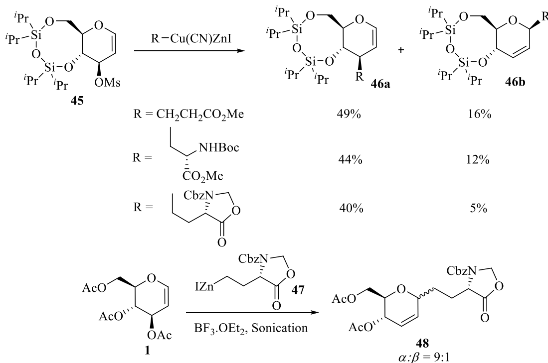
Scheme 21
