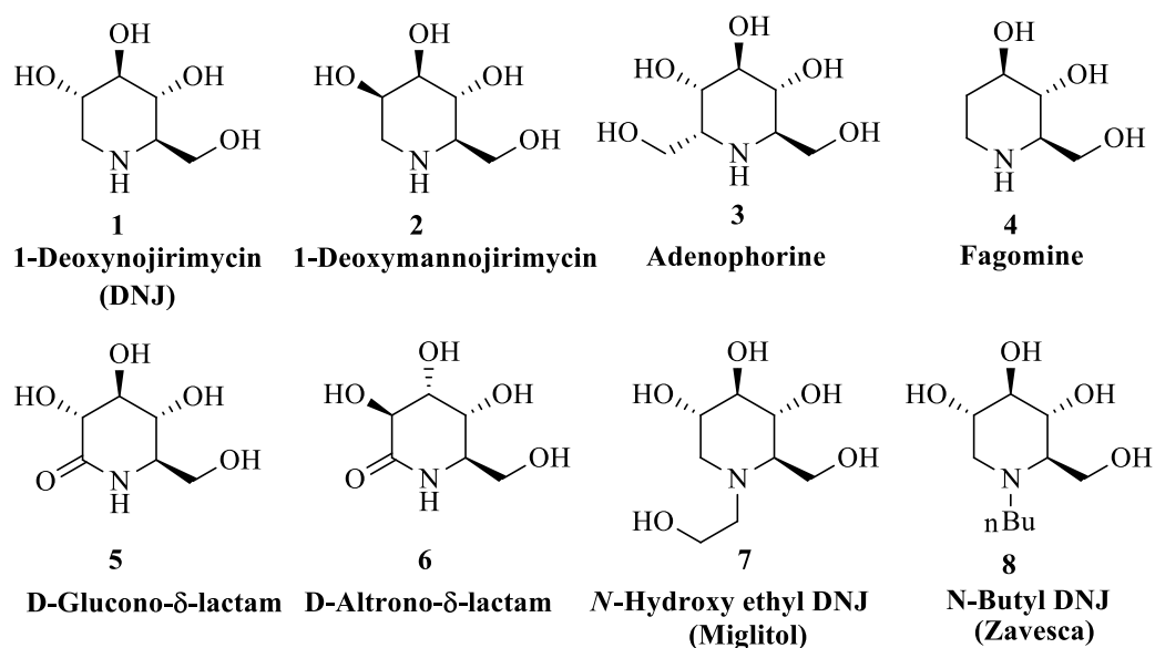
Figure 1. Some polyhydroxypiperidines.
