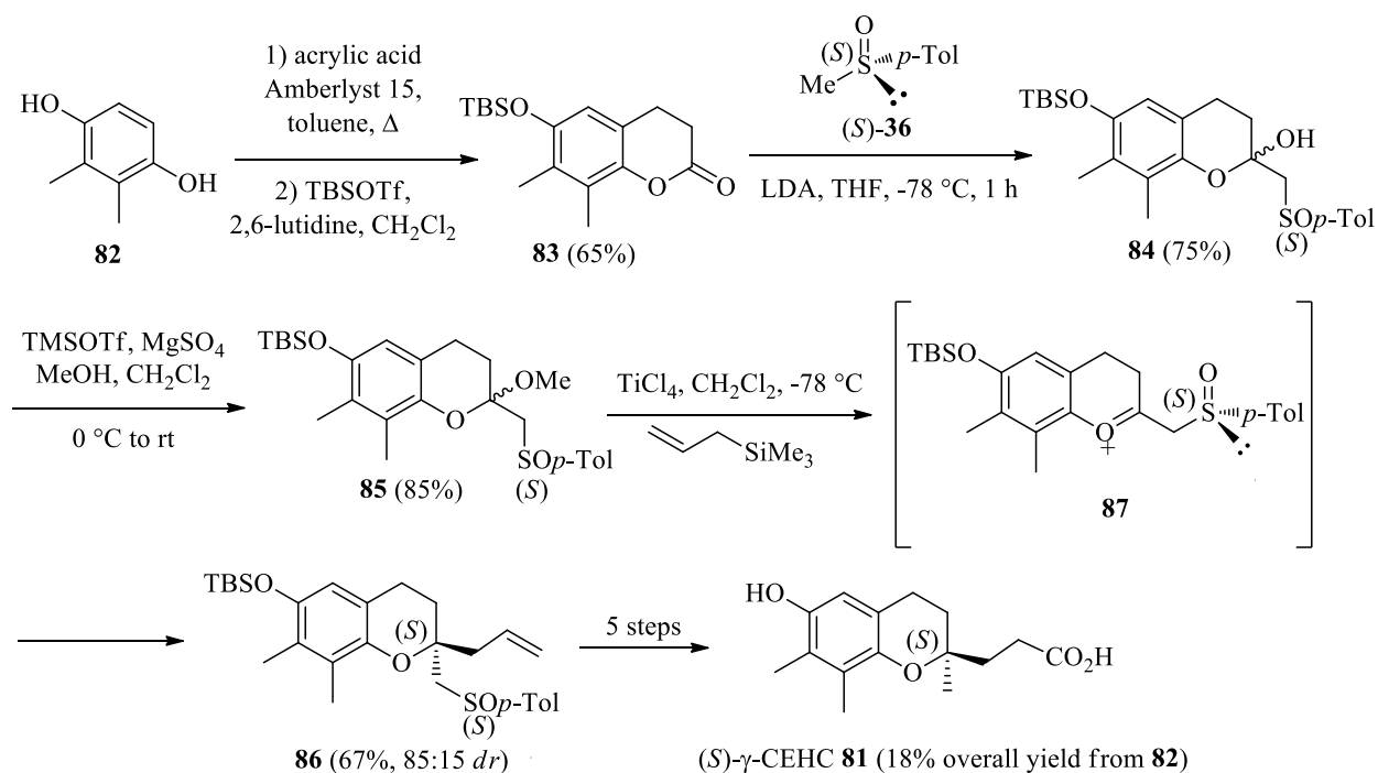
Scheme 21
